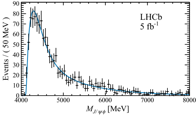
FIG. 2. Invariant-mass distribution of J/\psi\phi candidates for the sideband sample composed of events with more than four reconstructed VELO tracks. Note that all other selection requirements are applied, including the J/\psi and \phi mass-window requirements. The fit results are shown as a solid line.
