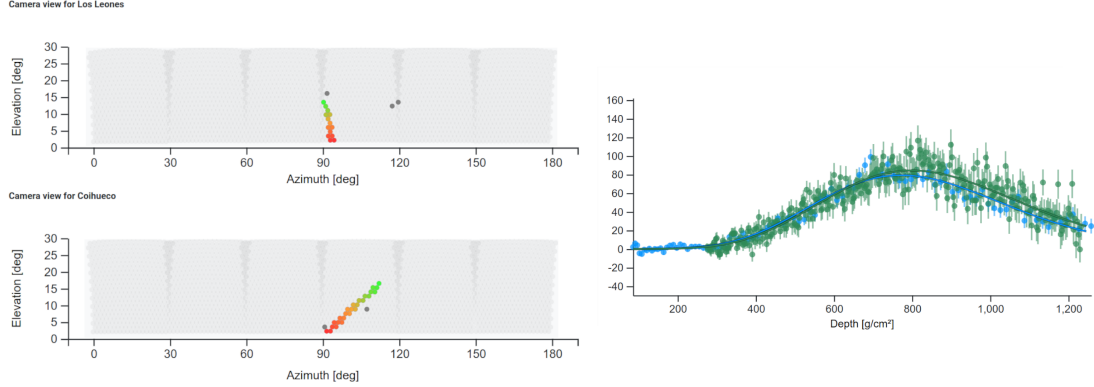
Figure 4: Visualization: the exemplary event, id 081847956000 (see text for details). Left panel: camera view of the fluorescence detector; the cosmic-ray shower is seen as a trace that moves along the pixels of the camera, from early (green) to late (red) pixels. Right panel: reconstructed energy deposit as a function of atmospheric depth as measured with the two telescopes participating in the event
