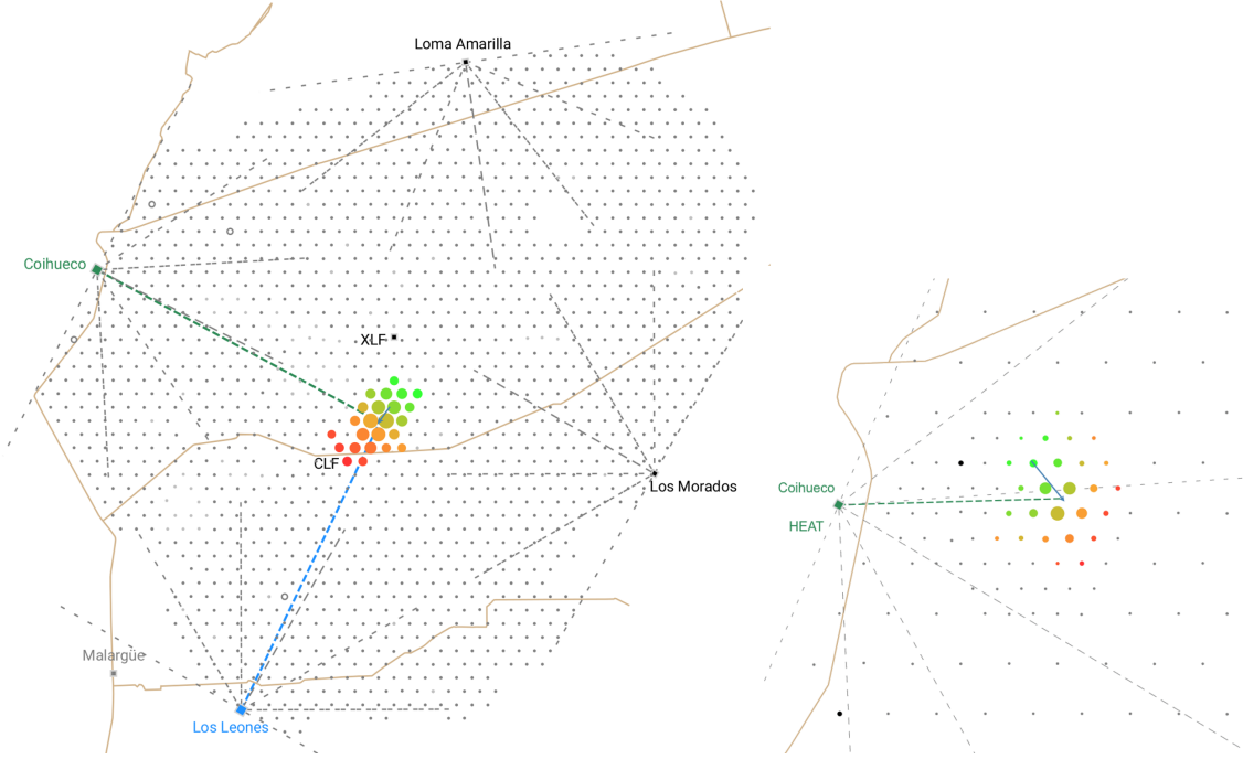
Figure 1: Map of the Observatory: left, surface detector stations (grey dots), position of the fluorescence detector eyes and field of view of the telescopes (squares, dashed lines) along with the footprint at the ground of one of the highest-energy multi-eye events in the released data sample (color scale from green to red reflects the arrival time of the shower particles at the ground). The positions of the atmospheric monitoring systems, XLF and CLF, are also shown. Right: footprint of an event detected by the SD-750 array in combination with the HEAT-Coihueco fluorescence telescopes, same color code
