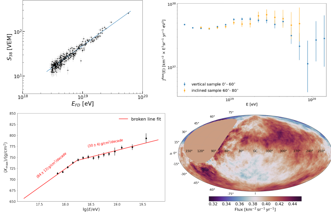
Figure 6: Analysis tab: exemplary plots resulting from the Python notebooks provided. Top left panel: energy calibration of the SD energy estimator ( S_{38} for the SD-1500 array); top right panel: energy spectrum for vertical and inclined sample; bottom left panel: depth of shower maximum as a function of primary energy; bottom right panel: flux map for events with energy above 8 EeV
