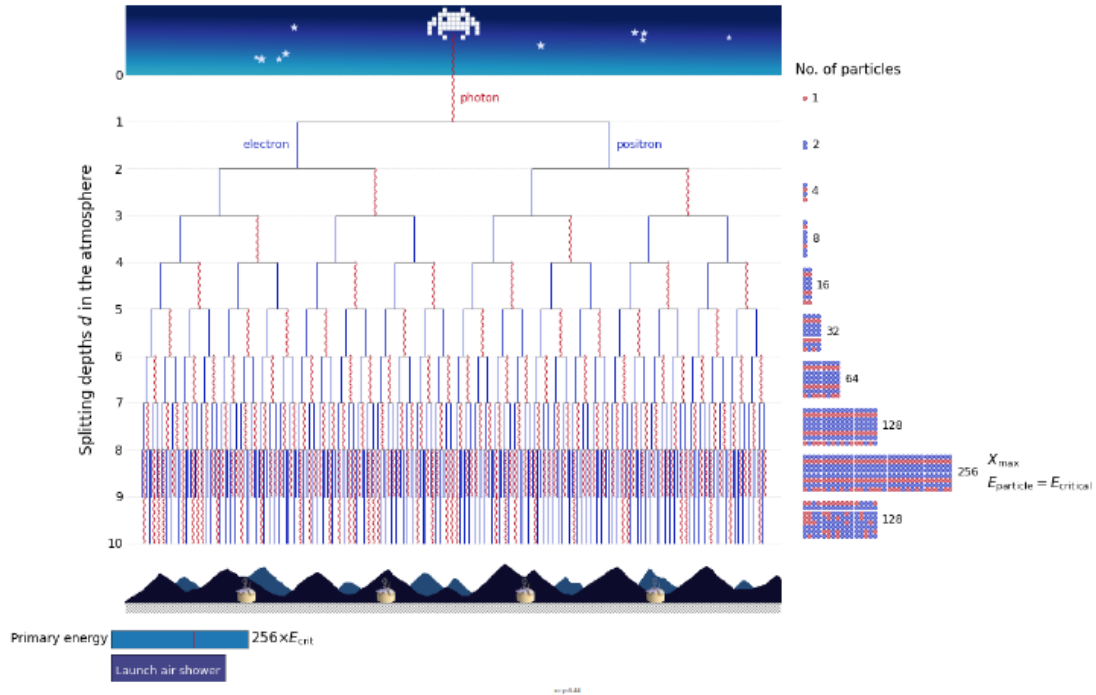
Figure 8: Toy model for the development of an electromagnetic cascade in the atmosphere
