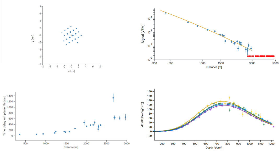
Figure 7: UHECR Catalog: the highest energy multi-eye hybrid event, PAO100815 (id 102266222400). Top left panel: footprint with respect to the shower plane; top right panel: lateral distribution of the signals as a function of the distance from the shower axis. Bottom left panel: time delays of the signals with respect to a fit with a plane shower front; bottom right panel: reconstructed energy deposited in the atmosphere
