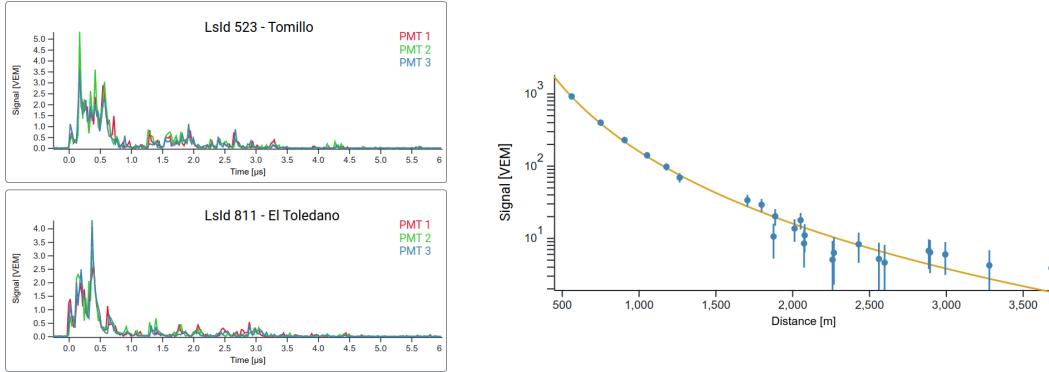
Figure 3: Visualization: the exemplary event, id 081847956000 (see text for details). Left panel: FADCs traces of the PMTs signals in two WCD stations participating in the event. Right: fall-off of the signal as a function of distance from the shower axis, the so-called lateral distribution function (LDF)
