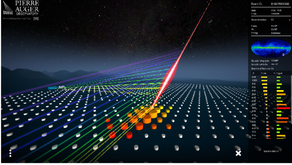
Figure 5: Visualization: a screenshot of the 3-dimensional display for the exemplary multi-eye hybrid event id 081847956000 (see text for details)
