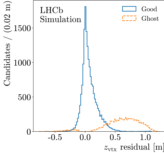
Figure 12: Residual distribution of the reconstructed \Lambda z position for \Lambda_b^0 \rightarrow J/\psi \Lambda signal candidates in simulation tagged as Good and Ghost , with true \Lambda vertex along the z axis above 6.0 m, before applying the BDT requirement.
