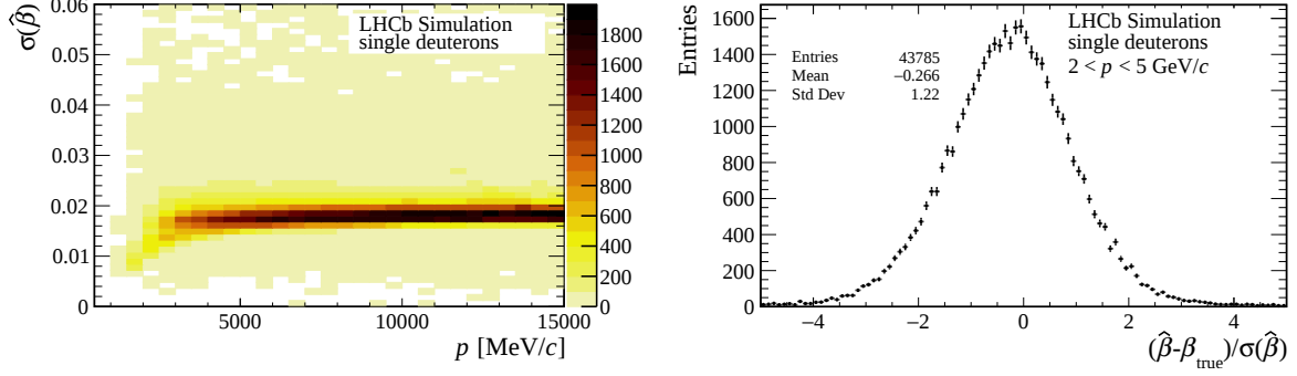
Figure 4: Performance of the \beta determination on the simulated sample of single deuteron tracks: (left) estimated uncertainty \sigma(\hat{\beta}) as a function of momentum; (right) normalised residuals for low-momentum particles.
