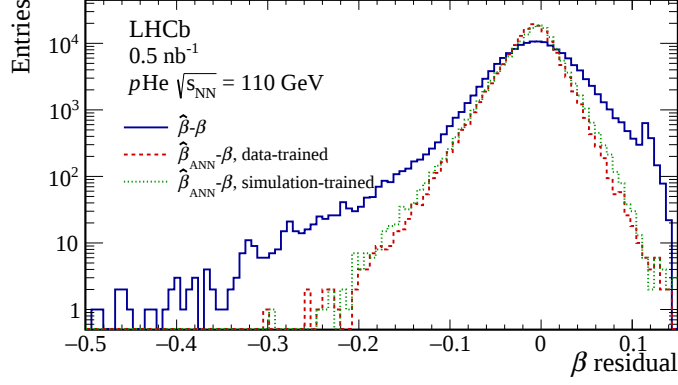
Figure 11: Performance of the \Delta\beta_{\text{ANN}} predictor on the calibration sample, for momenta lower than 5 GeV/c. The plot shows the difference between the \beta estimation and the expected value \beta = p/\sqrt{p^2 + (Mc)^2} , obtained from the measured momentum and the known mass M of the identified pion or proton. The comparison is performed on the 20% of calibration data not used for the training.
