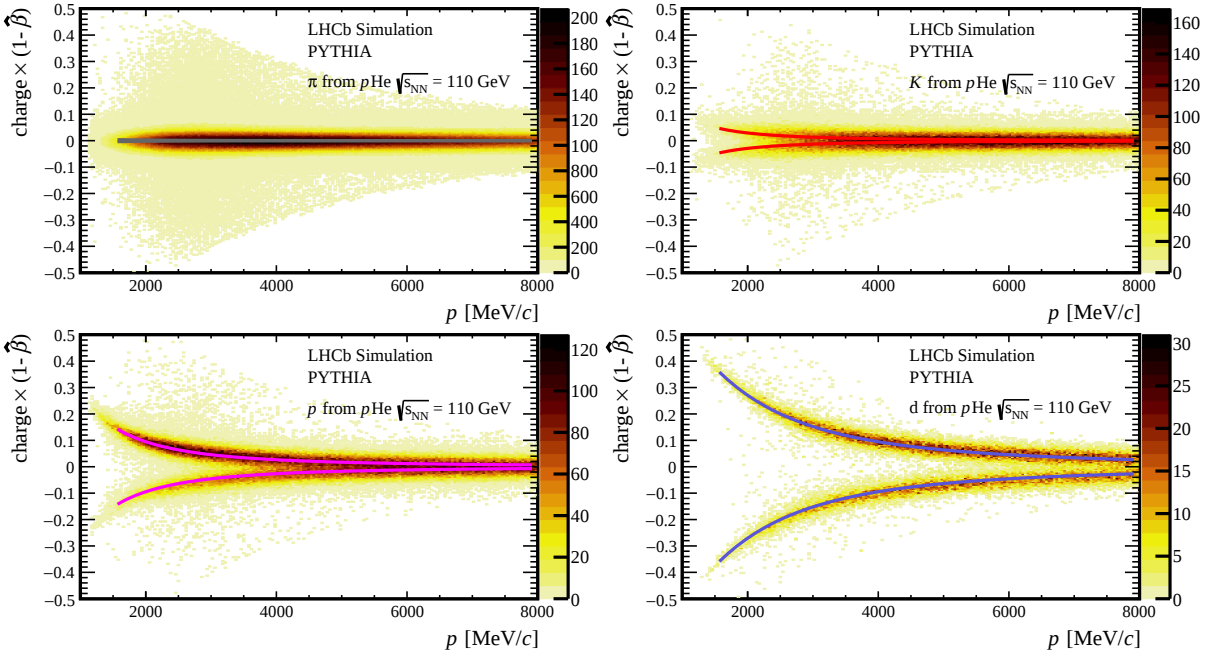
Figure 5: Difference with respect to 1 of \hat{\beta} , multiplied by the particle charge, as a function of the reconstructed momentum for four hadron species in the PYTHIA-based simulated sample: (top left) pions, (top right) kaons, (bottom left) protons and (bottom right) deuterons. The overlaid curves show the expected relations.
