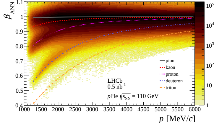
Figure 13: Estimated speed versus momentum for reconstructed tracks of positively charged particles in the p\text{He} collision sample, using the \hat{\beta}_{\text{ANN}} estimator and requiring |\Delta\beta_{\text{ANN}}| < 0.03 . The overlaid curves show the expected relations for different hadron species. Proton, deuteron and triton production can be seen. The momentum-dependent cutoff at low \beta corresponds to the maximum mass hypothesis allowed in the algorithm.
