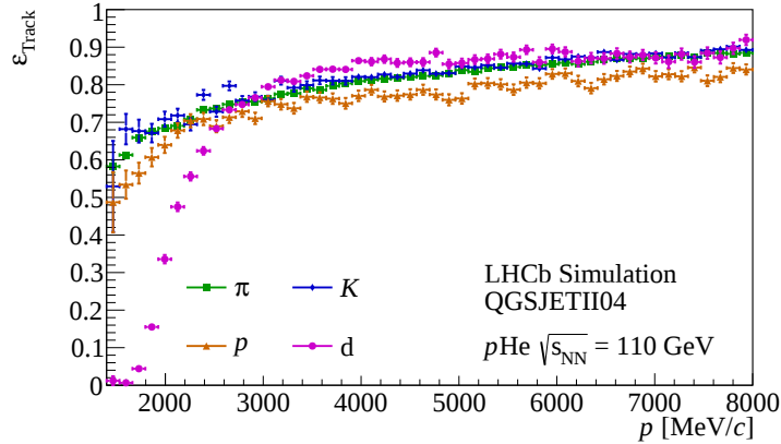
Figure 1: Track reconstruction efficiency \varepsilon_{\text{Track}} of the standard pattern recognition algorithm as a function of the momentum p for different hadron species in the QGSJET-based simulation sample.
