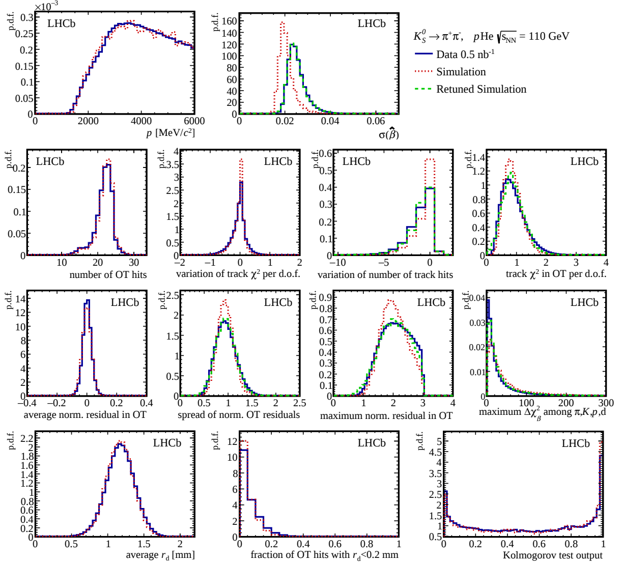
Figure 10: Distributions of the 13 observables, described in Sec. 3, used as input to the \Delta\beta_{\text{ANN}} predictor network. Data and simulation are compared for candidate pion tracks from K_S^0 decays with momentum below 6 \text{ GeV}/c . For six variables, notably \sigma(\hat{\beta}) , an empirical correction is applied to the simulated observables to improve the agreement with data.
