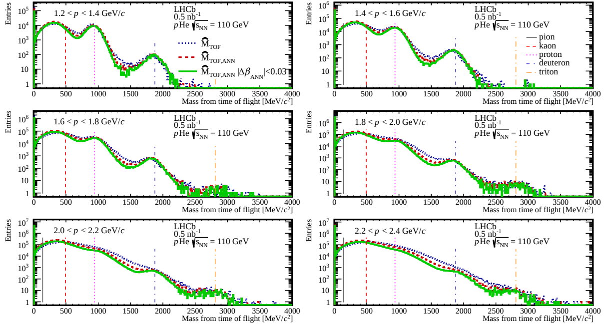
Figure 12: Estimated particle mass from the time of flight for reconstructed tracks of positively charged particles in the p\text{He} collision sample, for different momentum intervals. \hat{M}_{\text{TOF,ANN}} is obtained by replacing \hat{\beta} with \hat{\beta}_{\text{ANN}} in Eq. 2. The vertical lines correspond to the known mass of pions, kaons, protons, deuterons and tritons.
