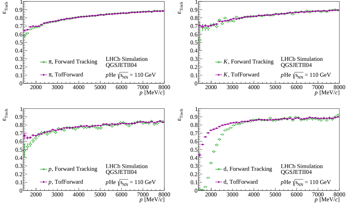
Figure 2: Track reconstruction efficiency as a function of the momentum for (top left) pions, (top right) kaons, (bottom left) protons and (bottom right) deuterons; the performance of (empty markers) the standard Forward Tracking algorithm and of (full markers) the TofForward algorithm is compared.
