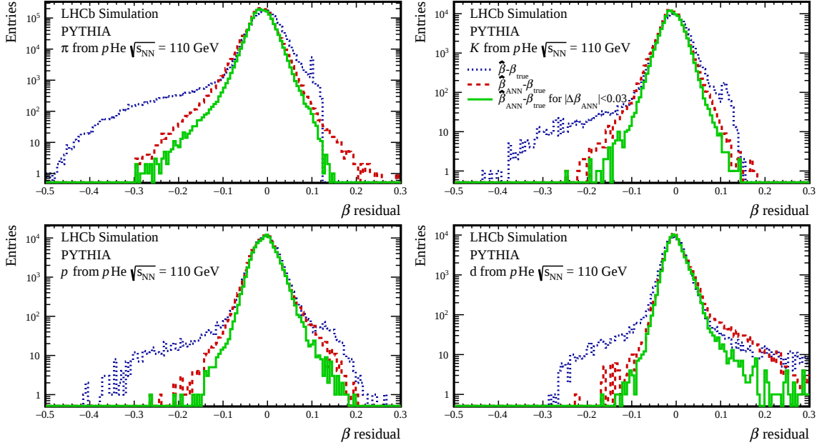
Figure 9: Impact of the use of the \Delta\beta_{\text{ANN}} predictor on the accuracy of the \beta determination for different hadron species in simulated collisions, for tracks with momentum lower than 5 GeV/c.
