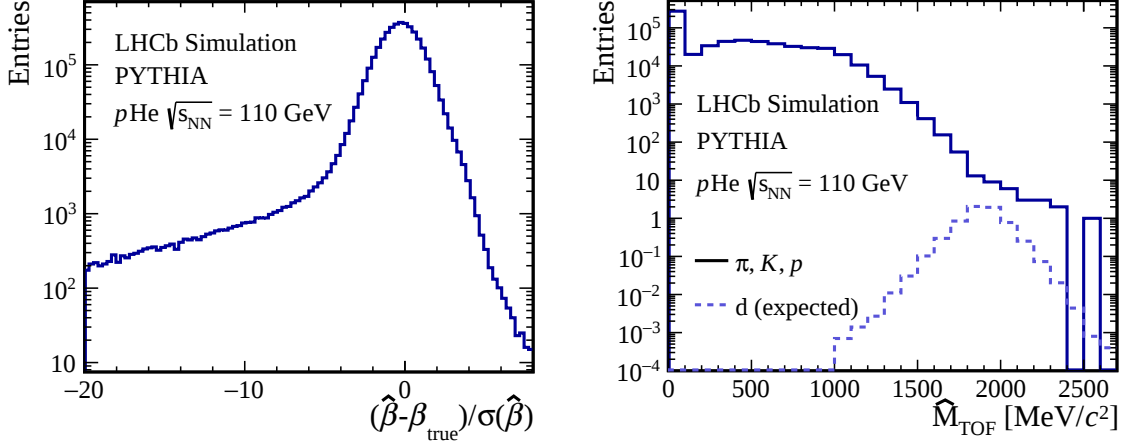
Figure 6: (Left) Residual of the \beta estimation normalised by its estimated uncertainty for simulated positively charged particles with momentum below 4 GeV/c. (Right) Distribution of the corresponding estimated mass \hat{M}_{\text{TOF}} , separately for deuterons and lighter particles, assuming that a deuteron is produced approximately one out of every 10^4 collisions.
