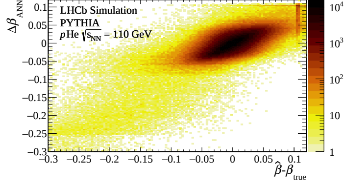
Figure 8: Performance of the \Delta\beta_{\text{ANN}} predictor on simulated collisions. The response is shown for all track candidates with momentum lower than 5 GeV/c. The structure at \Delta\beta = 0.1 is an artifact from the limit \beta < 1.1 on the sampled values.
