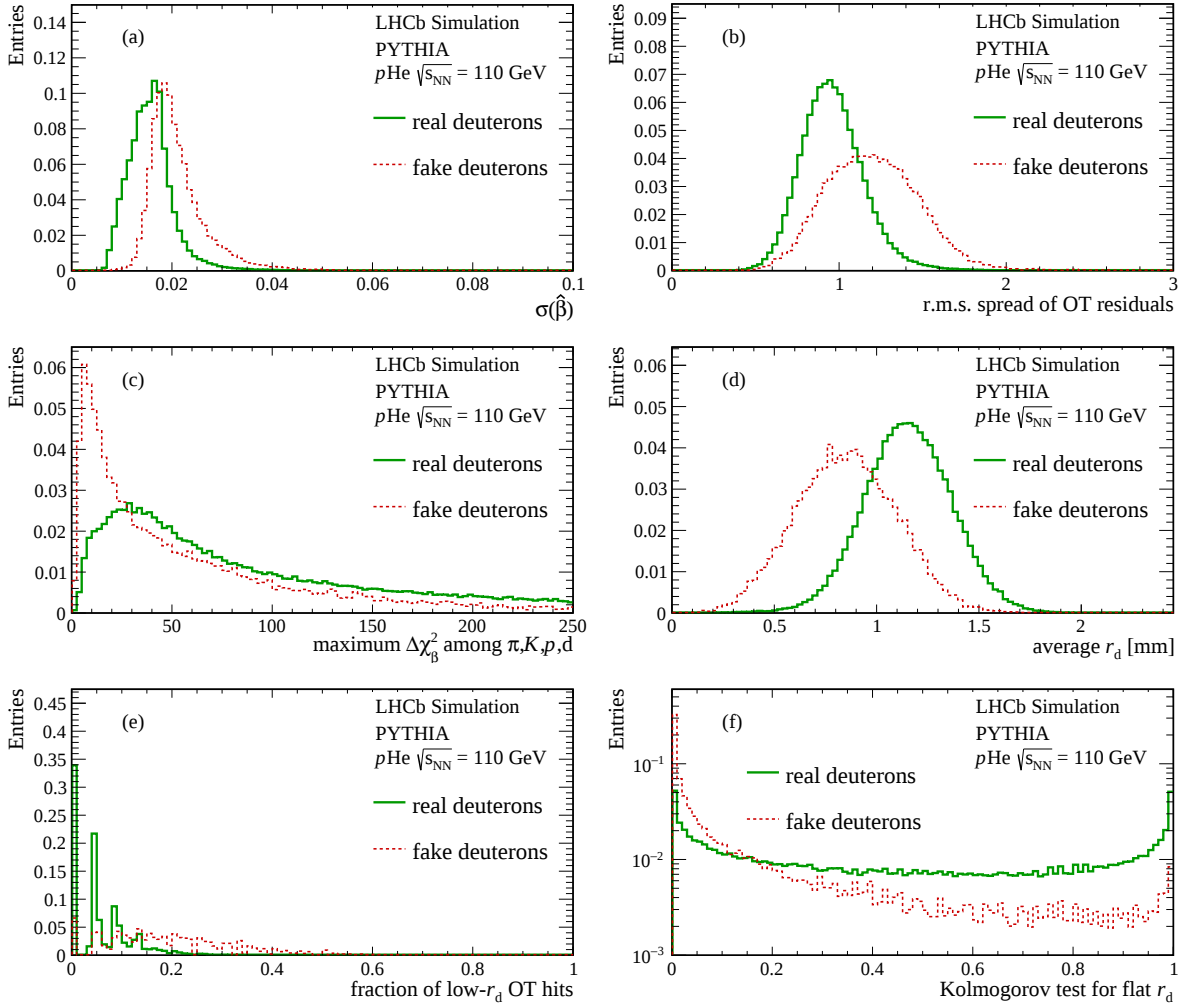
Figure 7: Distributions in simulation of some of the observables used to discriminate genuine deuterons from lighter particles with an \hat{M}_{\text{TOF}} value compatible with the deuteron mass (fake deuterons), for tracks with momentum lower than 3 \text{ GeV}/c .
