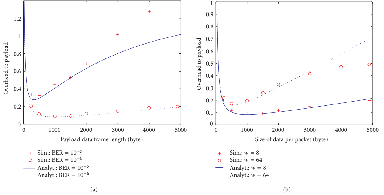
FIGURE 10: TCP layer Go-back-N ARQ validation and evaluation. The protocol overhead to payload ration in dependency on the frame length of the payload data is depicted. The lines are analytic results corresponding to (2), while the markers indicate simulative evaluation. (a) Varied BER = 10 -5 or 10 -6 and window length w = 8 . (b) Varied window length w = 8 or 64 and BER = 10 -6 .
