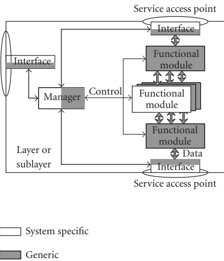
FIGURE 4: Composition of a protocol specific layer or sublayer on the basis of generic and system-specific functional modules.
