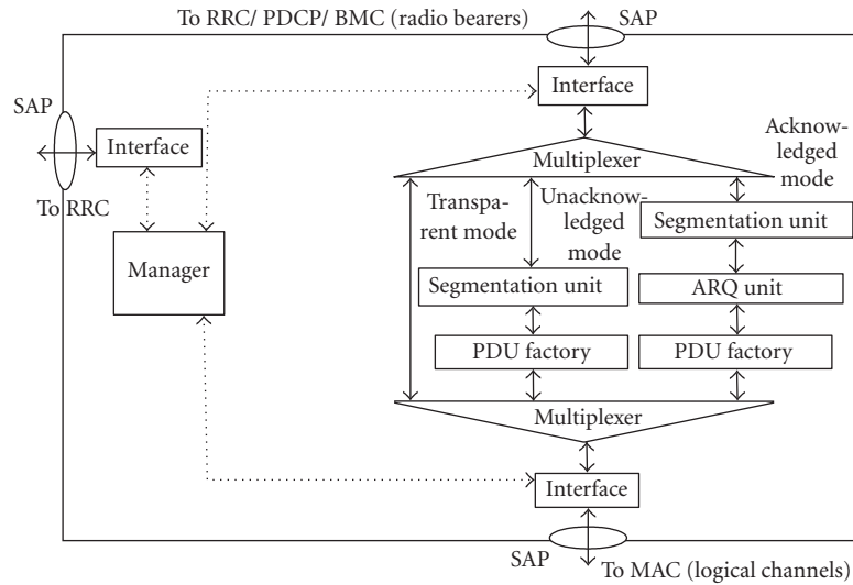
FIGURE 6: UMTS RLC layer based on the functional modules of the generic protocol stack.
