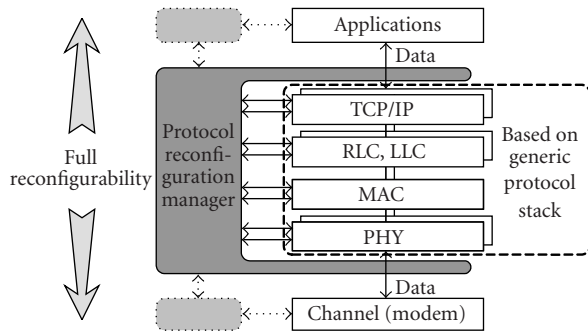
FIGURE 2: A reconfigurable protocol stack based on generic functional modules in the context of a completely reconfigurable terminal.
