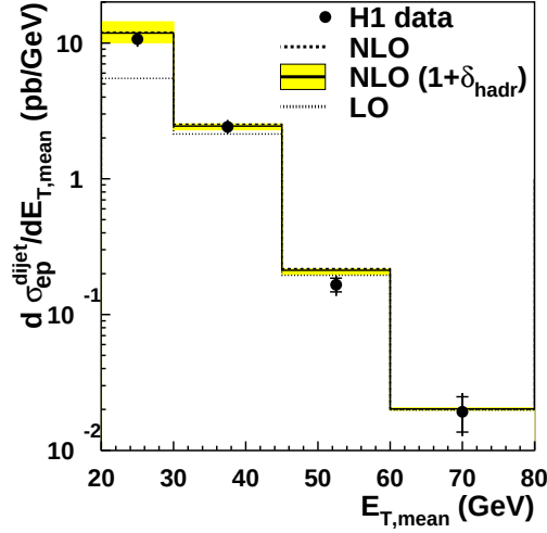
Fig. 6. Dijet cross section d\sigma/dE_{T,\text{mean}} as a function of E_{T,\text{mean}}
