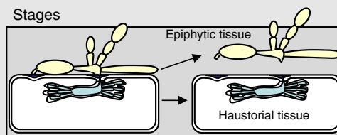
Figure 1 Summary of bioinformatics and expression analysis of CSEPs. Identification of CSEPs and family assignment. Workflow used to find and annotate CSEPs in the genome of B. graminis f.sp. hordei . After three iterative rounds of BLAST and annotation, genes were clustered into families as described in Methods. Protein analyses. The proteins predicted to be translated from the CSEP ORFs were analyzed to infer their 3D structure and presence of conserved motifs. These were then used to investigate evidence of different selection pressures during the course of evolution of the CSEP families. Expression analysis. Evidence to support the existence of CSEP genes was obtained from ESTs in the public databases, from RNAseq surveys and from the analysis of the proteomes of B. graminis and B. graminis -infected barley tissues by mass-spectrometry.
