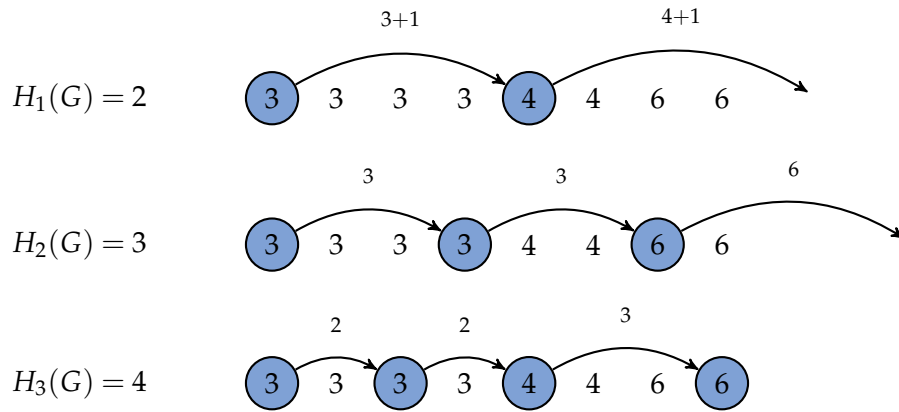
Figure 6.6: The principle of the H_k -algorithm
