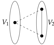
Figure 7.1: Extremal graph H with \pi(H) = (2, 2, 2)
