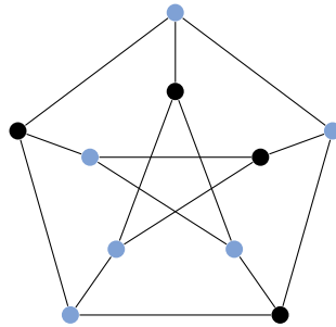
Figure 1.1: Petersen graph G with \alpha(G) = 4 (black) and \alpha_2(G) = 6 (blue)
