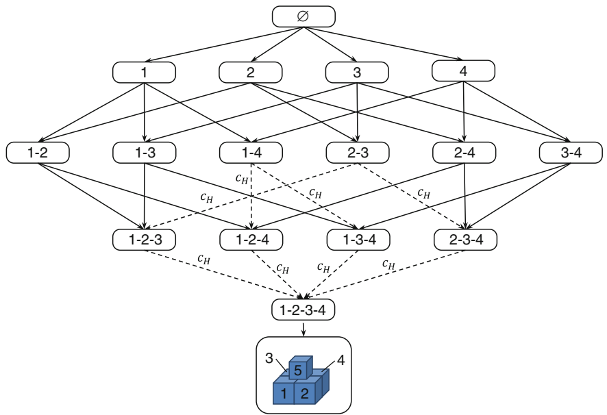
Fig. 11.2 Exemplary state graph of a simple product consisting of cubic parts. The dotted edges indicate assembly steps that have to be carried out by the human operator due to the technical restrictions of a two finger gripper (Faber et al. 2014)
