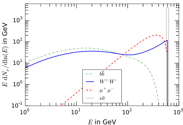
Fig. 4 Muon neutrino multiplicity per annihilation dN_\nu/d \ln(E) as function of energy is shown for the investigated benchmark channels and m_\chi = 600 GeV. The oscillation probability into muon neutrinos, in the long baseline limit, is included in dN_\nu/d \ln(E) . Beside the neutrino line spectrum, the spectra were calculated with DarkSUSY [37]
