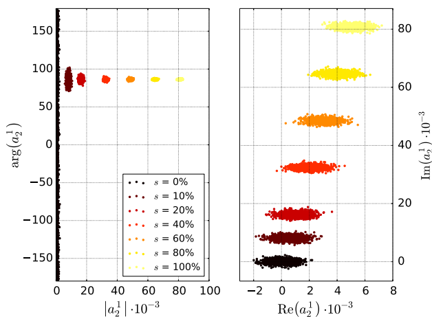
Fig. 6 The expansion coefficient a_2^1 for large signal strength s in the Euler representation (left panel) and in the complex plane (right panel). For each signal strength s 1,000 pseudo-experiments were generated and the expansion coefficient a_2^1 calculated
