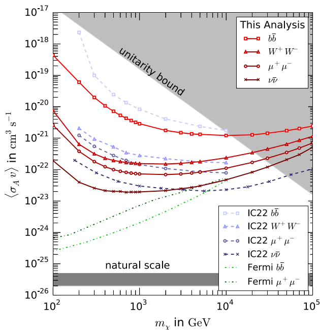
Fig. 17 Exclusion limits on dark matter self-annihilation cross-section from outer Galactic halo searches only. The results of this analysis and exclusion limits from the predecessor analysis of IceCube-22 [20] (both 90% CL) and from the Fermi-LAT [53] ( 3\sigma CL) are shown. The baseline limit curves are calculated for the NFW profile, however different normalization parameter are used. For reasons of comparison the limits from IC22 and Fermi are rescaled to the local density of \rho_{SC} = 0.47 \text{ GeV/cm}^3 that is used in this analysis. The gray band describes the natural scale if all dark matter consists of WIMPs and the gray upper region is excluded by the unitarity bound [5]
