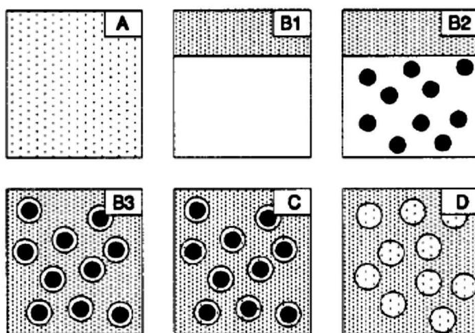
Figure 1-4: Groups of organic solvent reaction media. A) water-miscible solvent, B1) two-phase system with low volume organic solvent and solubilized biocatalyst, B2) two-phase system with low volume organic solvent and immobilized biocatalyst, B3) two-phase system with high volume organic solvent and immobilized biocatalyst, C) micro-aqueous system, D) reverse micelles. White area represents water, small black dots represent organic solvent, big black dots represent biocatalyst, and white dots represent micelles. This figure was taken from (Vermue and Tramper, 1995) under a free common license.
