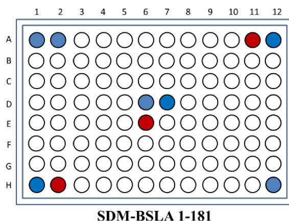
Figure 2-2: Scheme for MTP arrangement of generated SDM libraries. White colored wells contain SDM-BSLA variants, blue colored wells contain the WT (positive control: A1; A2, A12, D6, D7, H1, and H12) and red colored wells contain the EV (negative control, A1, E6, and H2).
