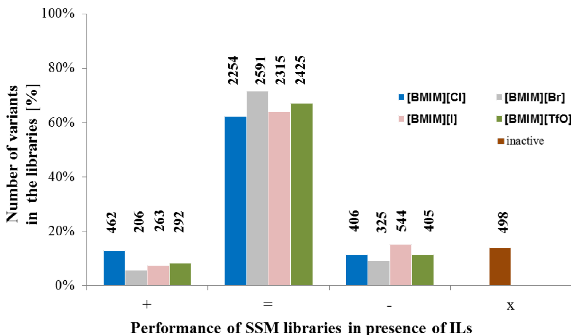
Figure 3-3: Number of SSM-BSLA variants, which lead to improved/unchanged/decreased IL resistance towards four ILs and/or inactivation of BSLA in buffer. All SSM-BSLA variants were grouped as described in the text: “+” representing variants with improved resistance, “=” representing variants with unchanged resistance, “-” representing variants with decreased resistance and “x” representing inactive variants in buffer.
