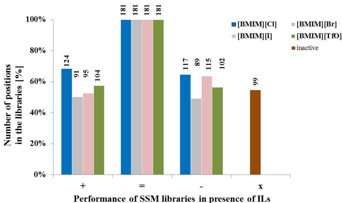
Figure 3-2: Number of amino acid positions, which lead to improved/unchanged/decreased IL resistance and/or inactivation of BSLA in buffer. All SSM-BSLA variants were grouped as described in the text: “+” representing variants with improved resistance, “=” representing variants with unchanged resistance, “-” representing variants with decreased resistance and “x” representing inactive variants in buffer.
