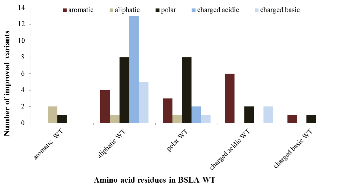
Figure 3-9: Number of improved variants with >2.5-fold improved IL resistance according to the amino acid substitution of BSLA WT for all four ILs. Variants with a value >2.5-fold are represented here. The nature of the substitution for each variant is also illustrated. Amino acids are grouped into: aromatic (F, Y, and W), aliphatic (A, V, L, I, and G), charged acidic (D, E), charged basic (H, K, and R), and polar (C, M, P, S, T, N, and Q).
