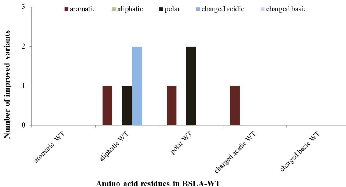
Figure 4-8: Number of improved variants according to the amino acid substitution of BSLA WT in all three OS. Variants with a value \geq 2.5 -fold are represented here. The nature of the substitution for each variant is also illustrated. Amino acids are grouped into: aromatic (F, Y, and W), aliphatic (A, V, L, I, and G), charged acidic (D, E), charged basic (H, K, and R), and polar (C, M, P, S, T, N, and Q).
