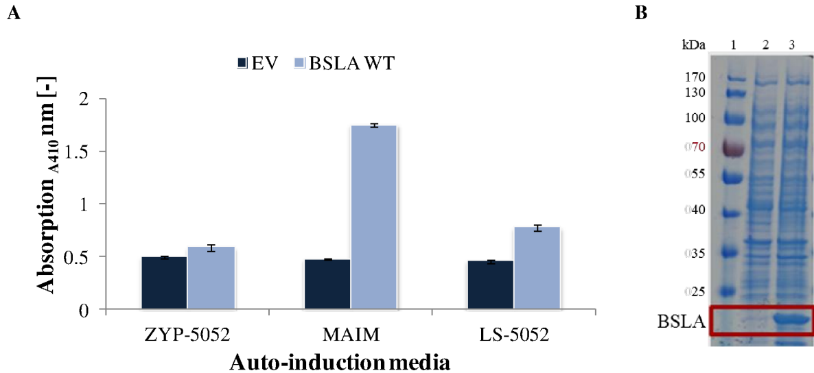
Figure 2-5: Comparison of BSLA WT activity in different auto-induction media (A) and BSLA protein expression in MAIM (B). A: ZYP-5052; MAIM and LS-5052 were used for expression followed by activity assay with p NPP as substrate. All measurements were performed in triplicate and errors were calculated and are represented as bar. B: Protein visualization of BSLA cultures on a 12% SDS-PAGE gel: 1) Molecular weight standard (PageRuler, Fermentas), 2) EV (empty vector), 3) BSLA WT. The red box marks the expected molecular weight of BSLA WT \approx 19.3 kDa.
