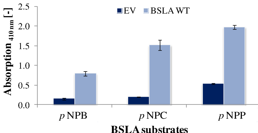
Figure 2-7: Comparison of BSLA WT activity using p NPB, p NPC, and p NPP. Endpoint measurement was performed at 410 nm (after 10 min incubation at RT) to determine BSLA WT activity with p NPB, p NPC and p NPP as substrates. All measurements were performed in sextuple and errors were calculated and are represented as bar.
