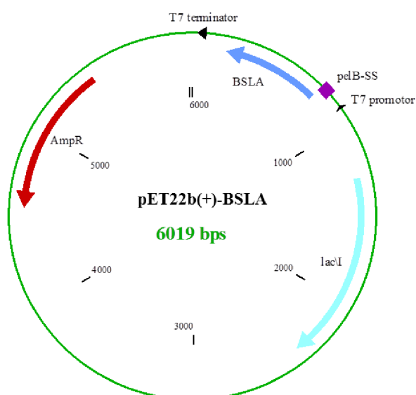
Figure 7-2: Plasmid map of pET22b(+)-BSLA. The expression vector pET22b(+) contains the gene bsla encoding for lipase A from Bacillus subtilis . SS: signal sequence, pelB-SS is the sequence responsible for periplasmid localization. Amp R : ampicillin resistance. LacI: gene encoding for the lactose repressor.
