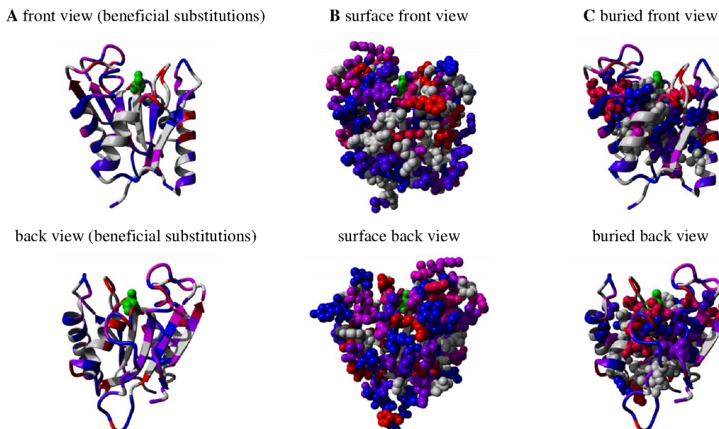
Figure 3-5: 3D model of BSLA (Protein Database code: 116W) displaying regions which contribute to the resistance of BSLA towards [BMIM][Cl] with a color scale. Positions at which no substitution led to improvements are colored grey. Positions with one substitution leading to improvements are colored blue. Positions with two to seven substitutions leading to improvements are colored purple (two positions) to magenta (seven positions). Red represents positions with eight or more substitutions leading to improvements. The active site residue Ser 77 is colored green. A) Cartoon representation of BSLA, B) Van der Waals representation of surface residues of BSLA, C) Van der Waals representation of buried residues of BSLA. The two N-terminal amino acids (Ala1 and Glu2) are also included. Yasara was used for visualization.
