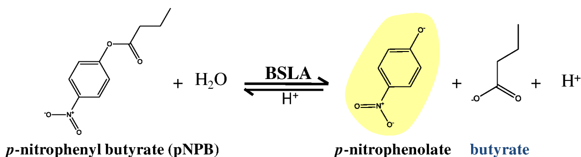
Figure 2-3: Schematic overview of an assay based lipase hydrolysis reaction. p -Nitrophenyl butyrate ( p NPB) was used as substrate. The formation of p -nitrophenolate is detected by the intensity of the yellow color at 410 nm.
