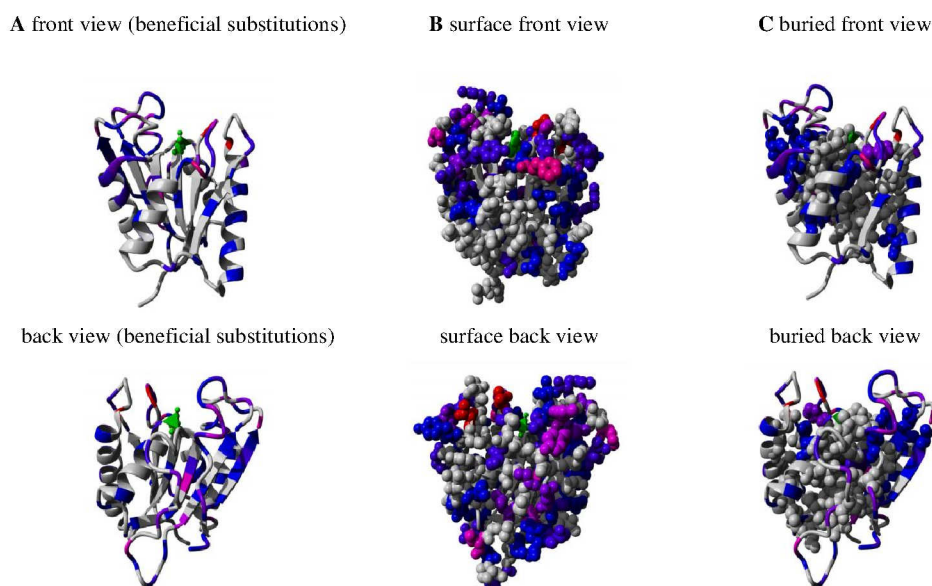
Figure 4-6: 3D model of BSLA (Protein Database code: 1I6W) displaying regions which favor BSLA resistance in presence of 1,4-dioxane in a color scale. Positions at which no substitution led to improvements are colored grey. Positions with one substitution leading to improvements are colored blue. Positions with two to seven substitutions leading to improvements are colored purple (two positions) to magenta (seven positions). Red represents positions with eight or more substitutions leading to improvements. The active site residue Ser 77 is colored green. A) Cartoon representation of BSLA, B) Van der Waals representation of surface residues of BSLA, C) Van der Waals representation of buried residues of BSLA. The two N-terminal amino acids (Ala1 and Glu2) are also included. Yasara was used for visualization.
