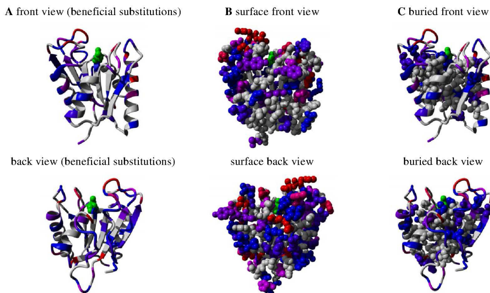
Figure 3-7: 3D model of BSLA (Protein Database code: 1I6W) displaying regions which favor BSLA resistance in presence of [BMIM][I] in a color scale. Positions at which no substitution led to improvements are colored grey. Positions with one substitution leading to improvements are colored blue. Positions with two to seven substitutions leading to improvements are colored purple (two positions) to magenta (seven positions). Red represents positions with eight or more substitutions leading to improvements. The active site residue Ser 77 is colored green. A) Cartoon representation of BSLA, B) Van der Waals representation of surface residues of BSLA, C) Van der Waals representation of buried residues of BSLA. The two N-terminal amino acids (Ala1 and Glu2) are also included. Yasara was used for visualization.
