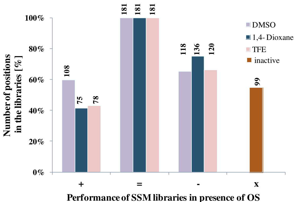
Figure 4-2: Number of amino acid positions which lead to improved/unchanged/decreased OS and/or inactivation of BSLA in buffer. All SSM-BSLA variants were grouped as described in the text: “+” representing variants with improved resistance, “=” representing variants with unchanged resistance, “-” representing variants with decreased resistance and “x” representing inactive variants in buffer.
