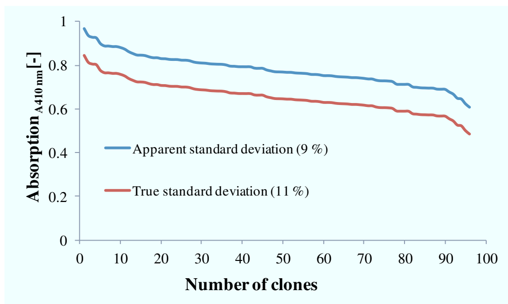
Figure 2-9: Standard deviation of BSLA activity in buffer. Activity values in decreasing order of the BSLA WT in a 96-well MTP using the optimized assay conditions. The apparent standard deviations were calculated without subtracting the background and the true standard deviations after background subtraction.
