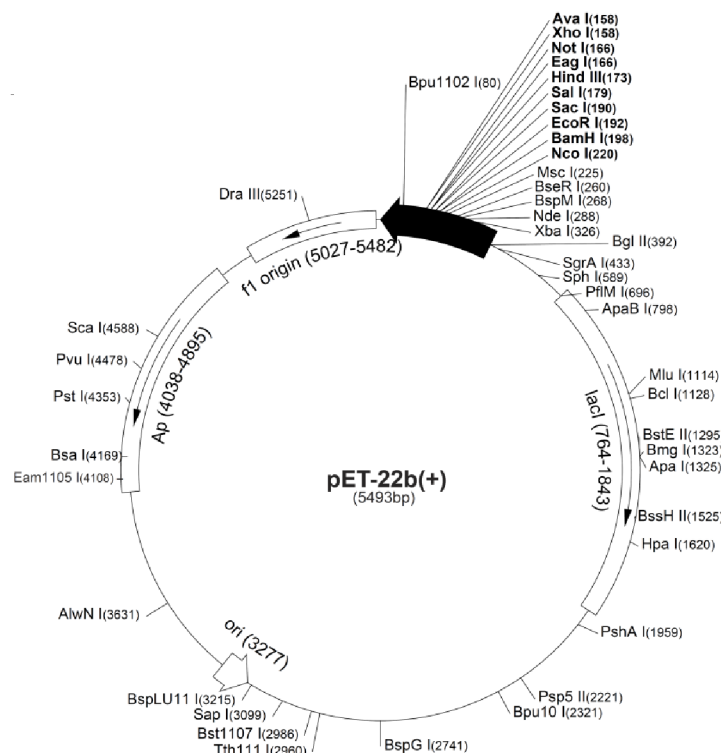
Figure 7-1: Plasmid map of the expression vector pET22b(+) from Novagen (Cat. No. 69744-3). Ap: ampicillin resistance. The black arrow represents the multiple cloning site (MCS).
