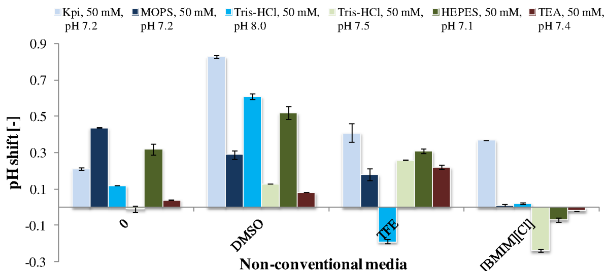
Figure 2-8: Comparison of buffer capacity for BSLA screening. The co-solvents (50% v/v) were incubated with BSLA culture supernatants (2h, RT, 1000 rpm) and substrate solution was added. Afterwards, pH values were measured and pH shifts were calculated (expected pH - measured pH). The measurements were performed in triplicate and errors were calculated and are represented as bar. DMSO: dimethyl sulfoxide; TFE: 2,2,2-trifluoroethanol; [BMIM][Cl]: 1-Butyl-3-methylimidazolium chloride.
