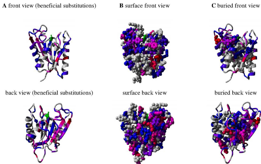
Figure 4-5: 3D model of BSLA (Protein Database code: 1I6W) displaying regions which favor BSLA resistance in presence of DMSO in a color scale. Positions at which no substitution led to improvements are colored grey. Positions with one substitution leading to improvements are colored blue. Positions with two to seven substitutions leading to improvements are colored purple (two positions) to magenta (seven positions). Red represents positions with eight or more substitutions leading to improvements. The active site residue Ser 77 is colored green. A) Cartoon representation of BSLA, B) Van der Waals representation of surface residues of BSLA, C) Van der Waals representation of buried residues of BSLA. The two N-terminal amino acids (Ala1 and Glu2) are also included. Yasara was used for visualization.
