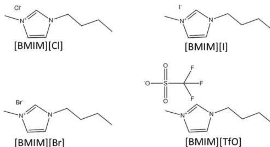
Figure 3-1: Chemical structures of the four selected ILs. [BMIM][Cl], [BMIM][Br], [BMIM][I], and [BMIM][TfO]. [BMIM] = 1-butyl-3-methylimidazolium [Cl] = chloride; [Br] = bromide, [I] = iodide, [TfO] = trifluoromethanesulfonate.
