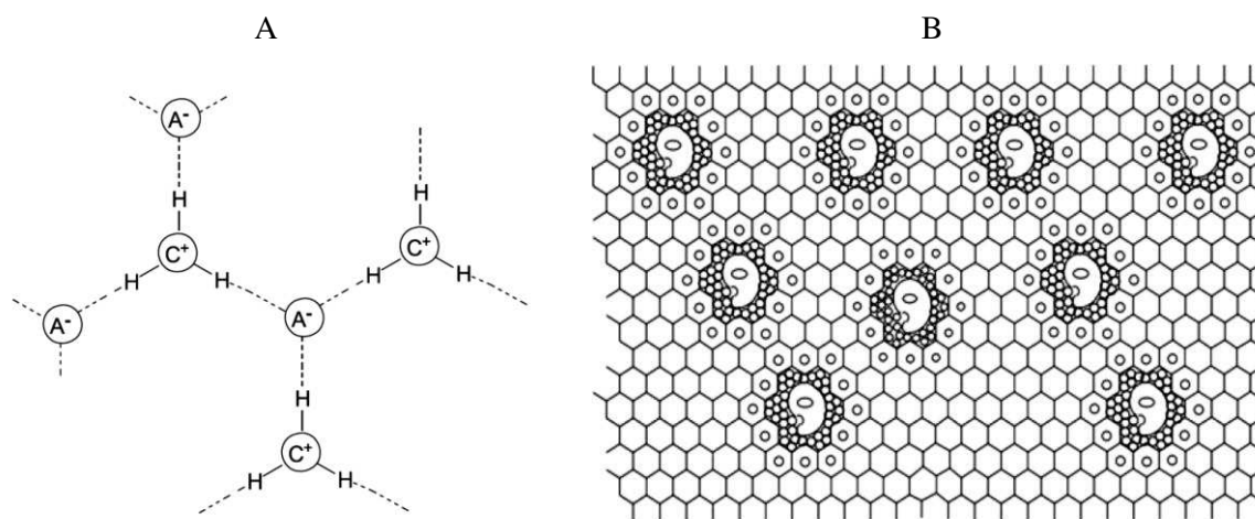
Figure 1-2: Two-dimensional simplified solid-state model of the polymeric supramolecular structure of 1,3-dialkyl imidazolium ILs and ILs's network. A: Two-dimensional simplified solid-state model of the polymeric supramolecular structure of 1,3-dialkyl imidazolium ILs illustrating the hydrogen bonds between the imidazolium cation (C) and the anions (A) (one cation is surrounded by three anions and vice-versa). B: Enzymes with a small amount of water are firmly trapped in the network of ILs. Figure A reproduced from (Dupont, 2004) under a creative common license and figure B from (Fehér et al. , 2007) with the permission of the Biochemical Society.
