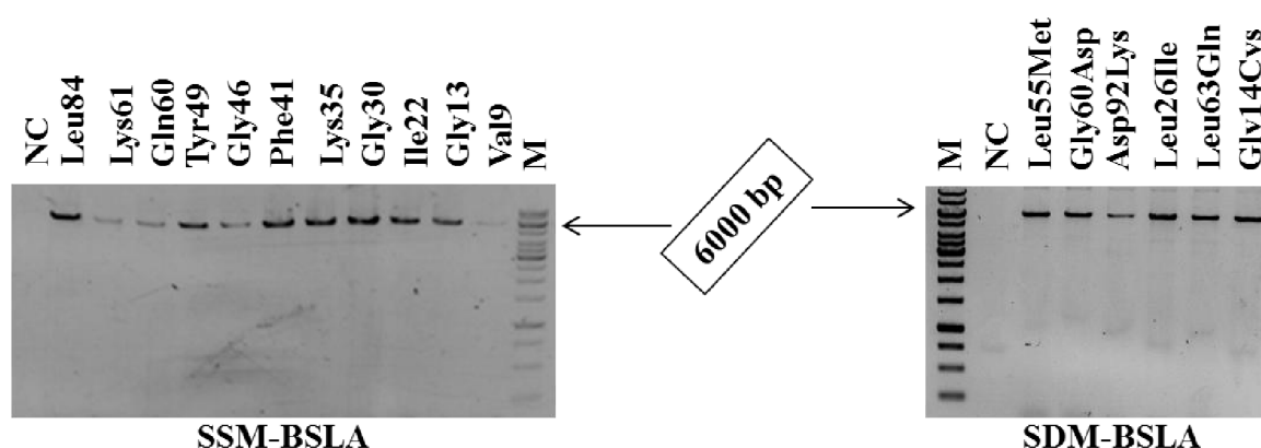
Figure 2-4: Exemplary agarose gel for SSM and SDM (QuikChange) at selected BSLA amino acid positions. 3 \mu L of each sample were mixed with 0.5 \mu L 6X loading dye and loaded. M (DNA marker, GeneRuler 1 kb DNA Ladder, Fermentas, St. Leon-Rot, Germany) is used for estimation of obtained DNA fragment sizes; NC= negative control. The expected size for each product was 6019 bp.
