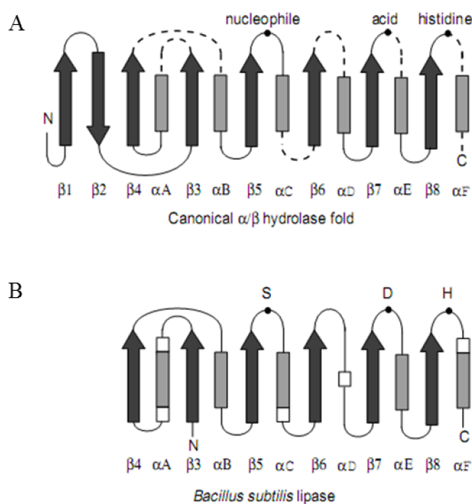
Figure 1-8: General folding model of the \alpha/\beta hydrolase. A: The canonic \alpha/\beta hydrolase fold; B: Bacillus subtilis lipase (BSL). The position of the catalytic triad is marked with bold points. This figure was taken from (van Pouderooyen et al. , 2001) with the permission of Elsevier provided by Copyright Clearance Center.
