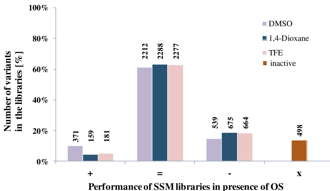
Figure 4-3: Number of SSM-BSLA variants leading to improved/unchanged/decreased OS resistance and inactivation of BSLA. All SSM-BSLA variants were grouped as described in the text: “+” representing variants with improved resistance, “=” representing variants with unchanged resistance, “-” representing variants with decreased resistance and “x” representing inactive variants in buffer.
