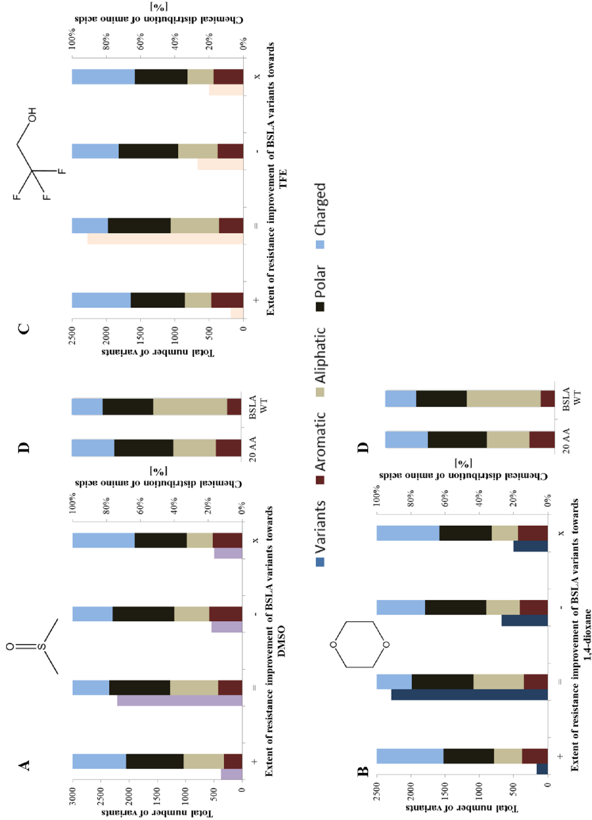
Figure 4-4: Distribution of amino acid substitutions of SSM-BSLA libraries with improved/unchanged/decreased OS resistance.
