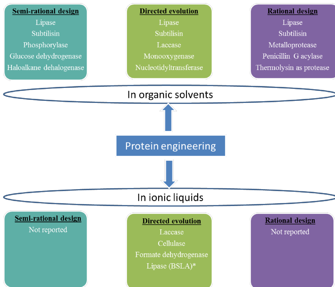
Figure 1-6: Examples of solvent-resistant enzymes achieved by protein engineering. This figure was partly adapted from (Stepankova et al. , 2013) with the permission of American Chemical Society provided by Copyright Clearance Center.*: First report in this work (chapter 3).
