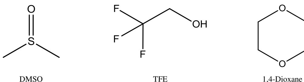
Figure 4-1: Chemical structure of the three selected OS: DMSO = dimethyl sulfoxide, TFE = 2,2,2-trifluoroethanol.
