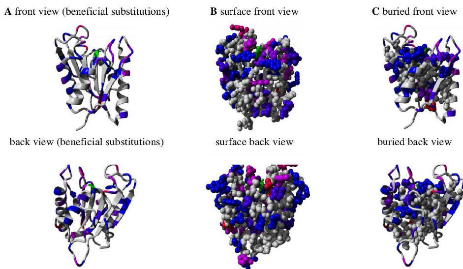
Figure 4-7: 3D model of BSLA (Protein Database code: 1I6W) displaying regions which favor BSLA resistance in presence of TFE in a color scale. Positions at which no substitution led to improvements are colored grey. Positions with one substitution leading to improvements are colored blue. Positions with two to seven substitutions leading to improvements are colored purple (two positions) to magenta (seven positions). Red represents positions with eight or more substitutions leading to improvements. The active site residue Ser 77 is colored green. A) Cartoon representation of BSLA, B) Van der Waals representation of surface residues of BSLA, C) Van der Waals representation of buried residues of BSLA. The two N-terminal amino acids (Ala1 and Glu2) are also included. Yasara was used for visualization.
