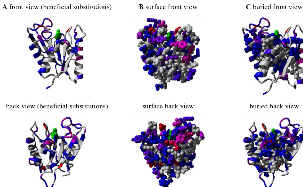
Figure 3-6: 3D model of BSLA (Protein Database code: 116W) displaying regions which favor BSLA resistance in presence of [BMIM][Br] in a color scale. Positions at which no substitution led to improvements are colored grey. Positions with one substitution leading to improvements are colored blue. Positions with two to seven substitutions leading to improvements are colored purple (two positions) to magenta (seven positions). Red represents positions with eight or more substitutions leading to improvements. The active site residue Ser 77 is colored green. A) Cartoon representation of BSLA, B) Van der Waals representation of surface residues of BSLA, C) Van der Waals representation of buried residues of BSLA. The two N-terminal amino acids (Ala1 and Glu2) are also included. Yasara was used for visualization.
