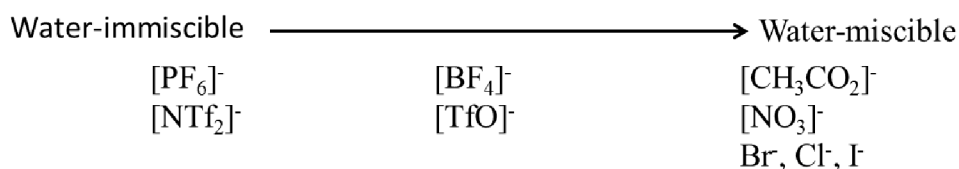
Figure 1-1: Examples of cations and anions used in ionic liquid systems. A: common used IL-cations, B: common used IL-anions. The anions are classified in increased order of water-miscibility. [PF 6 ] - : hexafluorophosphate, [NTf 2 ] - : bis(trifluoromethylsulfonyl) imide, [BF 4 ] - : tetrafluoroborate, [TfO] - : trifluoromethanesulfonate, [CH 3 CO 2 ] - : acetate, [NO 3 ] - : nitrate, Br - : bromide, Cl - : chloride, I - : iodide. This schema was partly adapted from (Plechova and Seddon, 2007) with the permission of Royal Society of Chemistry provided by Copyright Clearance Center.
