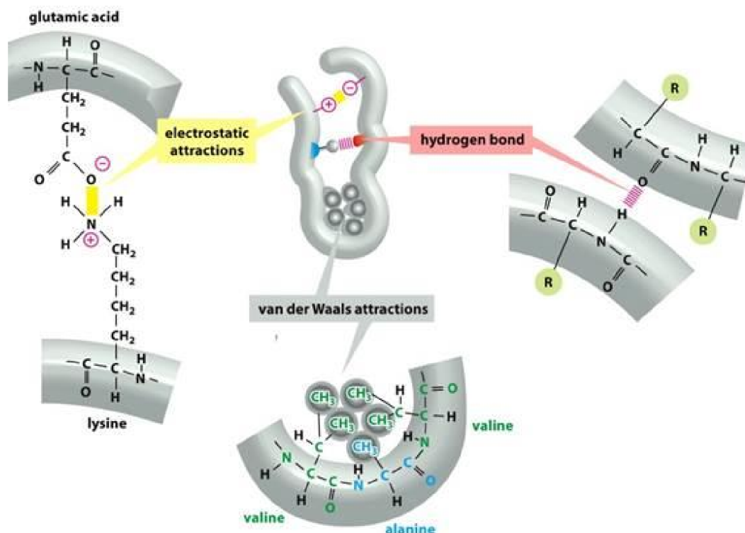
Figure 1-5: Various types of interactions stabilizing proteins. Some examples between residue chains are shown. R= amino acid side chain, yellow represents electrostatic interactions, red represents hydrogen bonds and grey represents van der Waals interactions. This figure was reproduced from Essential Cell Biology , 4 th Edition by Alberts et al. with the permission of Garland Science/Taylor & Francis LLC.
