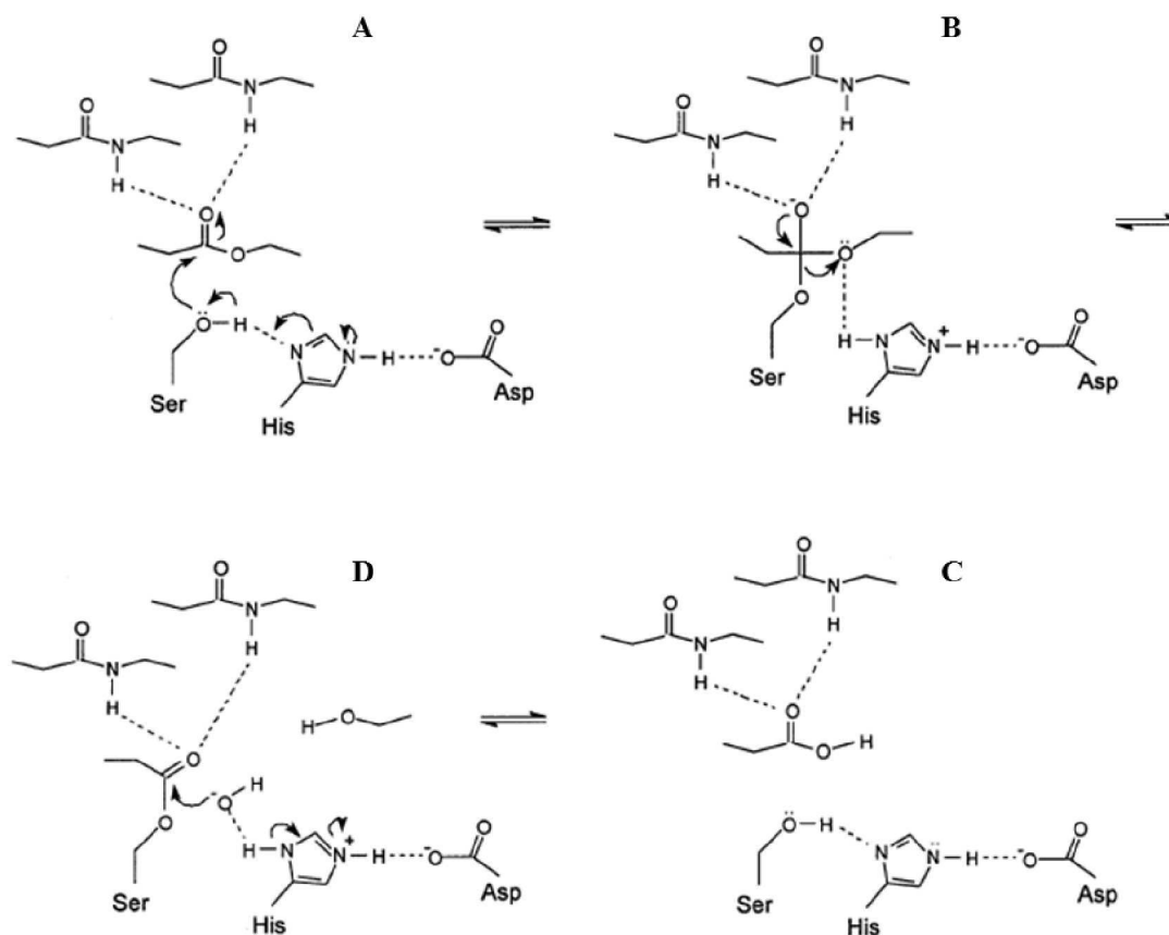
Figure 1-9: Catalytic mechanism of lipases. Ser, His and Asp represent the catalytic active amino acids. A: nucleophile attack, B: transient tetrahedral intermediate, C: covalent intermediate (acyl enzyme), D second transient tetrahedral intermediate. This figure was taken from (Jaeger et al. , 1999) under a free common licence.
