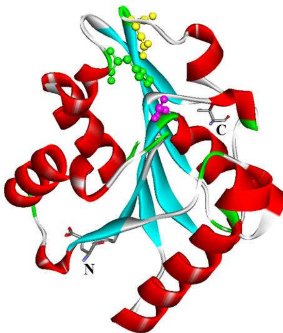
Figure 1-10: Crystal structure of Bacillus subtilis LipA (BSLA). PDB ID: 16WP, catalytic triad residues are highlighted: Ser77 (pink), His156 (green) and Asp133 (yellow). N: N-terminal and C: C-terminal. Yasara was used for visualization.
