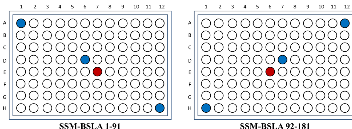
Figure 2-1: Scheme for MTP arrangement of generated SSM libraries. White colored wells contain SSM-BSLA variants, blue colored wells contain the WT (positive control, for SSM-BSLA 1-91: A1; D6 and H12; for SSM-BSLA 92-181: A12, D7 and H1) and red colored wells contain the EV (negative control, E7 for SSM-BSLA 1-91 and D6 for SSM-BSLA 92-181).
