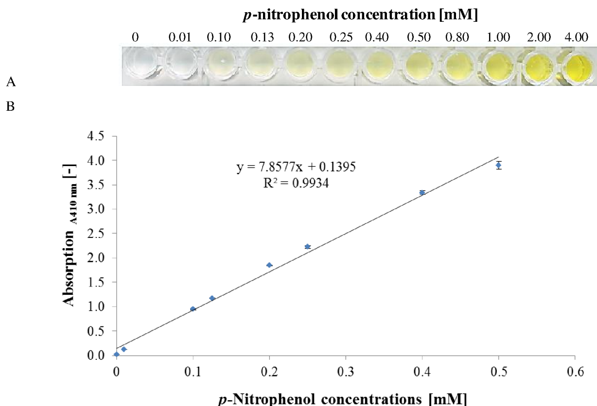
Figure 2-6: (A) Color development of p -nitrophenol relating to the concentration and (B) standard curve of p -nitrophenol. p -Nitrophenol was dissolved in Sørensen buffer (50 mM, pH 8.0) and different concentrations (0 to 4.0 mM) were obtained by dilution. Absorbance at A410 nm was measured in triplicate for each sample. Errors were calculated and are represented as bar.
