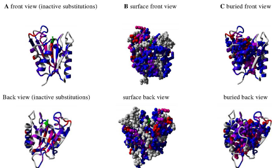
Figure 7-3: 3D model of BSLA (Protein Database code: 1I6W) displaying regions which inactivated BSLA. These numbers are identical in all OS and ILs since inactivation resulted from the mutations and did not depend on the non-conventional media used. Positions which did not harbor inactive substitutions are colored grey. Positions with one substitution leading to inactivation are colored blue. Positions with two to seven substitutions leading to inactivation are colored purple (two positions) to magenta (seven positions). Red represents positions with eight or more substitutions leading to inactivation. The active site residue Ser 77 is colored green. A) Cartoon representation of BSLA, B) Van der Waals representation of surface residues of BSLA, C) Van der Waals representation of buried residues of BSLA. The two N-terminal amino acids (Ala1 and Glu2) are also included. Yasara was used for visualization
