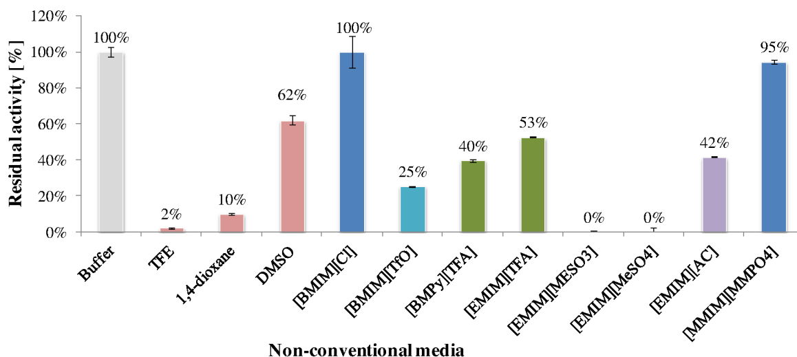
Figure 2-10: Selection of non-conventional media. EV and each BSLA sample were incubated with 50% v/v non-conventional media (2 h, RT, 1000 rpm) and the absorbance was recorded (410 nm, 8 min). The given co-solvent concentrations are related to the concentration in the 100 \mu L incubation mixture (10 \mu L supernatant + 90 \mu L co-solvent solution). A buffer MTP was also measured as control to enable residual activity calculation. Each sample was measured in triplicate and errors were calculated and are represented as bar. OS: DMSO (dimethyl sulfoxide), 1,4-dioxane, and TFE (2,2,2-Trifluoroethanol). ILs: [BMIM]: 1-butyl-3-methylimidazolium; [Cl]: chloride; [TfO]: trifluoromethanesulfonate, [BMPy]: 1-methylpyrrolidinium, [TFA]: trifluoroacetat, [EMIM]: 1-ethyl-3-methylimidazolium, [MeSO 3 ]: methanesulphate, [MeSO 4 ]: methylsulphate; [MMIM]: 1,3-Dimethylimidazolium Dimethyl, [MMPO 4 ]: dimethyl phosphate, [AC]: acetate.
