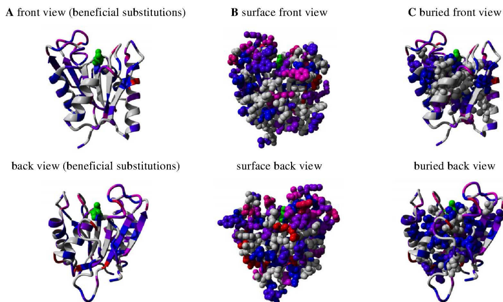
Figure 3-8: 3D model of BSLA (Protein Database code: 1I6W) displaying regions which favor BSLA resistance in presence of [BMIM][TfO] in a color scale. Positions at which no substitution led to improvements are colored grey. Positions with one substitution leading to improvements are colored blue. Positions with two to seven substitutions leading to improvements are colored purple (two positions) to magenta (seven positions). Red represents positions with eight or more substitutions leading to improvements. The active site residue Ser 77 is colored green. A) Cartoon representation of BSLA, B) Van der Waals representation of surface residues of BSLA, C) Van der Waals representation of buried residues of BSLA. The two N-terminal amino acids (Ala1 and Glu2) are also included. Yasara was used for visualization.
