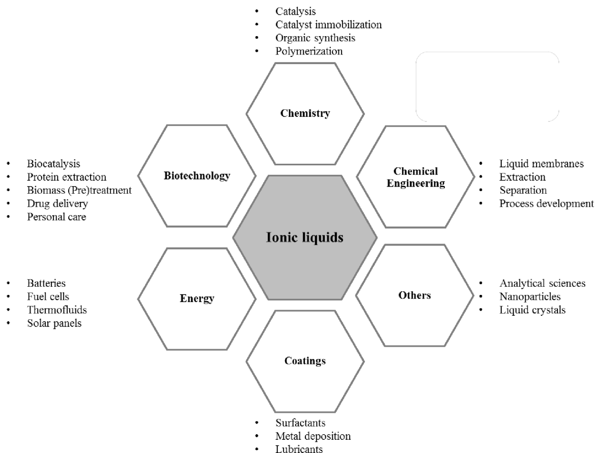
Figure 1-3: Overview of possible applications of ILs in different areas. This figure was adapted from (Domínguez de María, 2012; Patel et al. , 2014; Plechkova and Seddon, 2007).
