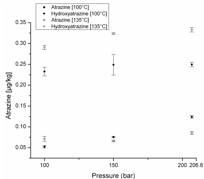
Figure 14: Extraction yields of Krauthausen soil B (KS-B) for different ASE temperature - pressure combinations. Error bars indicate standard deviations for triplicates.
