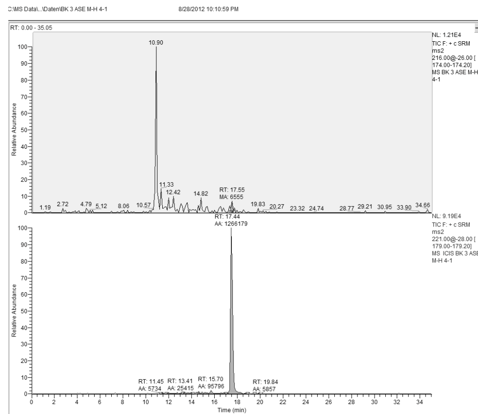
Figure 18: Top: Chromatogram of LC-MS/MS analysis of extracts of Krauthausen Soil B (KS-B) using 100°C and 206.8 bar as ASE Parameters and the old short gradient of 35 min, Atrazine is not detectable. Bottom: Chromatogram of the internal standard deuterated atrazine.
