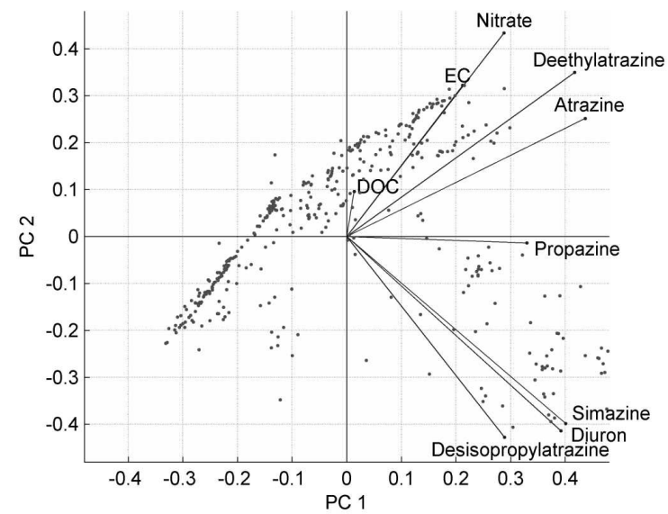
Figure 13: Loadings and scores plot of PCA.
