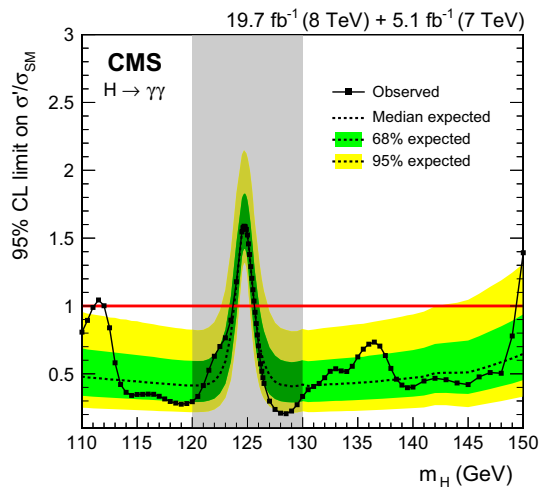
Fig. 27 Exclusion limit on the signal strength, \sigma'/\sigma_{\text{SM}} , for a second Higgs-boson-like state with SM couplings taking the observed state at 125 GeV as part of the background. The shading indicates a window with a width of 10 GeV, centred at the best-fit mass, where the expected sensitivity to a second Higgs boson is severely degraded due to the presence of the already observed state
