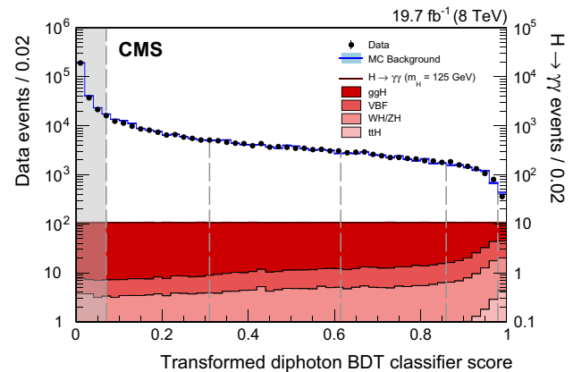
Fig. 6 Transformed diphoton BDT classifier score for events satisfying the full diphoton preselection in the 8 TeV data (points with error bars, left axis), and for simulated signal events from the four production processes (solid filled histograms, right axis). The outlined histogram, following the data points, is for simulated background events. The vertical dashed lines show the boundaries of the untagged event classes, with the leftmost dashed line representing the score below which events are discarded and not used in the final analysis (described in Sect. 6.3)
