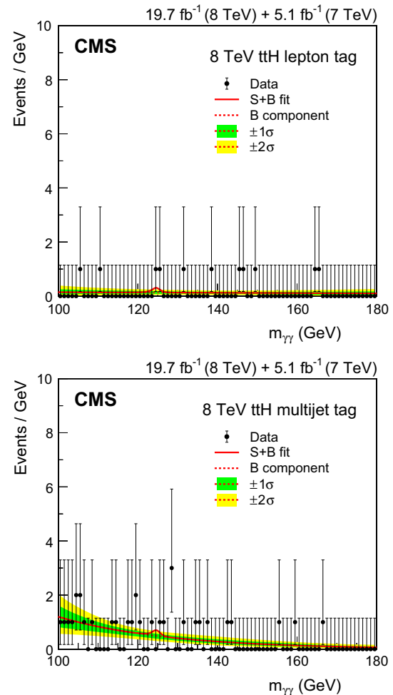
Fig. 16 Events in the two t\bar{t}H -tagged classes of the 8 TeV dataset, binned as a function of m_{\gamma\gamma} , together with the result of a fit of the signal-plus-background model. The 1\sigma and 2\sigma uncertainty bands shown for the background component of the fit are computed from the fit uncertainty in the background yield in bins corresponding to those used to display the data. These bands do not contain the Poisson uncertainty that must be included when the full uncertainty in the number of background events in any given mass range is estimated
