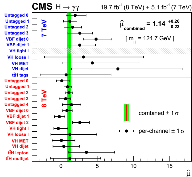
Fig. 21 Values of \hat{\mu} measured individually for all event classes in the 7 and 8 TeV datasets, fixing m_H = 124.7 GeV. The horizontal bars indicate \pm 1\sigma uncertainties in the values, and the vertical line and band indicate the best-fit signal strength in the combined fit to the data and its uncertainty
