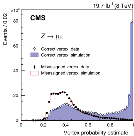
Fig. 5 Distribution of the vertex probability estimate in Z \rightarrow \mu^+\mu^- events. The vertex probability estimates in 8 TeV data (points), are compared to the estimates in MC simulation (histograms). The comparison is made separately for events in which the vertex is assigned to the same (open circles and filled histogram), or to a different vertex (filled circles and outlined histogram), as that identified by the muons
