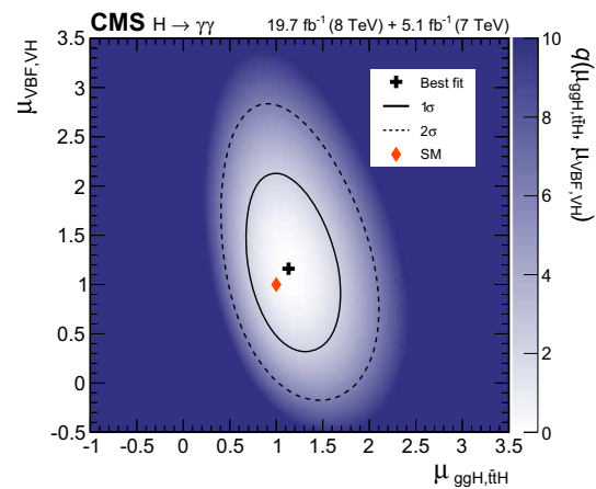
Fig. 23 Map of the likelihood ratio q(\mu_{ggH, \bar{t}tH}, \mu_{VBF, VH}) with m_H treated as an unconstrained parameter. The 1\sigma and 2\sigma uncertainty contours are shown. The cross indicates the best-fit values, (\hat{\mu}_{ggH, \bar{t}tH}, \hat{\mu}_{VBF, VH}) = (1.13, 1.16) , and the diamond represents the SM expectation
