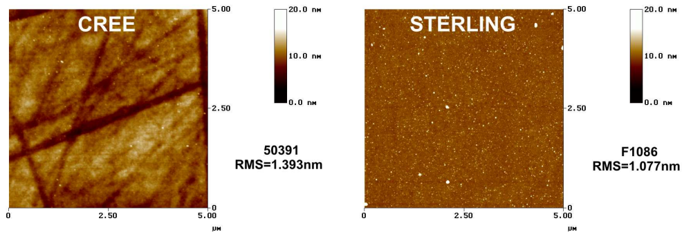
Figure 6.6: Surface morphology of Cree substrate (left) and Sterling substrate (right) on 5 \times 5 \mu\text{m}^2 scanning area measured by AFM. The substrate from Cree Research Inc. perform rough surface with many scratches, the substrates from Sterling Semiconductor Inc. are flatter.
