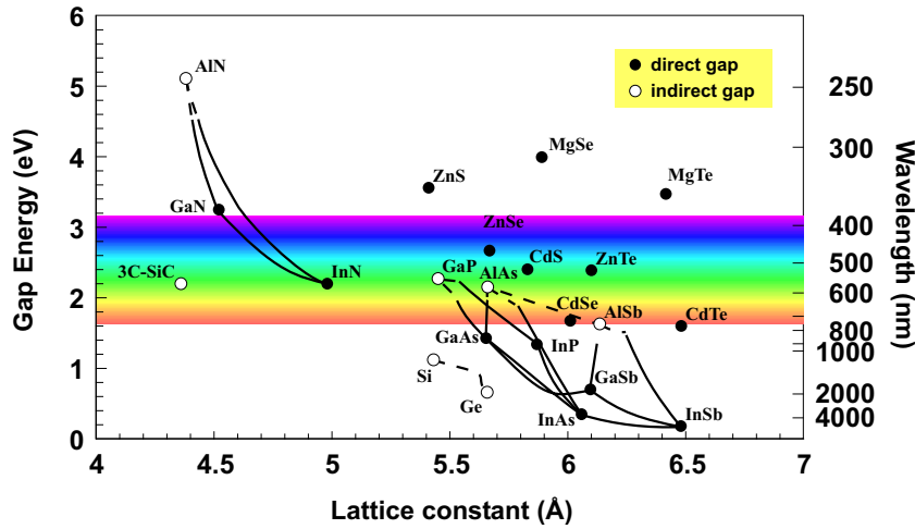
Figure 1.1: Bandgaps of the most important elementary and binary semiconductors versus their lattice parameter. For group III-nitrides the values of cubic polytypes are shown.
