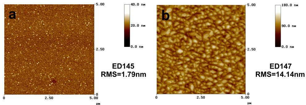
Figure 6.33: AFM images of III-N layers grown on Si(111) substrate:
