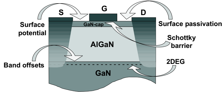
Figure 2.19: Properties forming the knowledge basis for understanding and improving the performance of AlGaN/GaN HEMTs.
