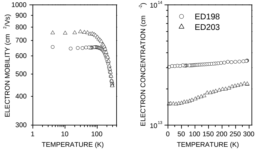
Figure 6.21: Temperature dependent Hall experiment data of AlGaIn/GaN MBE structures grown on 6H i-SiC.
