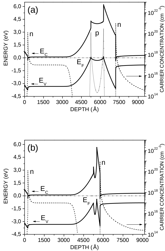
Figure 6.42: One dimensional band scheme calculation of the Al 0.25 Ga 0.75 N/GaN/Al 0.4 Ga 0.6 N/AlN/Si heterostructure with: (a) undoped Al 0.4 Ga 0.6 N(100 nm)/AlN(100 nm) buffer-nucleation layer, (b) Al 0.4 Ga 0.6 N(25 nm, N D = 1 × 10 19 cm -3 doped)/AlN(25 nm, undoped) buffer-nucleation layer.
