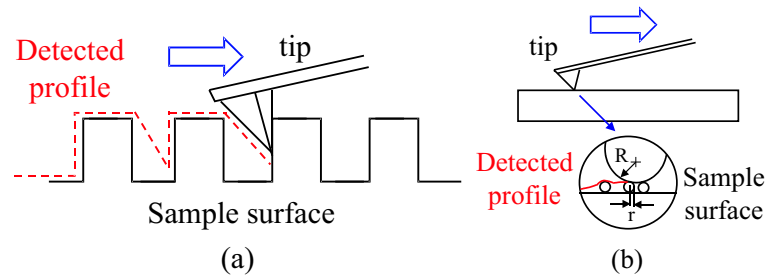
Figure 3.6: Errors deriving from surface geometry (a) and tip geometry (b) during AFM characterization.
