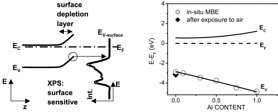
Figure 6.45: An depletion layer is formed under the n-type semiconductor surface due to the Fermi level pinning (left). Measured Fermi level pinning position of AlGaIn at the surface displayed as function of Al content (right). The gap energy was added to the measured points using the following approximation E_G(x) = (1 - x) \cdot E_G(\text{GaIn}) + x \cdot E_G(\text{AlIn})b \cdot x(1 - x) , where b = (0.98 \pm 0.1) \text{ eV} [192].
