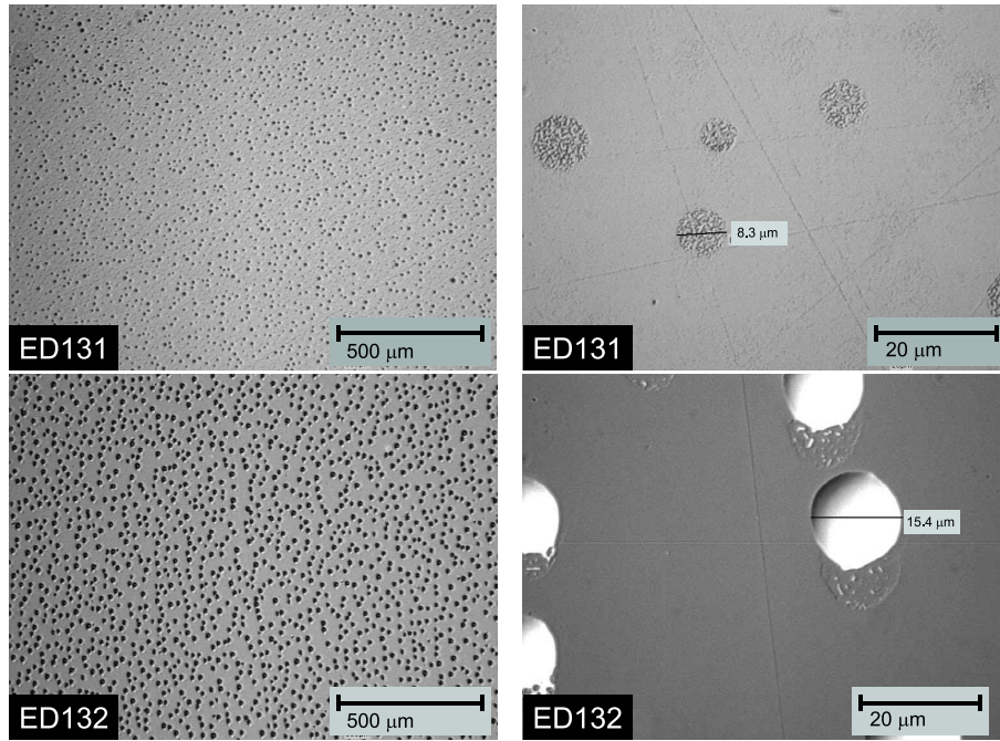
Figure 6.3: Optical microscope picture of ED131 and ED132 samples captured with two different magnifications. The circular “rougner” structures in ED131 are supposed to be the first stage for the formation of droplets. ED132 grown with a higher Ga flux shows formation of real droplets.
