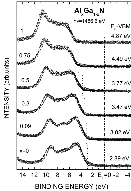
Figure 6.44: In-situ photoemission (XPS) valence band spectra of a series of \text{Al}_x\text{Ga}_{1-x}\text{N} layers ( \sim 1 \mu\text{m} of thickness, x from 0 to 1.0). The energy distance between the Fermi level ( \text{BE}=0 ) and the valence band maximum was determined by fitting the measured spectra in a small region close to the VBM (continuous line).
