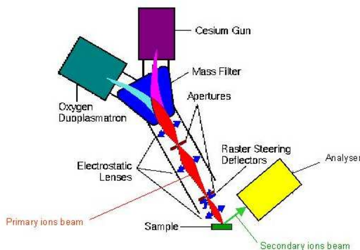
Figure 3.9: Schematic description of a SIMS equipment.
