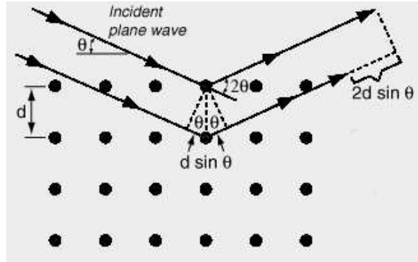
Figure 3.7: Diffraction of X-rays by a crystal.
