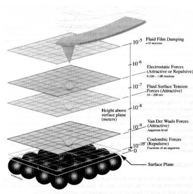
Figure 3.5: Representation of the interactions between the AFM scanning tip and the sample surface.
