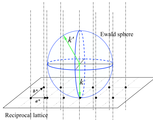
Figure 3.3: Ewald diagram describing the diffraction from a surface. The reciprocal lattice can be described by parallel rods intersecting the Ewald sphere.
