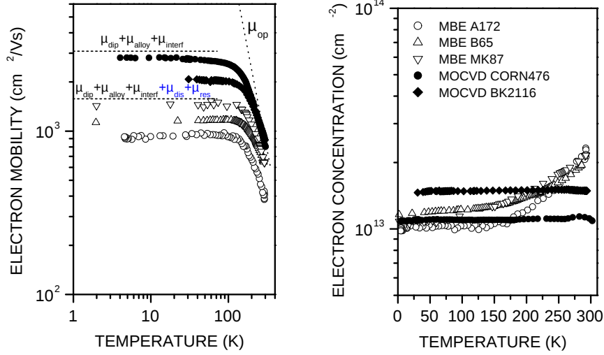
Figure 6.22: Temperature dependent Hall experiment data for AlGaIn/GaN heterostructures. The MBE structures are grown on 6H n-SiC(0001) and two MOCVD samples on sapphire. The dotted lines are qualitative model estimations representing electron-scattering mechanism.
