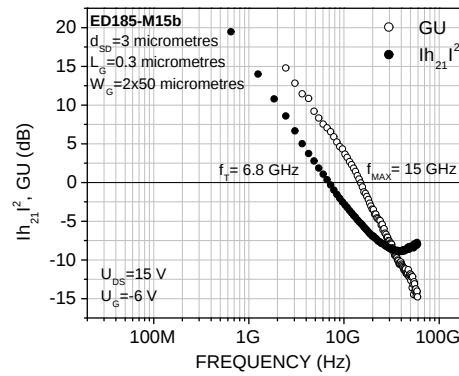
Figure 6.26: RF measurements of a 0.3 \times 50 \mu\text{m} AlGaIn/GaN HEMT.
