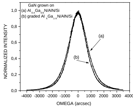
Figure 6.36: \omega -rocking curve of the (0002) reflection of a GaN layer grown on the AlGaIn/AlN buffer (ED156) (a) and on graded AlGaIn/AlN buffer (ED166) (b).
