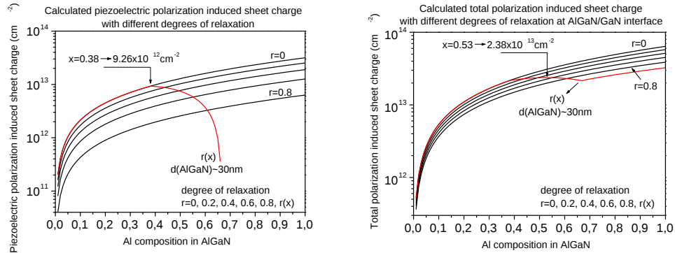
Figure 2.7: Calculated piezoelectric (left) and total (right) polarization induced sheet charge versus Al composition in AlGa N barrier at AlGa N /Ga N interface displayed as a function of degree of relaxation.
