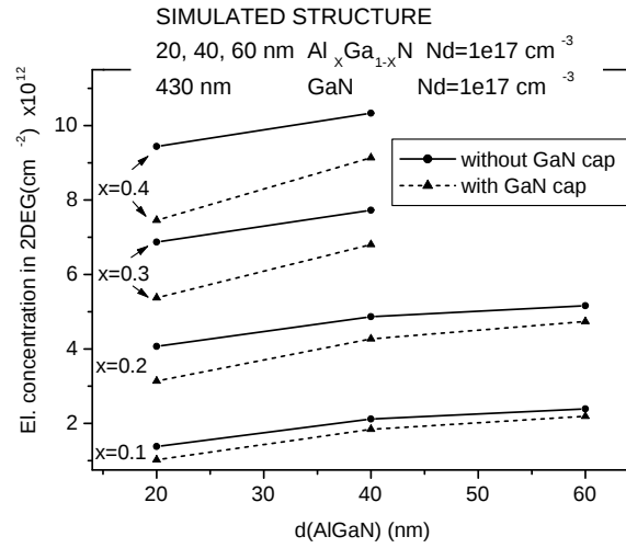
Figure 5.8: n_{2\text{DEG}} comparison between \text{Al}_x\text{Ga}_{1-x}\text{N}/\text{GaN} heterostructure with and without GaN cap for various Al composition ( x=0.1, 0.2, 0.3, 0.4 ) and barrier thickness ( d = 20, 40, 60 \text{ nm} ) calculated using band scheme simulation.
