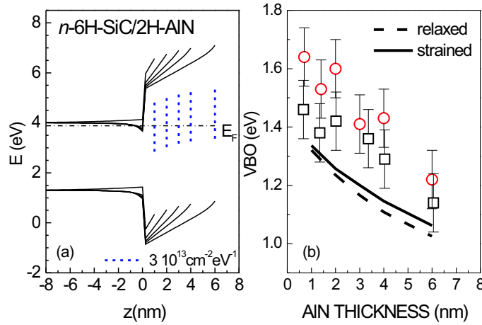
Figure 2.21: (a) Tight Binding self consistent calculation of a relaxed AlN/SiC heterostructure as a function of the overlayer thickness taking into account a constant density of surface states \text{SDOS} = 3 \times 10^{13} \text{ cm}^{-2} \text{ eV}^{-1} (sketched with a vertical dashed line). (b) VBO as a function of the AlN overlayer thickness: experimental XPS data determined from different runs (symbols) compared with the model (see text) for a pseudomorphic and relaxed overlayer (continuous and dashed line, respectively).
