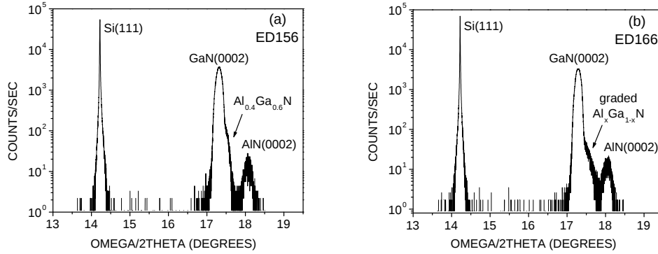
Figure 6.37: \omega - 2\theta scan of a GaN layer grown on the AlGaN/AlN buffer (sample ED156) (a) and on graded AlGaN/AlN buffer (sample ED166) (b). Three peaks can be seen: Si substrate peak, GaN (0002) reflection and AlN (0002) reflection. The right shoulder of the GaN peak corresponds to \text{Al}_{0.4}\text{Ga}_{0.6}\text{N} (a) and to graded \text{Al}_x\text{Ga}_{1-x}\text{N} (b) interlayer.
