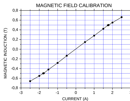
Figure 4.8: Magnetic field calibration of the Varian Magnet.
