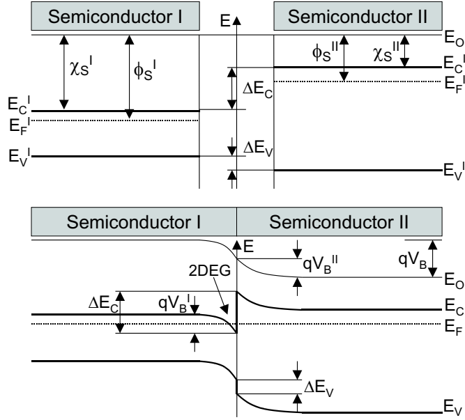
Figure 2.8: Band scheme of a lightly n-doped narrow-gap semiconductor (I) and a moderately/heavily n-doped wide-gap semiconductor (II) before (top) and after contact (bottom). In thermal equilibrium (bottom), the electrons are confined in the triangular quantum well of the narrow-gap semiconductor (I) and form a two dimensional electron gas (2DEG). E_C is the conduction band minimum, E_V the valence band maximum, E_F the Fermi level, \phi_S the semiconductor work function, \chi_S the electron affinity and V_B the built-in voltage.
