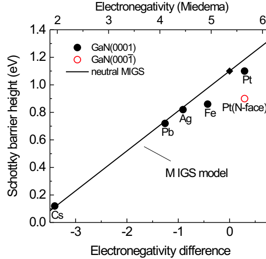
Figure 2.22: Barrier heights of laterally homogeneous GaN Schottky contacts as a function of the metal and the GaN electronegativity difference. The MIGS line is drawn after \phi_{Bn} = \phi_{bp} + S_X(X_m - X_s) with \phi_{bp} = 1.1 eV and S_X = 0.29 eV/Miedema-unit, derived from a charge neutrality condition, which does not take into account the polarization charge close to the GaN surface (after Ref. [127]).
