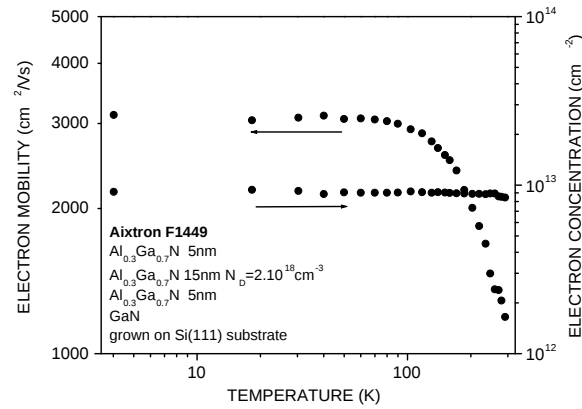
Figure 6.43: Temperature dependent Hall experiment data of \text{Al}_{0.3}\text{Ga}_{0.7}\text{N}/\text{GaN} MOCVD structure grown on Si(111) (sample F1149).
