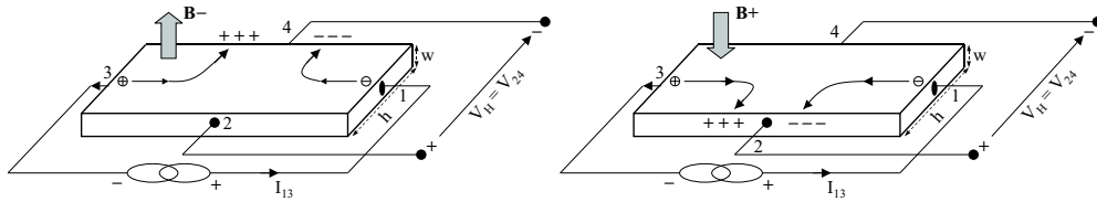
Figure 3.17: Van der Pauw arrangement for measuring the Hall factor of an arbitrary shaped sample. If R_{B+} - R_{B-} > 0 then the semiconductor is P-type and if R_{B+} - R_{B-} < 0 then the semiconductor is N-type, assuming single type conductivity semiconductor.
