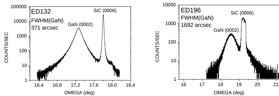
Figure 6.12: XRD rocking curve ( \omega -scan with wide open detector) of the ED132 and ED196. The peak of SiC is very wide (FWHM= 810 arcsec) for the Sterling substrate (ED196), while is reasonably narrow (FWHM= 54 arcsec) for the Cree substrate (ED132).
