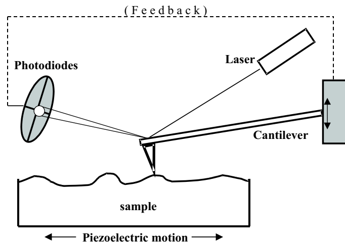
Figure 3.4: Schematic description of the AFM operation principle.
