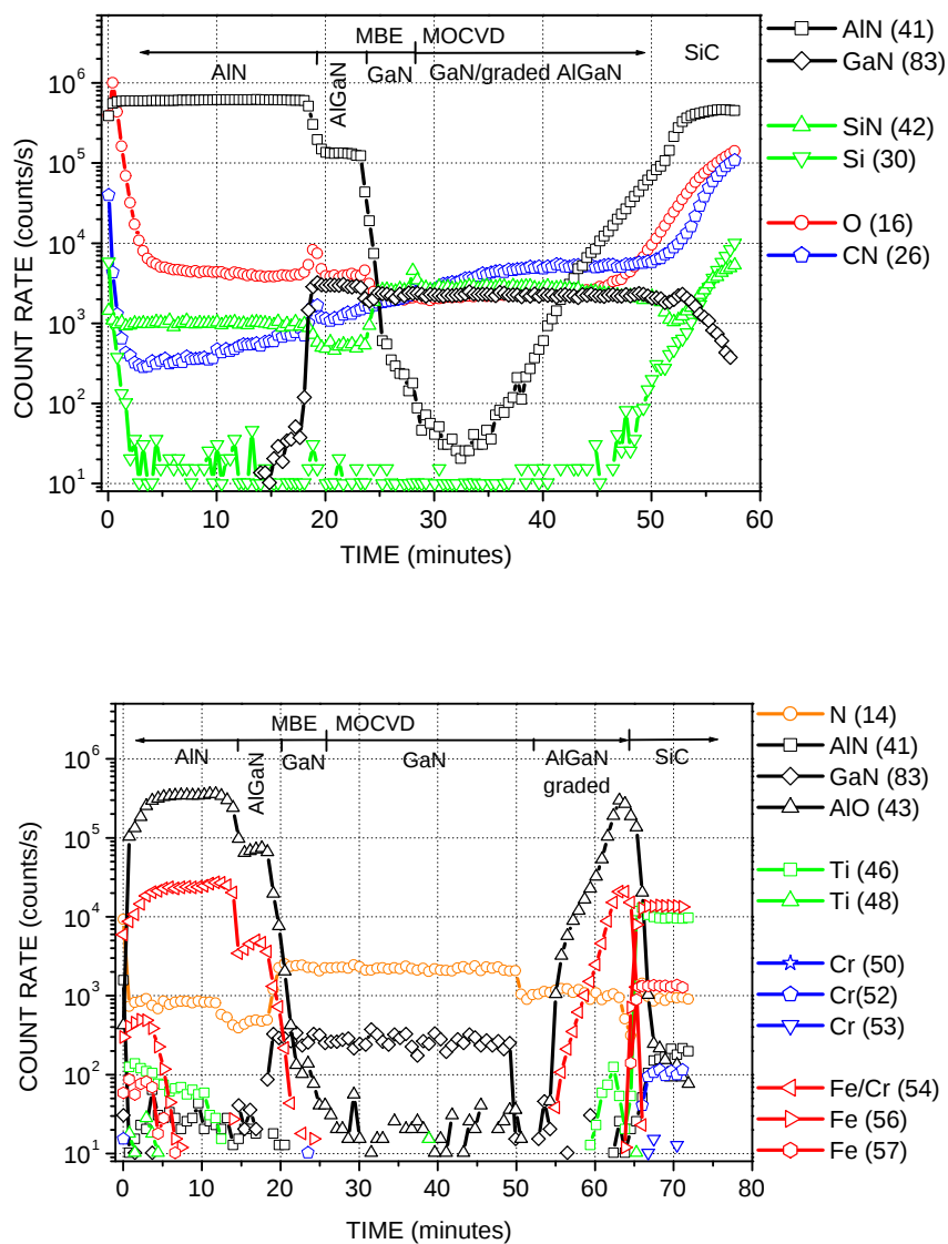
Figure 6.15: SIMS analysis of the sample ED168. The numbers reported in brackets in the legend are relative atomic masses. (top graph: \text{Cs}^+ ions, energy: 6 kV, current: 57 nA, normal incidence; bottom graph: \text{O}_2^+ ions, energy: 6 kV, current: 248 nA, normal incidence)
