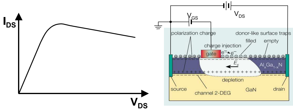
Figure 2.23: Negative biased gate leads to trapping of electrons in the surface states and formation of the virtual gate in the region between gate and drain (right). Consequently the drain-source current is reduced (left), the current collapse effect occurs.
