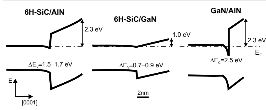
Figure 2.20: Schematic plots of the band scheme at the studied heterojunctions: the band offsets and the surface Fermi level pinning positions are those derived from the XPS experiments.
