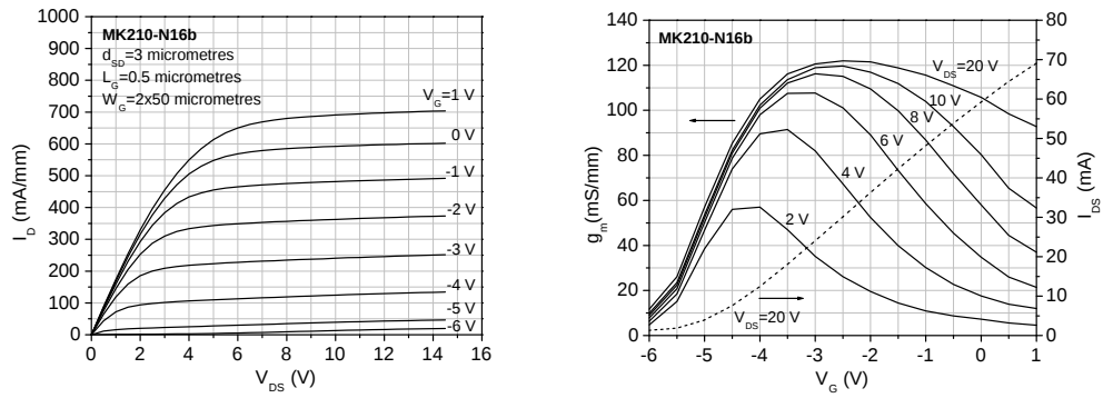
Figure 6.28: Output (left) and transfer (right) characteristics of a 0.5 \times 50 \mu\text{m} AlGaIn/GaN HEMT.
