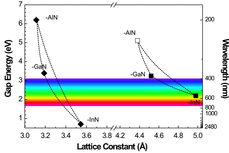
Figure 2.1: Energy gaps and lattice constants for III-N semiconductors with wurzite ( \alpha -phase) and zincblende ( \beta -phase) structures.
