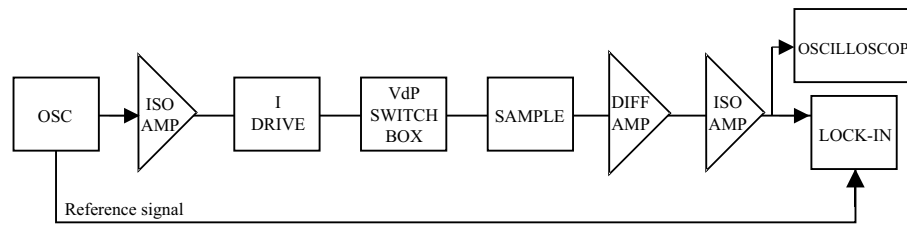
Figure 4.9: Hall measurement circuit scheme.
