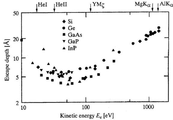
Figure 3.11: Dependence of the photoelectron escape depth on the kinetic energy [143]. The energies of different typical radiation sources are also given.
