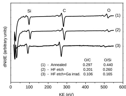
Figure 6.7: Comparison between Auger spectra of SiC substrates cleaned in different ways (see text). The ratio between the peaks of silicon and oxygen and between carbon and oxygen is also shown.
