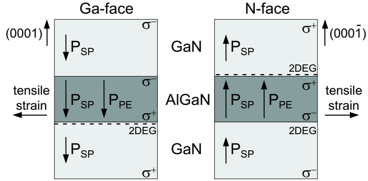
Figure 2.10: Spontaneous, piezoelectric polarization bound interface charges and 2DEGs in pseudomorphic GaN/Al x Ga 1-x N/GaN heterostructures with Ga-face (left) and N-face (right).
