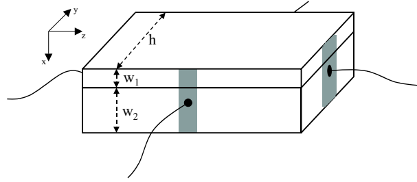
Figure 3.18: Non-uniform sample in the form of two parallel slabs with different thickness, carrier density and mobility. Current flow is everywhere parallel to z direction and is uniform within the individual slabs.
