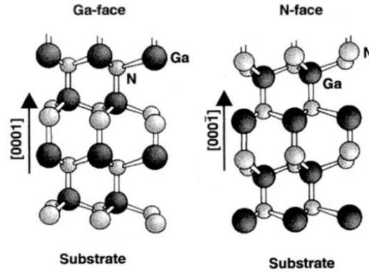
Figure 2.3: Structure of the N-face and Ga-face GaN.
