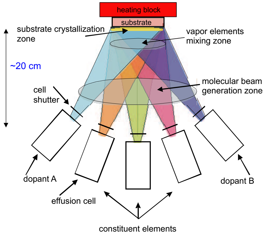
Figure 2.17: Schematic description of a MBE chamber.
