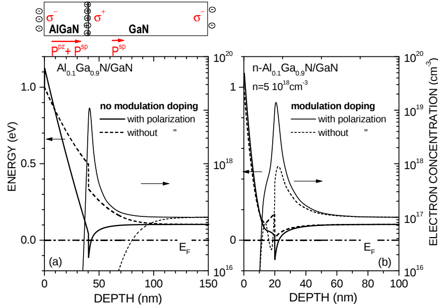
Figure 5.3: Self-consistent Schrödinger-Poisson calculation for an \text{Al}_{0.1}\text{Ga}_{0.9}\text{N}/\text{GaN} pseudomorphic heterostructure with and without modulation doping. The conduction band edge profile is shown (left scale) together with the electron concentration (right scale) along the undoped (left) and doped n = 5 \times 10^{18} \text{ cm}^{-3} (right) AlGaN/GaN heterostructure.
