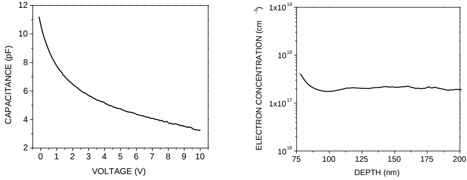
Figure 6.18: Measured capacitance-voltage characteristic of GaN grown on 6H i-SiC substrate (sample ED174) (left) and calculated carrier concentration profile (right). In the first about 80 nm the electron concentration is higher due to the Si-doping of the top of the structure, while in the bulk it is in the order of 2 \times 10^{17}\ \text{cm}^{-3} .
