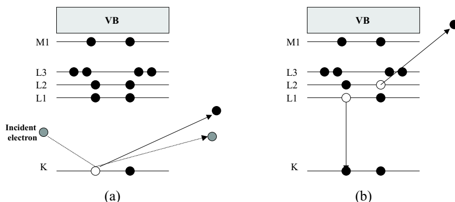
Figure 3.1: Explanation of the Auger process on the basis of atomic level schemes. A primary electron produces an initial hole in a core level (a). Another electron is deexcited from a higher shell and the deexcitation energy is then transferred to a third electron, which leaves the system as an Auger electron (b).
