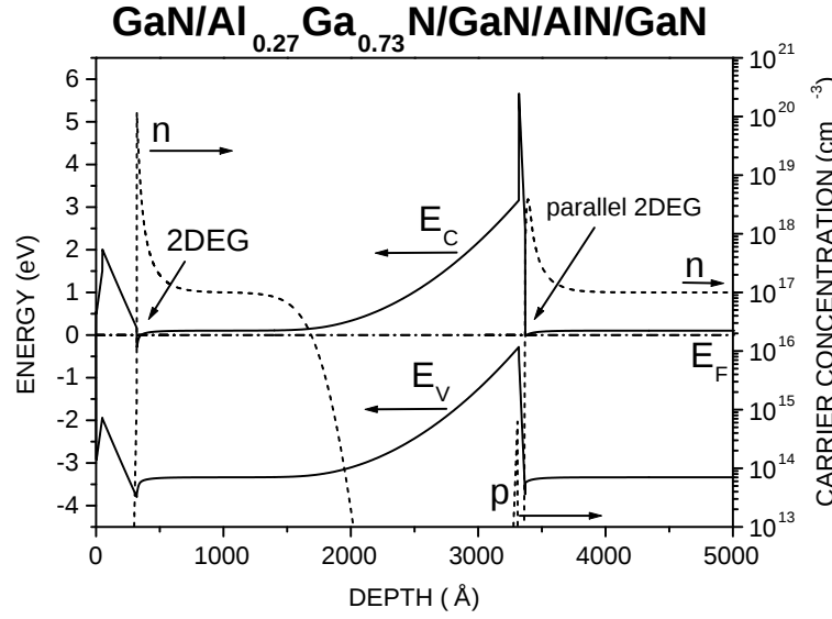
Figure 6.20: Simulation of the band scheme and carriers concentration of (GaN/Al 0.27 Ga 0.73 N/GaN/AlN/GaN) obtained from the Schrödinger-Poisson equation solver [158].
