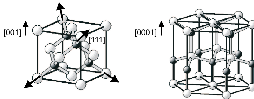
Figure 2.4: Cubic zincblende and hexagonal wurtzite-type of structure. Sum of the microscopic dipoles result in zero spontaneous polarization (zincblende) and in non-zero spontaneous polarization (wurtzite structure).
