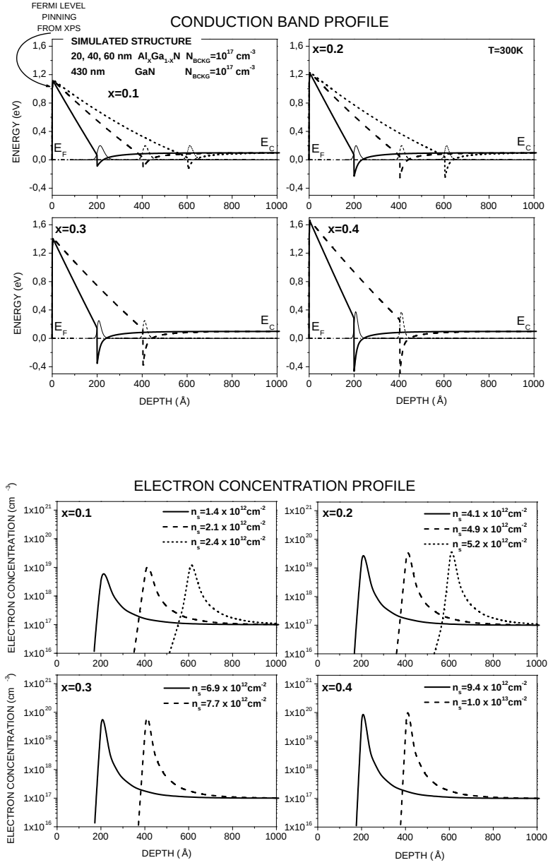
Figure 5.6: Band scheme simulation of an Al x Ga 1-x N/GaN heterostructure with various Al concentrations ( x=0.1, 0.2, 0.3, 0.4 ) and barrier thickness ( d = 20, 40, 60 \text{ nm} ). The conduction band minimum E_C with the probability function |\psi_1|^2 of the first discrete energy state in the triangular quantum well (top) and electron concentration profile (bottom) are displayed. The concentration in 2DEG is shown in the legend for all calculations.
