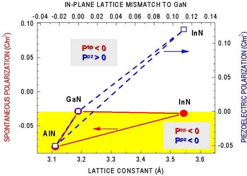
Figure 2.5: Spontaneous ( filled circles ) and piezoelectric ( open squares ) polarizations for the binary III-N compounds. The piezoelectric polarization is calculated for a pseudomorphic epitaxial layer on a GaN substrate, with the assumption of biaxial strain in the basal plane. The spontaneous polarization values are taken from [11].
