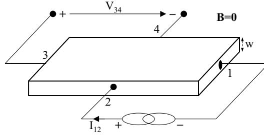
Figure 3.16: Van der Pauw arrangement for measuring the conductivity of an arbitrary shaped sample.
