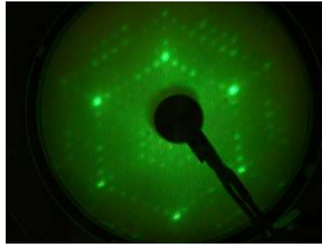
Figure 6.31: LEED image of a clean Si(111) surface. 7 \times 7 reconstruction was observed.
