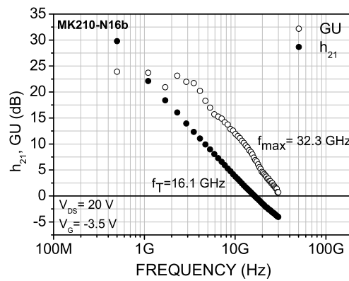
Figure 6.29: RF measurements of a 0.5 \times 50 \mu\text{m} AlGaIn/GaN HEMT.
