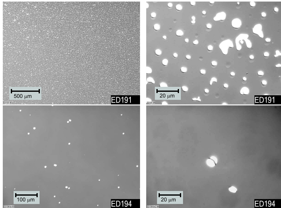
Figure 6.9: Optical microscope pictures of AlN nucleation layers grown on i-SiC substrate, ED191 and ED194, obtained with two different magnifications. Many Al droplets can be recognized on ED191, while few of them are present on ED194.
