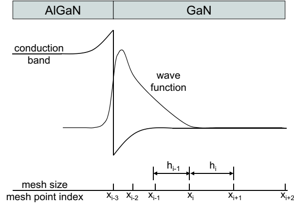
Figure 5.2: Band diagram of a single heterojunction AlGaIn/GaN and its bounded state wave function (top) and discretization of the potential using a nonuniform mesh (bottom).
