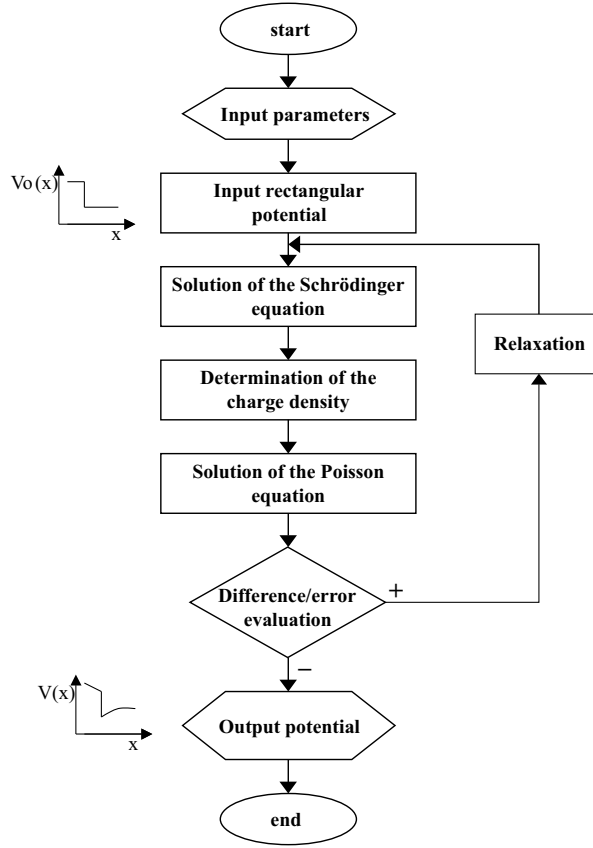
Figure 5.1: Self-consistent algorithm of solving Schrödinger and Poisson equation.
