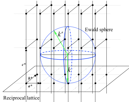
Figure 3.2: Ewald diagram describing the diffraction from a three dimensional crystal lattice. The Laue condition is fulfilled when the surface of the sphere touches a point of the reciprocal lattice.
