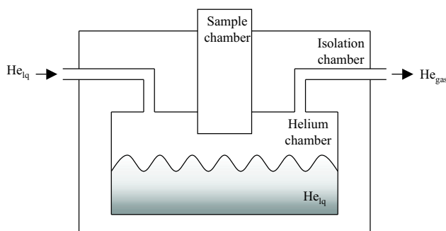
Figure 4.6: ^4\text{He} -overflow cryostat consists of three chambers.
