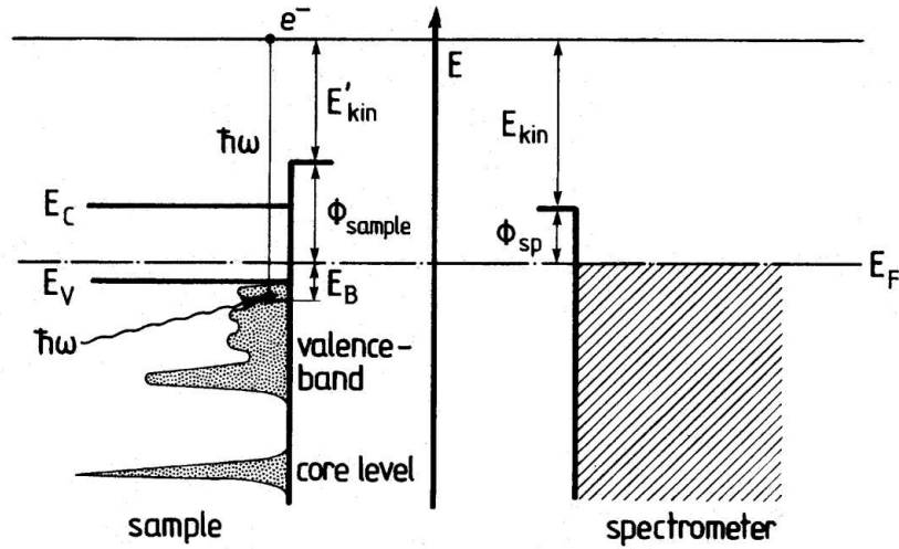
Figure 3.10: Schematic representation of the processes occurring in photoemission spectroscopy
