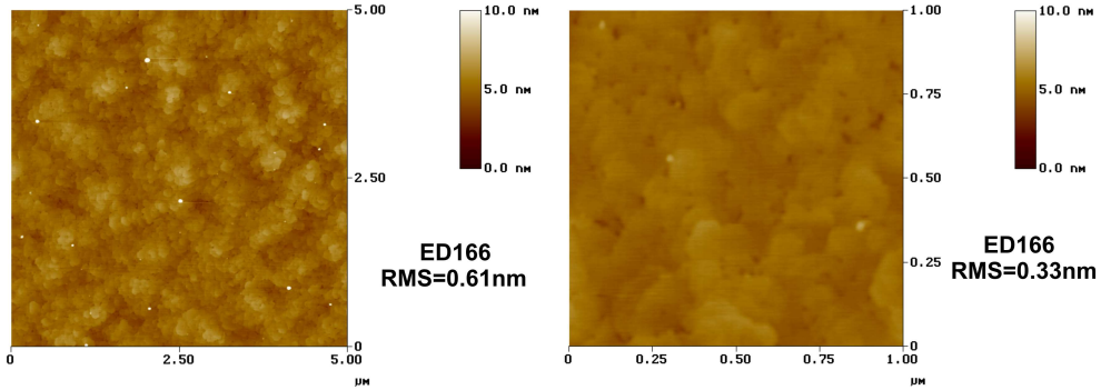
Figure 6.35: AFM image of the GaN(1 \mu\text{m} ) layer grown on graded AlGaIn(100 nm)/AlN(100 nm) buffer, rms=0.61 nm (sample ED166). 5 \times 5 \mu\text{m}^2 and 1 \times 1 \mu\text{m}^2 scan area is displayed on the left and right side, respectively.
