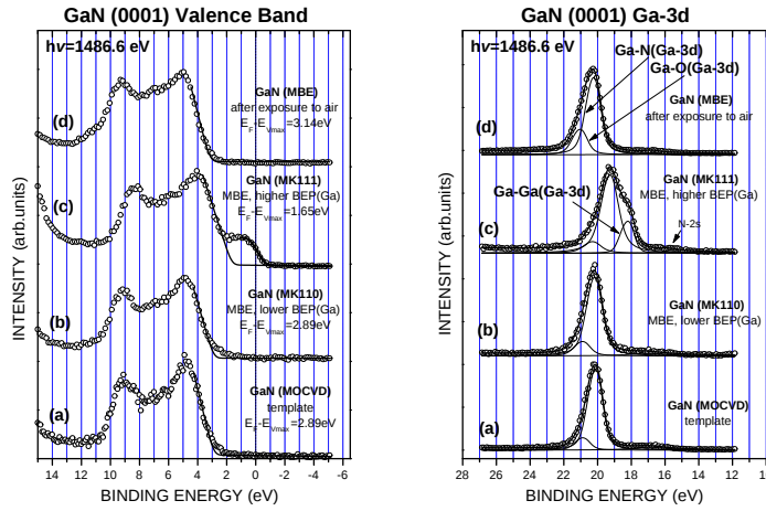
Figure 6.48: XPS spectra in the energy region of the valence band (left side) and of the Ga-3d core level (right side) measured at different GaN surfaces. (a) MOCVD template after UHV annealing at 770 °C, 10 min; MBE as grown surfaces (b) MK110: \text{BEP}(\text{Ga}) = 2.0 \times 10^{-7} mbar and (c) MK111: \text{BEP}(\text{Ga}) = 2.5 \times 10^{-7} mbar; (d) after exposure to air and reinsertion in UHV (see text). The solid lines represent the best fit close to the VBM region (left side), which provides the indicated VBM energy and the best fit of the Ga-3d core level (right side) decomposed in its single components.
