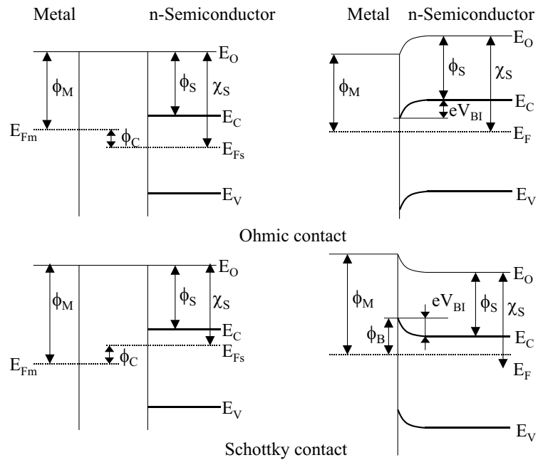
Figure 3.13: Energy band diagram of ohmic (top) and Schottky contact (bottom). Thermal equilibrium of the metal and semiconductor (left) and of the metal-semiconductor junction brought into contact (right). ( \phi_C is the contact potential energy.)
