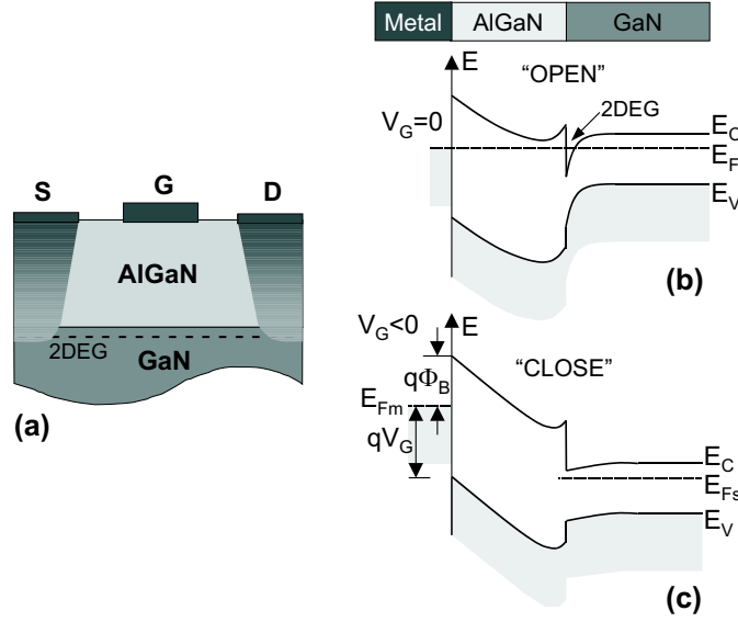
Figure 2.12: Schematic structure (a) and electronic band scheme perpendicular to the wafer surface underneath the gate electrode of an AlGaN/GaN HEMT device (b,c). The conductive channel is formed by 2DEG. The band schemes are under zero gate voltage, in thermal equilibrium, (b) and under negative gate bias (c). E_C is the conduction band minimum, E_V the valence band maximum, E_{Fm} the Fermi level in metal, E_{Fs} the Fermi level in the semiconductor, q\Phi_B the Schottky barrier height and V_G the gate voltage.
