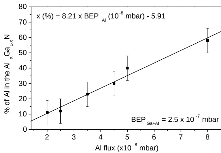
Figure 6.5: Al concentration in \text{Al}_x\text{Ga}_{1-x}\text{N} grown with different Al fluxes measured by RBS. The linear fit was thereafter used to grow layers with the desired composition.
