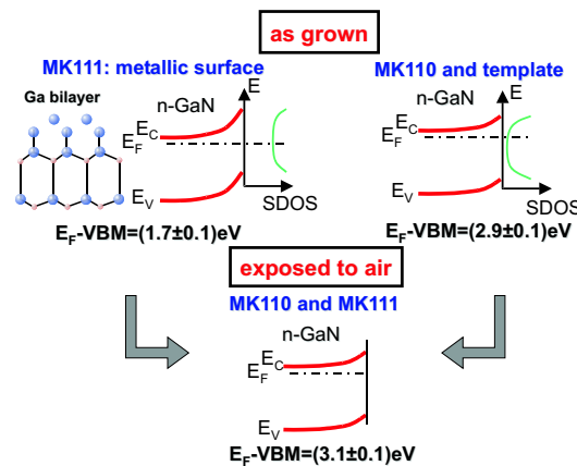
Figure 6.49: Band bending under the surface of as grown and air-exposed GaN MBE layers grown under different conditions. The values of the Fermi level pinning measured by XPS are displayed. The surface of the Ga-rich grown sample, MK111, have a Ga-adatom bilayer on the surface according to the theoretical investigations of Zywiets et al. [194].
