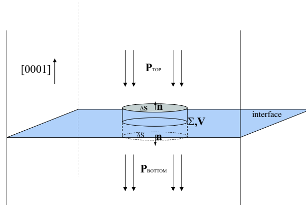
Figure 2.6: The close surface \Sigma enclosing the volume V can be used to calculate \sigma (charge density at the interface) through the theorem of divergency.
