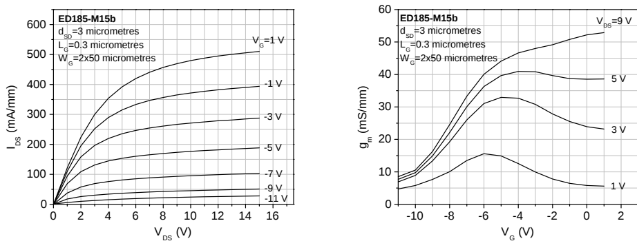
Figure 6.25: Output (left) and transfer (right) characteristics of a 0.3 \times 50\ \mu\text{m} AlGaN/GaN HEMT.
