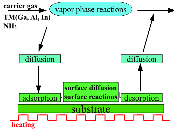
Figure 2.18: The principle of a MOCVD.
