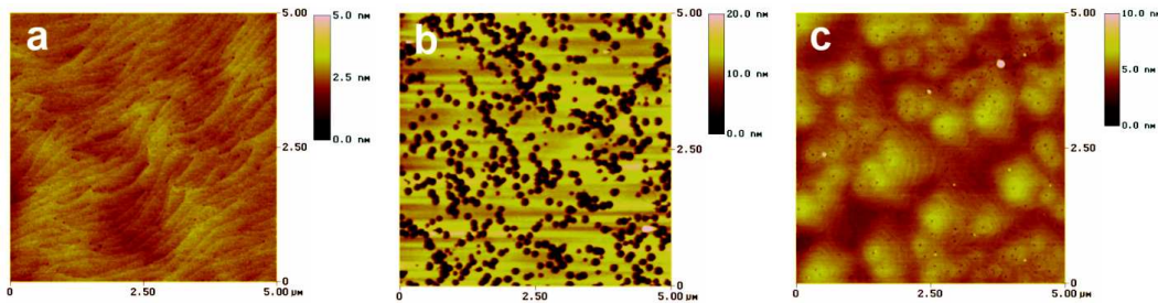
Figure 6.46: AFM images showing the surface morphology of GaN films grown by MBE on the MOCVD template (a) using a Ga flux of: \text{BEP}(\text{Ga}) = 2.0 \times 10^{-7} \text{ mbar} (sample MK110) (b) and \text{BEP}(\text{Ga}) = 2.5 \times 10^{-7} \text{ mbar} (sample MK111) (c).
