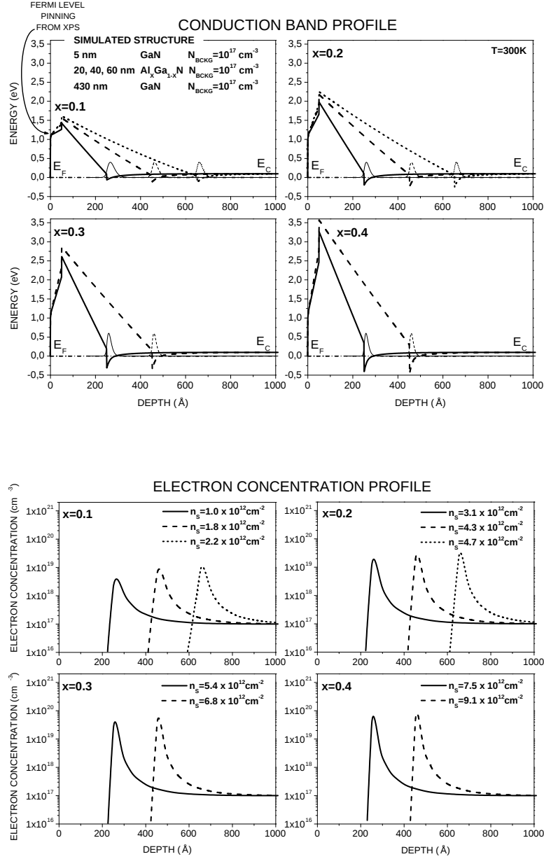
Figure 5.7: Band scheme simulation of a GaNcap/ \text{Al}_x\text{Ga}_{1-x}\text{N} /GaN heterostructure with various Al concentrations ( x = 0.1, 0.2, 0.3, 0.4 ) and barrier thickness ( d = 20, 40, 60 \text{ nm} ). The conduction band minimum E_C with the probability function |\psi_1|^2 of the first discrete energy state in the triangular quantum well (top) and electron concentration profile (bottom) are displayed. For all calculations the concentration in 2DEG is shown in the legend.
