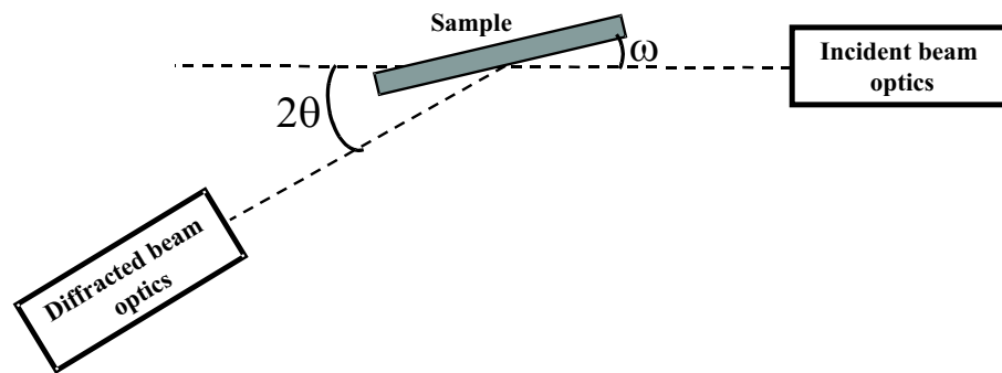
Figure 3.8: Schematic setup of a XRD measurement system.
