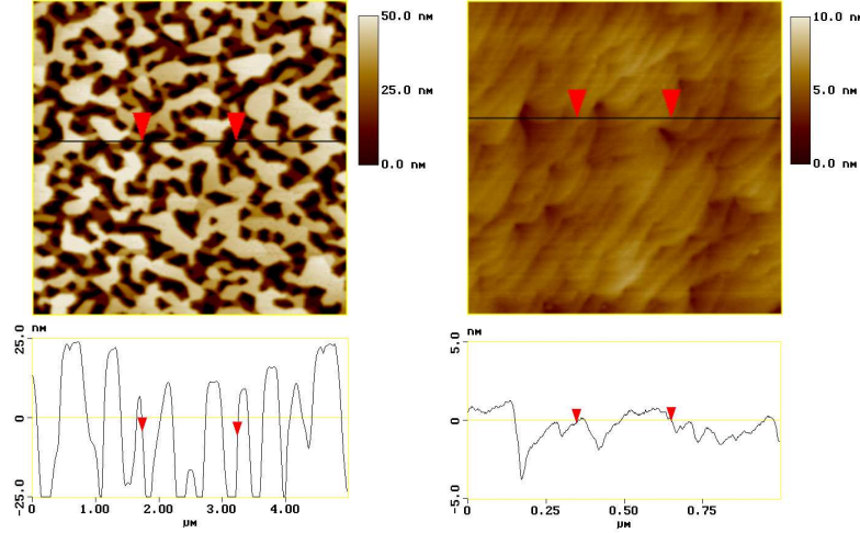
Figure 6.11: AFM picture and cross section of GaN layers grown on i-SiC substrate, ED195 ( 5 \times 5 \mu\text{m}^2 , RMS=20 nm) and ED196 ( 1 \times 1 \mu\text{m}^2 , RMS=0.8 nm).
