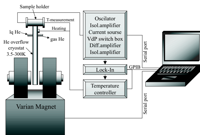
Figure 4.5: Low temperature Hall measurement setup.
