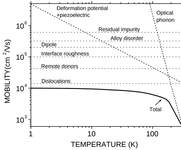
Figure 2.11: Theoretical temperature dependence of electron mobility in a \text{Al}_{0.15}\text{Ga}_{0.85}\text{N}/\text{GaN} modulation doped heterostructure. All curves are calculated mobilities (see text). The 2DEG density for this case is 1.6 \times 10^{12} \text{ cm}^{-2} , the concentration of residual ionized impurities in the GaN is 4 \times 10^{15} \text{ cm}^{-3} , the remote donor concentration in AlGaIn barrier 10^{18} \text{ cm}^{-3} and the dislocation density 10^9 \text{ cm}^{-2} .
