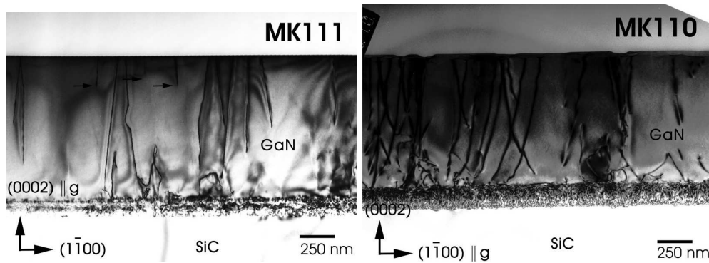
Figure 6.47: Cross-sectional bright-field TEM image of sample MK111 (left) and of sample MK110 (right).
