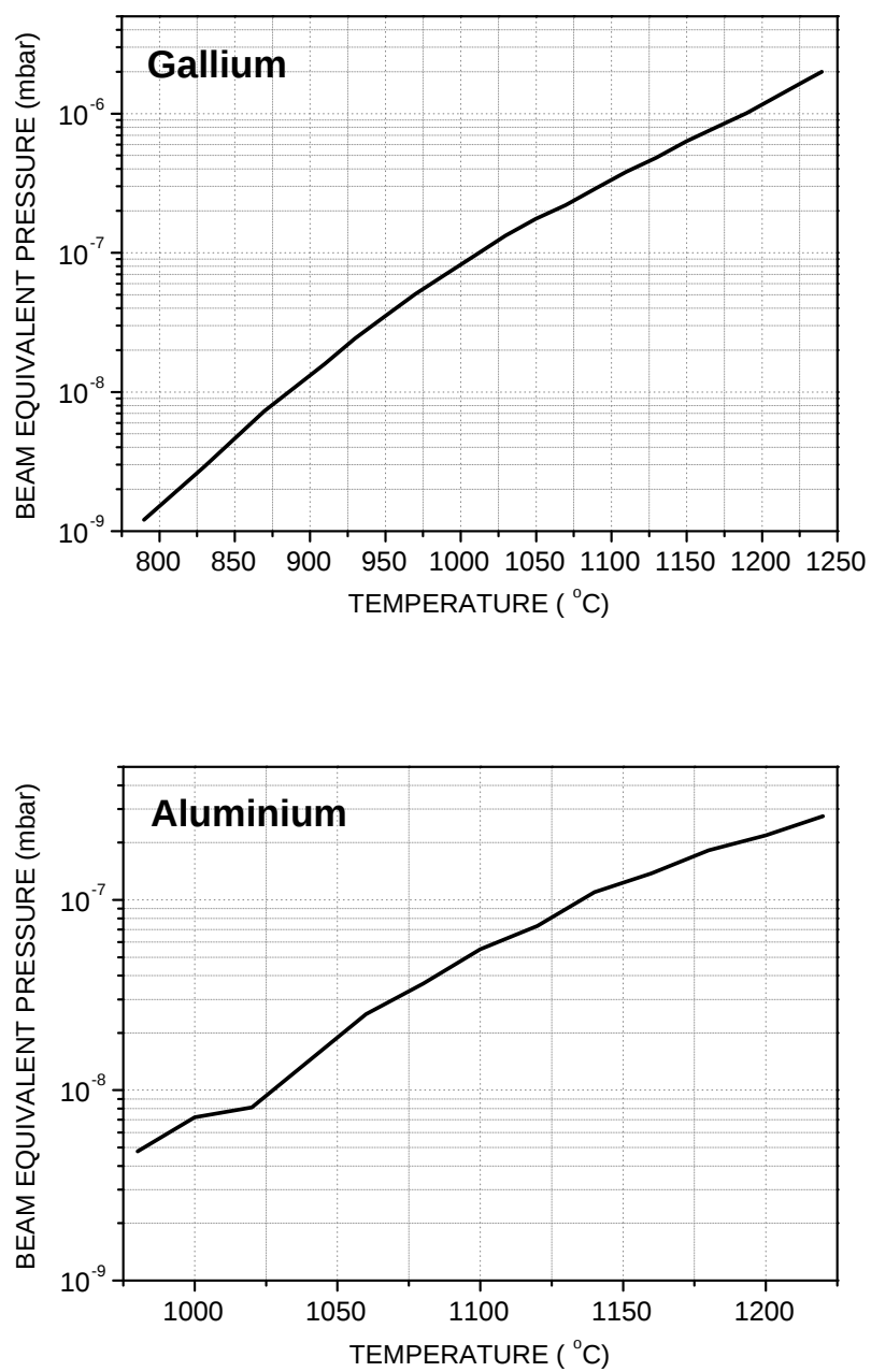
Figure 4.2: Beam equivalent pressure (BEP) of the gallium (top) and aluminium (bottom) effusion cells as a function of temperature.
