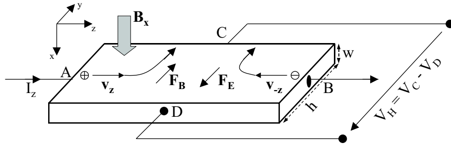
Figure 3.15: Sign convention and terminology for a rectangular Hall sample.
