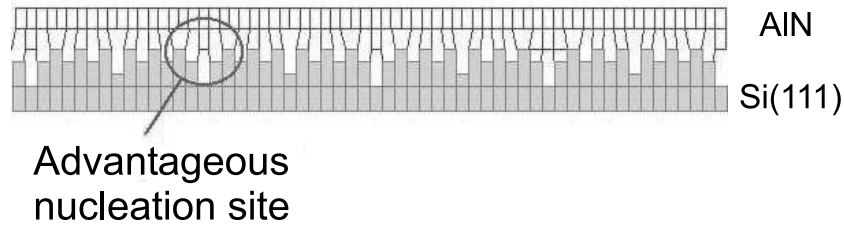
Figure 6.32: 17:14 lattice matching of a AlN on the (7 \times 7) reconstructed surface of Si(111) [181].
