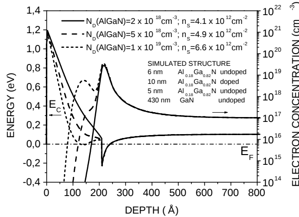
Figure 5.9: Band scheme simulation of a modulation doped \text{Al}_{0.18}\text{Ga}_{0.82}\text{N}/\text{GaN} heterostructure with three different doping densities: 2 \times 10^{18} , 5 \times 10^{18} , 1 \times 10^{19} \text{ cm}^{-3} . The conduction band minimum profile (left scale) and free electron concentration profile (right scale) are displayed. A background electron concentration of 10^{17} \text{ cm}^{-3} is assumed in undoped layers. The concentration in 2DEG is shown in the legend for all calculations.
