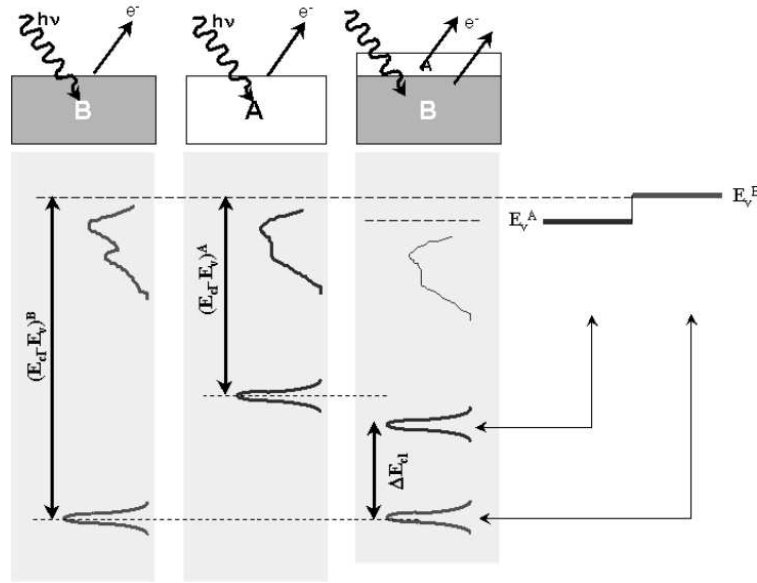
Figure 3.12: Schematic representation of the measurement of the valence band offset at an interface by means of photoemission spectroscopy.
