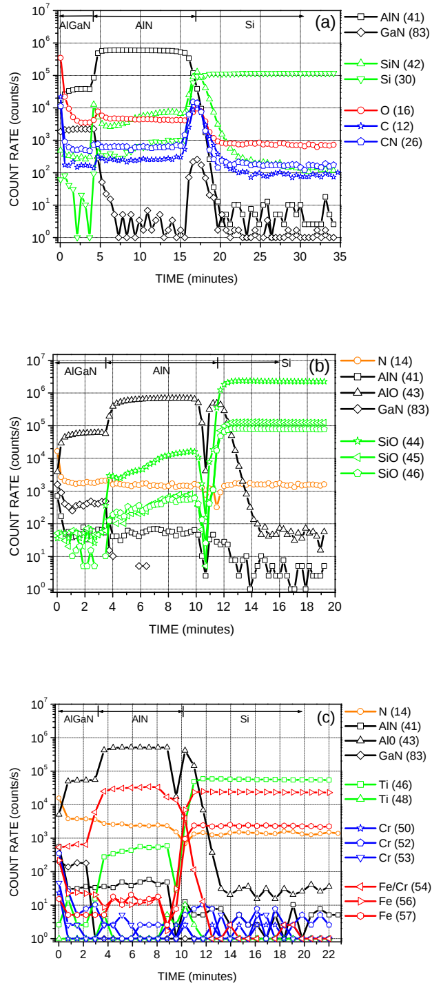
Figure 6.39: SIMS analysis of the sample ED153 ( \text{Al}_{0.11}\text{Ga}_{0.89}\text{N}(100\text{ nm})/\text{AlN}(100\text{ nm})/\text{Si}(111) ). The numbers reported in brackets in the legend are relative atomic masses.
