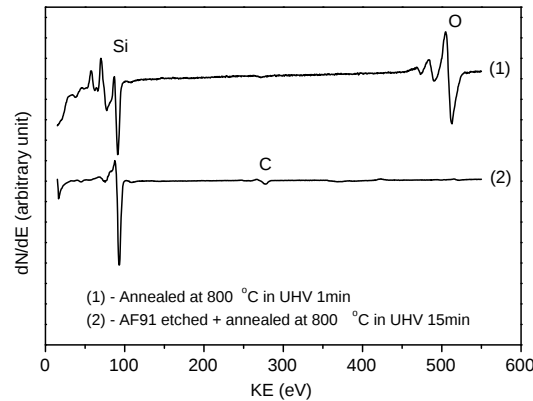
Figure 6.30: Comparison between Auger spectra of Si substrates cleaned in different ways (see text).
