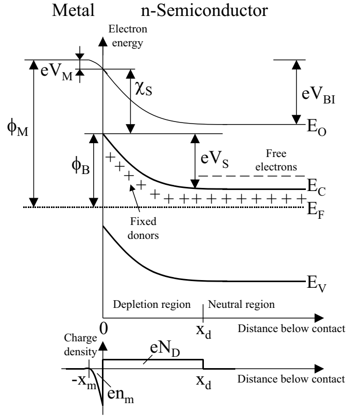
Figure 3.14: Energy band diagram of a metal-semiconductor Schottky barrier and associated charge density profile for uniformly doped material. The diagram is constructed assuming the vacuum level is continuous across the interface.
