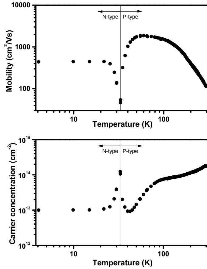
Figure 6.41: Temperature dependent Hall experiment data of AlGaIn/GaN MBE structures grown on Si(111).
