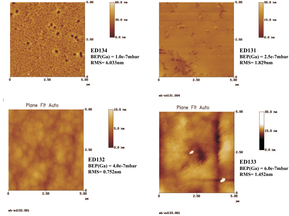
Figure 6.4: Comparison of the surface morphologies of GaN layers grown with different Ga fluxes.
