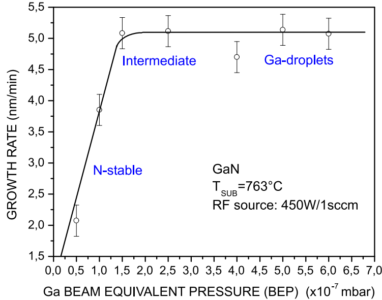
Figure 6.2: GaN growth rate for different Gallium beam equivalent pressures. The N flux was 1 sccm and the RF power 450 W.
