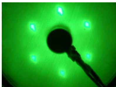
Figure 6.8: LEED image of a SiC substrate after the cleaning procedure.
