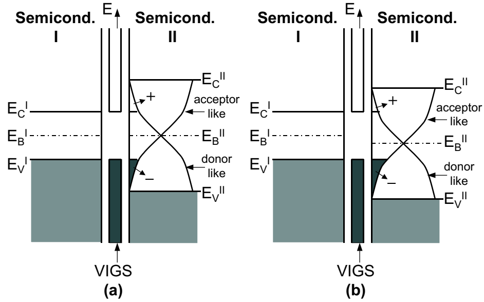
Figure 2.9: Schematic explanation of the formation of a semiconductor heterostructure in terms of Virtual Induced Gap States (VIGS) model. The band schemes of two semiconductors are plotted with conduction-band edge E_C and valence-band edge E_V . The matching of the two band schemes, i.e. the band off-sets, are determined by charge neutrality within the VIGS.
