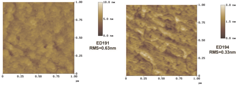
Figure 6.10: 1 \times 1 \mu\text{m}^2 AFM picture of ED191 and ED194. Notice that the color scales are different.
