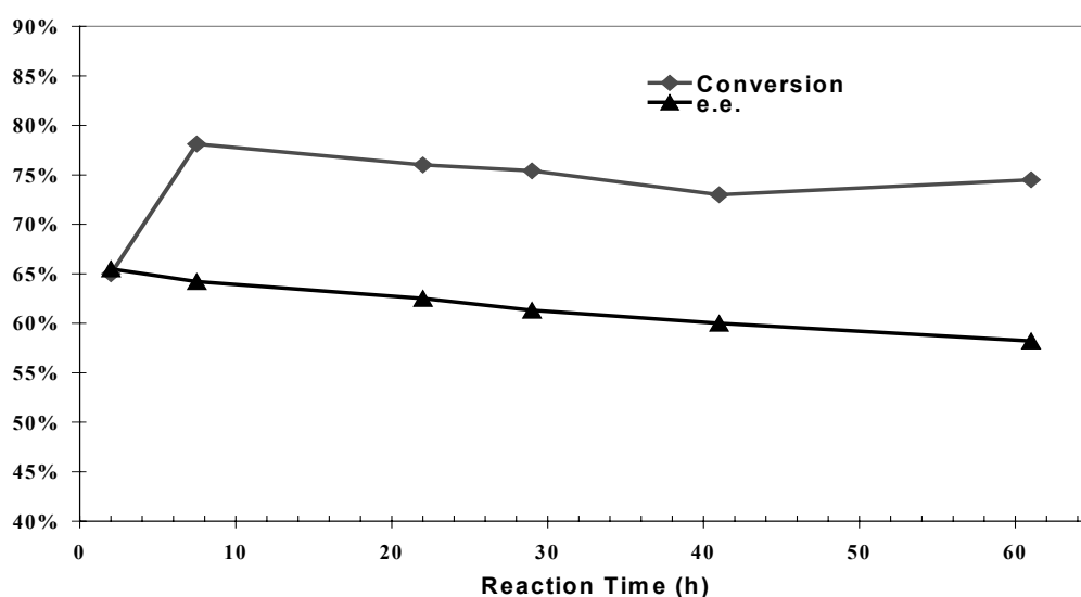
Figure 2-24: Lifetime study for the Wilke's catalyst in the continuous flow hydrovinylation of styrene.
