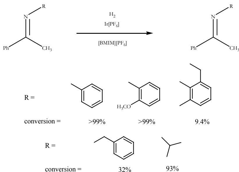
Scheme 2-22: Substrate scope of the iridium catalyst \text{Ir}[\text{PF}_6] in the ionic liquid [\text{BMIM}][\text{PF}_6]
