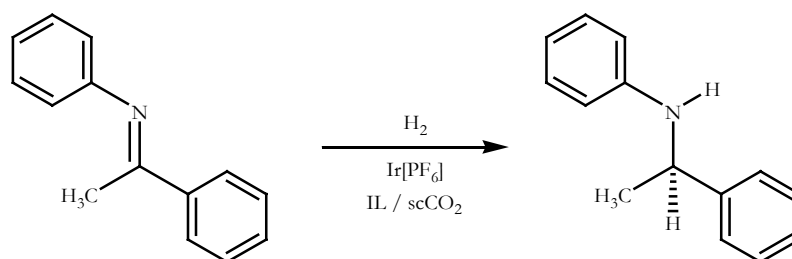
Scheme 2-21: Enantioselective imine hydrogenation with the phosphanodihydrooxazole iridium catalyst Ir[PF 6 ] in IL/CO 2 system.
