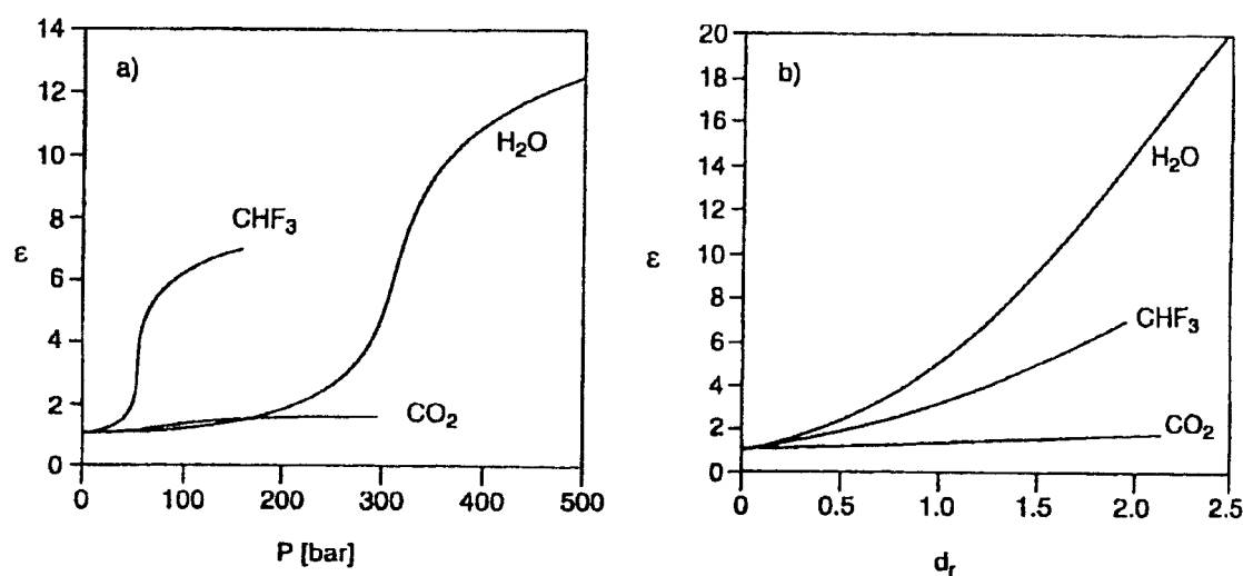
Figure 2-3: Variation of the dielectric constant of \text{H}_2\text{O} (at 400 °C, T_r = 1.04 ), \text{CO}_2 (at 40 °C, T_r = 1.03 , and \text{CHF}_3 (30 °C, T_r = 1.01 ) as a function of pressure and reduced density. Taken from reference [6a].
