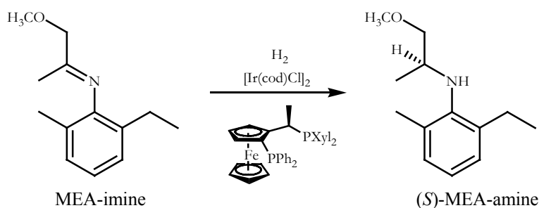
Scheme 2-18: Enantioselective hydrogenation of the (2-ethyl-6-methyl-phenyl)-(2-methoxy-1-methyl-ethylidene)-amine (MEA imine) with iridium-xylyphos.
