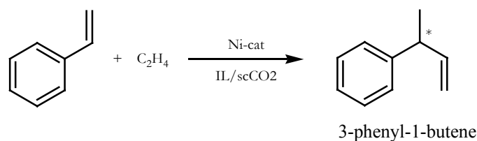
Scheme 2-16: Enantioselective hydrovinylation of styrene in ionic liquid / \text{scCO}_2 system.
