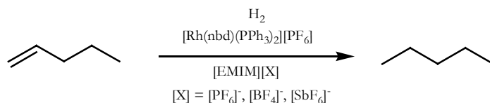
Scheme 2-10: Biphaseic hydrogenation of 1-pentene in [\text{BMIM}][\text{X}] ionic liquids.
