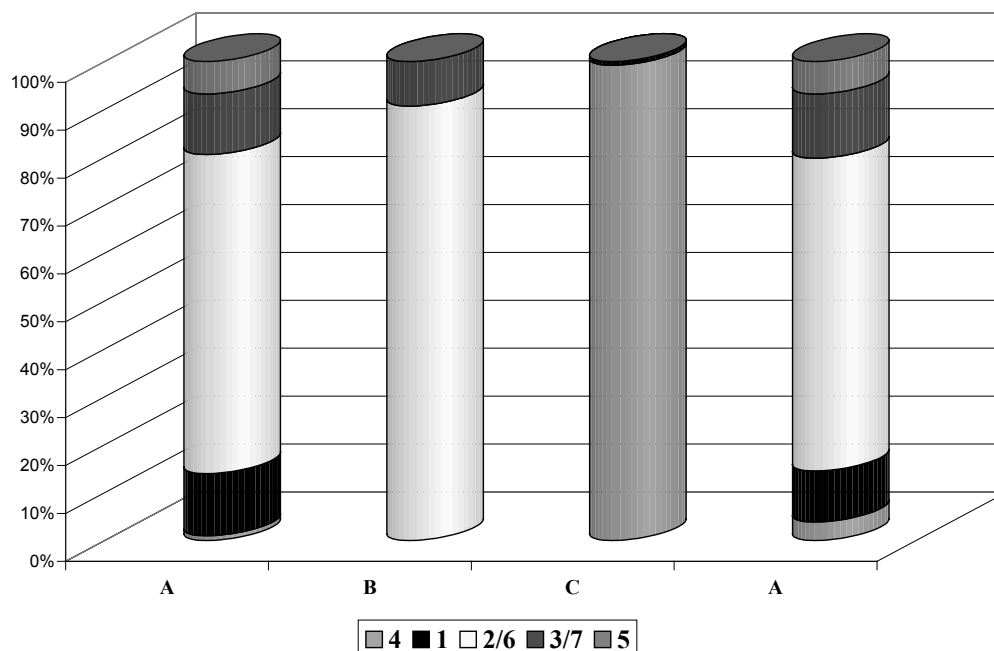
Figure 3-5: Series of consecutive reactions using the same catalytic solution; the extraction is performed with \text{scCO}_2 . ( [\text{Rh}(\text{CO})_2(\text{acac})] = 0.01 \text{ mmol} ; ligand \text{MeOPEG}_{750}\text{PPh}_2 = 0.05 \text{ mmol} ; styrene = 10 mmol; Reaction A : Pinacolborane = 10 mmol bar; time = 3 hours; temp. = 25 °C; Reaction B : \text{CO}/\text{H}_2 = 50 \text{ bar} , time 2 hours, temp. 70 °C; Reaction C : \text{H}_2 = 50 \text{ bar} ; time 2 hours, temp. = 50 °C).
