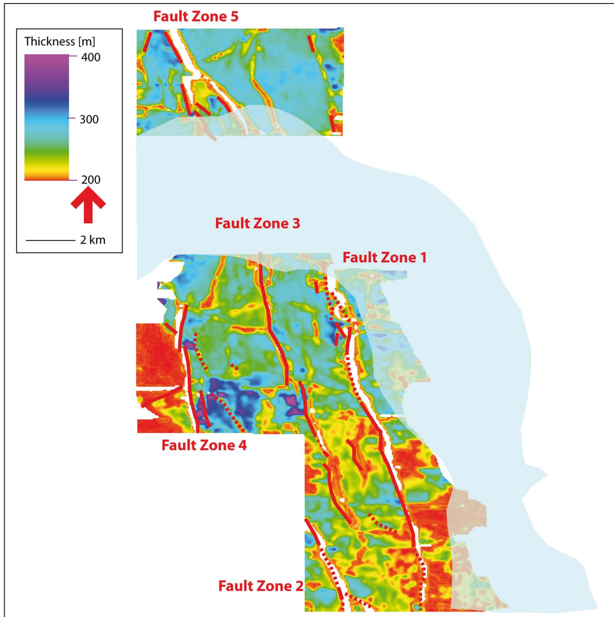
Fig. 4.5. Upper Rotliegend II isopach Map; note that Rotliegend in the study area comprises Base Ebstorf until Top Heidelberg. Faults with a paleorelief observed for the Rotliegend are marked in red. Overlying diapiring Zechstein salt, which affects the seismic resolution, is depicted in transparent blue. A left-lateral pull-apart sub-basin provides a localized depocentre associated with Fault Zone 1. The lowest sediment thickness developed on the footwall of Fault Zone 4, whereas the area of highest sediment thickness is located on the hangingwall of Fault Zone 4, forming a Rotliegend depocentre. Fault Zone 3 shows pronounced sediment thickness variations between foot- and hangingwall in the middle part with high thicknesses of up to 400m developed on the hangingwall.
