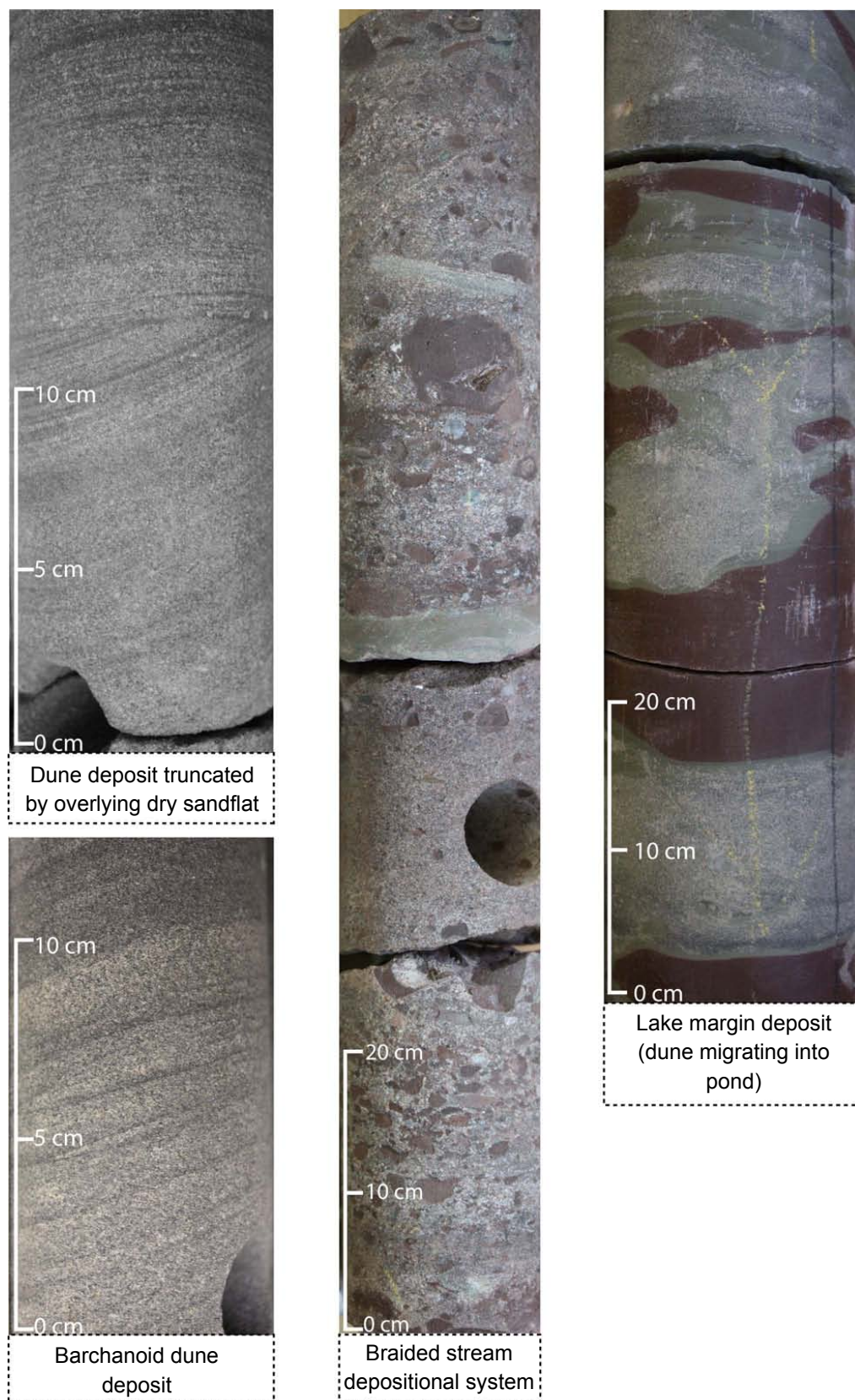
Fig. 4.8. Core material of Well 3. The core succession is dominated by wet to dry aeolian deposits. Volcanics and their overlying breccias and the deposits of braided stream dominated alluvial fans are situated in the lower part of the core beneath the reservoir rocks.
