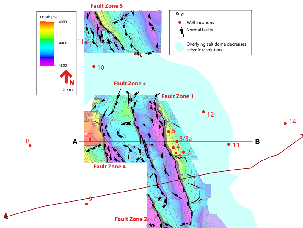
Fig. 4.1. Field development and structural features of the study area illustrated on the Top Rotliegend Depth Map. The W-E-trending red line depicts detailed interpreted seismic section shown in Fig. 4.2. Line with arrowheads displays orientation of regional 2D Seismic Line.
