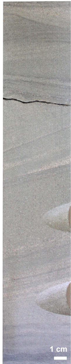
Fig. 3.14. Aeolian dune base and dune deposits. N C GER, Well II.
