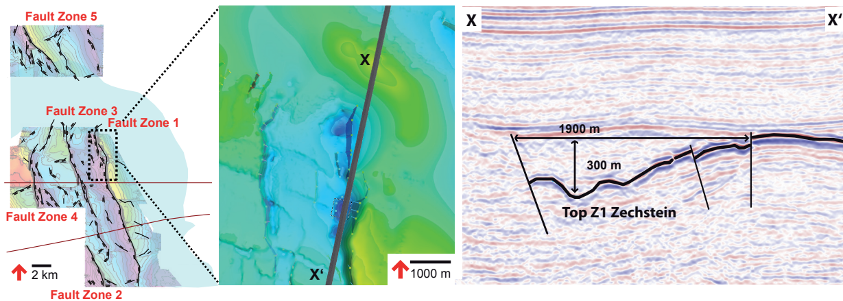
Fig. 4.4. Fault-controlled sub-basin. Left: Basemap. Middle: Depth Map of Zechstein Z1 Surface. Right: Seismic Section running parallel to the elongate sub-basin with faults depicted in thinner stroke and Top Z1-Zechstein seismic horizon displayed in thicker stroke.
