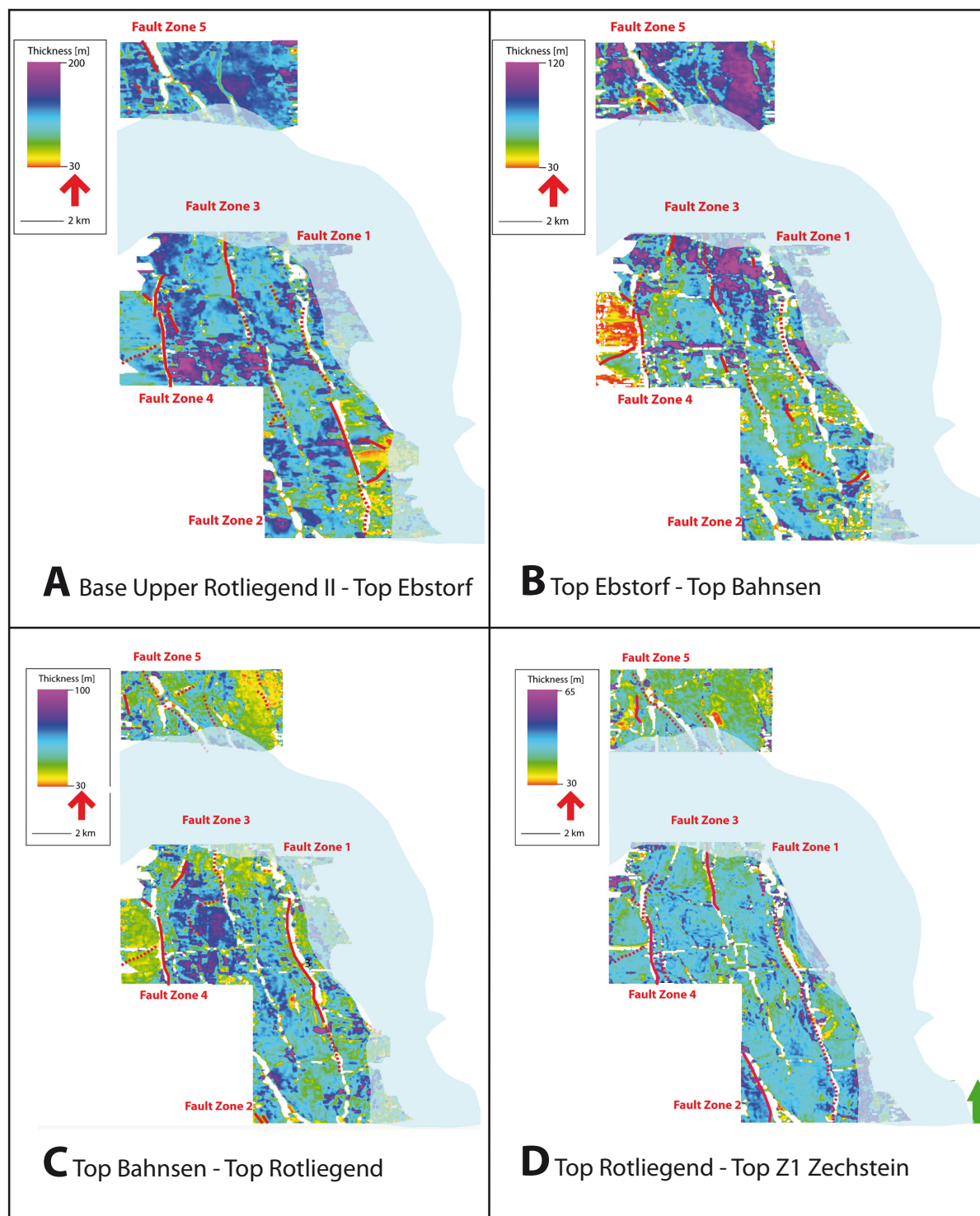
Fig. 4.6. Detailed isopach maps of the Rotliegend and Lower Zechstein. A: Base Upper Rotliegend II – Top Ebstorf: B: Top Ebstorf to Top Bahnsen = reservoir isopach map: C: Top Bahnsen – Top Rotliegend: Fault Zone 4 with paleorelief. D: Zechstein Z1 Isopach Map. Enlarged sediment thicknesses can be observed for the area around the wedge-like structure between fault zones 1 and 3. It is displayed separately in Fig. 4.9. Faults with a palaeo-relief observed are marked in red. Overlying Zechstein salt which affects the seismic resolution is depicted in transparent blue.
