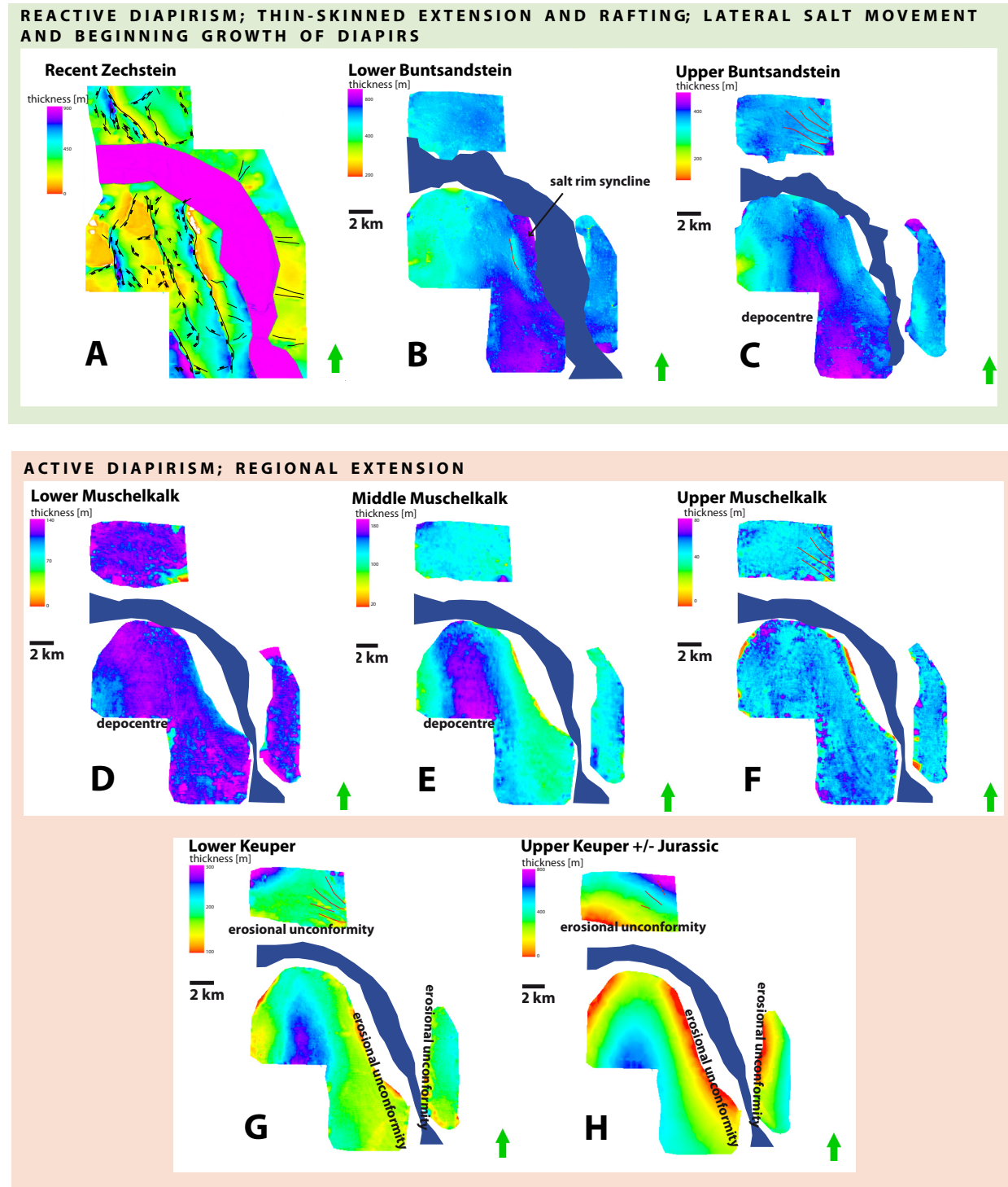
Fig. 6.5. Part 1. Isopach maps of the study area from old to young. Plot is in context to different salt tectonic mechanisms.
