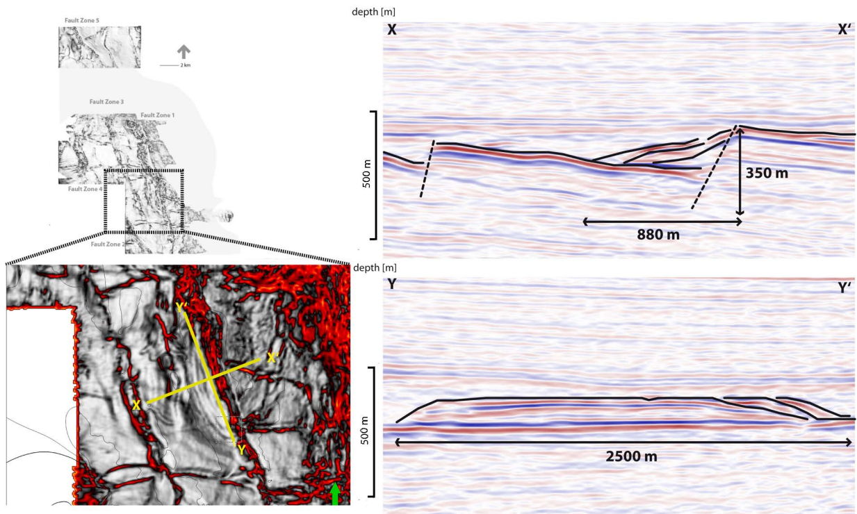
Fig. 4.9. Arcuate salt removal wedge on Top Z1-Zechstein variance horizon slice and in seismic sections. Upper left: Top Z1-Zechstein variance horizon slice with overlying salt and fault zone annotations. Lower left: Z1 Zechstein variance horizon slice zoomed on the outlines of the wedge-like structure. X-X' and Y-Y' Location of seismic sections displayed on the right. Upper right: seismic section perpendicular to Fault Zone 1 that borders the wedge-like structure. Different salt removal cycles or reflectors of floaters can be observed. Lower right: seismic section cut parallel to Fault Zone 1. The reflectors outline a lobate structure with removal cycles or floater reflectors to the N.
