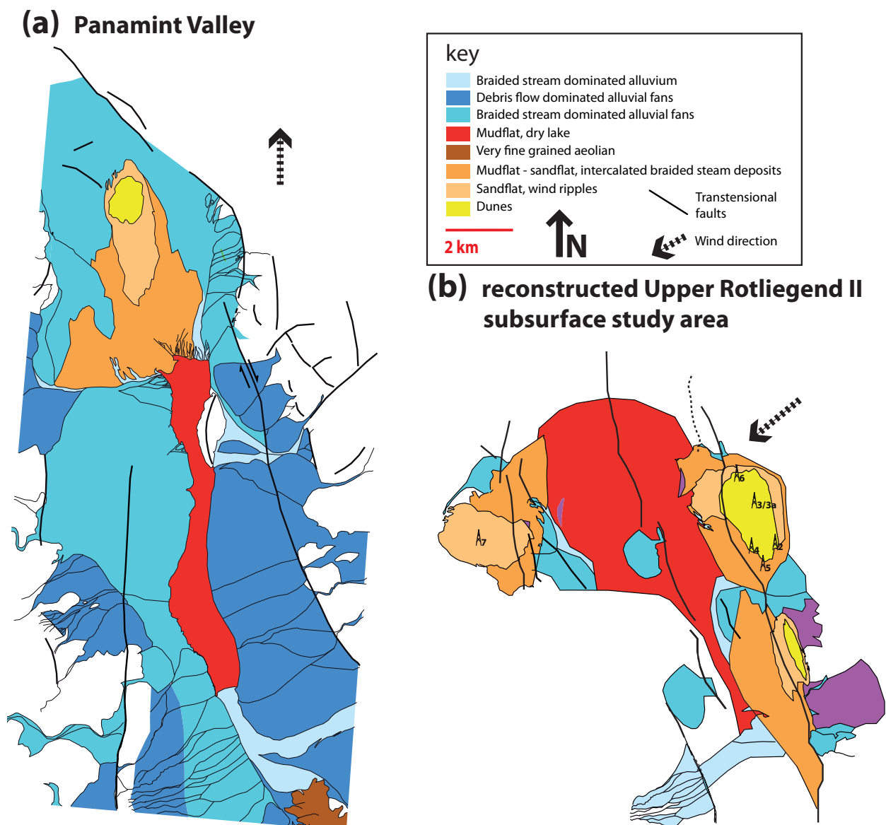
Fig. 5.9. Comparison between the simplified sedimentary facies distribution of Panamint Valley (a) on the left and of the German subsurface study area on the right (b).
