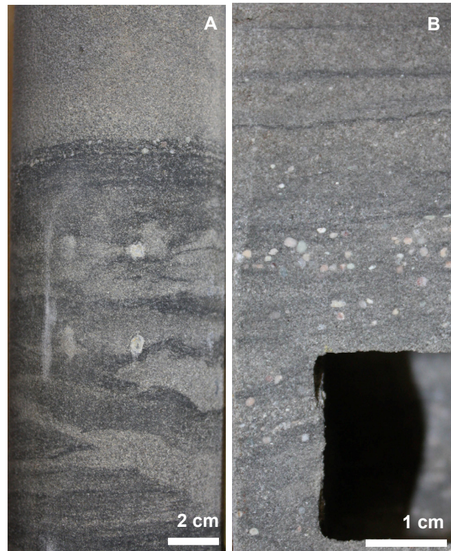
Fig. 3.10. A: Damp sandflat deposit truncated by deflation lag. NW GER, Well 3. B: Damp sandflat deposit with adhesion lags. N C GER, Well IV.
