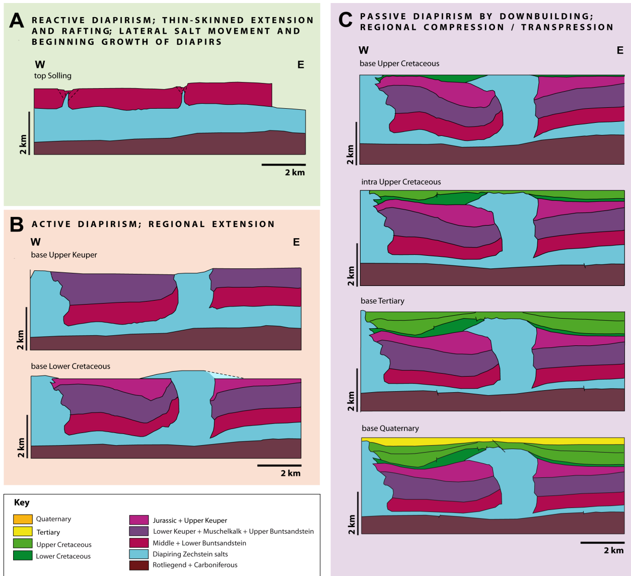
Fig. 6.8. Retro-deformed, depth converted seismic line from northern central Germany. Illustration from old to young (inverse), depicted in context of different salt tectonic mechanisms, indicated by coloured frames.
