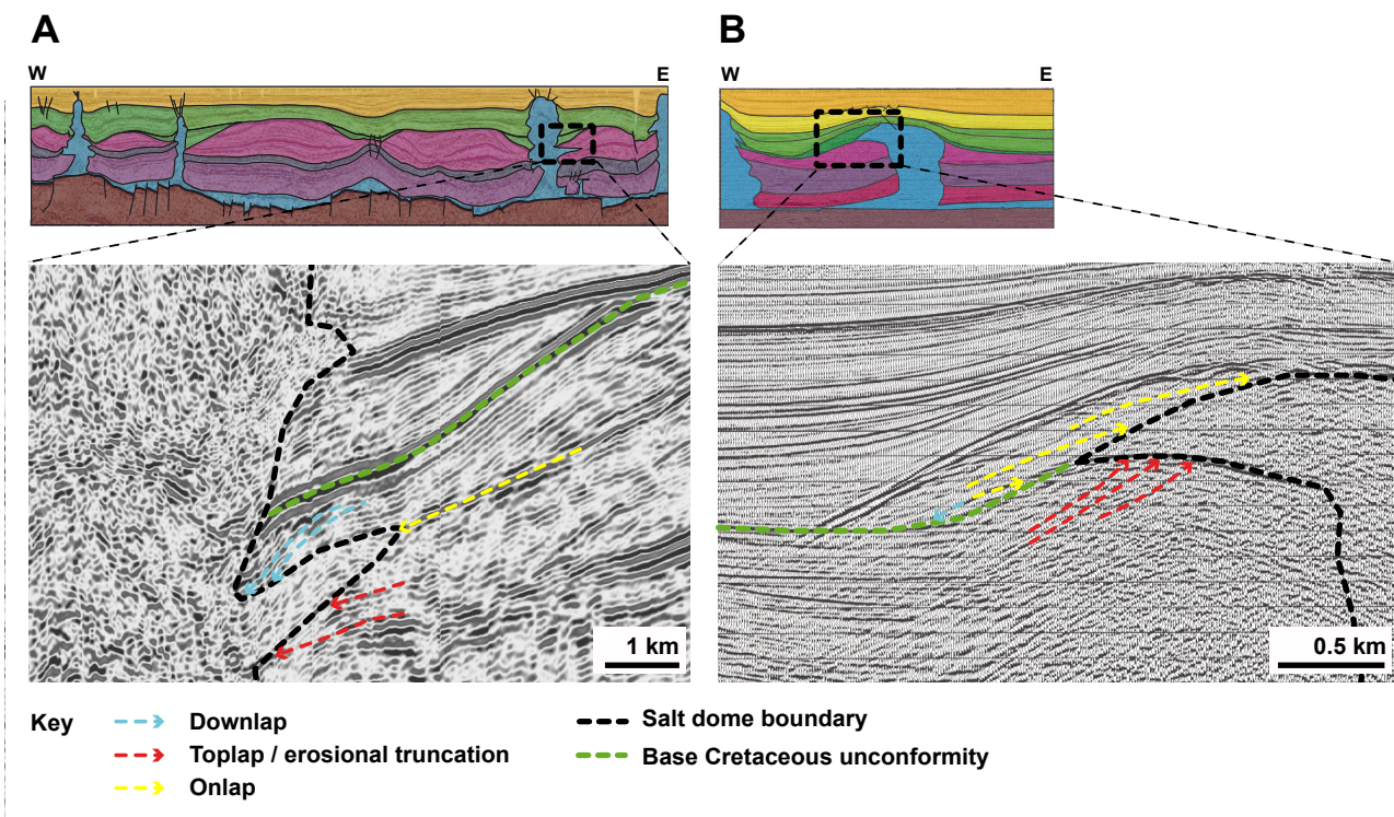
Fig. 6.9. Zoom of the areas of huge potential salt namakiers with lap geometries of underlying and overlying sediments displayed. Left: salt namakier in 2D Regional seismic line in north-western Germany. Right: Salt namakier in northern central German 2D seismic line.
