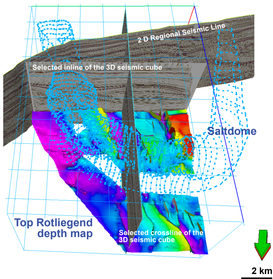
Fig. 3.2. Overview of the seismic data set from north-western Germany, view from the north. 3D seismic survey displayed with structural model, salt diapir extent and Top Rotliegend depth map. The regional 2D seismic line crosses the 3D seismic survey in the south and continues eastwards for another ~80 km. The salt dome extent is extrapolated towards the west. Shape of the salt dome outside the seismic survey based on Jaritz (1973) and Baldschuhn et al. (1999).
