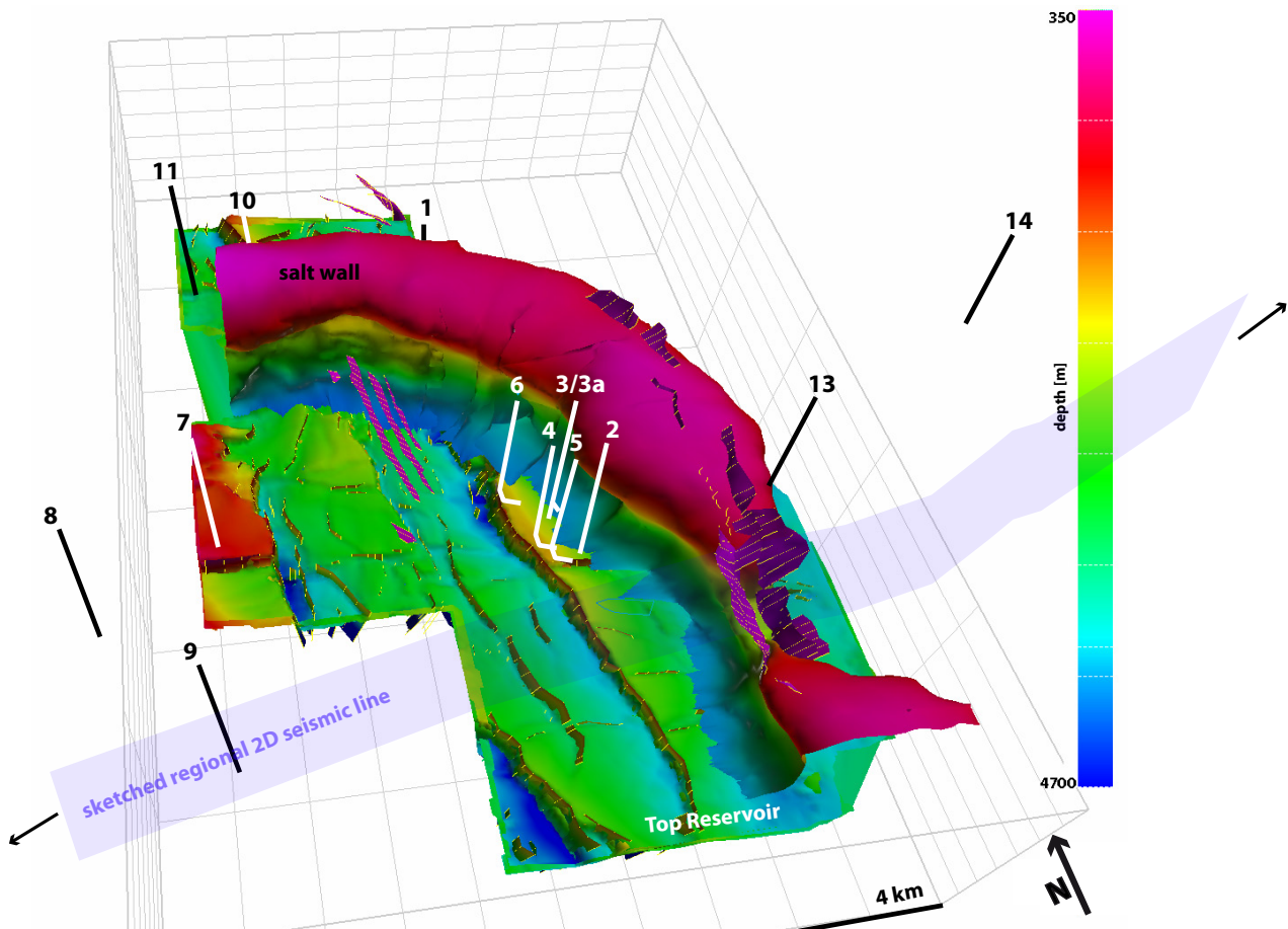
Fig. 3.1. Overview of the seismic data set from north-western Germany, view from the south. 3D seismic survey displayed with faults, salt wall and Top Reservoir depth map. Faults of Zechstein overburden strata are displayed in pink. The regional 2D seismic line (blue shade) crosses the 3D seismic survey in the south and continues eastwards for another ~80 km. The existing wells are depicted in black and white.
