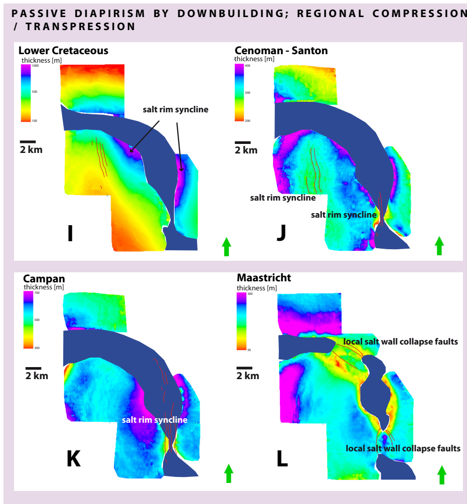
Fig. 6.5. Part 2. Isopach maps of the study area from old to young. Plot is in context to different salt tectonic mechanisms.
