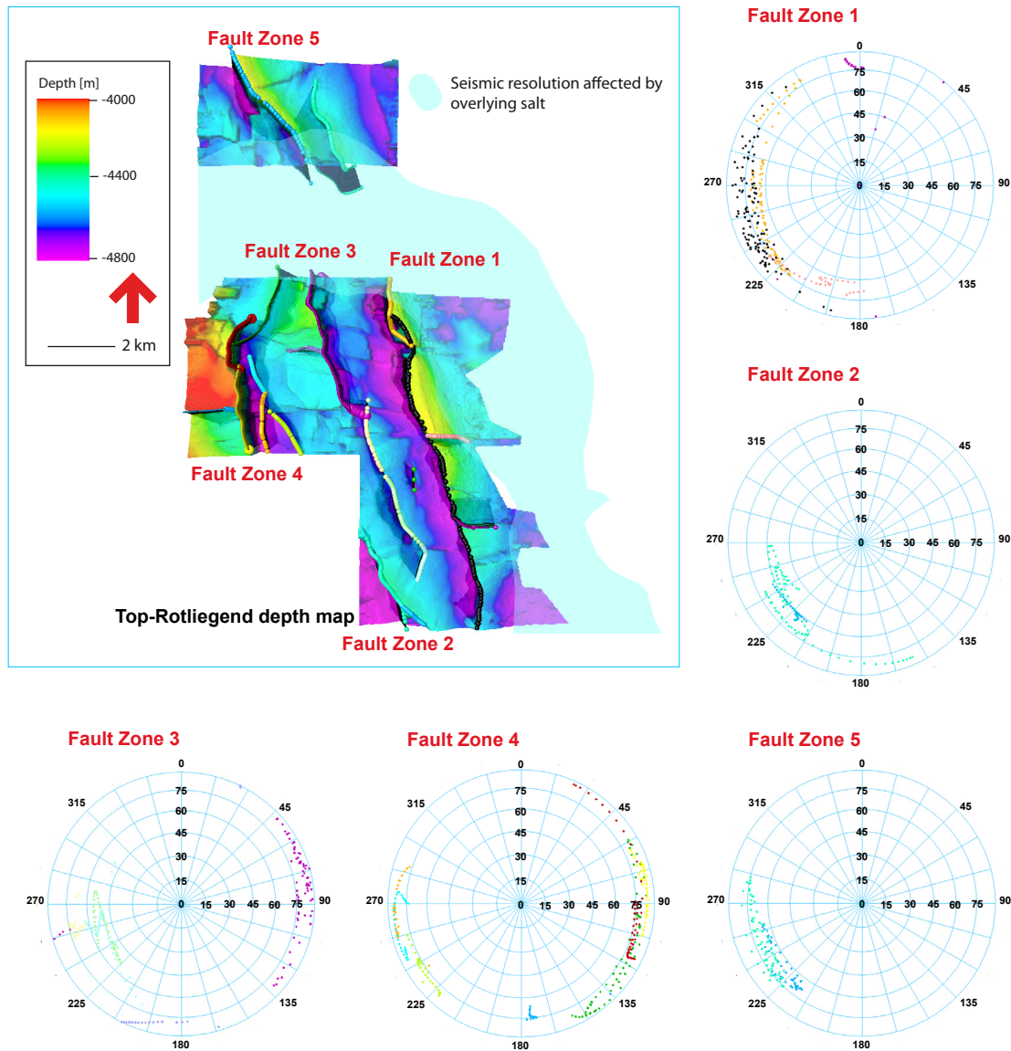
Fig. 4.3. Upper left: Major fault zones of the study area (see text for explanation.). Right and below: Orientations of fault planes constructed from structural analysis on seismic data plotted in Schmidt equal-area, upper-hemisphere contour diagrams.
