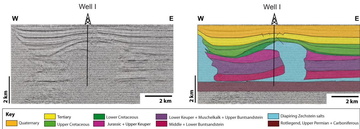
Fig. 6.4. Left: Northern central German 2D seismic line used for retro-deformation (orange framed in Fig. 6.1). Right: Seismic line with overlying interpretation and well position.
