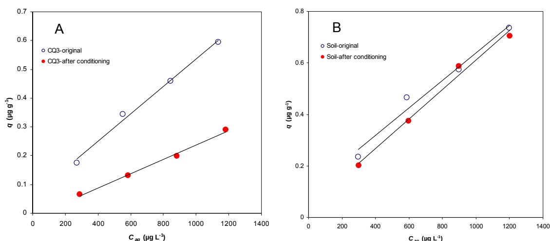
Figure 4.38 Adsorption comparison before and after conditioning (A: sediment CQ3; B: soil)
