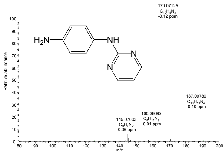
Figure 4.12 Accurate mass: APCI-FTICR-MS product ion spectrum of p-(pyrimidin-2-yl)aminoaniline ( MS^2 of precursor ion m/z 187). The empirical formulas are calculated on the basis of the high resolved masses, the deviations from the theoretical masses are expressed in ppm
