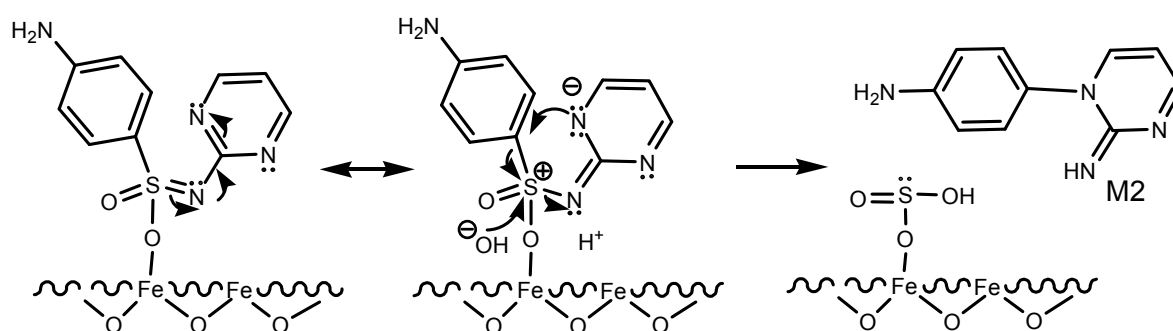
Figure 4.19 Proposed transformation pathway of SDZ to M2 in SDZ-goethite suspension
