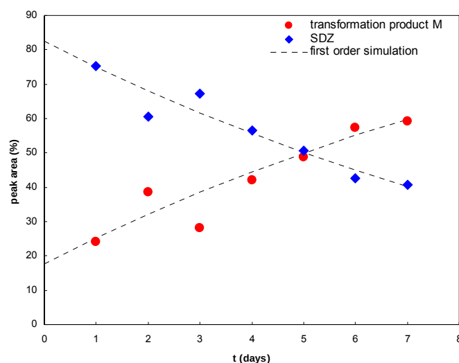
Figure 4.4 Peak area of transformation product M and SDZ (Radio-HPLC) versus contact time ( ^{14}\text{C} -SDZ: 0.5 \text{ mg L}^{-1} , goethite: 20 \text{ g L}^{-1} , in dark)
