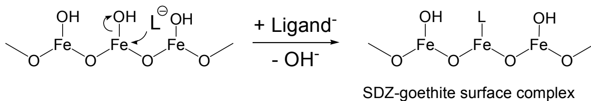
Figure 4.18 Formation of SDZ-goethite surface complex
