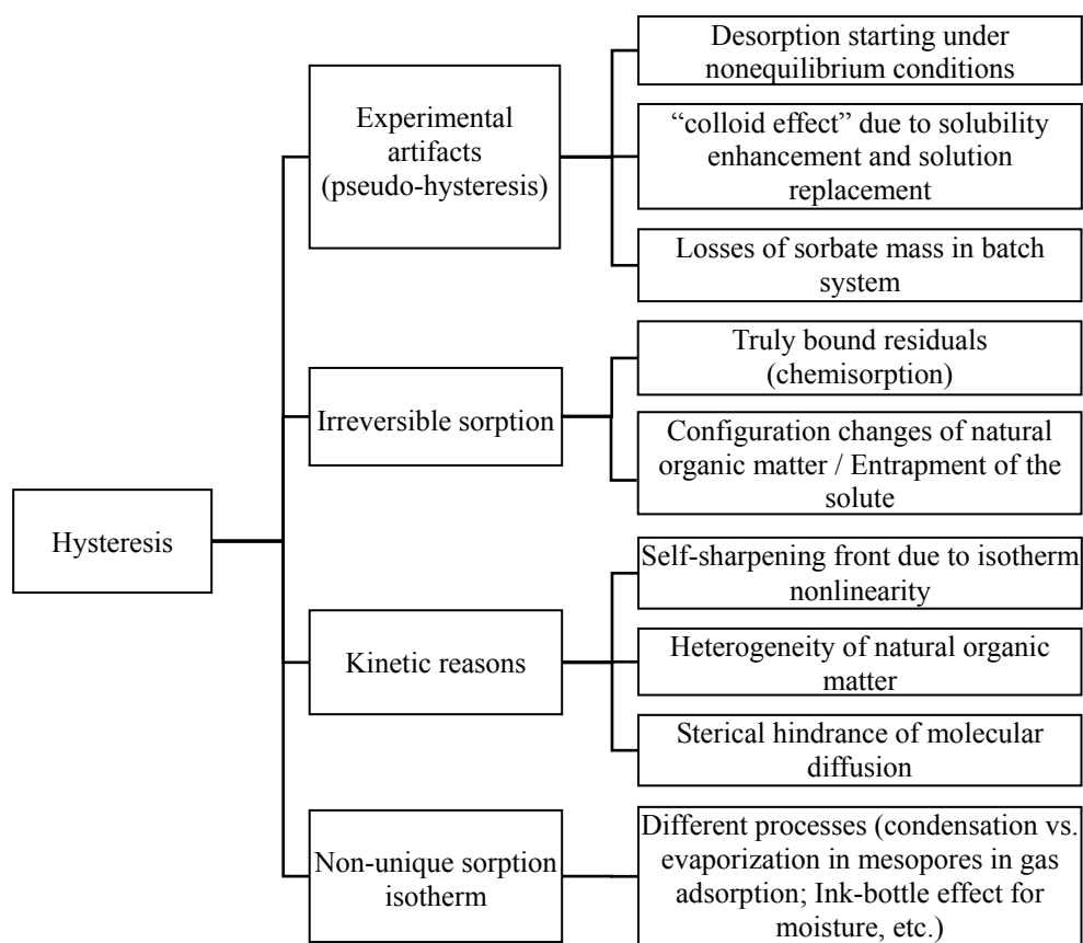
Figure 2.6 Process and manifestations of hysteresis (Wang, 2008)
