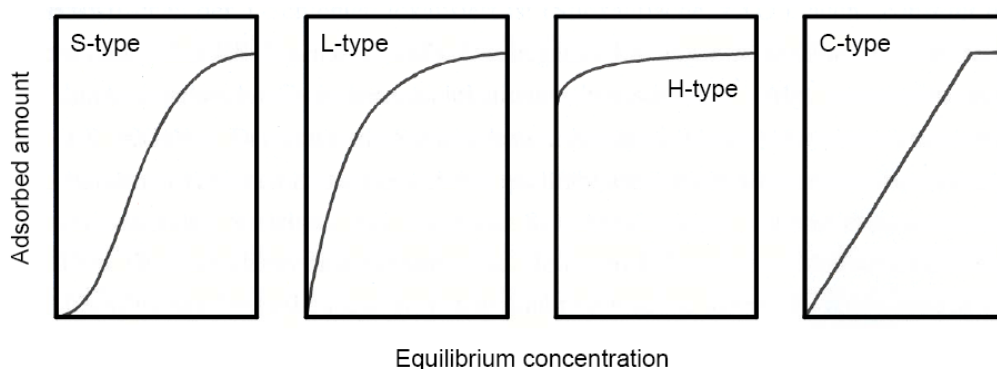
Figure 2.5 Classification of adsorption isotherms (Giles et al., 1974)
