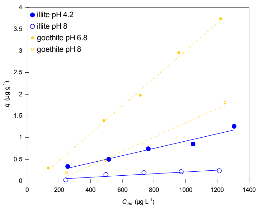
Figure 4.24 ^{14}\text{C} -SDZ adsorption isotherms on illite and goethite with pH adjustment (on goethite, the “adsorption isotherm” cannot be evaluated because of the simultaneous transformation process; pH was adjusted by Tris buffer)
