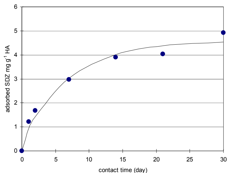
Figure 4.26 Sorption kinetic uptake curve of SDZ on IHSS-HA, curve was fitted by first order kinetics ( C_{HA} = 1500 \text{ mg L}^{-1} , C_{SDZ_{initial}} = 60 \text{ mg L}^{-1} , pH = 6)
