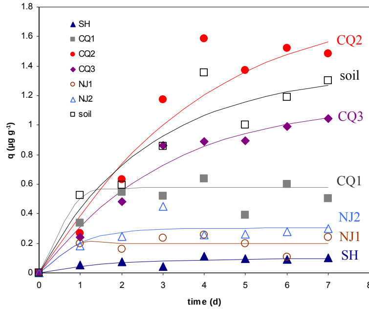
Figure 4.27 ^{14}\text{C} -SDZ sorption kinetics on Yangtze sediments and Merzenhausen soil in 7 days; curves are fits by first order kinetics ( C_{\text{SDZ}_{\text{initial}}} = 0.5 \text{ mg L}^{-1} , C_{\text{sediment, soil}} = 100 \text{ g L}^{-1} )
