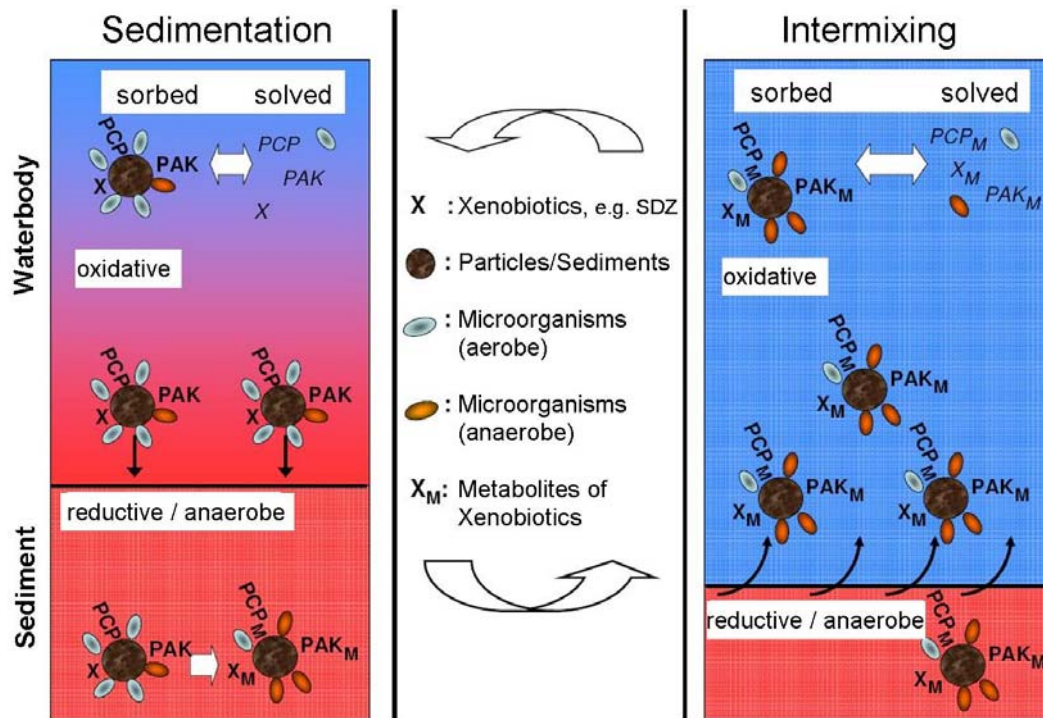
Figure 1.1 Physicochemical and biological interactions in the pollutant/water/sediment system (Thiem et al.)
