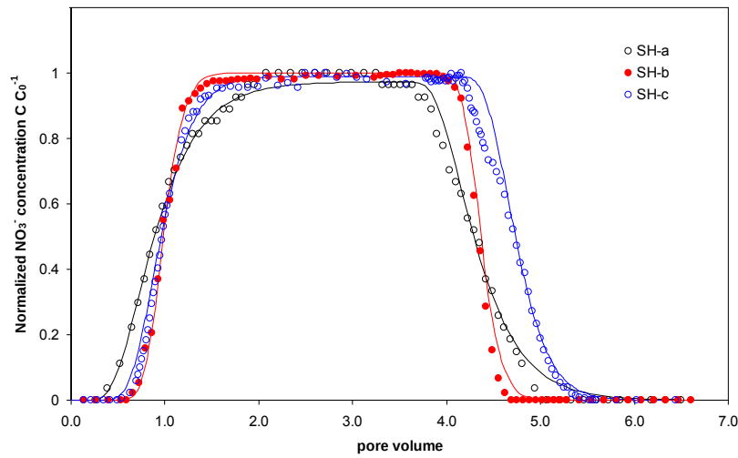
Figure 4.34 Breakthrough curves of nitrate for the SH sediment at different conditions. Experimental data - colored points, fitted curves by equilibrium CDE - colored lines (flow velocity: SH-a, 0.2 ml min -1 ; SH-b, 0.2 ml min -1 ; SH-c, 0.05 ml min -1 )
