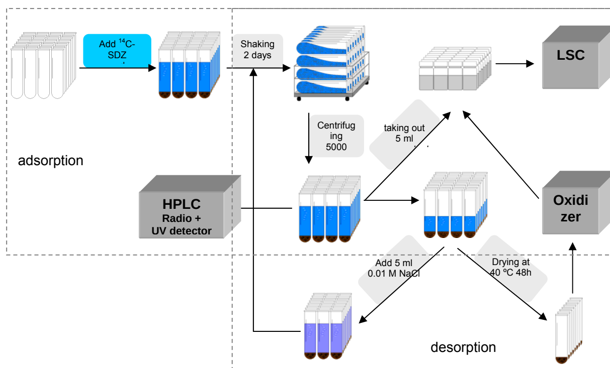
Figure 3.2 Ad/desorption procedure
