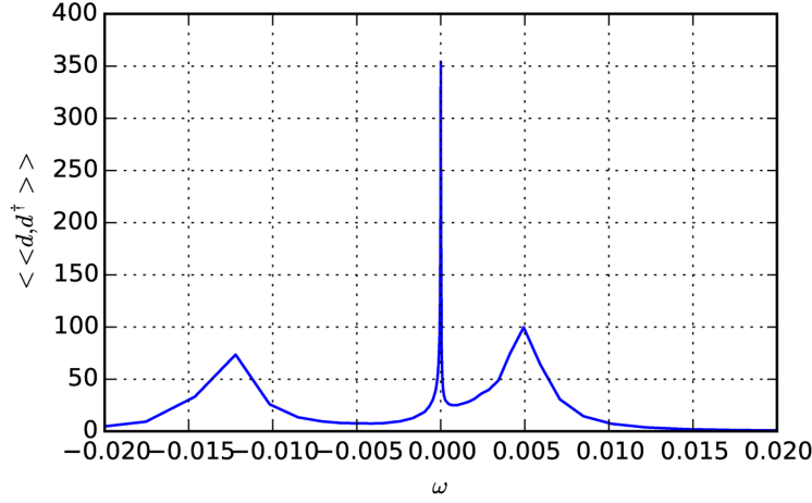
Figure 2.6: The figure shows the spectral function \mathcal{A}_{\mathbf{d},\mathbf{d}^\dagger}(\omega) evaluated at single shells. The discretization parameters used were n_z = 64 and \Lambda = 8 .
