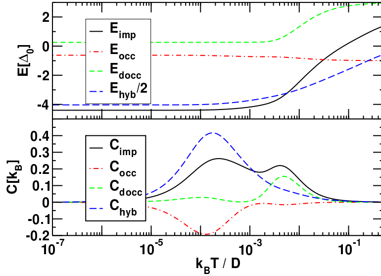
Figure 3.7: Individual contribution of (a) E_{\text{occ}} , E_{\text{docc}} and E_{\text{hyb}}/2 to E_{\text{imp}} as a function of temperature for the asymmetric model with parameters as in Figure 3.1 but \varepsilon_d = -1\Delta_0 . (b) Temperature derivative of the above yielding the individual contributions C_{\text{occ}} , C_{\text{docc}} and C_{\text{hyb}} to the impurity specific heat C_{\text{imp}} .
