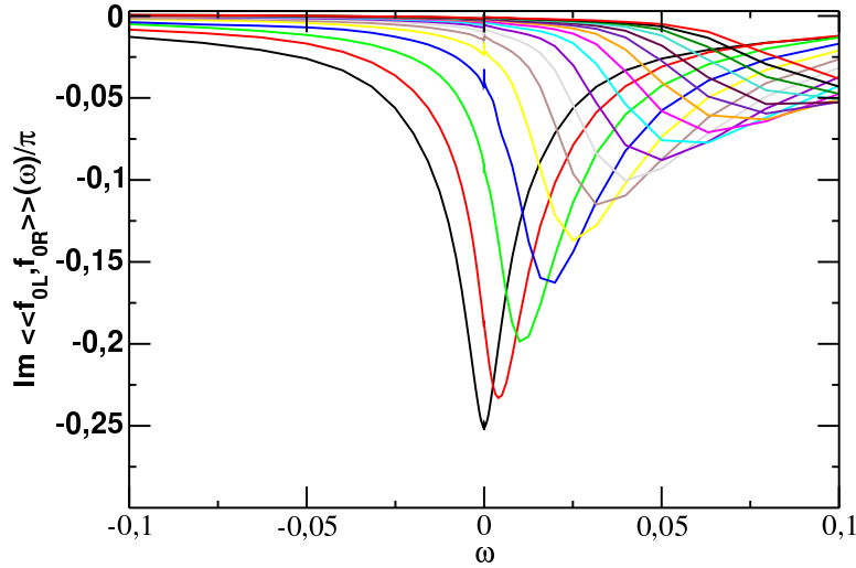
Figure 7.3: \mathcal{A}_{f_{0,R}, f_{0,L}^{\dagger}}(\omega) for different values of \varepsilon_d = -\Gamma \dots 15\Gamma , U = 2\Gamma , \Gamma = 0.01 , U' = 0 . There is a numerical problem at \omega \approx 0 even for \omega > T .
