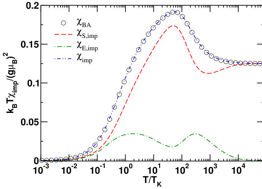
Figure 4.1: Impurity contribution to the susceptibility from Bethe ansatz ( \chi_{\text{BA}} ) and FDM ( \chi_{\text{imp}} ) vs T/T_K for the symmetric Anderson model [ U/\Delta_0 = 12 and \Delta_0 = 0.001D with T_K defined in Equation (4.15)]. Also shown are the impurity contributions k_B T \chi_{\text{S,imp}}(T)/(g \mu_B)^2 and k_B T \chi_{\text{E,imp}}(T)/(g \mu_B)^2 as defined at the end of Section 4.3. The calculations are for \Lambda = 10 with an energy cut-off e_c(\Lambda) = 15\sqrt{\Lambda} \approx 47 , with z -averaging [ n_z = 4 , z = 1/8, 3/8, 5/8, 7/8 ].
