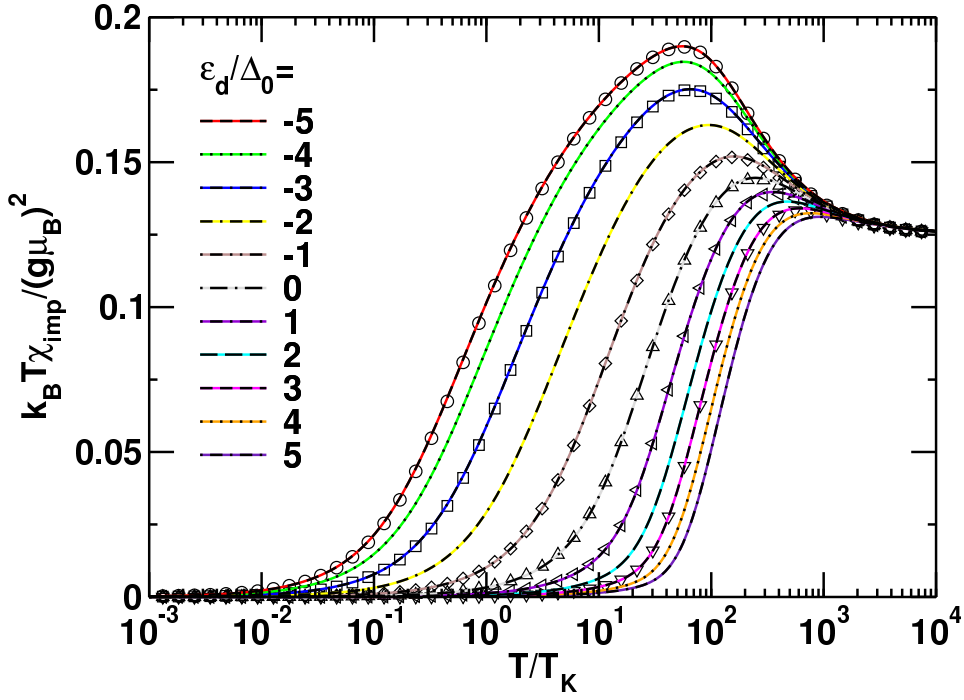
Figure 4.5: Impurity susceptibility, \chi_{\text{imp}}(T) , vs T/T_K for the asymmetric Anderson model with U/\Delta_0 = 12 , \Delta_0 = 0.001D and several values of \varepsilon_d/\Delta_0 with T_K defined in Equation (4.15). Broken lines: FDM approach. Solid lines: conventional approach. Symbols: Bethe ansatz (for selected values of \varepsilon_d/\Delta_0 = -5, -3, -1, 0, +1, +3 ). As a guide to the eye, note that the susceptibility curves shift to higher temperatures with increasing \varepsilon_d . NRG and z -averaging parameters as in Figure 4.1.
