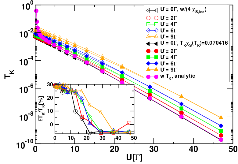
Figure 7.7: Comparison between different methods to calculate the Kondo Temperature for the symmetric Anderson Model with screening. The Wilson number w = 0.41071\dots connects T_0 with the Kondo Temperature T_K . T_K was extracted by linear interpolation of T\chi_S(T) for T = 1 \times 10^{-10} \dots 1 \times 10^{-1} using 51 values for T . Both methods give similar results in the Kondo limit. The calculation details are the same as in Figure 7.9.
