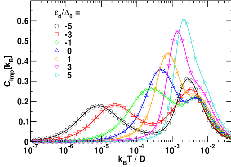
Figure 3.10: Temperature dependence of C_{\text{imp}}(T) for U/\Delta_0 = 12 , \Delta_0 = 0.001D and local level positions \varepsilon_d/\Delta_0 ranging from Kondo ( \varepsilon_d/\Delta_0 \leq -1 ), mixed valence ( |\varepsilon_d/\Delta_0| \leq 1 ), and empty orbital ( \varepsilon_d/\Delta_0 > 1 ) regimes. Symbols: NRG calculations (new approach, z -averaging and NRG parameters as in Figure 3.1). Lines: Bethe ansatz calculations.
