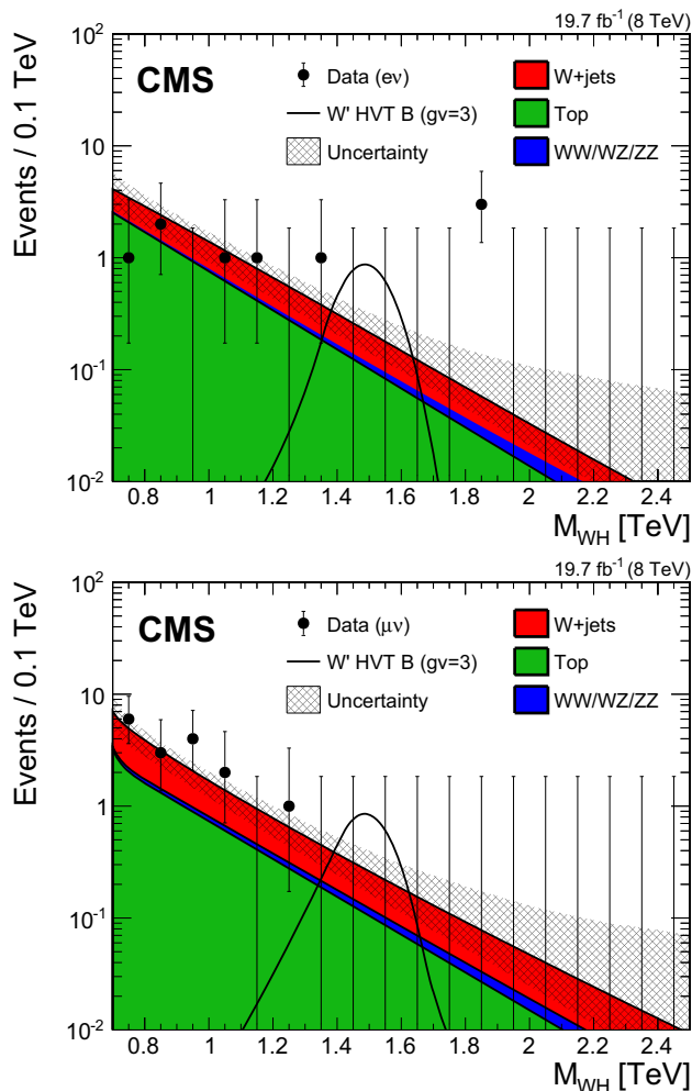
Fig. 4 Final distributions in M_{WH} for data and expected backgrounds for electron (top) and muon (bottom) categories. The 68 % error bars for Poisson event counts are obtained from the Neyman construction [77]. The hatched region indicates the statistical uncertainty of the fit combined with the systematical uncertainty in the shape. This figure also shows a hypothetical W' signal with mass of 1.5 TeV, normalized to the cross section predicted by the HVT model B with parameter gv = 3 as described in Sect. 8.2
