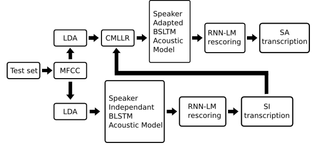
Figure 1: Decoding pipeline
