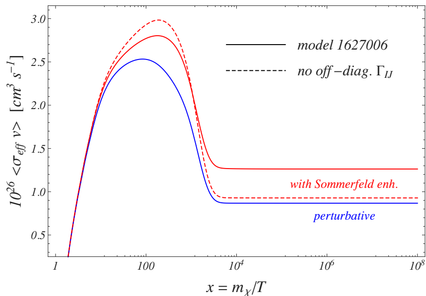
Figure 5. The thermally averaged effective annihilation rate \langle\sigma_{\text{eff}}v\rangle as a function of the scaled inverse temperature x = m_{\chi_1^0}/T for the pMSSM Snowmass model 1627006 with higgsino-like \chi_1^0 . The upper two (red) curves refer to the Sommerfeld-enhanced cross sections: the solid line includes the off-diagonal annihilation rates while the dashed curve does not. The lowermost (blue) curve corresponds to the perturbative result.
