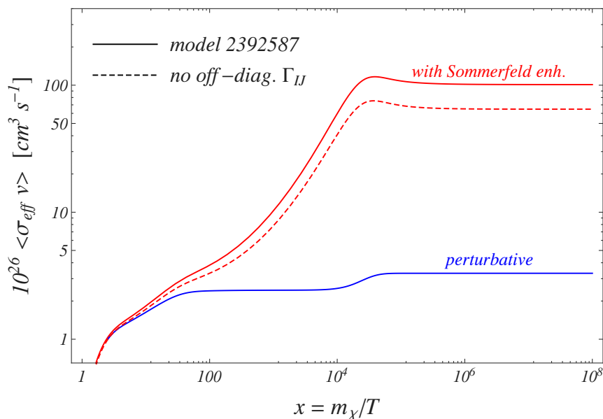
Figure 2. The thermally averaged effective annihilation rate \langle\sigma_{\text{eff}}v\rangle as a function of the scaled inverse temperature x = m_{\chi_1^0}/T in case of Snowmass model 2392587. The two upper (red) curves correspond to the Sommerfeld-enhanced annihilation cross sections including (solid line) or neglecting (dashed line) the off-diagonals in the annihilation matrices. The lower (blue) curve represents \langle\sigma_{\text{eff}}v\rangle obtained from perturbative (tree-level) cross sections.
