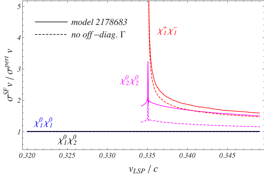
Figure 7. (\sigma^{\text{SF}} v)/(\sigma^{\text{pert}} v) for the neutral-sector states in the light scenario (Snowmass model 2178683). Solid (dashed) curves show the enhancement for the case of properly included (wrongly neglected) off-diagonal annihilation rates.
