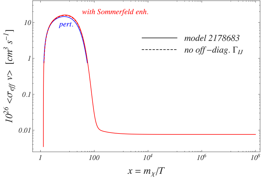
Figure 8. The thermally averaged effective rate \langle \sigma_{\text{eff}} v \rangle(x) within the pMSSM Snowmass model 2178683 with Sommerfeld enhancements (upper red curve) and in the perturbative computation (lower blue curve). The result from disregarding off-diagonal rates in the Sommerfeld-enhanced processes is plotted by the dashed line. However the latter curve basically overlays with the upper (red) curve in this plot. This is because the Sommerfeld-enhanced \langle \sigma_{\text{eff}} v \rangle(x) is dominated by the \chi_2^0 \chi_2^0 and \chi_1^+ \chi_1^- rates (before \chi_2^0 and \chi_1^\pm decoupling), and the effect of disregarding off-diagonals in the latter gives a correction of around 10% only, see figure 7.
