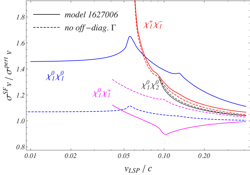
Figure 4. Enhancement factors (\sigma^{\text{SF}} v)/(\sigma^{\text{pert}} v) in the four most relevant two-particle channels \chi_1^0 \chi_1^0 , \chi_1^+ \chi_1^- , \chi_1^0 \chi_2^0 and \chi_1^0 \chi_1^+ of Snowmass model 1627006. The enhancement factor for the additionally relevant channel \chi_1^0 \chi_1^- agrees with the one for the \chi_1^0 \chi_1^+ pair. Solid lines refer to the calculation of the Sommerfeld-enhanced rates with off-diagonal terms in the annihilation matrices properly included. Dashed curves show the enhancement when the off-diagonal annihilation rates are neglected.
