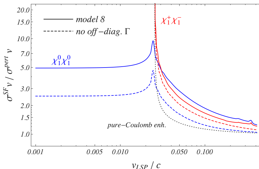
Figure 12. Enhancements (\sigma^{\text{SF}}v)/(\sigma^{\text{pert}}v) in the two neutral channels \chi_1^0\chi_1^0 and \chi_1^+\chi_1^- of model 8 of the wino-to-higgsino trajectory discussed in section 5. Solid (dashed) curves refer to the results with (without) off-diagonal annihilation rates included.
