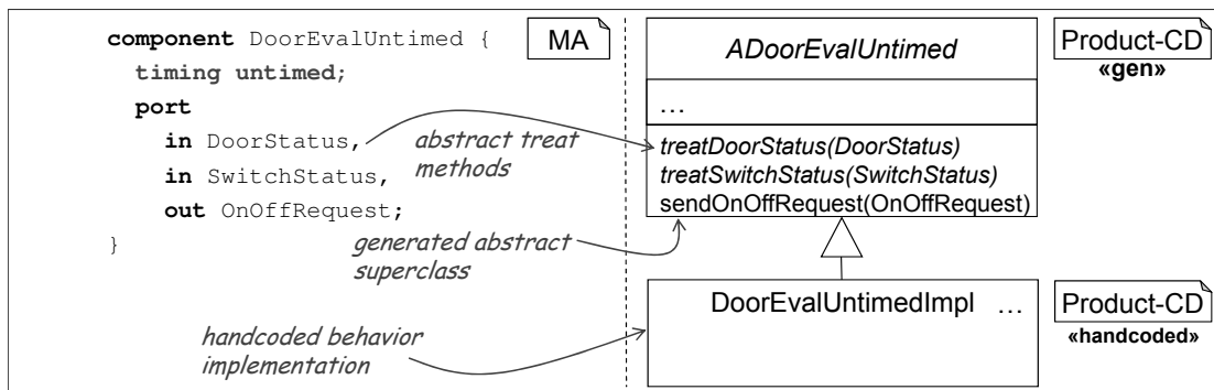
Figure 5.41: Atomic component DoorEvalUntimed , the corresponding generated superclass, and the implementation.
