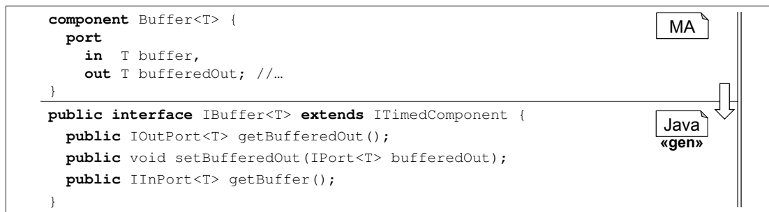
Figure 5.28: Generated interface for a generic component.
