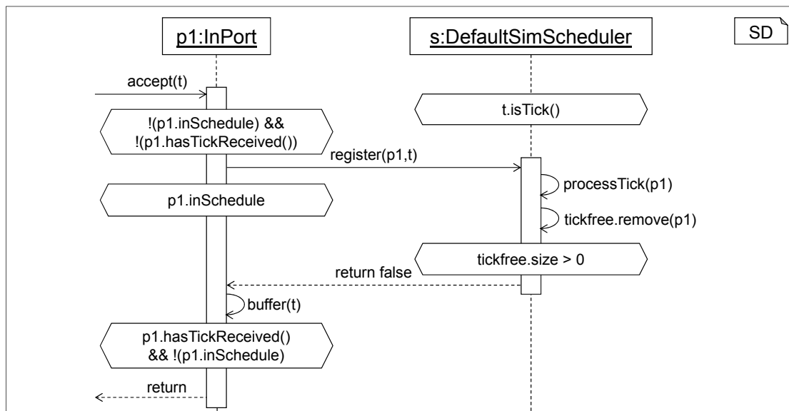
Figure 4.16: Scheduling of any \surd messages.
