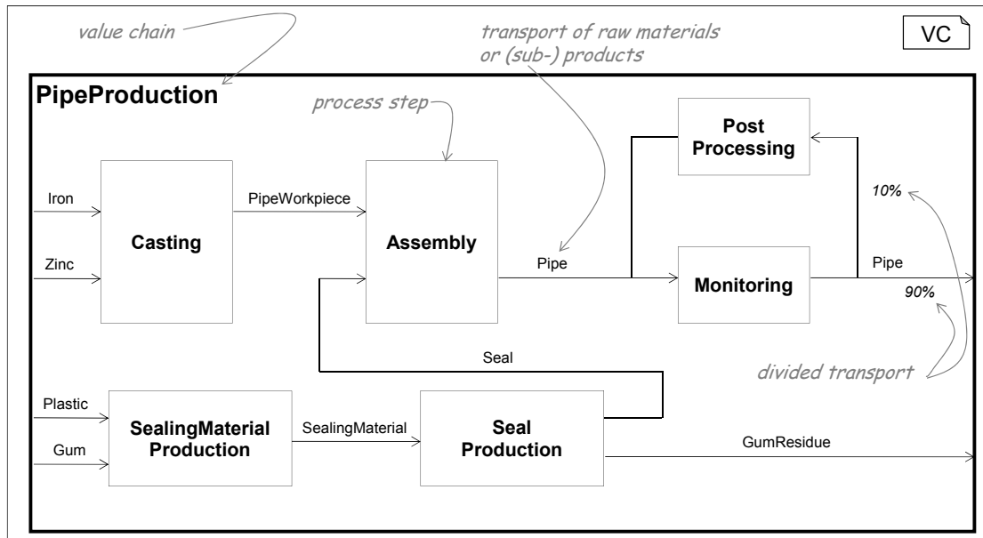
Figure 9.8: Exemplary value chain that models the dependencies between different process steps to manufacture pipes.
