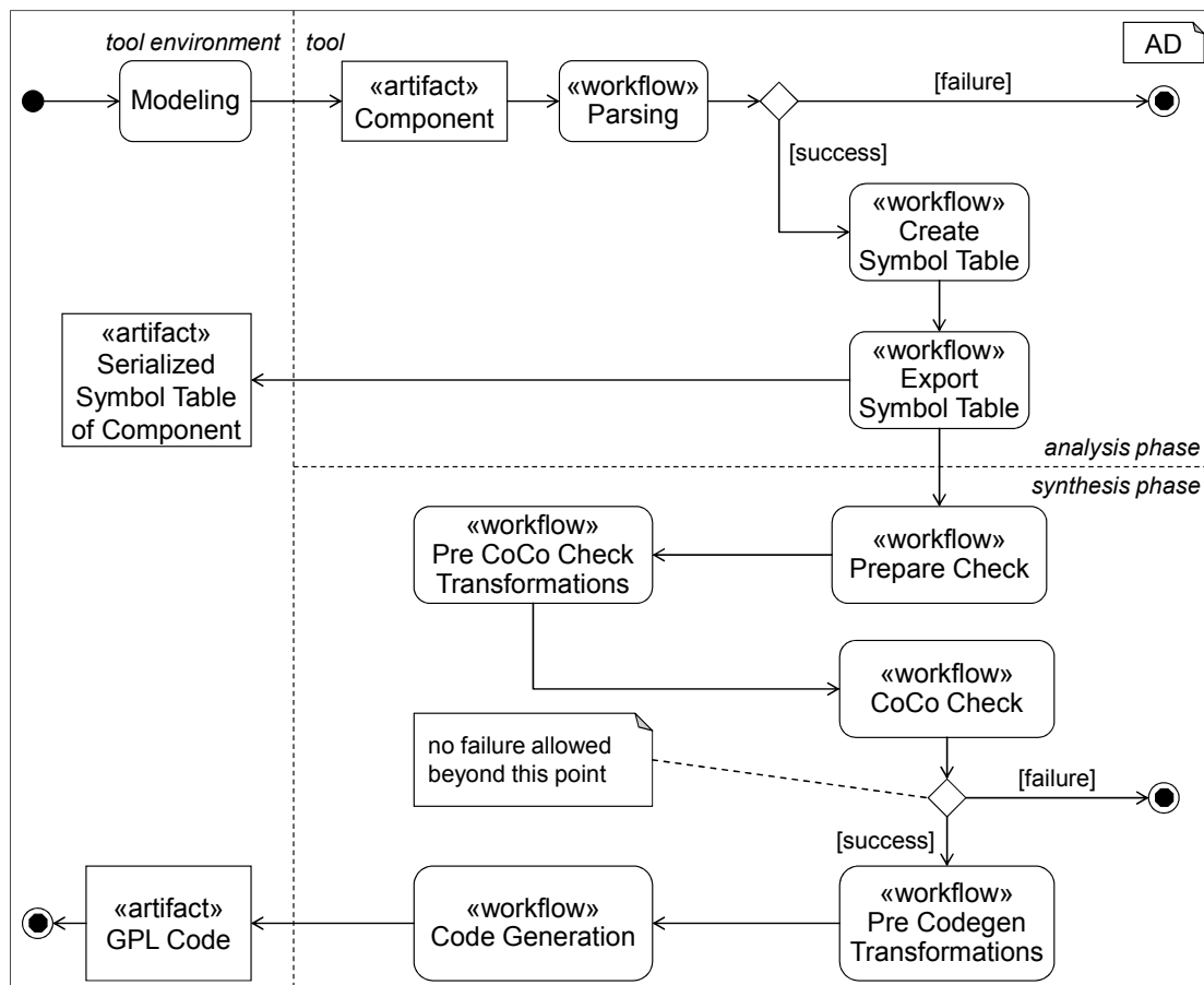
Figure 5.4: Overview of MontiArc workflows and produced artifacts.
