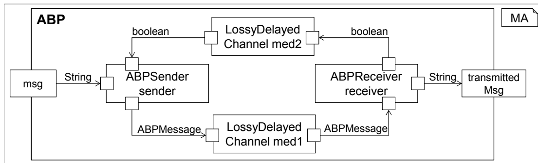
Figure 6.3: Alternating Bit Protocol component model.
