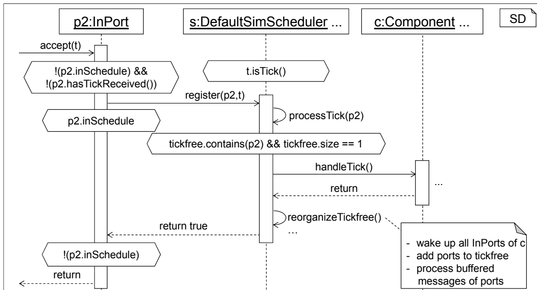
Figure 4.17: Scheduling the final \surd message.
