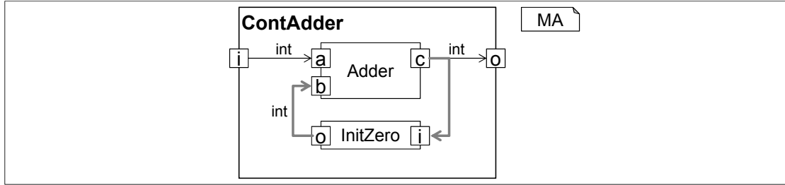
Figure 3.55: CG1: Communication cycle between subcomponents.
