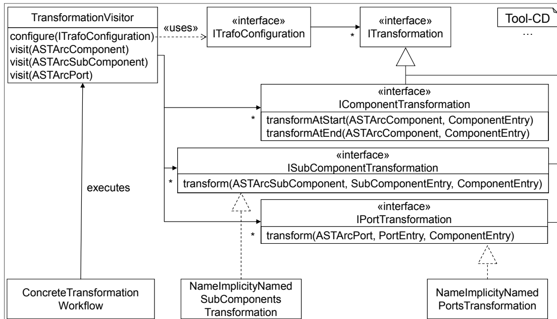
Figure 5.24: Important classes of MontiArc’s transformation framework.
