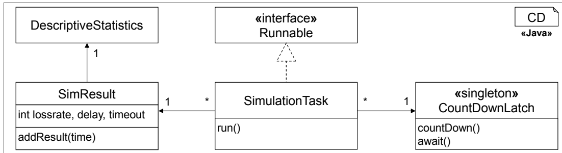
Figure 6.36: Involved classes of a parallelized optimization test.
