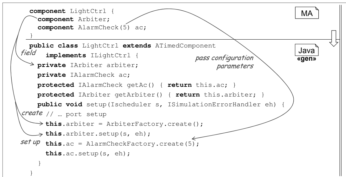
Figure 5.37: Code generation for subcomponents.
