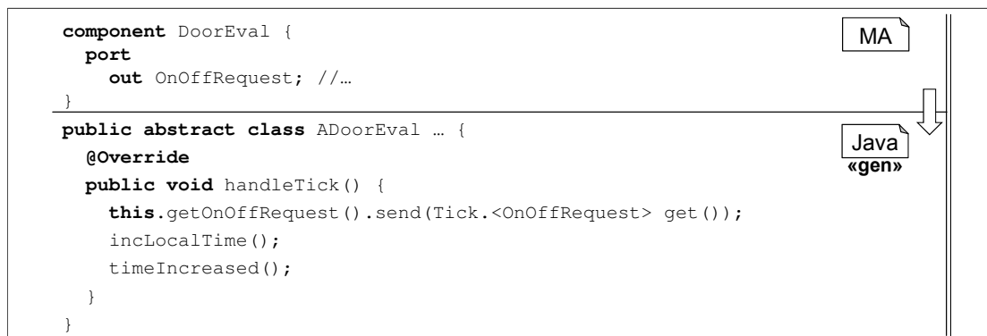
Figure 5.35: Generated method handleTick() that emits ticks at the end of a time interval.
