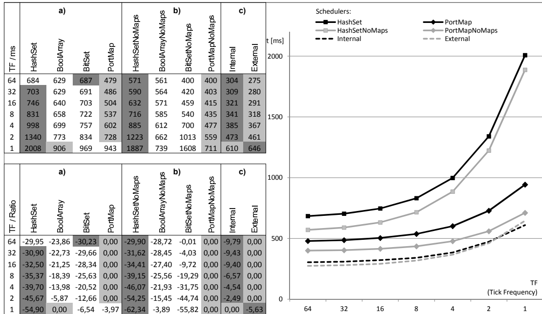
Figure 4.30: Scheduler comparison results of the average execution time in milliseconds for component LoadTest_2.50. The tick frequency of the distinct scenarios is ranging from 64 to one.
