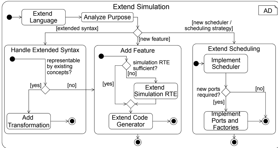
Figure 7.6: Activities to extend the simulation of MontiArc models.
