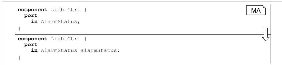
Figure 5.19: Pre Codegeneration Trafo: Name Implicitly Named Ports.
