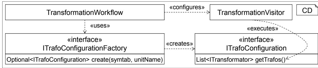
Figure 7.5: Interfaces used as extension points to add further transformations to MontiArc.
