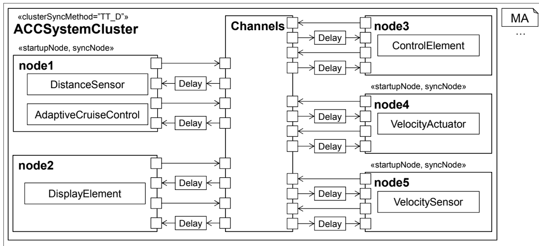
Figure 8.7: Exemplary FlexRay cluster with five nodes which host the components of the cruise control system (adapted from [Rab13]).
