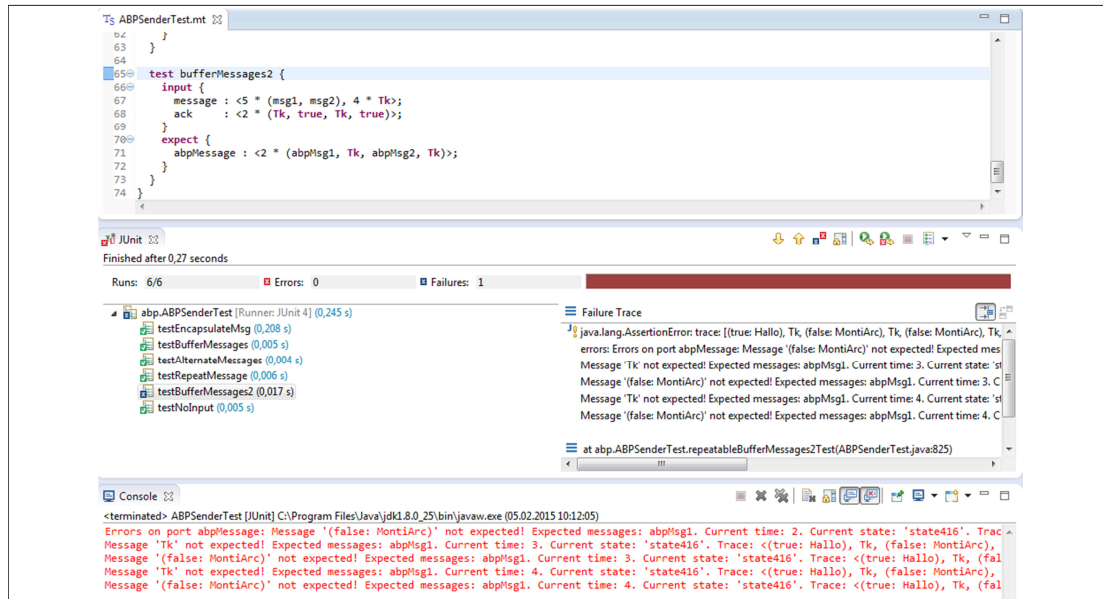
Figure 6.25: Screenshot of executed I/O-Tests with the failing test testBufferMessages2 .
