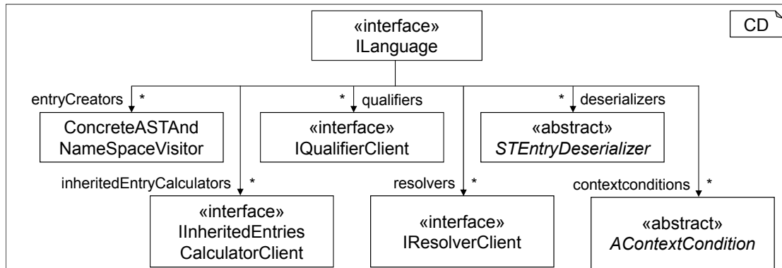
Figure 5.6: Most important technical symbol table components (according to [Völ11]).
