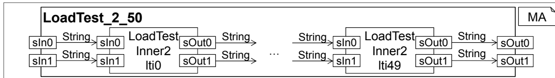
Figure 4.28: Component LoadTest_2_50 used to compare the discussed scheduler variants in a setup with many subcomponents with few ports.
