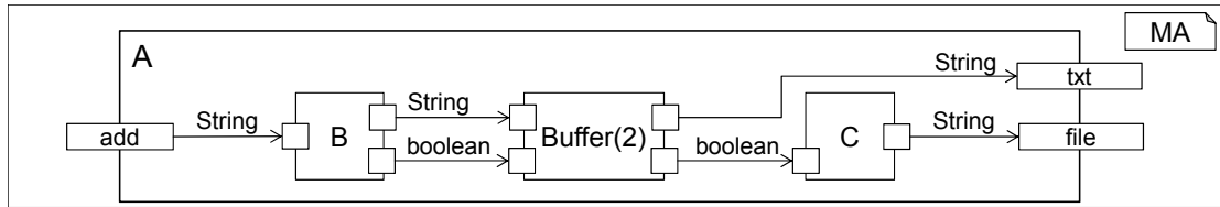
Figure 5.49: Exemplary dirty components.
