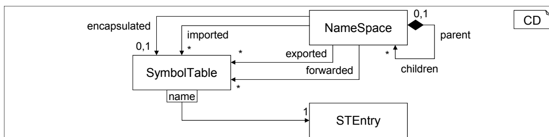
Figure 5.5: Relation of namespaces, symbol tables, and entries (according to [Völ11]).
