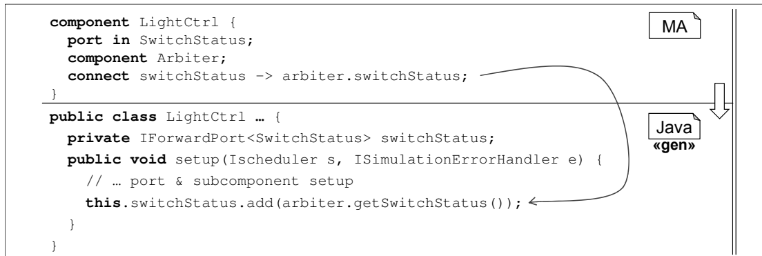
Figure 5.38: Generated code for connectors from incoming ports of decomposed components to incoming ports of subcomponents.
