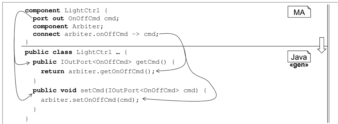
Figure 5.40: Generated code for connectors which connect outgoing ports of subcomponents with outgoing ports of decomposed components.
