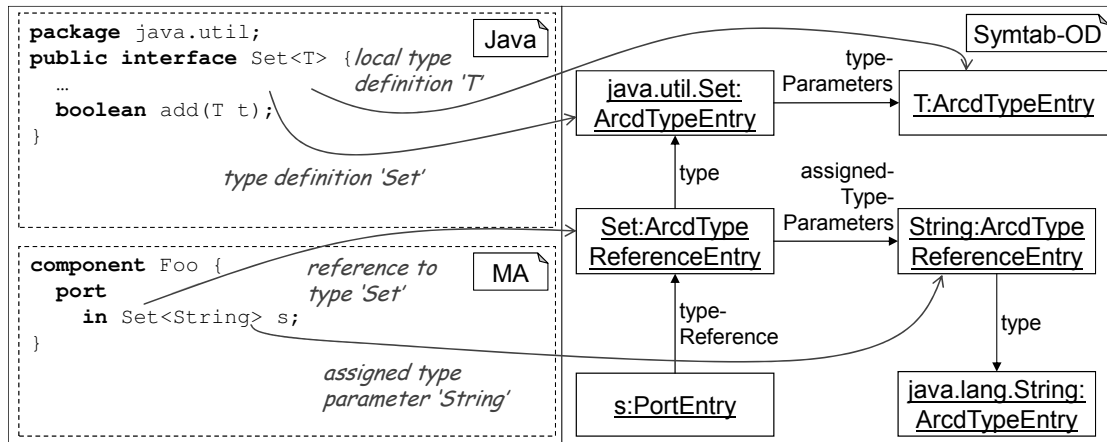
Figure 5.10: Relation between type definition and type reference manifested in the MontiArc symbol table.
