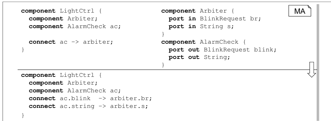
Figure 5.15: Pre CoCo Trafo: Qualify Subcomponent Connectors.
