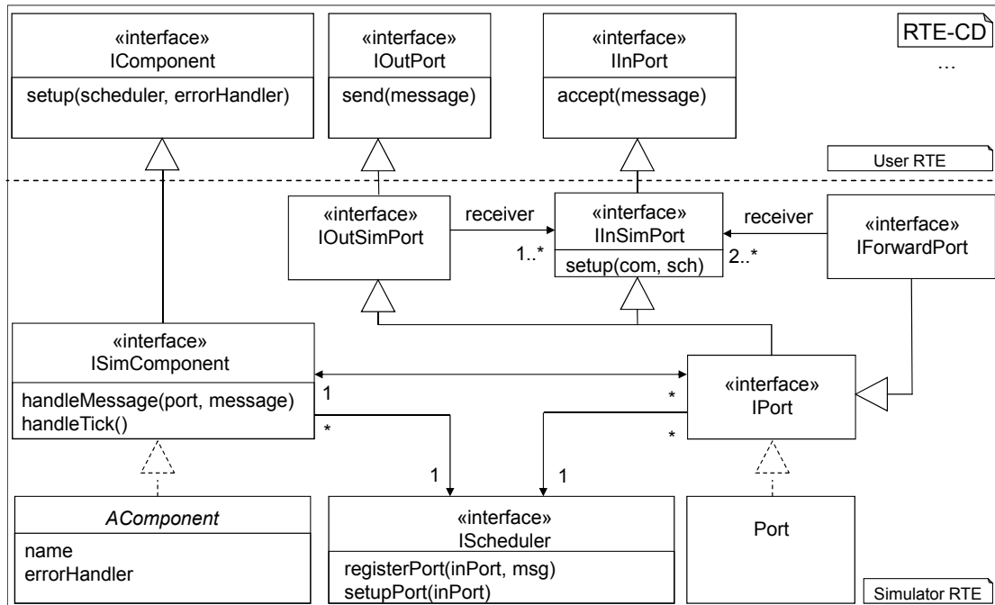
Figure 4.10: MontiArc's RTE. The User RTE parts are used when setting up a simulation or atomic components are implemented. Parts of the Simulator RTE are used by the scheduler and the generated simulation code (see Section 5.4).
