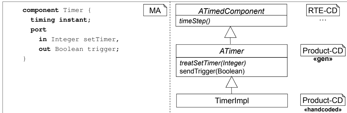
Figure 5.45: Timed component Timer , the corresponding generated superclass, and the handwritten implementation.
