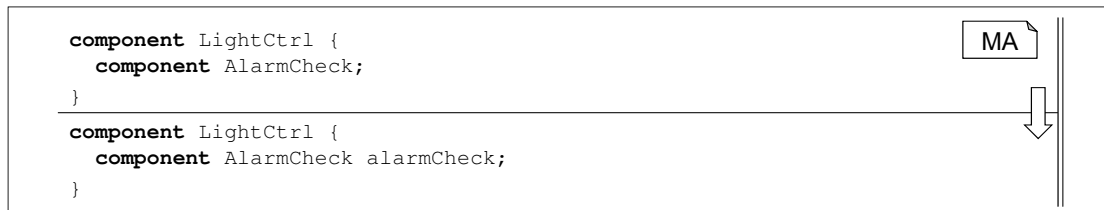
Figure 5.18: Pre Codegeneration Trafo: Name Implicitly Named Subcomponents.
