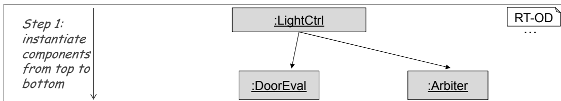
Figure 4.4: Instantiation of components as simulation objects. Step 1: instantiate components from top to bottom.
