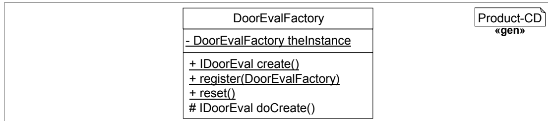
Figure 5.47: Generated factory for component DoorEval .
