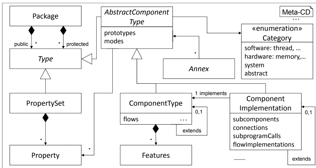
Figure D.1: Extract of the AADL metamodel (adapted from [FGH06, FG12]).
