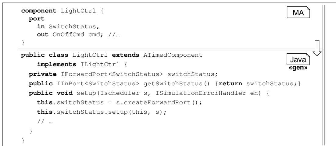
Figure 5.36: Incoming ports of decomposed components.
