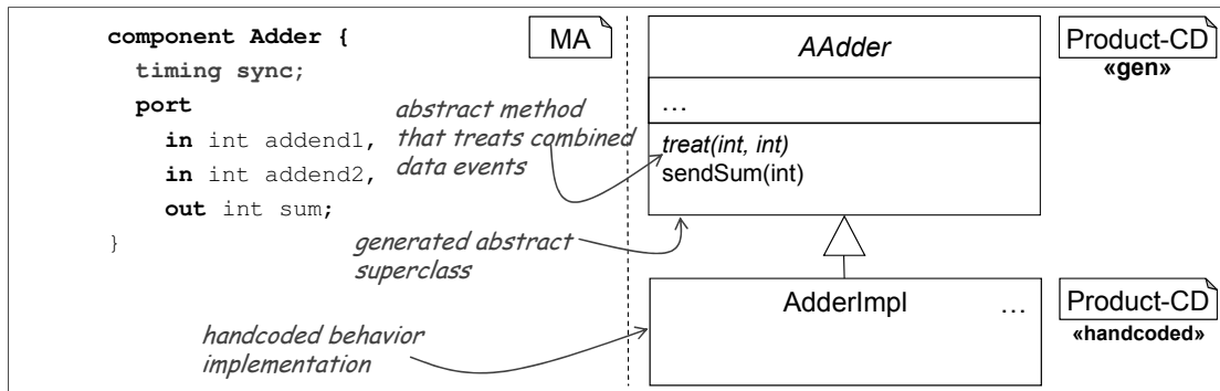
Figure 5.43: Synchronous atomic component Adder , the corresponding generated superclass, and the handwritten implementation.
