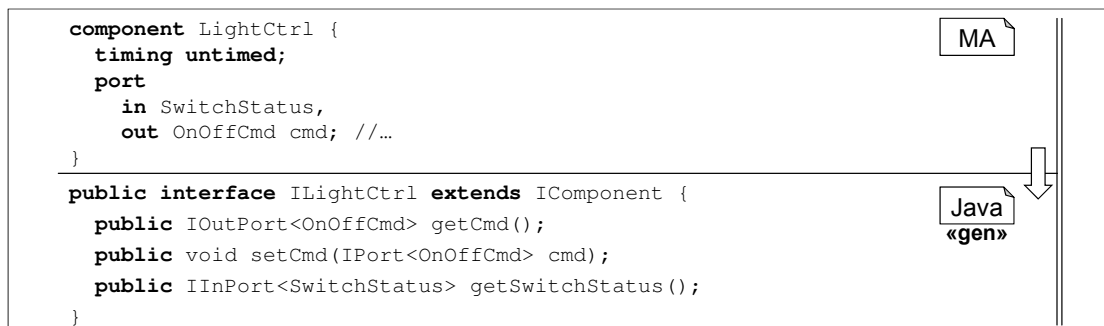
Figure 5.27: Generated interface for an untimed component.
