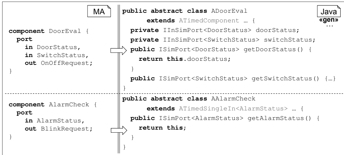
Figure 5.52: Optimization: Difference between the generated code for single-in and regular atomic components.
