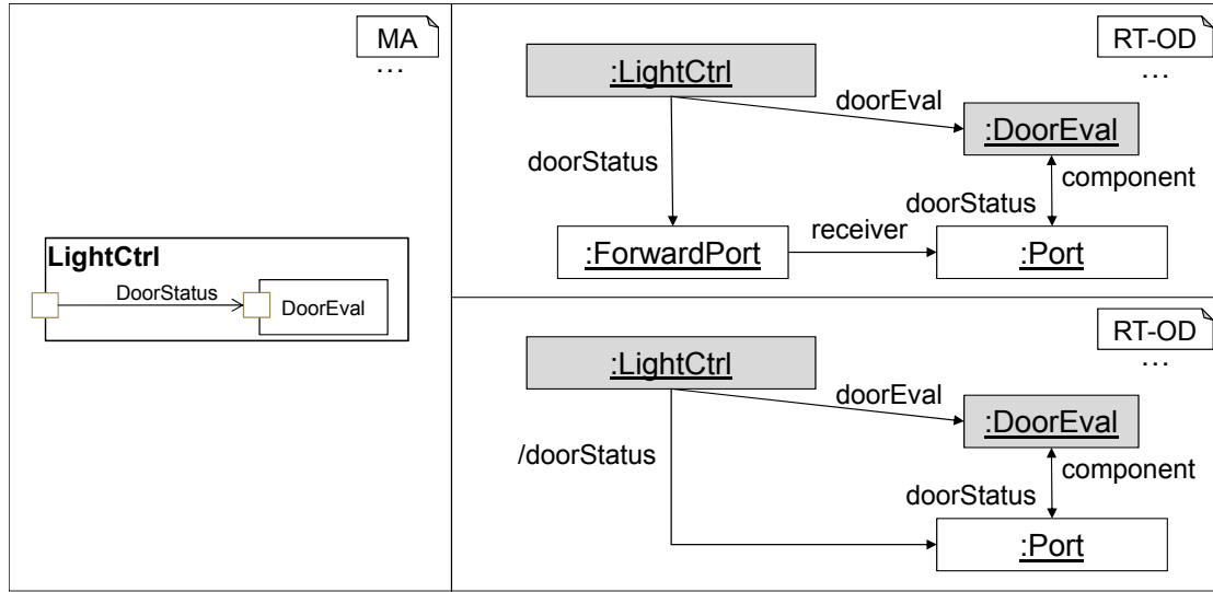
Figure 5.53: Optimization: Avoiding not needed ForwardPorts in decomposed components.
