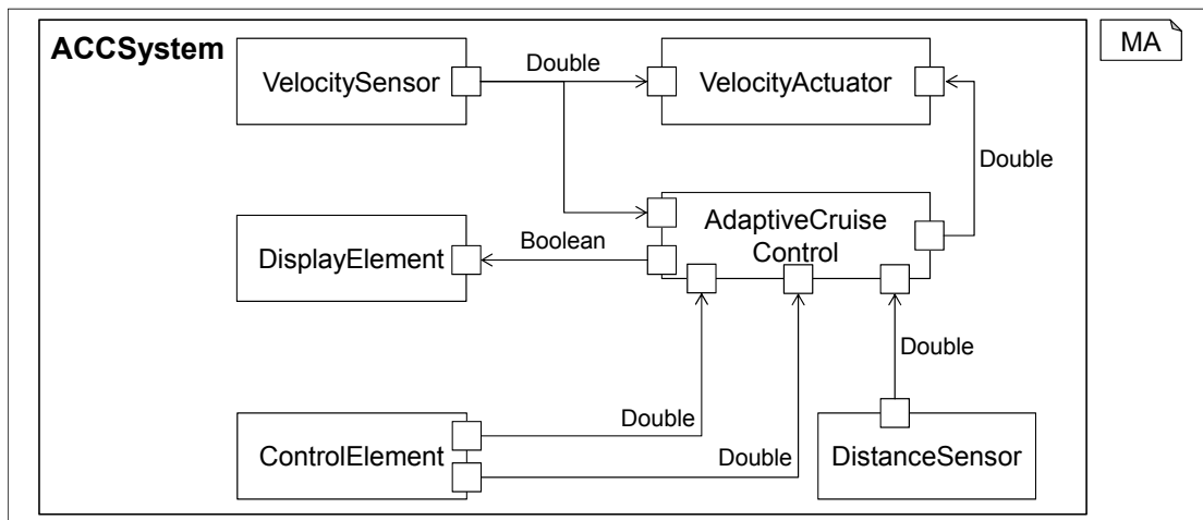
Figure 8.6: Running example of an adaptive cruise control system (adapted from [Rab13]).
