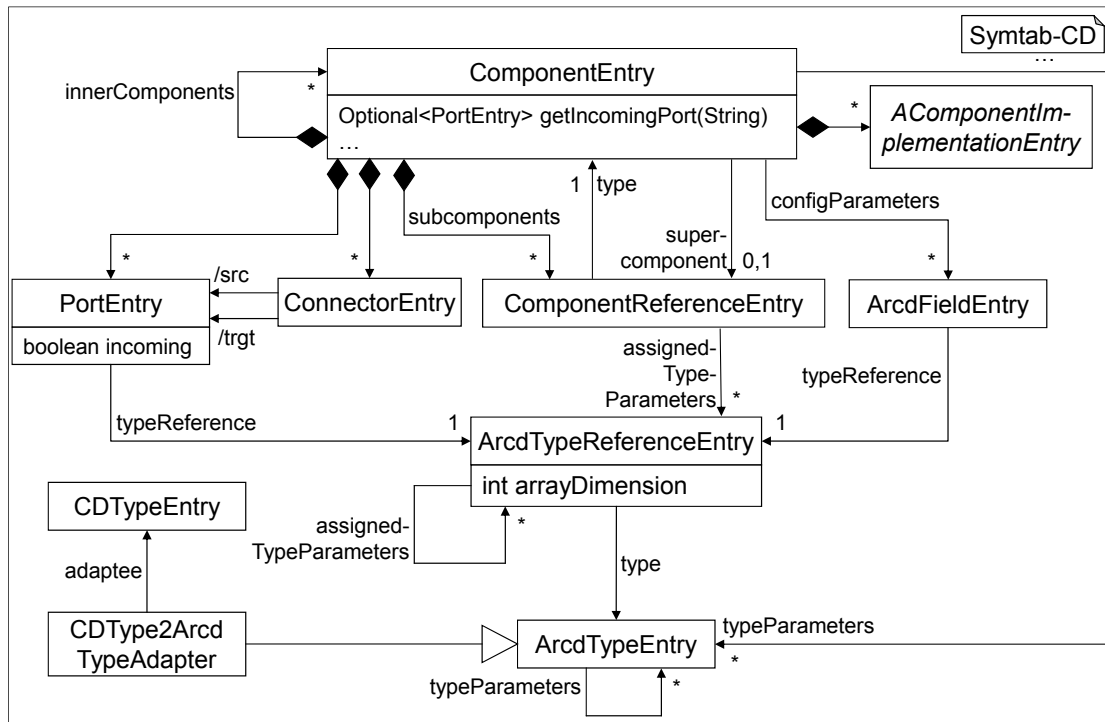
Figure 5.8: Entry classes of the MontiArc symbol table and their relations.
