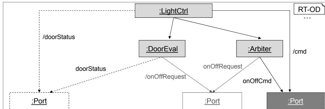
Figure 4.8: Instantiation of components as simulation objects. Optimized object structure.
