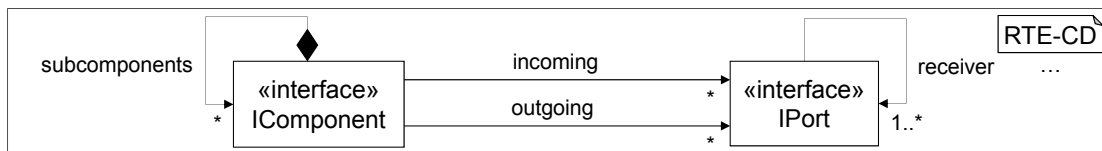
Figure 4.9: Components and Ports in MontiArc's RTE.
