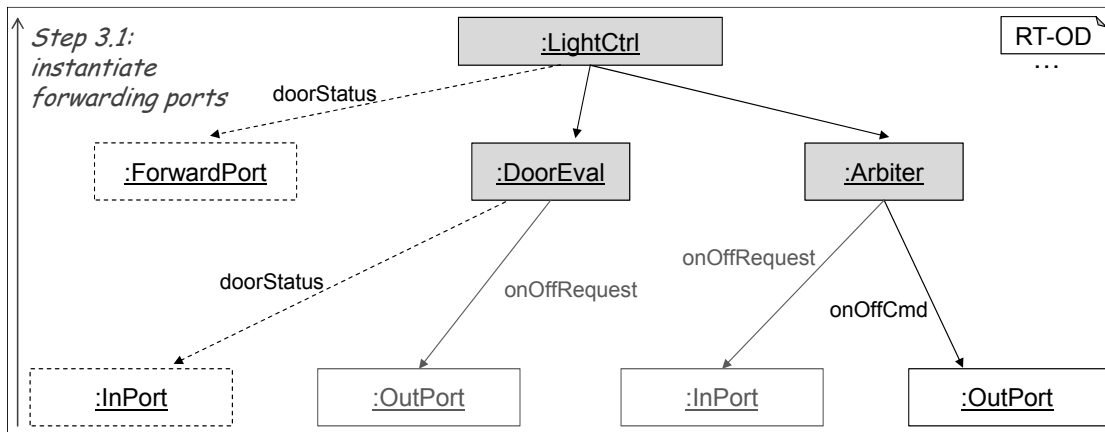
Figure 4.6: Instantiation of components as simulation objects. Step 3.1: instantiate forwarding ports.
