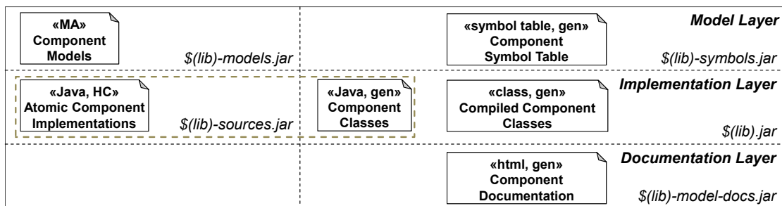
Figure 6.42: Layers of a component library.
