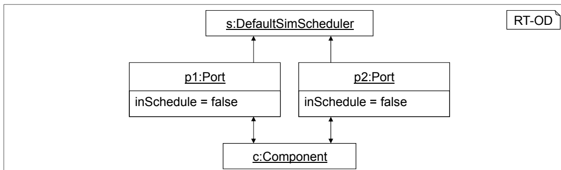
Figure 4.13: Scheduled component c and the state of its ports.
