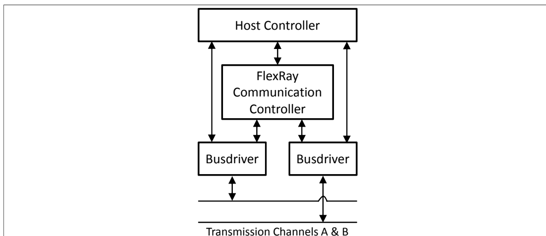
Figure 8.4: Overview of a FlexRay node (adapted from [Hei12]).
