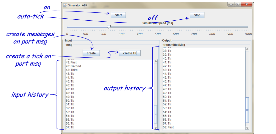
Figure 6.15: Interactive ABP simulation.
