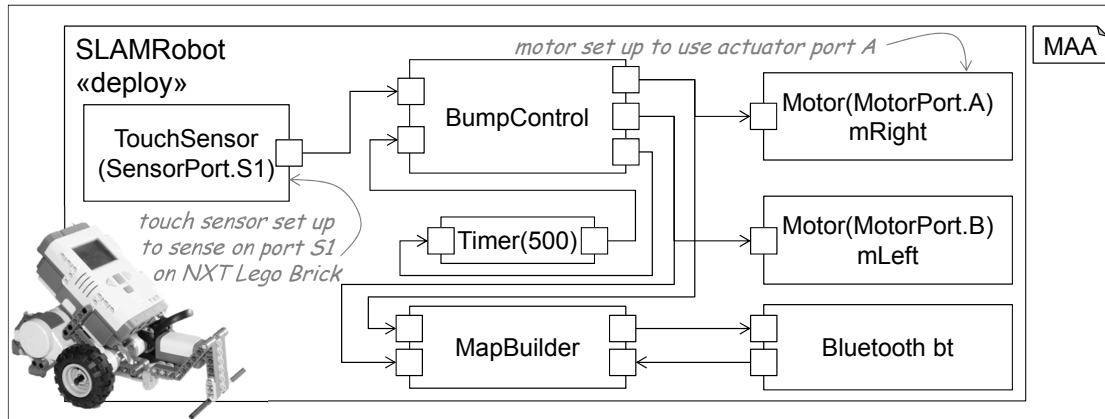
Figure 9.5: A SLAMRobot constructed with an NXT Lego Brick. The architecture and the behavior of SLAMRobots is modeled with MontiArcAutomaton (according to [RRW13b]).
