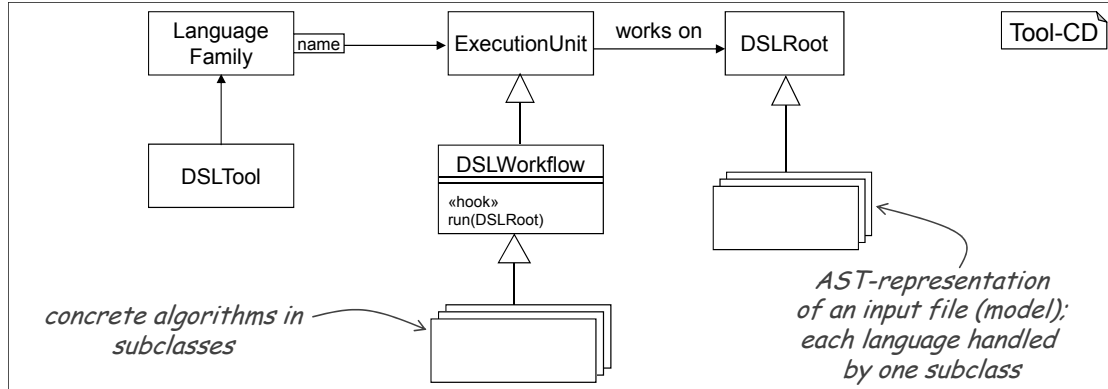
Figure 5.1: Important classes of the MontiCore DSLTool-Framework according to [Kra10].
