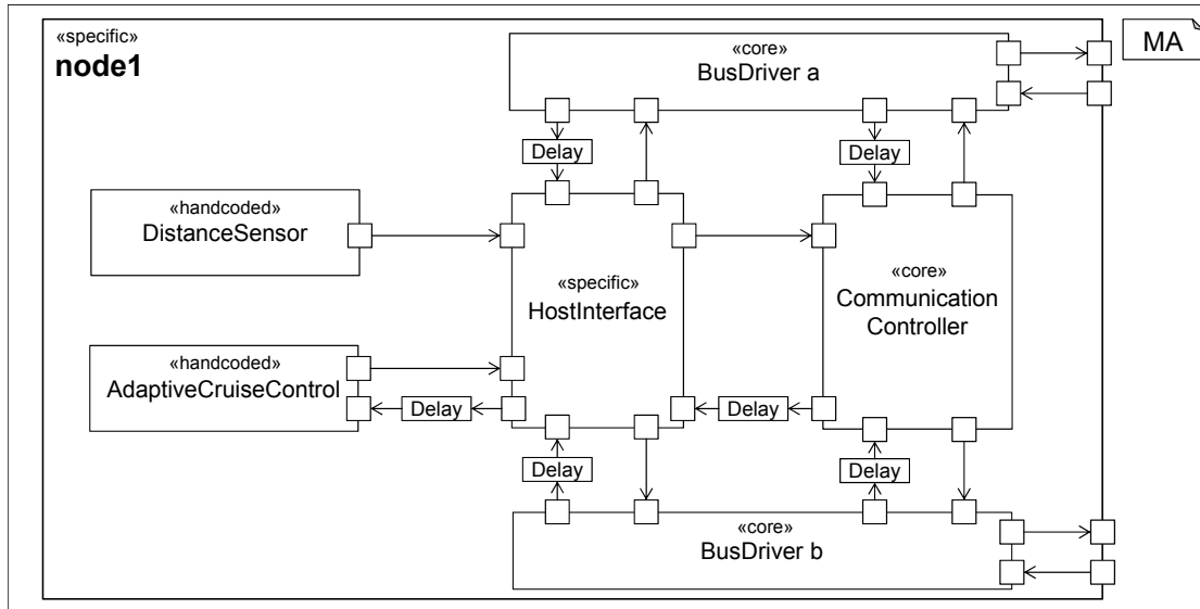
Figure 8.8: Detailed architecture of a FlexRay node component (adapted from [Rab13]).
