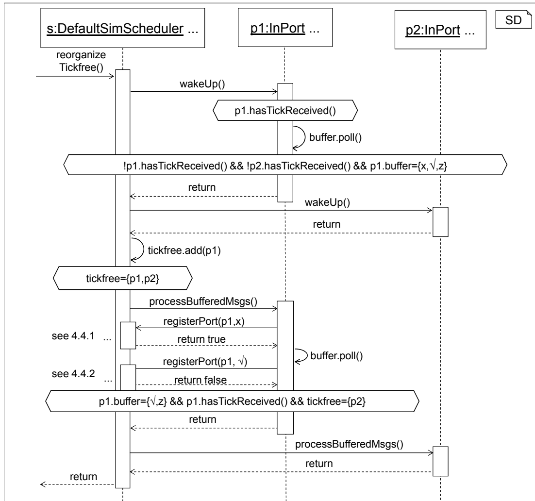
Figure 4.20: Reorganization and waking up of ports.
