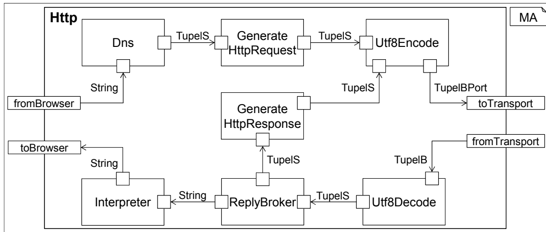
Figure 8.2: Architecture of the HTTP protocol in MontiArc (adapted from [Sch13]).
