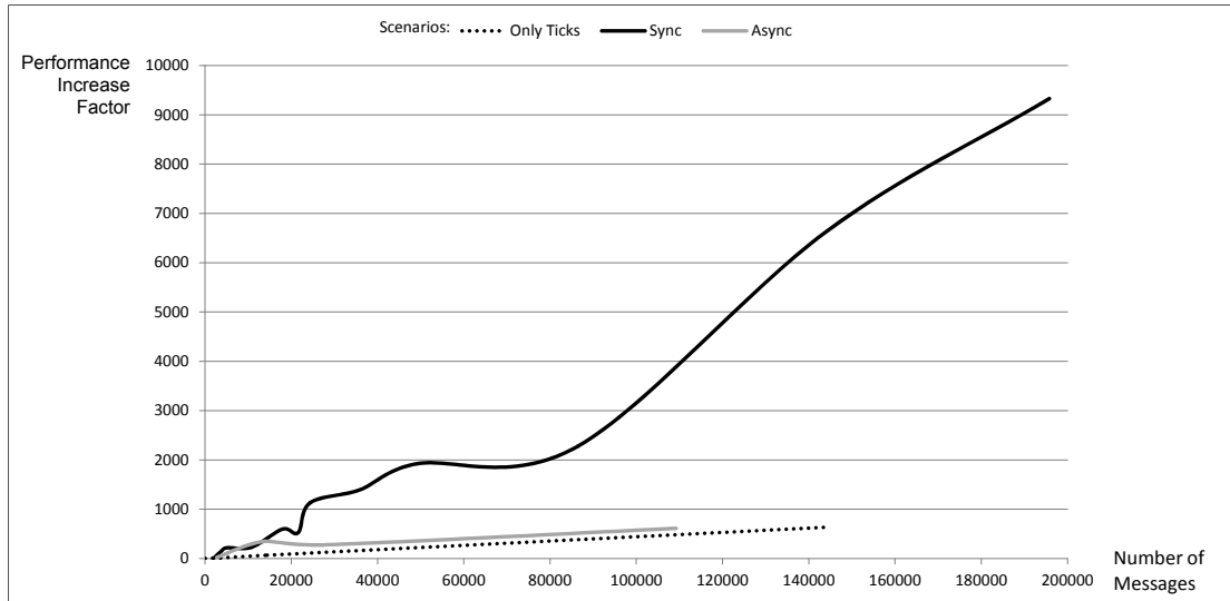
Figure 4.27: Comparison results: Round robin vs. MontiArc scheduler. The Performance Increase Factor is the quotient of the average execution time of the RRS and the average execution time of the MontiArc scheduler. Number of Messages = Number of ticks + Number of data messages.
