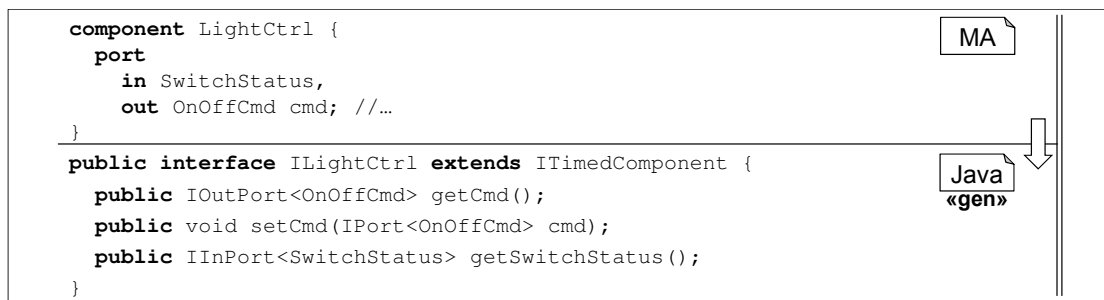
Figure 5.26: Generated interface for a timed component.
