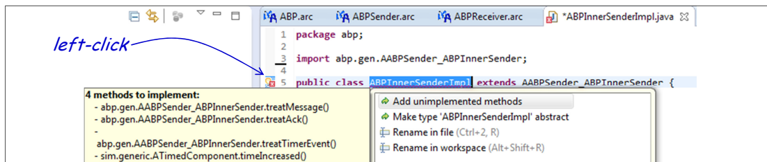
Figure 6.14: Quick fix to add missing event methods.
