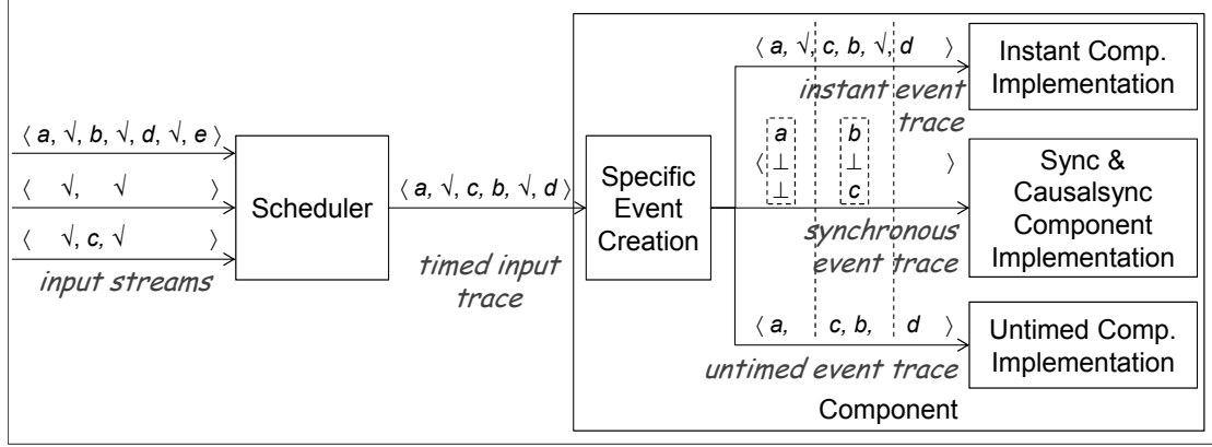
Figure 4.21: Creation of timing domain specific event traces from timed input streams.
