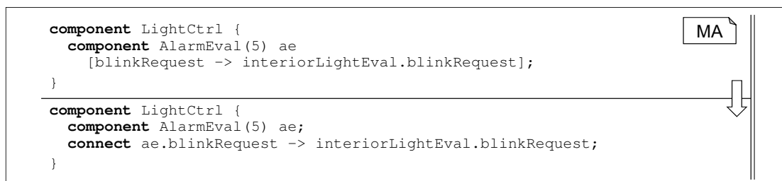
Figure 5.20: Pre Codegeneration Trafo: Expand Simple Connectors.
