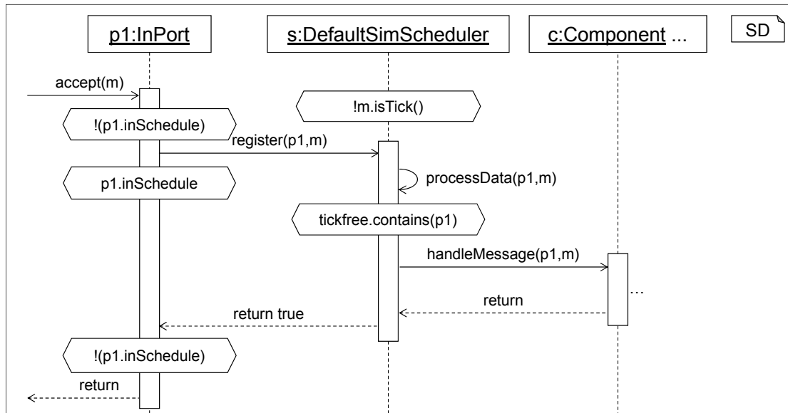
Figure 4.14: Scheduling data messages on a tickfree port.
