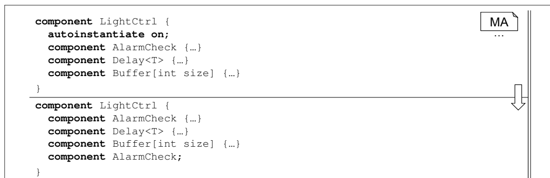
Figure 5.17: Pre CoCo Trafo: Expand Autoinstantiate.
