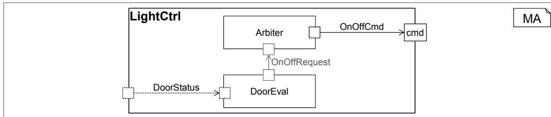
Figure 4.3: Excerpt of component LightCtrl.
