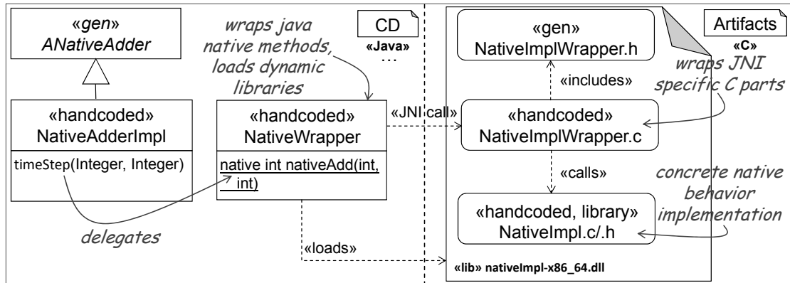
Figure 6.18: Pattern to integrate existing C code into atomic MontiArc components.
