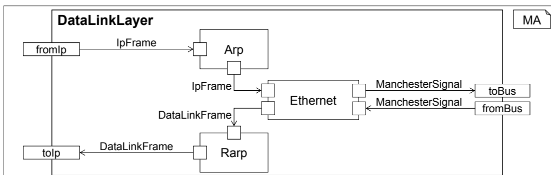
Figure 8.3: The data link layer that is realized using a combination of Arp , Rarp , and the ethernet protocol (adapted from [Sch13]).
