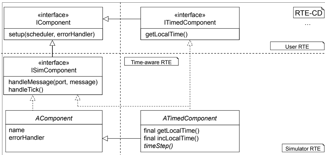
Figure 4.11: Components and Timing in MontiArcs RTE.
