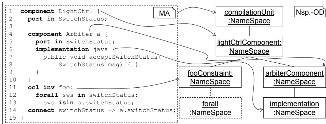
Figure 5.7: Namespace hierarchy of component LightCtrl .
