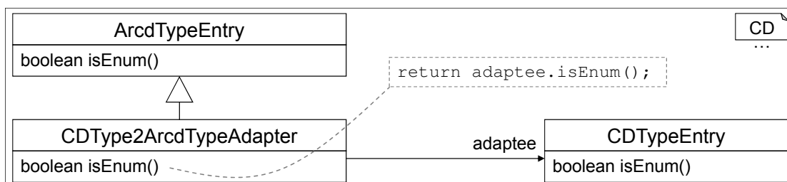
Figure 7.16: Adapter to translate CD type entries to ArcD type entries.
