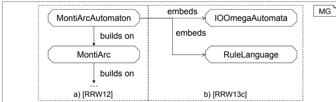
Figure 9.7: MontiCore Grammar hierarchy for a) the initial MontiArcAutomaton version that uses inheritance and b) the current MontiArcAutomaton version that uses embedding to extend MontiArc with I/O^\omega automata.
