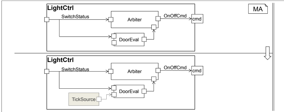
Figure 5.22: Pre Codegeneration Trafo: Connecting Unconnected Incoming Ports of Subcomponents.
