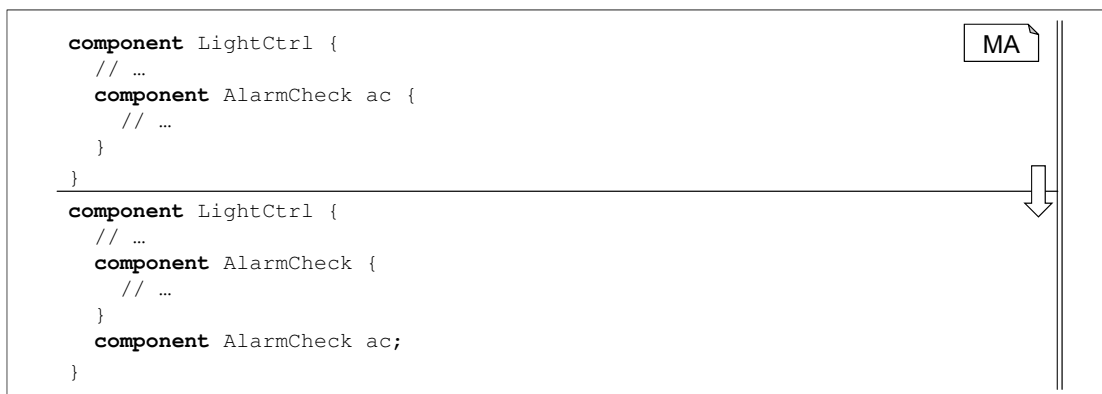
Figure 5.14: Pre CoCo Trafo: Instantiation of Named Inner Component Definitions.
