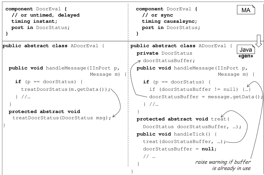
Figure 5.33: Message propagation of atomic components.
