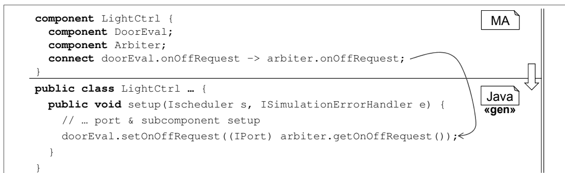
Figure 5.39: Generated code for connectors which connect two subcomponents.
