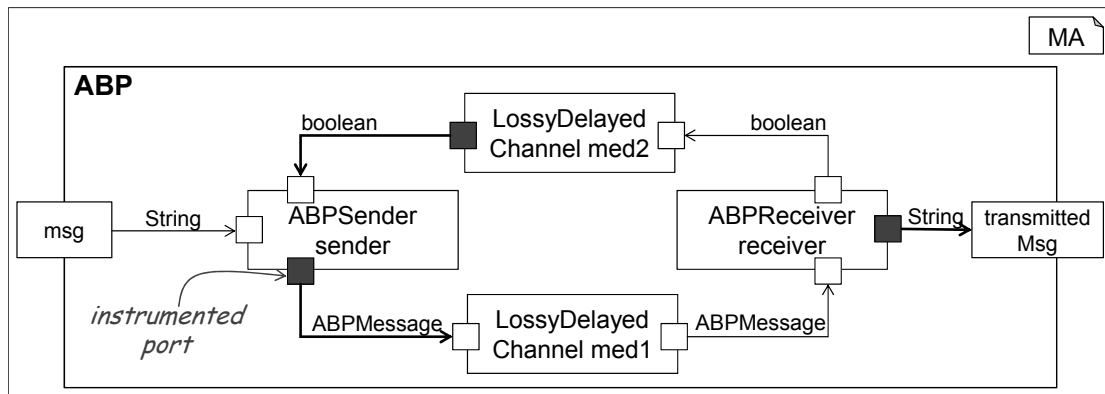
Figure E.6: Instrumented ports of ABP's subcomponents in the white-box test given in Listing E.7.
