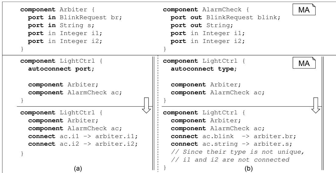
Figure 5.16: Pre CoCo Trafo: Expand autoconnect port (a) and type (b).
