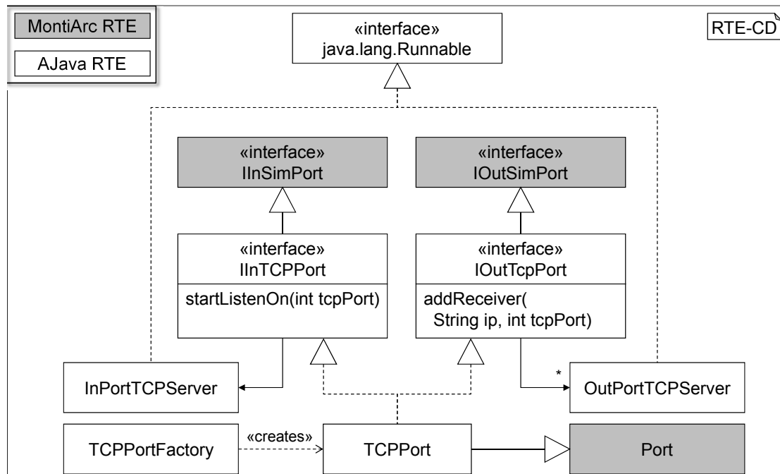
Figure 9.4: AJava RTE extensions of the MontiArc RTE.
