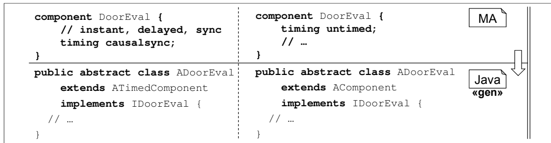
Figure 5.29: Generated abstract class for an atomic component.
