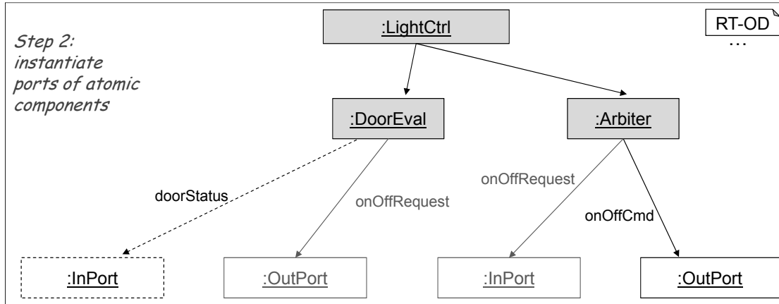
Figure 4.5: Instantiation of components as simulation objects. Step 2: instantiate ports of atomic components.
