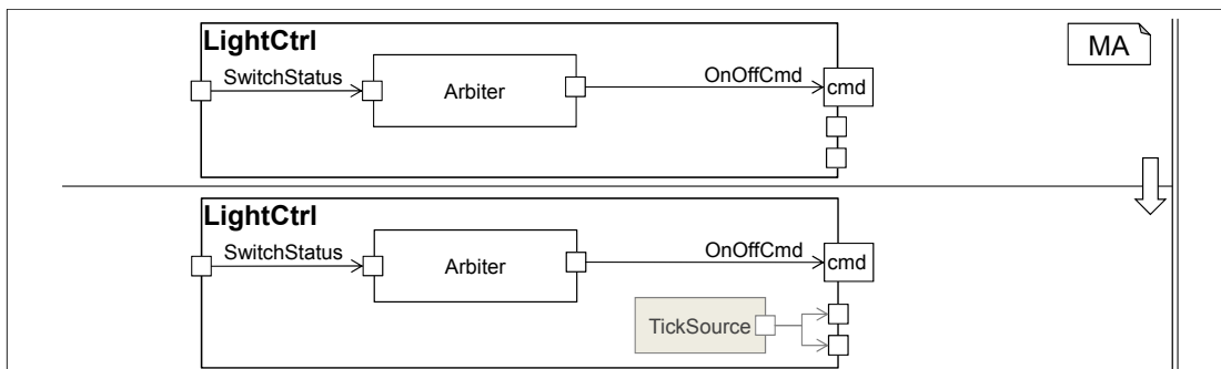
Figure 5.23: Pre Codegeneration Trafo: Connecting Unconnected Ports of Subcomponents.
