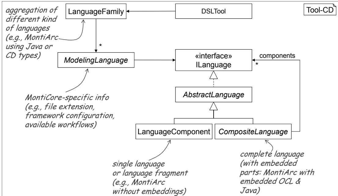
Figure 5.2: Technical realization of MontiCore's language composition mechanisms according to [Völ11, Sch12].
