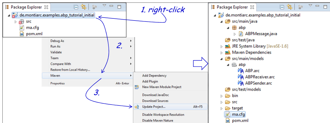
Figure 6.5: Updating a Maven project.
