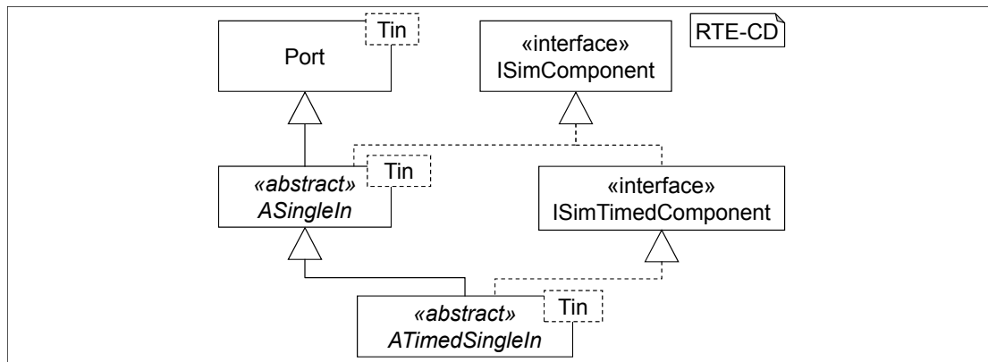
Figure 5.51: Extension of the RTE to support single-in components.
