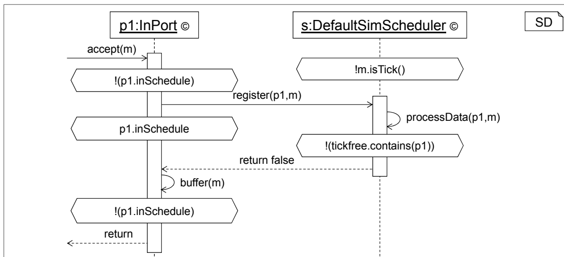
Figure 4.15: Scheduling data messages on a blocked port.
