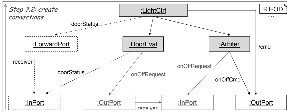
Figure 4.7: Instantiation of components as simulation objects. Step 3.2: create connections.
