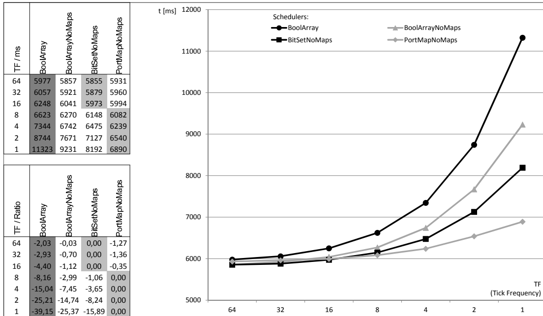
Figure 4.31: Scheduler comparison results of the average execution time in milliseconds for component LoadTest_100.8. The tick frequency of the distinct scenarios is ranging from 64 to one.
