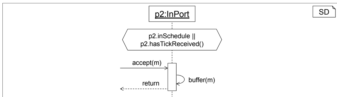
Figure 4.18: Scheduling of data or \surd messages on a port which is already involved in a scheduling process.
