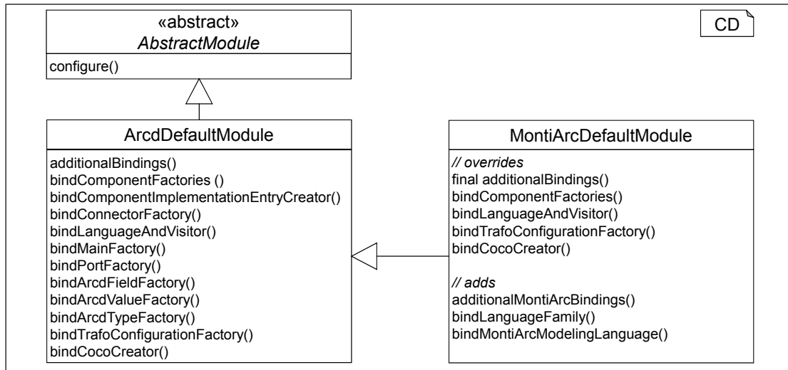
Figure 7.2: Default modules to configure dependency injection.
