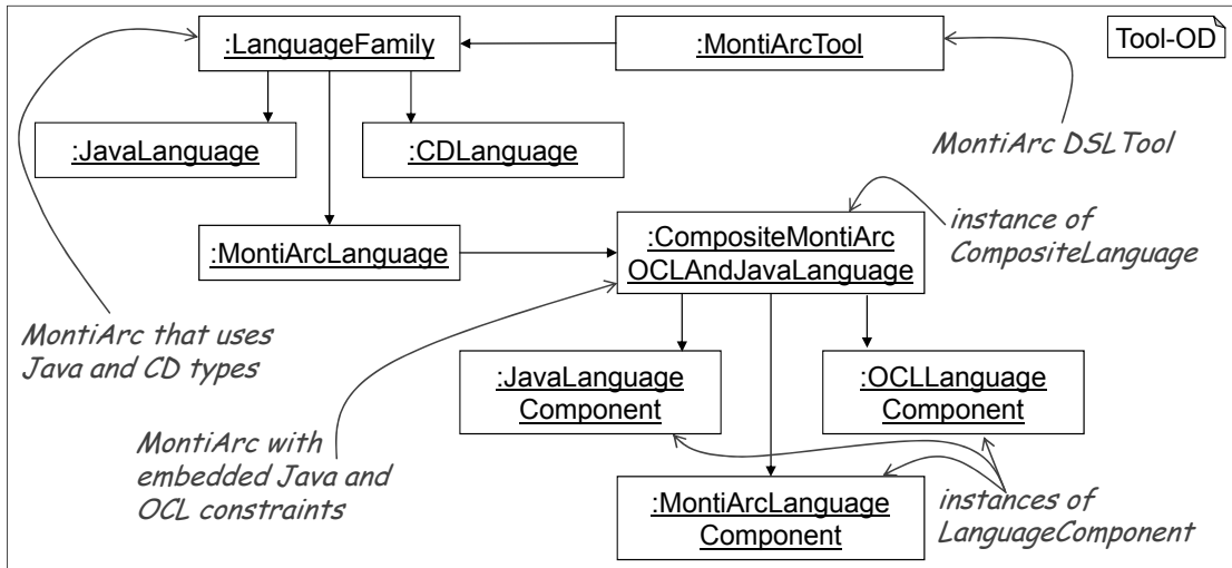
Figure 5.3: Object graph of the MontiArc DSLTool with the technical languages it uses.
