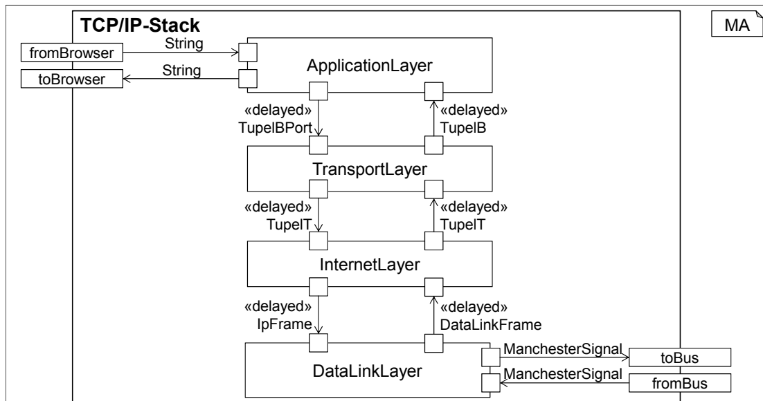
Figure 8.1: Overview of the TCP/IP stack realized in MontiArc (adapted from [Sch13]).
