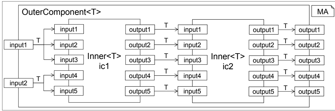
Figure 4.26: Component setup used to compare the RRS and the presented MontiArc scheduler.
