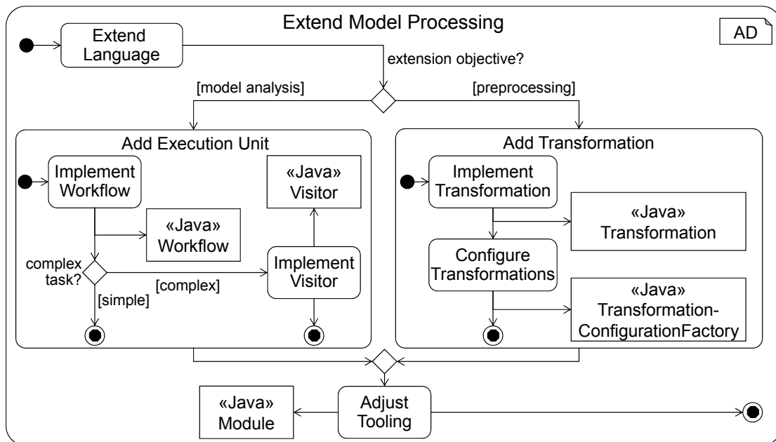
Figure 7.1: Activities to extend the processing of MontiArc models.
