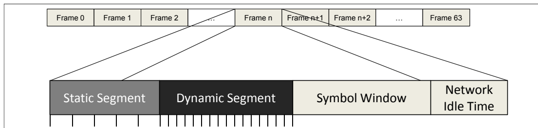
Figure 8.5: FlexRay communication cycles (adapted from [Hei12]).
