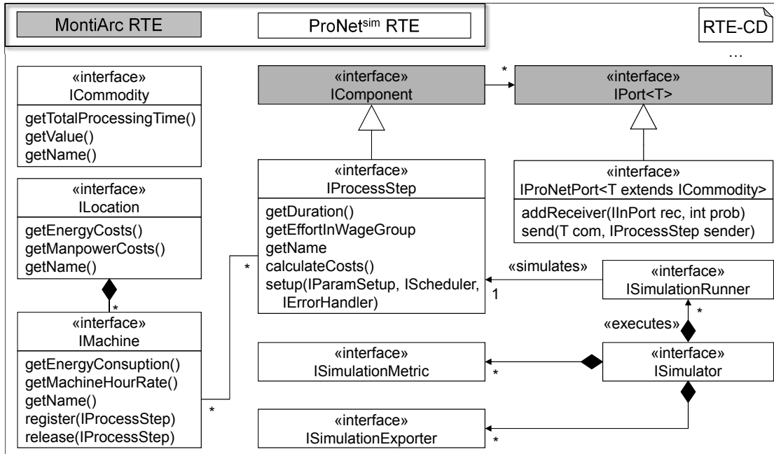
Figure 9.10: ProNet sim extensions of the MontiArc RTE.
