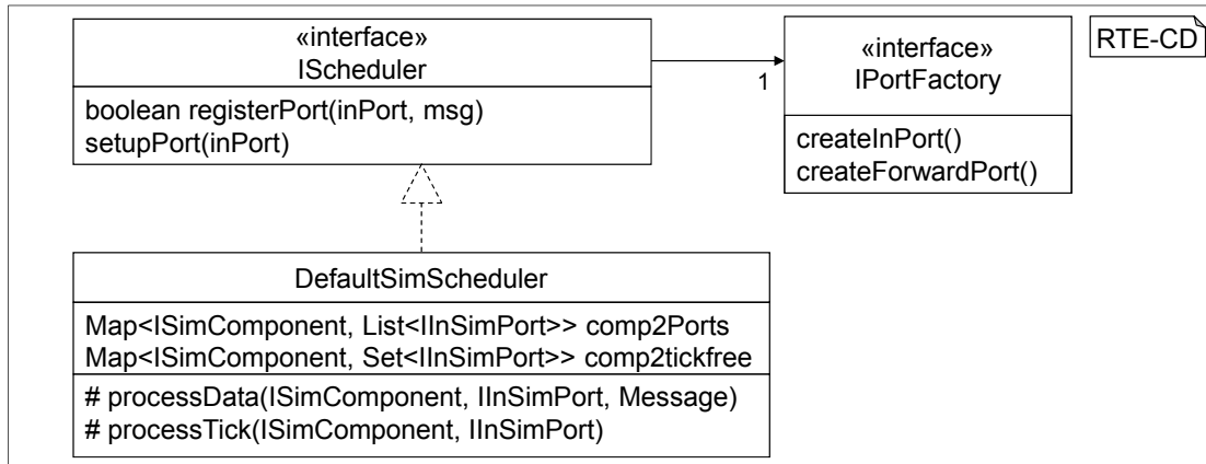
Figure 4.12: Default Simulation Scheduler.
