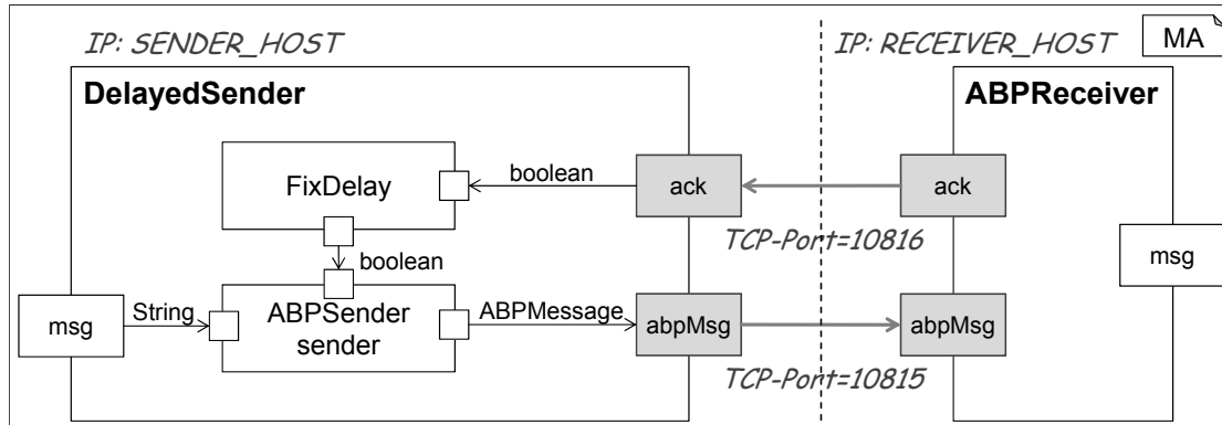
Figure 6.45: A physically distributed ABP simulation.
