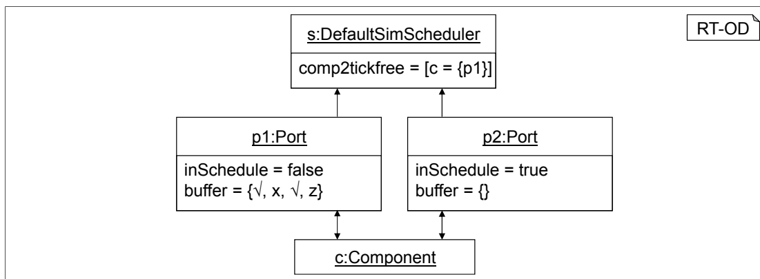
Figure 4.19: Object diagram which depicts the initial situation of the 'waking up ports' scenario.
