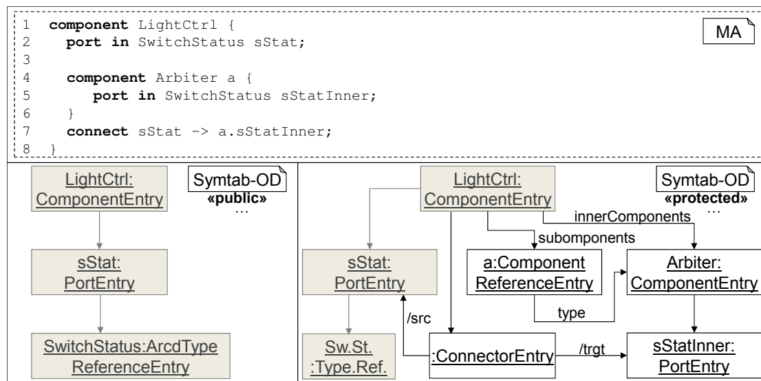
Figure 5.12: Difference between the public and the protected model interface.
