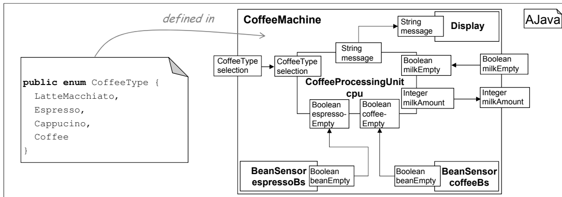
Figure 9.1: Architectural model of a coffee machine (according to [HRR10]).
