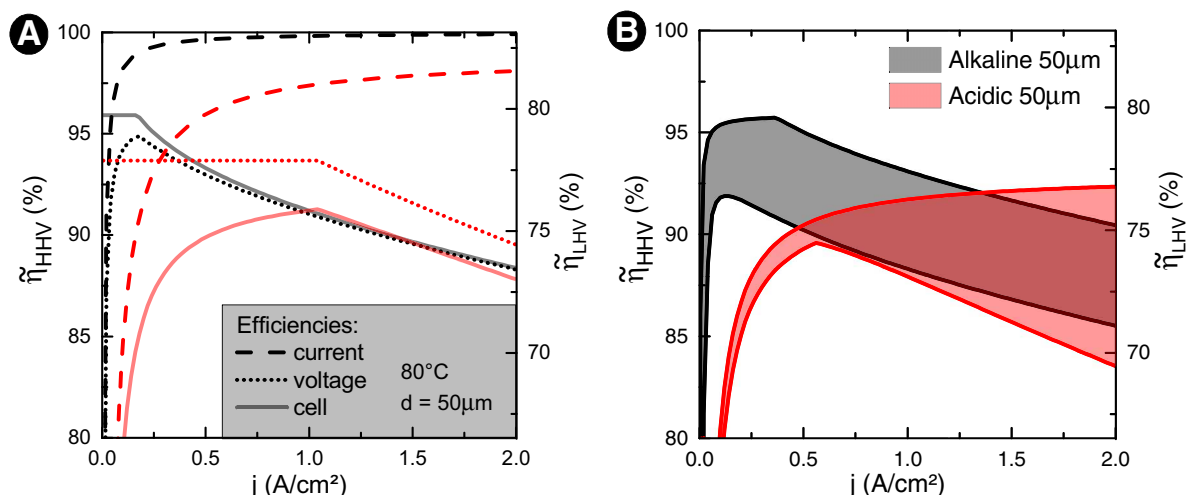
Figure 6. (A): Modeled cell efficiencies of the alkaline (black) and acidic PEM (red) water electrolyzer for separator thicknesses of 50 μm and a temperature of 80°C using the equations summarized in the Calculation of the cell efficiency section and the parameters stated in Table II. As motivated in the text, p^a = p^c = 6 bar were assumed for the alkaline cell while p^a = 6 bar and p^c = 2 bar were used to model the acidic cell. Dotted lines: Voltage efficiencies including heat balance. Dashed lines: Current efficiencies. Solid lines: Cell efficiencies. Left scale: Scale for the current efficiency, while voltage and cell efficiencies are normalized to the higher heating value. Right scale: Voltage and cell efficiency normalized to the lower heating value. (B): Error analysis of the cell efficiencies plotted in (A). The smallest and highest efficiencies that result from the experimentally determined parameters at the margins of their error range was plotted. The area between highest and lowest efficiencies was shaded gray for the alkaline cell and red for the acidic cell.
