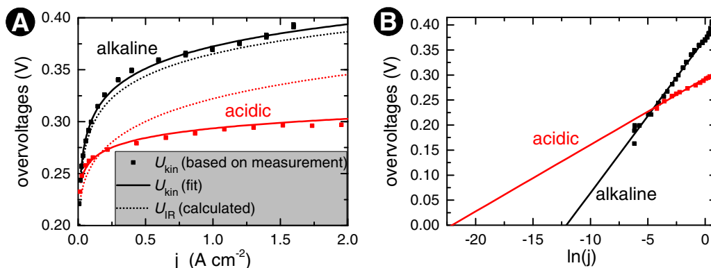
Figure 4. Kinetic overvoltages U_{kin} and IR-corrected overvoltages U_{IR} of the alkaline (black) and acidic (red) water electrolyzer as a function of the linear (A) and logarithmic current density (B). Scatter: U_{kin} obtained from the measurements graphed in Figure 3 via Equation 29. Solid lines: Fit to U_{kin} data by Equation 11 for (A) and linear fit for (B). Dotted lines: U_{IR} calculated by Equation 30. The fit parameters are stated in Table II.
