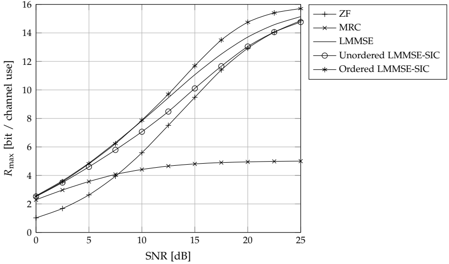
Figure 4.7: Upper bounds on the achievable data rates of a 4 \times 4 MIMO system with a Gray-mapped 16-QAM modulation, for different low-complexity detectors
