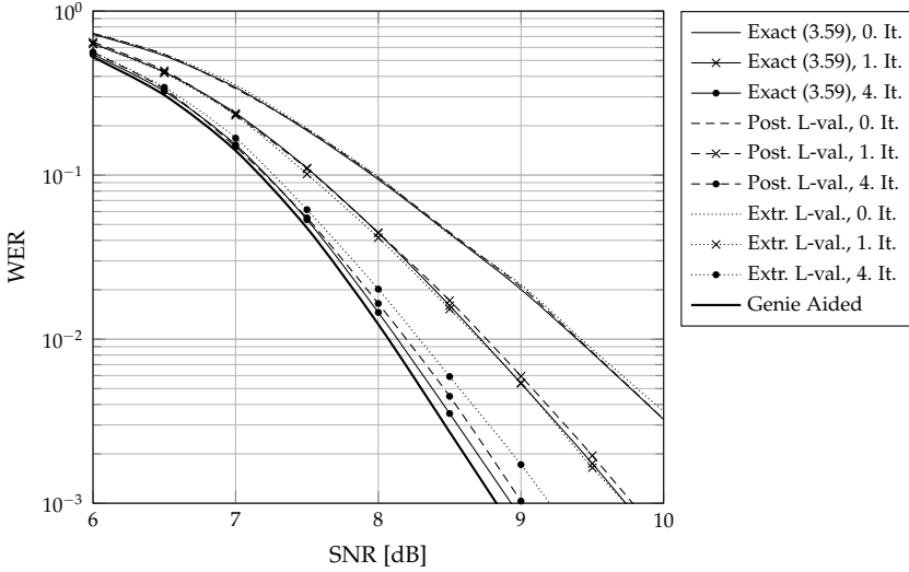
Figure 3.11: Comparison of different ways to compute the feedback q(x_D)
