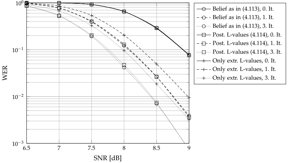
Figure 4.24: Performance of the MRC-Soft-PIC detector with different kinds of information that is being passed to the interference canceller and the MRC filter
