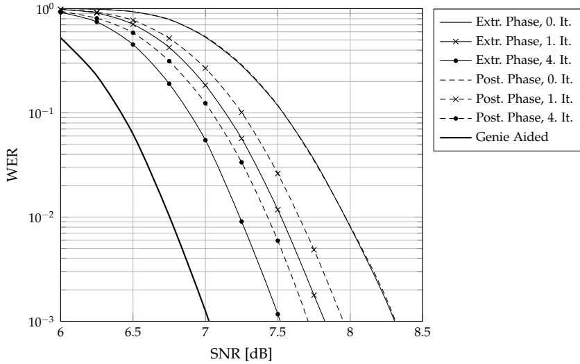
Figure 3.20: Comparison of extrinsic ( \vec{\zeta} ) and posterior ( \zeta = \vec{\zeta} + \vec{\zeta} ) phase information
