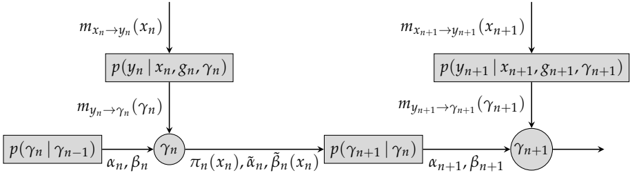
Figure 3.30: Detail of the factor graph which shows the relevant parts for the \gamma -estimator
