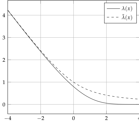
Figure A.1: The function \lambda(x) = \frac{f_{\mathcal{N}}(x)}{F_{\mathcal{N}}(x)} needed for evaluating the moments of the truncated Gaussian distribution, and its approximation \tilde{\lambda}(x) = \frac{1}{2}\sqrt{x^2 + 4} - \frac{x}{2} ( x \lesssim -3 )
