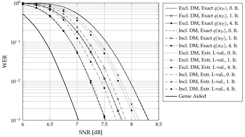
Figure 3.19: Comparison of exclusive (3.73) and inclusive (3.78) DM
