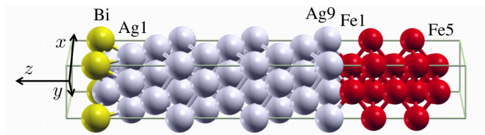
Figure 5.20.: Illustration of the unit cell of a \text{Ag}_2\text{Bi} -terminated \text{Ag}(111) film grown on ferromagnetic \text{Fe}(110) . Bi, Ag and Fe atoms are shown in yellow, gray and red respectively. Atomic coordinates are given in Table 5.5.
