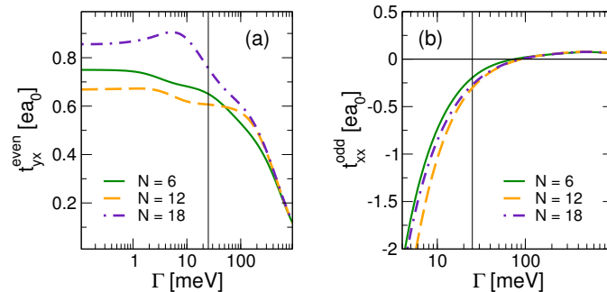
Figure 5.2.: a) Even torkance t_{yx}^{\text{even}} and b) odd torkance t_{xx}^{\text{odd}} in \text{L1}_0\text{-FePt}^2/\text{Pt}^N for N = 6 (green solid), 12 (orange dashed) and 18 (blue dot-dashed). Solid vertical lines correspond to the value of disorder strength \Gamma = 25 meV.
