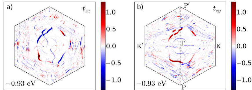
Figure 5.24.: Distribution of (a) \mathcal{T}_z(\mathbf{k})\lambda_x(\mathbf{k})/|\mathbf{v}(\mathbf{k})| and (b) \mathcal{T}_z(\mathbf{k})\lambda_y(\mathbf{k})/|\mathbf{v}(\mathbf{k})| in the Brillouin zone in units of \hbar . The Fermi energy is set 930 meV below its true value.
