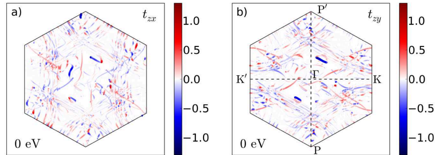
Figure 5.23.: Distribution of (a) \mathcal{T}_z(\mathbf{k})\lambda_x(\mathbf{k})/|\mathbf{v}(\mathbf{k})| and (b) \mathcal{T}_z(\mathbf{k})\lambda_y(\mathbf{k})/|\mathbf{v}(\mathbf{k})| in the Brillouin zone in units of \hbar . The Fermi energy is set to its true value.
