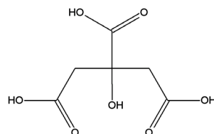
Figure 4: Chemical structure of citric acid.
