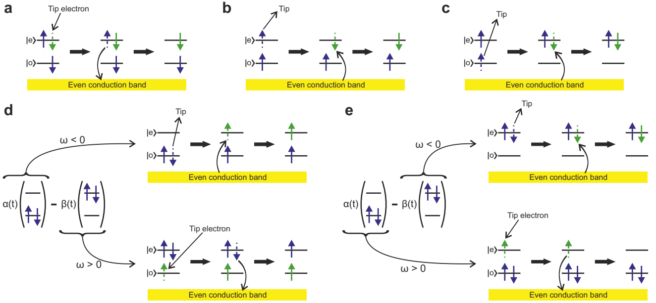
FIG. S6. Diagrams of different processes due to electron injection (extraction) to (from) the even/odd state. Symbols as in Fig. 3b and d in the paper. Note that the |o\rangle orbital decouples from the even conduction band (parity-symmetry), and accordingly no transitions between the two can occur. For a detailed discussion, refer to the text of the supplement.
