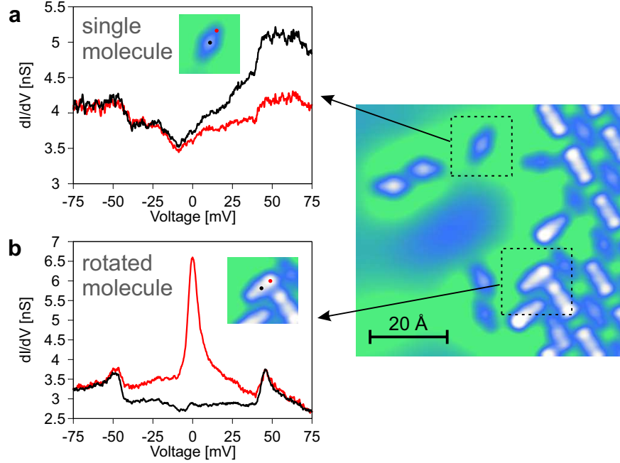
Figure 5.5: a dI/dV conductance spectra of an isolated single NTCDA molecule measured at different locations above the molecule as indicated in the inset. Measurements were performed at T = 4.3 K. b As panel a, but for a rotated molecule at the edge of a NTCDA island (rippled phase). The right panel shows an overview constant current STM image of the area where the single and rotated molecule are located ( I = 200 pA, V = 50 mV).
