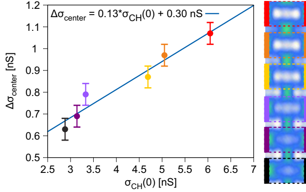
Figure 5.8: Plot of the step height \Delta\sigma_{\text{center}} at the center as a function of the height \sigma_{\text{CH}}(0) of the Kondo resonance at the CH site. The values are obtained from the different molecules in the rippled phase of NTCDA (see Fig. 5.2b and c). Color coding as in Fig. 5.2. Data points have been fitted by a linear function of the form \Delta\sigma_{\text{center}} = c * \sigma_{\text{CH}}(0) + b .
