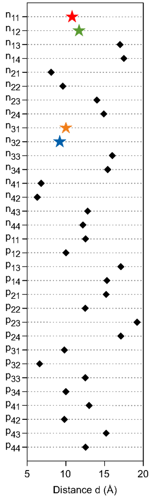
FIG. S2. Distance dependency of the dimers' spectral properties. Au-Au distances for the various dimer configurations. Symbols refer to dimer's spectral properties, black diamonds: unbroadened Kondo peaks, stars: broadened or gapped zero bias peaks (colour-code matches Fig. 1c and d in the paper).
