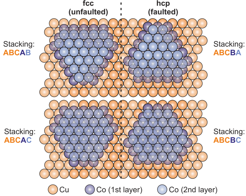
Figure 6.4: Illustration of the different stackings of the Co islands on Cu(111) using the hard sphere model. The adsorption of Co atoms on fcc or hcp sites of the Cu(111) surface leads to the formation of fcc (unfaulted) or hcp (faulted) Co islands, respectively. Model has been adapted from [149, 168].
