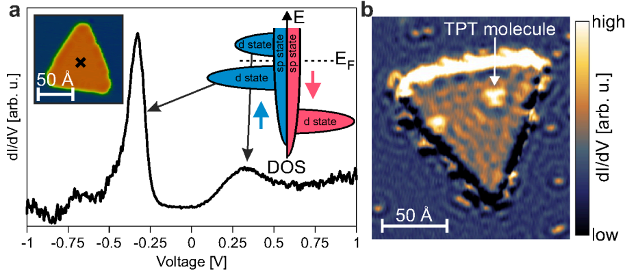
Figure 6.5: a Differential conductance dI/dV spectra acquired in the center of a Co island. For the measurement a non-magnetic tungsten tip has been used. Left inset shows the STM image of the corresponding Co island with the marked spectroscopy location ( V = 500 mV, I = 200 pA). Right inset illustrates the spin-polarized density of states (DOS) of Co islands according to Ref. [163, 169]. b Spectroscopic image of a Co island at V = +690 mV. The spatially modulated pattern is a result of the sp electron confinement in the Co island. A detailed analysis of the adsorption of the TPT molecules is presented in section 6.5.
