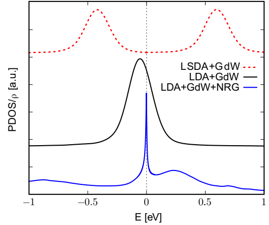
FIG. 11. (Color online) Projected density of states of the LUMO+Au orbital from an unpolarized LDA+ GdW calculation (black) in comparison to the spin-polarized LSDA+ GdW result (red dashed) of Fig. 10. In addition, the LDA+ GdW +NRG result is included ( T = 0 K and U = 1.2 eV, see Sec. III D).
