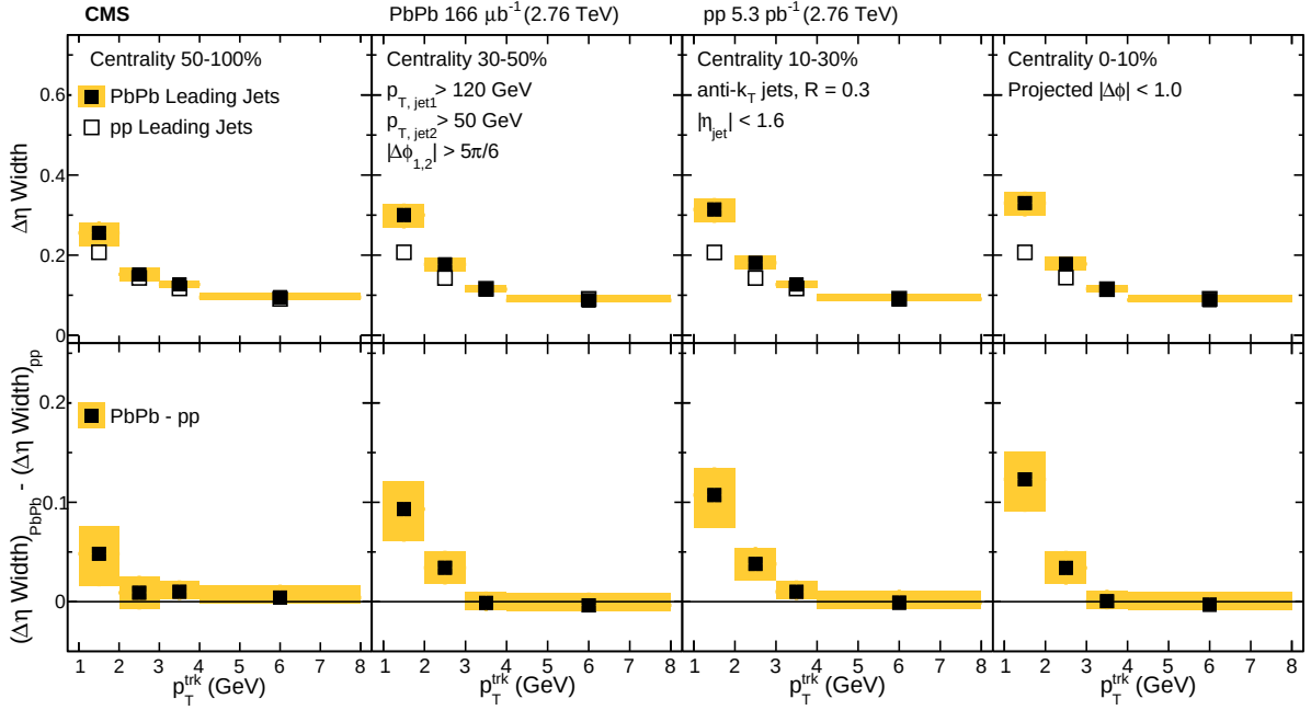
Figure 8: Comparison of the widths in PbPb and pp of the \Delta\eta charged-particle distributions correlated to leading jets with p_{T,\text{jet1}} > 120 GeV, as a function of p_T^{\text{trk}} . The bottom row shows the difference of the widths in PbPb and pp data. The shaded band corresponds to systematic uncertainty, and statistical uncertainties are smaller than symbol size.
