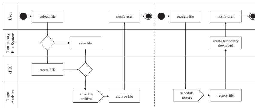
Fig. 2: Simplified overview of simpleArchive processes
