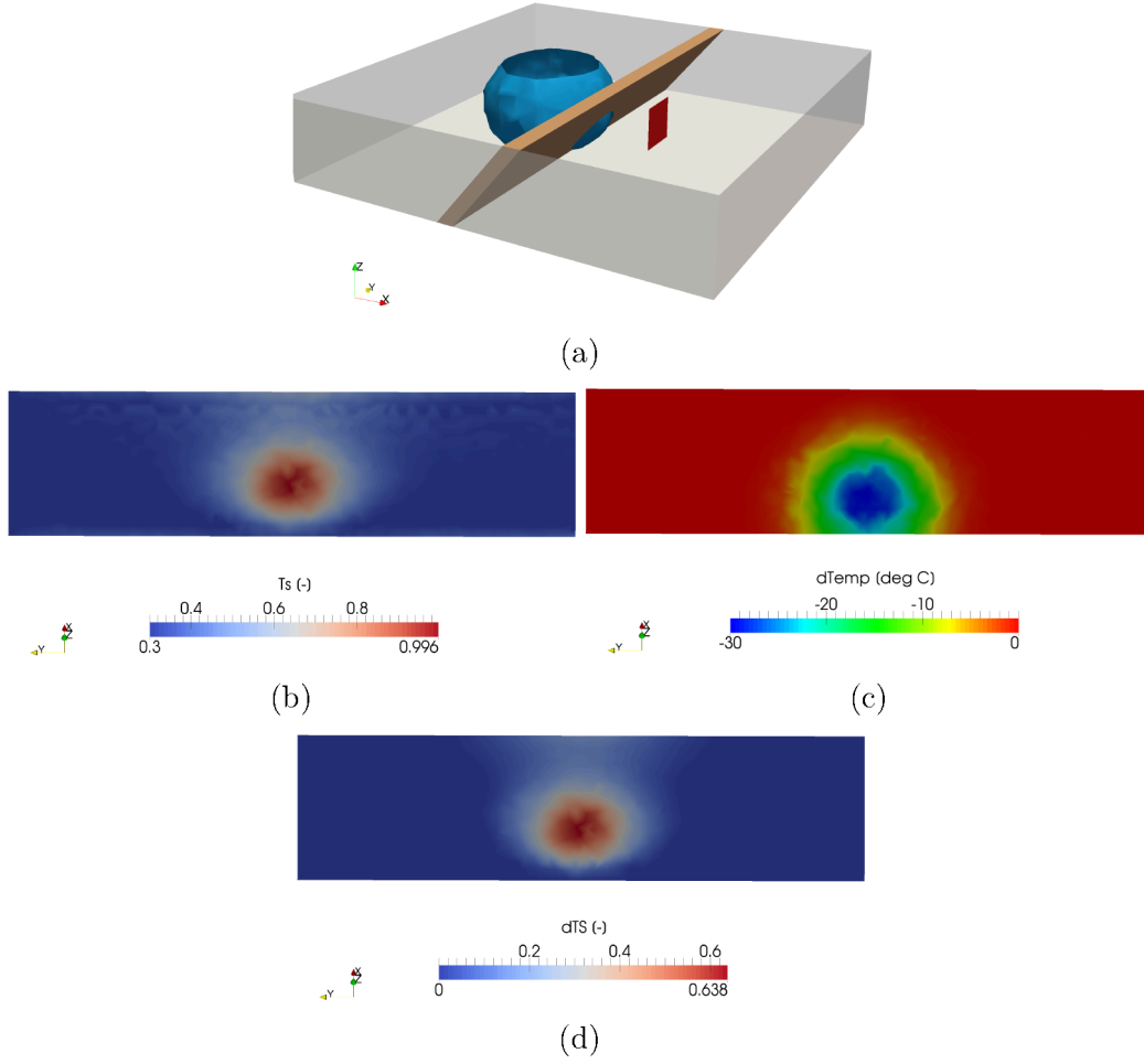
Fig. 5.4 Results after 15 years of injection. (a) The 3-D model with the 130^\circ\text{C} isotherm (in blue). (b) 2-D view of a cross-section on the fault place showing the slip tendency T_s distribution. (c) On the same cross-section, distribution of the temperature difference with initial conditions. (d) On the same cross-section, distribution of the slip tendency difference with initial conditions ( dT_s = T_s - T_s^i ).
