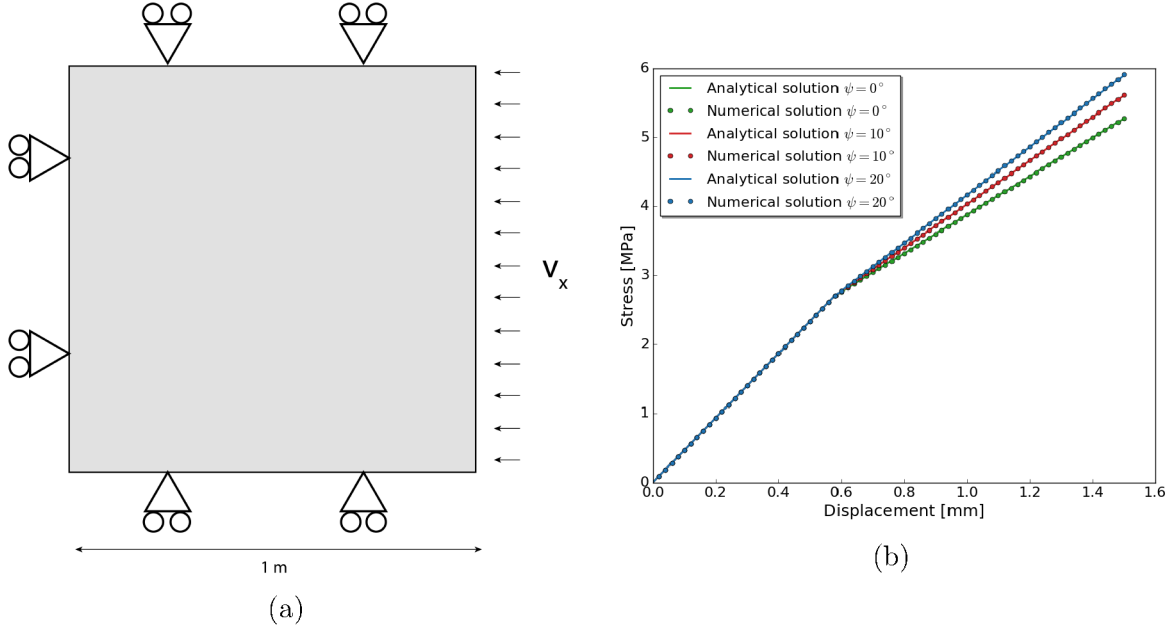
Fig. 2.6 Problem formulation and results of the oedometer benchmark. Panel 2.6a shows the problem formulation. Panel 2.6b illustrates the results for different dilation angles with the stress-displacement curves.
