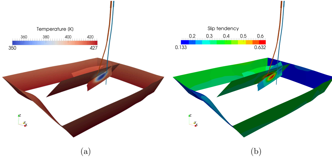
Fig. 5.7 Results of fully coupled THM process modelling for the Groß Schönebeck geothermal reservoir. Here only the faults in the reservoir are shown after 100 years of injection of cold fluid (70 °C) at 30 \text{ m}^3 \cdot \text{h}^{-1} . (a) Temperature distribution. (b) Slip tendency. The blue line represent the path of the injection well and the red one the path of the production well.
