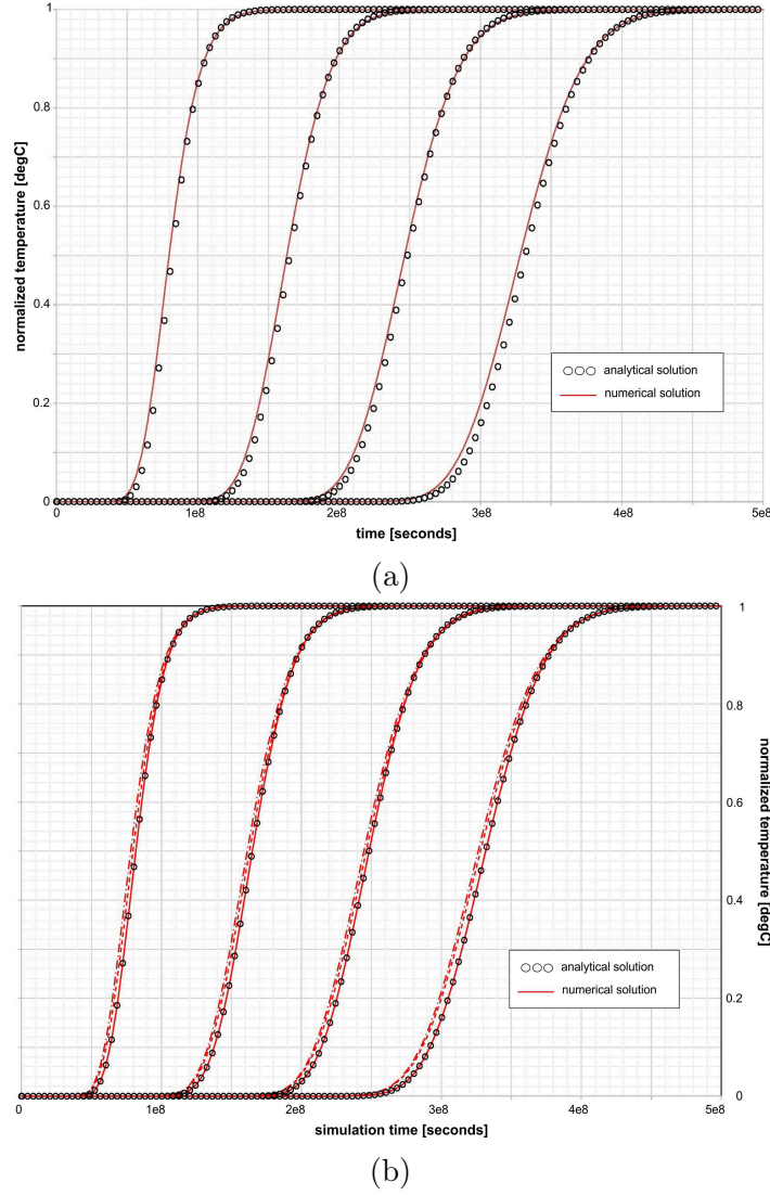
Fig. 2.3 Comparison of numerical results (red curves) and analytical solutions (black circles) for heat transport in a fracture. Panel 2.3a shows the temperature evolution at different positions along the fracture as a function of time. The mesh resolution was kept constant and equal to 0.2m. Panel 2.3b illustrates the same results but considering a refinement in the discretisation (mesh resolution of 0.1 m).
