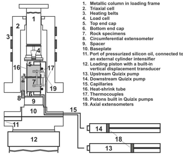
Fig. C.1 Sketch of the triaxial cell with connected pore fluid pump system (Pei et al., 2016).
