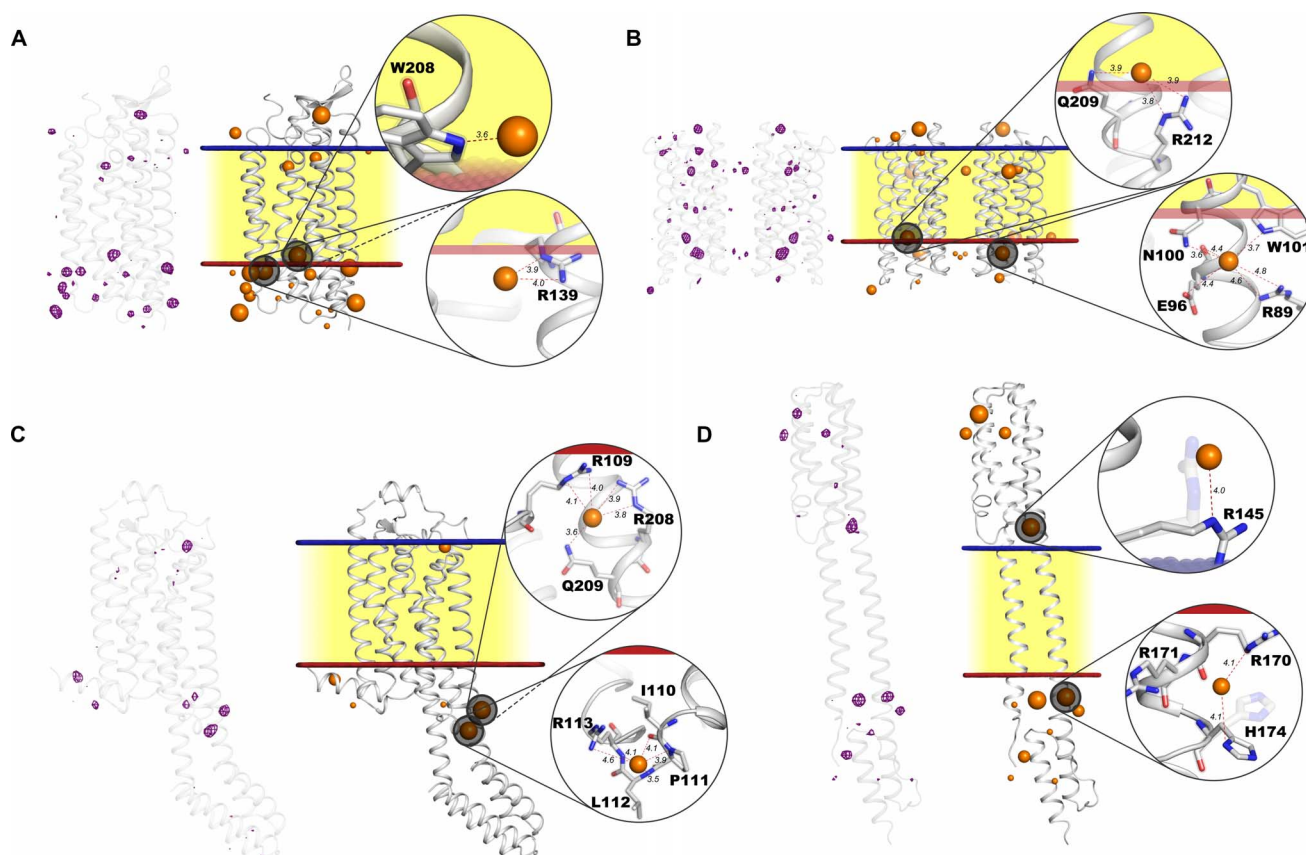
Fig. 4. Cartoon representations of the crystal structures of the four classes of MP solved using the I-SAD/I-SIRAS technique. (A) KR2. (B) MACR (noncrystallographic dimer). (C) A 2A -AR-BRIL-ΔC. (D) NarQ. On the left of each representation, peaks in I-SAD anomalous difference Fourier maps [purple chicken wire, highest-resolution I-SAD data sets for each target (Table 1), contoured at the 3.5 × r.m.s. (root mean square) level] are shown superposed on the C α backbone of the protein. On the right of each panel, the blue and red lines represent outer and inner lipidic membrane surfaces, respectively, with the hydrophobic region of the lipidic membrane represented in yellow. Iodine ions are shown as orange spheres, divided into three sizes based on the height of anomalous difference map peaks. Two iodine binding sites per crystal structure are highlighted to illustrate their environment. In (D), it is clear that protein residues may change their side-chain conformation upon binding of iodide (conformation in native structures shown as shadows).
