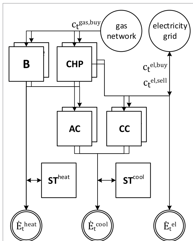
FIGURE 4 | Superstructure of real-world example based on Voll et al. (2013): boiler (B), combined heat and power unit (CHP), compression chiller (CC), and absorption chiller (AC) extended by thermal storage (ST) with variable capacity for cooling and heating. Time series (Figure 5) of volatile energy prices c_t and energy demands \dot{E}_t are considered.
