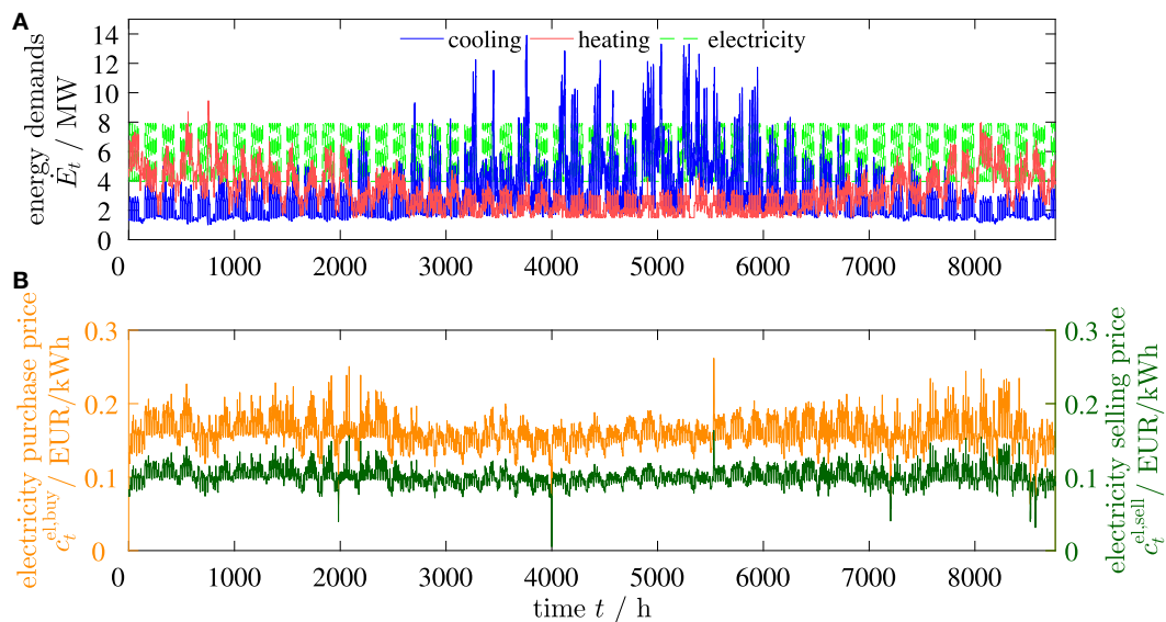
FIGURE 5 | Time series \mathcal{T}\mathcal{S} of the original instance for (A) heating, cooling, and electricity demands, and (B) electricity purchase and selling price over 1 year with a resolution of 1 h.
