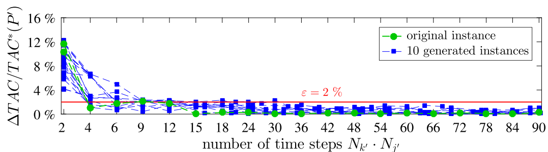
FIGURE 7 | Normalized accuracy measure \Delta TAC divided by total annualized cost of the aggregated synthesis problem TAC^*(P') as function of number of time steps ( N_{k'} \cdot N_{j'} ) for the original instance and 10 generated instances, threshold value of \varepsilon = 2\% as solid red line.
