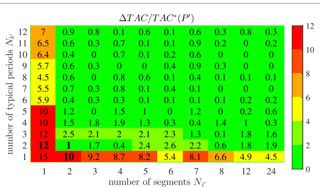
FIGURE 8 | Normalized accuracy measure \Delta TAC divided by total annualized cost of the aggregated synthesis problem TAC^*(P') in percent as numbers in the cells and color code. The path of the iterative method is indicated with bold numbers.
