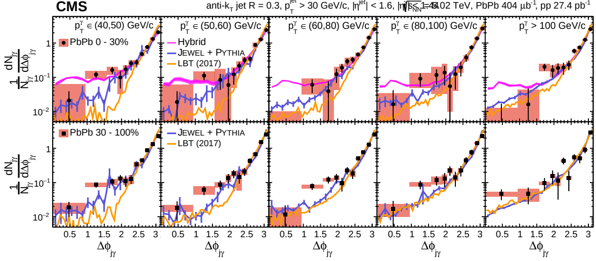
Figure 8: The azimuthal correlation of photons and jets in five p_T^\gamma intervals for 0–30% centrality (top, full circles) and 30–100% centrality (bottom, full squares) PbPb collisions. The data points shown are identical to those in Fig. 2. Theoretical calculations from JEWEL [37, 60], LBT [34], and hybrid model [35, 36] are included for comparison.
