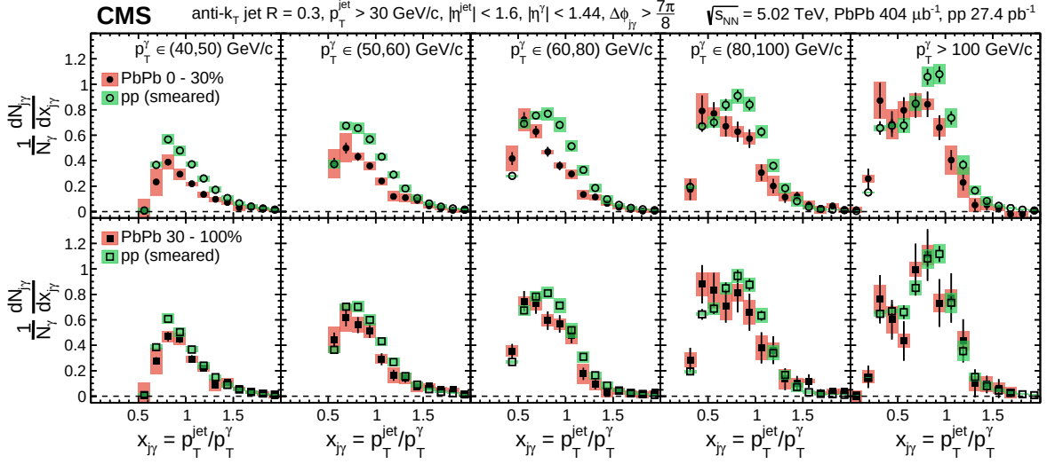
Figure 3: Distribution of x_{j\gamma} = p_T^{jet}/p_T^\gamma in five p_T^\gamma intervals for 0–30% centrality (top, full circles) and 30–100% centrality (bottom, full squares) PbPb collisions. The smeared pp data (open symbols) are included for comparison. The vertical lines (bands) through the points represent statistical (systematic) uncertainties.
