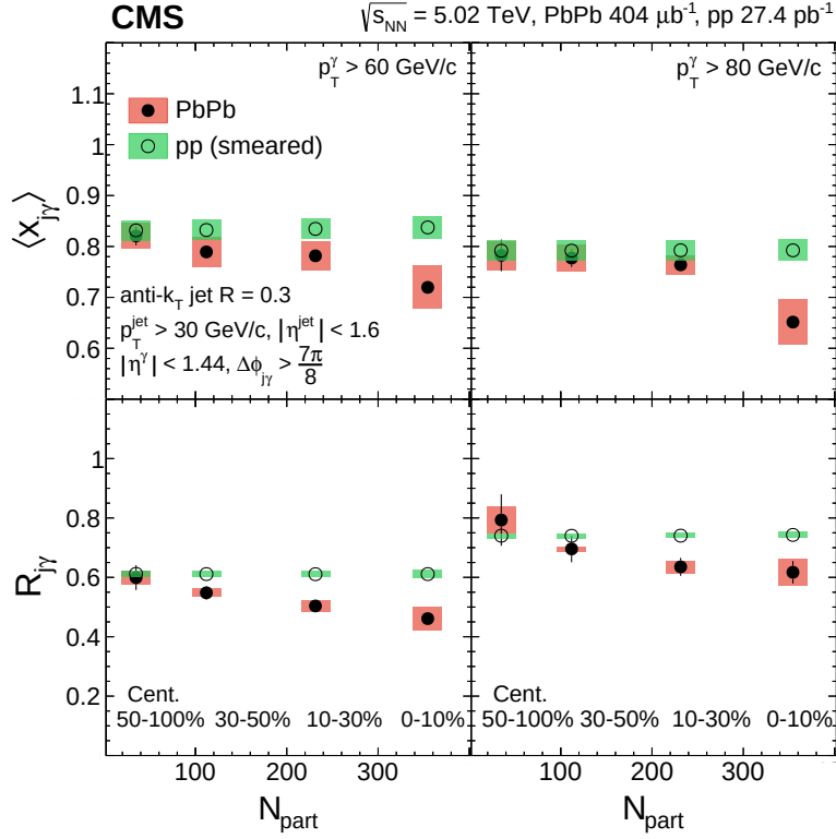
Figure 7: The \langle x_{j\gamma} \rangle (top) and R_{j\gamma} (bottom) as a function of \langle N_{part} \rangle for p_T^\gamma > 60 GeV/c (left) and p_T^\gamma > 80 GeV/c (right). The PbPb results (full markers) are compared to pp results (open markers) smeared by the relative jet energy resolution corresponding to each centrality interval. The vertical lines (bands) through the points represent statistical (systematic) uncertainties.
