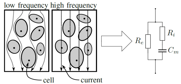
Figure 1: Current flow through biological tissue at low and high frequencies and electrical equivalent circuit (from [11]).
