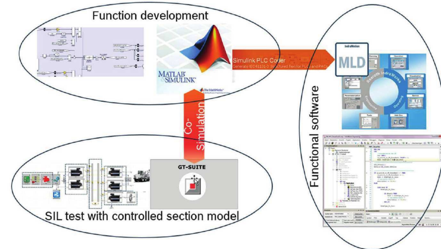
Figure 9: Tool chain for sample development of an electric traction drive
