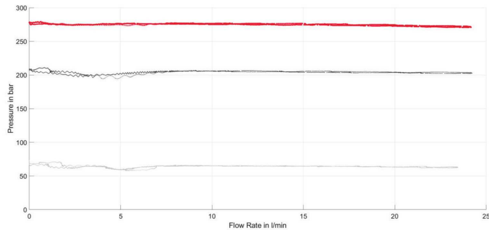
Figure 6: Pressure-flow-characteristic.
