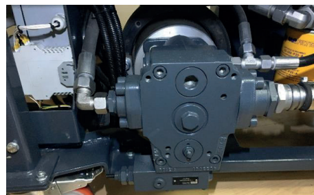
Figure 2. Hydraulic power unit with variable displacement axial piston pump
