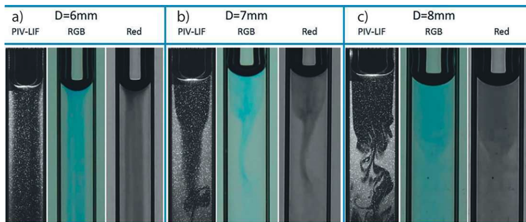
Figure 28. Wake structures of rising Taylor bubbles in different channels with (a) laminar wake, (b) toroidal wake and (c) turbulent wake. Reproduced from ref. [24]
