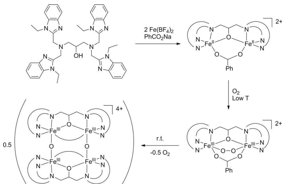
Scheme 12. Reaction of Et-HPTB stabilised iron species with dioxygen. [101]
