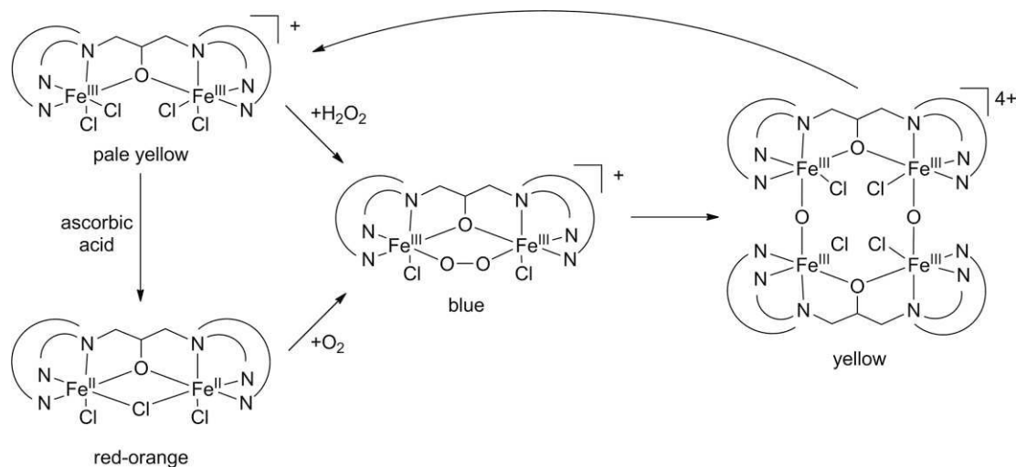
Scheme 14. Reaction of HPTB iron system with O_2 and H_2O_2 . [111]
