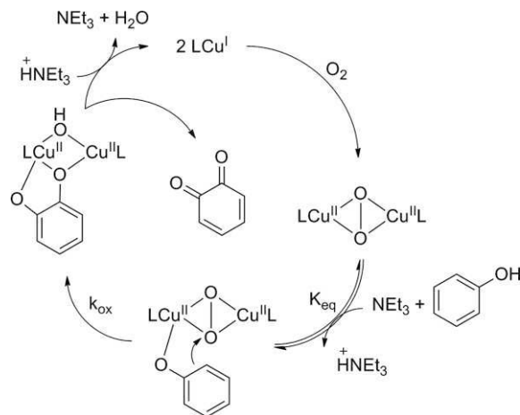
Scheme 7. Proposed reaction mechanism of catalytic phenol oxidation in presence of triethylamine.
