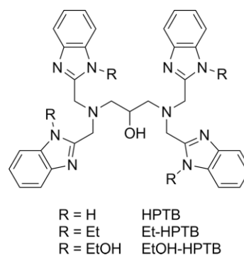
Figure 29. Ligand system HPTB and its derivatives.
