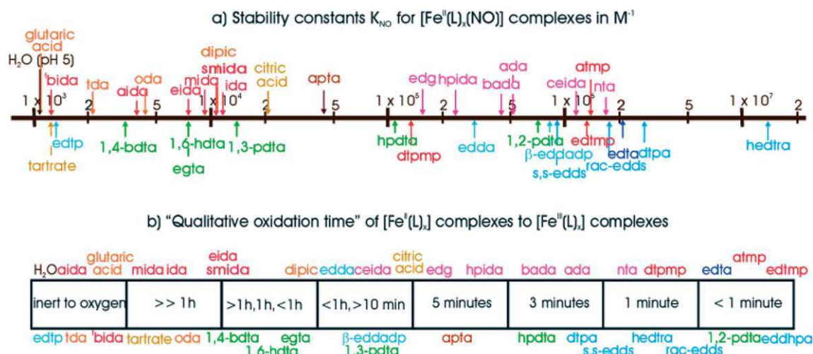
Figure 32. Correlation between K_{\text{NO}} and qualitative oxidation time of [\text{Fe}^{\text{II}}(\text{L})_x] complexes. Reproduced from ref. [124]
