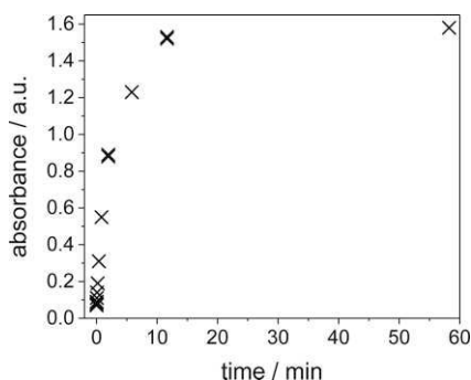
Figure 27. SFM measurement of the formation of an O species with the [Cu(TMGdmap)] system in MeCN at ambient temperatures ( \lambda_{\text{max}} = 395 \text{ nm} ). [92]
