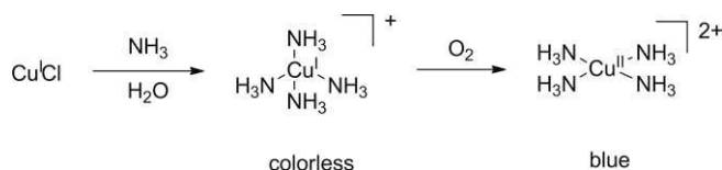
Scheme 9. Reaction of CuCl in aqueous ammonia and consecutive reaction with dioxygen.
