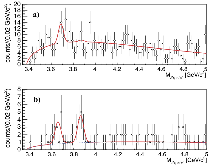
Fig. 4. (a) The J/\psi\pi^+\pi^- invariant mass distributions for the J/\psi\pi^+\pi^\pm final state (two entries per event) for non-exclusive events ( -12 \text{ GeV} < \Delta E < -4 \text{ GeV} ) and (b) for exclusive events ( -4 \text{ GeV} < \Delta E < 4 \text{ GeV} ) with missing mass M_{\text{miss}} above 3 \text{ GeV}/c^2 (see text for the definition of M_{\text{miss}} ).
