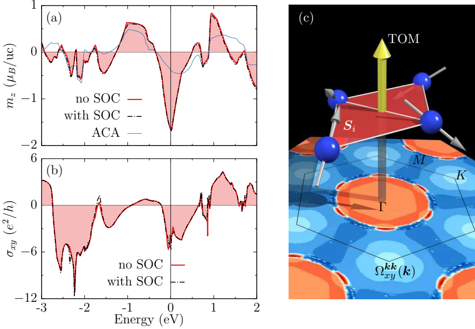
Figure 6.5: (a) Out-of-plane orbital magnetization m_z and (b) anomalous Hall conductivity \sigma_{xy} of the unsupported Mn monolayer in the 3Q state. The calculations were performed without (red solid line) and with (black dashed line) including the effect of spin-orbit coupling (SOC). The blue thin line refers to the atom-centered approximation (ACA). (c) Emergence of a topological orbital moment (TOM) that roots solely in the complex phase-space geometry as revealed by the distribution of the Berry curvature \Omega_{xy}^{kk} . The latter quantity ranges from large positive (dark red) to large negative (dark blue) values.
