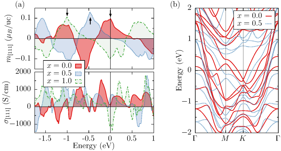
Figure 6.7: Transport and magnetic properties in strained \gamma\text{-Fe}_x\text{Mn}_{1-x} with \delta = 0.95 and non-collinear 3Q spin structure. (a) Dependence of the orbital magnetization and the anomalous Hall conductivity on the position of the Fermi level in various alloys. Characteristic features that shift towards lower energies with increasing x are marked by black arrows. The magnetic in-plane unit cell of four atoms is denoted by “uc”. (b) The band structures for the two concentrations x = 0.0 and x = 0.5 reveal strong correlations due to the similar electron configuration of Fe and Mn. Spin-orbit coupling was not taken into account in (a) and (b).
