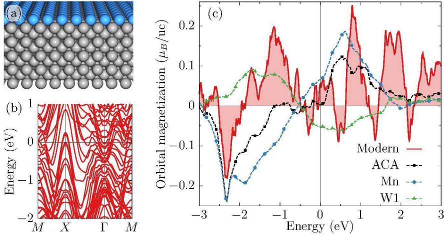
Figure 6.2: (a) Crystal structure and (b) band structure of a Mn monolayer on nine atomic layers of W(001). (c) Orbital magnetization perpendicular to the film plane of Mn/W(001). The dependence of m_z on the position of the Fermi level is presented within the modern theory (red solid line) and the atom-centered approximation (ACA, black squares), where the orbital magnetization is given in units of Bohr magneton per in-plane unit cell. In addition, the local orbital moments in the muffin tins of Mn and the W at the interface (W1) are indicated by blue circles and green triangles, respectively.
