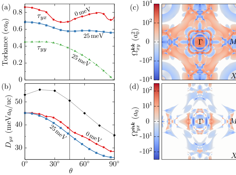
Figure 8.2: Anisotropy of (a) torkance and (b) spiralization with respect to the magnetization direction \hat{\mathbf{m}} = (\sin \theta, 0, \cos \theta) in Mn/W(001). While \tau_{yx} and D_{yx} are shown in the clean limit as well as for \Gamma = 25 meV, the anisotropy of \tau_{yy} is studied only for moderate disorder. The behavior of D_{yx} is compared in (b) to data points (black diamonds) each of which was extracted from a separate set of maximally-localized Wannier functions [238]. (c,d) Distribution of momentum Berry curvature \Omega_{xy}^{kk} and mixed Berry curvature \Omega_{yx}^{mk} throughout the Brillouin zone for an out-of-plane magnetization.
