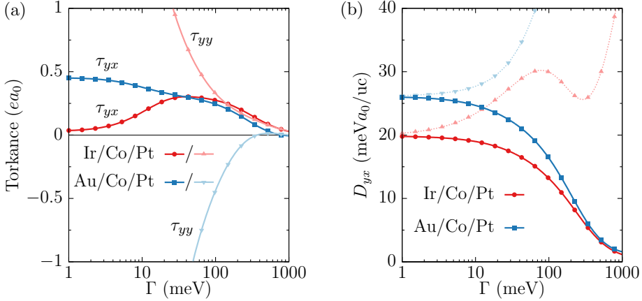
Figure 8.5: Behavior of (a) torkance and (b) spiralization with increasing band broadening \Gamma in the compounds Ir/Co/Pt (red) and Au/Co/Pt (blue) with perpendicular magnetization. In panel (a), dark and light colors are used to illustrate the even torkance \tau_{yx} and the odd torkance \tau_{yy} , respectively. In addition to the dependence of D_{yx} , we depict in (b) the contribution proportional to the imaginary part of the logarithm in Eq. (4.61) using dotted lines.
