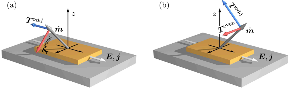
Figure 4.6: If an electric field \mathbf{E} (or, equivalently, a charge current \mathbf{j} ) is applied to an inversion-asymmetric magnetic heterostructure, the magnetization reorients its direction \hat{\mathbf{m}} as a response to the resulting spin-orbit torques. These torques can be decomposed into an antidamping (even) and a field-like (odd) contribution according to Eqs. (4.44) and (4.45).
