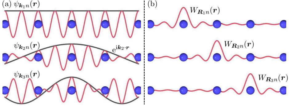
Figure 5.1: Real-space representation of the electronic structure of a periodic crystal in terms of (a) Bloch functions \psi_{\mathbf{k}n}(\mathbf{r}) and (b) Wannier functions W_{\mathbf{R}n}(\mathbf{r}) for various values of the crystal momentum \mathbf{k} and the direct lattice vector \mathbf{R} . While the Bloch states are delocalized in real space, the localized Wannier functions exhibit well-defined centers. The black lines in (a) indicate the phase factor e^{i\mathbf{k}\cdot\mathbf{r}} of the Bloch functions. Figure inspired by [168].
