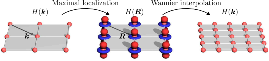
Figure 5.3: Illustration of the Wannier interpolation scheme. Starting from the electronic structure as encoded in the Hamiltonian H(\mathbf{k}) on a coarse \mathbf{k} -grid, we construct Wannier functions that are localized in real space at the positions \mathbf{R} . Using these functions to represent efficiently the electronic structure in terms of the hoppings H(\mathbf{R}) , we obtain ultimately the Hamiltonian on a much denser mesh of \mathbf{k} -points via an inverse Fourier transformation. Figure inspired by [168].
