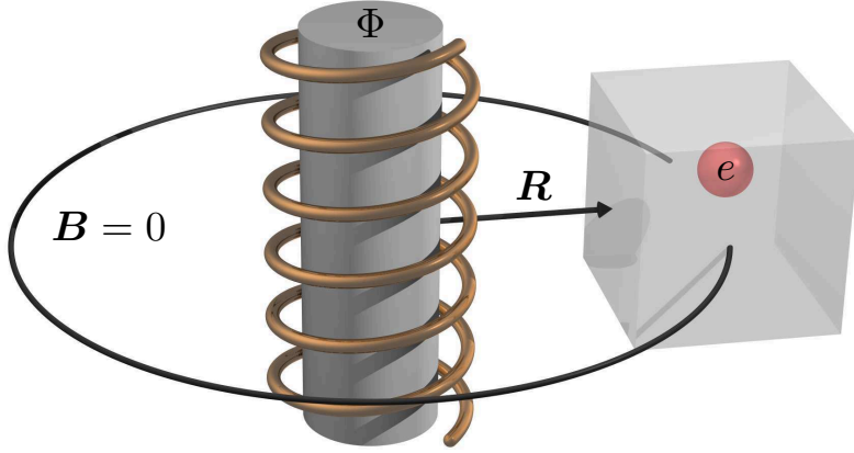
Figure 4.2: Setup for the Aharonov-Bohm effect. The magnetic field is restricted in real space to an infinitely long solenoid around which the box of the electrons (red sphere) is dragged. Due to the magnetic flux \Phi piercing the encompassed region, a topological Berry phase manifests in the electronic wave function.
