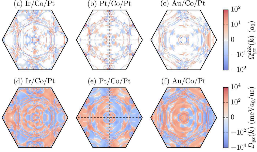
Figure 8.6: Distribution of the mixed Berry curvature \Omega_{yx}^{mk} (top) and the Dzyaloshinskii-Moriya spiralization D_{yx} (bottom) of all occupied bands in the hexagonal Brillouin zone for the three stoichiometric heterostructures (a,d) Ir/Co/Pt, (b,e) Pt/Co/Pt, and (c,f) Au/Co/Pt. The Co monolayer in these thin films is perpendicularly magnetized. In the labels, a_0 denotes Bohr’s radius and “uc” stands for the in-plane unit cell. Note the logarithmic color scale.
