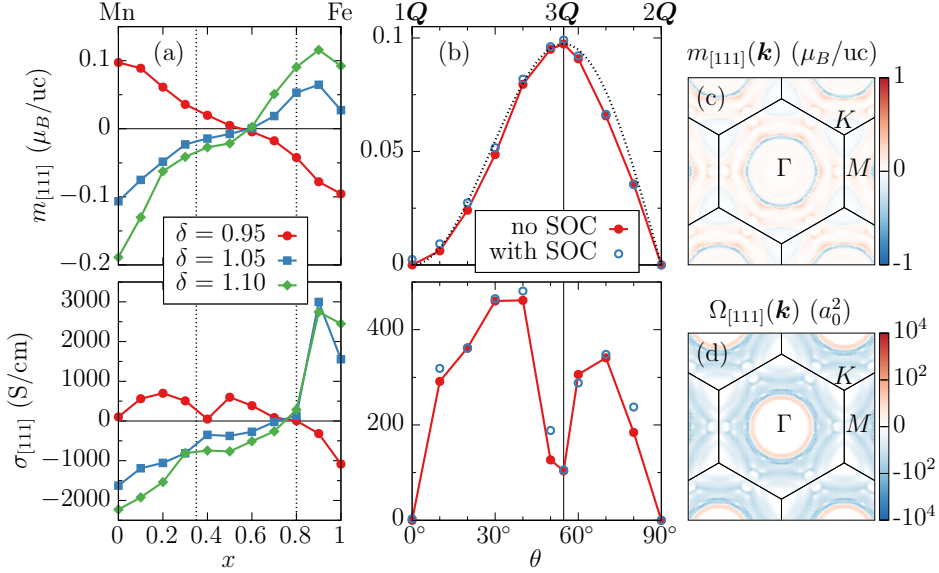
Figure 6.8: Effect of composition ratio and spin texture in strained \gamma\text{-Fe}_x\text{Mn}_{1-x} without spin-orbit coupling (SOC). (a) Orbital magnetization m_{[111]} and anomalous Hall conductivity \sigma_{[111]} for varying composition ratio x and several choices of the strain \delta . The imposed 3Q state is experimentally confirmed to arise in the unstrained compounds within the region bounded by dotted vertical lines. (b) Dependence of m_{[111]} and \sigma_{[111]} on the polar angle \theta that characterizes the antiferromagnetic spin texture, for x = 0 and \delta = 0.95 . Additionally, the spin-orbit interaction was included in the case of the blue open circles, and the black dotted line marks the angular dependence of the scalar spin chirality, Eq. (6.4). (c,d) Distribution of the \mathbf{k} -resolved orbital magnetization and the Berry curvature in momentum space for the 3Q state without spin-orbit coupling. Note the logarithmic color scale used for the Berry curvature.
