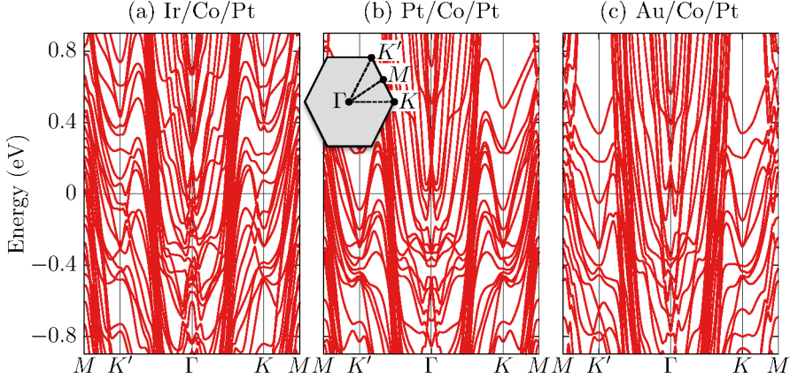
Figure 8.3: Electronic band structure along the high-symmetry lines of the hexagonal Brillouin zone (see inset of the middle panel) in the three stoichiometric heterostructures of (a) Ir/Co/Pt, (b) Pt/Co/Pt, and (c) Au/Co/Pt. The energy scale is relative to the corresponding Fermi level. In all of these cases, the Co layer is magnetized perpendicular to the film plane, which corresponds to the polar angle \theta = 0 .
