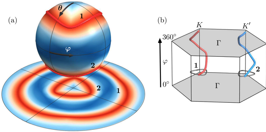
Figure 9.6: Mixed nodal lines in the functionalized bismuth film. (a) The global band gap evolves with the magnetization direction \hat{\mathbf{m}} = (\cos \varphi \sin \theta, \sin \varphi \sin \theta, \cos \theta) as indicated by the colors ranging from red (no gap) to blue (finite gap). The energy gap vanishes along two closed loops in the upper (1) and lower (2) hemisphere, respectively, and the topological Berry phase is non-trivial around these two mixed nodal lines. (b) These loops can be understood as mixed Weyl points that are dragged around either K (1, red) or K' (2, blue) in the hexagonal Brillouin zone as \varphi varies and \theta is adapted accordingly. Solid gray lines denote projections of these nodal lines to the plane.
