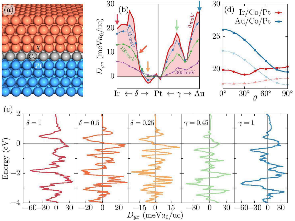
Figure 8.4: (a) Crystal structure of the Co-based heterostructures comprising the Pt substrate, the Co monolayer, and the overlayers X. (b) Spiralization D_{yx} for varying overlayer composition in \text{Ir}_\delta\text{Pt}_{1-\delta}/\text{Co}/\text{Pt} and \text{Au}_\gamma\text{Pt}_{1-\gamma}/\text{Co}/\text{Pt} , respectively, where the magnetization is perpendicular to the film plane. While the solid red curve corresponds to the clean limit, the dotted lines include the effect of disorder due to a finite broadening \Gamma of the energy bands by 25 meV, 100 meV, and 300 meV. The spiralization is given in units of \text{meV}a_0/\text{uc} , where “uc” stands for the in-plane unit cell. (c) Energy dependence of D_{yx} in the clean limit for the different alloy concentrations that are marked in (b) by correspondingly colored arrows. The energy scale is relative to the according Fermi level. (d) Anisotropy of D_{yx} with respect to the magnetization direction represented by the polar angle \theta in the compounds \text{Ir}/\text{Co}/\text{Pt} and \text{Au}/\text{Co}/\text{Pt} for \Gamma = 0 meV (solid lines) and \Gamma = 25 meV (dotted lines).
