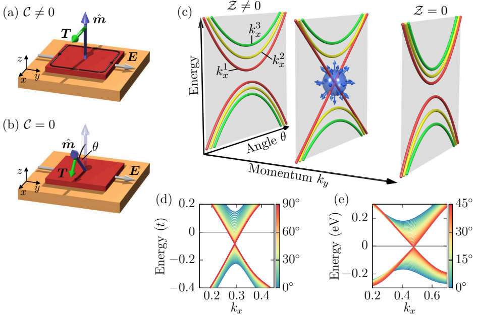
Figure 9.1: Emergence of mixed Weyl points in the complex phase space of crystal momentum and magnetization direction. (a) If an electric field \mathbf{E} is applied, the magnetization \hat{\mathbf{m}} of a topologically non-trivial insulator is subject to the antidamping torque \mathbf{T} . (b) The resulting reorientation of \hat{\mathbf{m}} by an angle \theta can trigger a topological phase transition to the trivial insulator. (c) Schematic evolution of two energy bands in the complex phase space, where colors represent different values of k_x . If we tune k_y , the electronic structure displays a monopole as signaled by the change of the mixed Chern number \mathcal{Z} . Indeed, such crossing points are observed in (d) the model of magnetically doped graphene with hopping t and atomic distance a , and (e) the functionalized bismuth film, where colors indicate the magnetization direction \hat{\mathbf{m}} = (\sin \theta, 0, \cos \theta) in both cases. The value of k_y is fixed to (d) k_y = 0.41 \cdot 4\pi/(3a) and (e) k_y = 0.19 in internal units.
