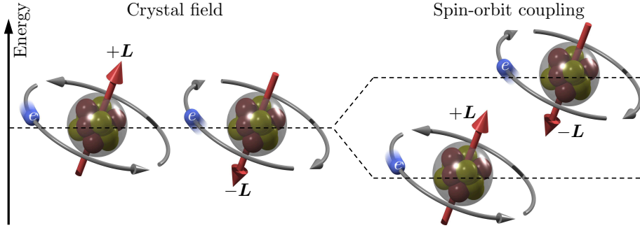
Figure 4.4: If electrons circulate with a certain rotational sense around the nucleus, an orbital angular momentum +L emerges. In the crystal field, however, this state is energetically equivalent to the situation with the opposite rotational sense, which leads to a cancellation and no net orbital moment. Only when coupling the spin degrees of freedom to the crystal lattice via the spin-orbit interaction, we break this orbital degeneracy such that a finite orbital moment may manifest.
