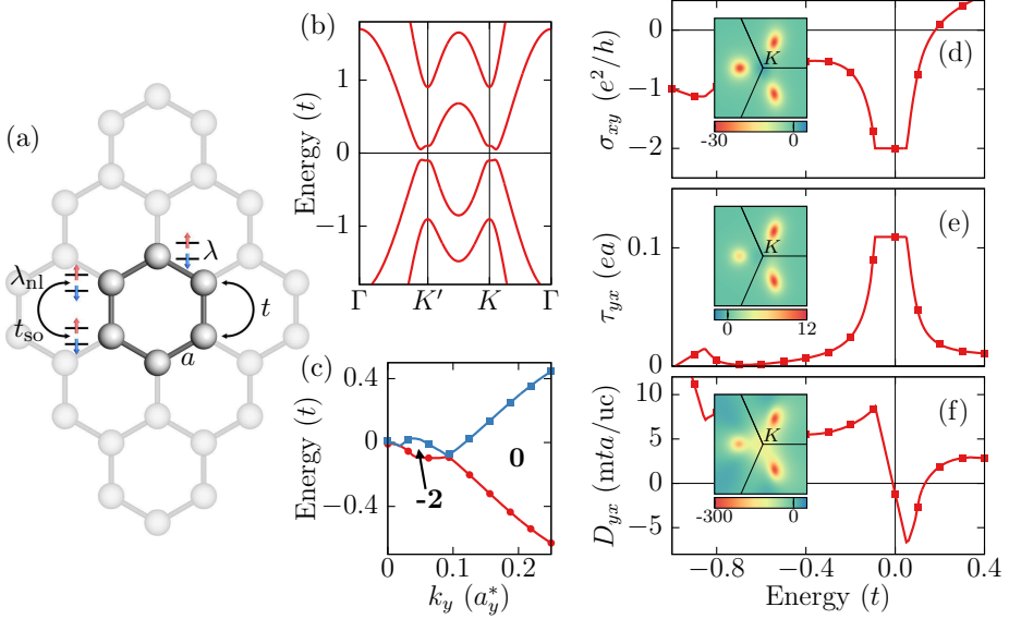
Figure 9.2: Model of magnetically doped graphene. (a) Sketch of the tight-binding model and the parameters therein. (b) Band structure with out-of-plane magnetization and t_{so} = 0.3t , \lambda = 0.1t , \lambda_{nl} = 0.4t . (c) Evolution of the valence band top (red circles) and conduction band bottom (blue squares) with k_y , where the depicted gap closing occurs for \theta = -90^\circ and \mathbf{k} = (0.71a_x^*, 0.09a_y^*) with a_x^* = 2\pi/(\sqrt{3}a) and a_y^* = 4\pi/(3a) . Bold integers denote the mixed Chern number \mathcal{Z} in the insulating regions. (d)–(f) Energy dependence of the anomalous Hall conductivity \sigma_{xy} = Ce^2/h = e^2/(2\pi h) \int \Omega_{xy}^{kk} dk_x dk_y , the torkance \tau_{yx} , and the spiralization D_{yx} , respectively, for an out-of-plane magnetization. Insets show the corresponding momentum-space distributions summed over all occupied states in the vicinity of the K -point.
