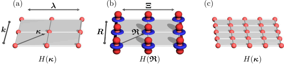
Figure 7.2: Scheme of the higher-dimensional Wannier interpolation. (a) Initially, the electronic structure is known on a coarse mesh of few \mathfrak{R} -points, where the variable \mathfrak{R} = (\mathbf{k}, \lambda) encompasses the crystal momentum \mathbf{k} and the abstract parameter \lambda . (b) Based on this information, we construct a set of higher-dimensional Wannier functions that are localized at positions \mathfrak{R} = (\mathbf{R}, \Xi) in the extended real space. (c) Using the generalized hoppings H(\mathfrak{R}) , we establish by means of an inverse Fourier transformation an efficient but accurate interpolation of the Hamiltonian onto a much denser \mathfrak{R} -grid.
