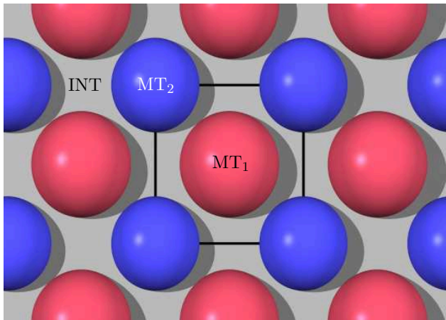
Figure 3.1: In the augmented-plane-wave method, the real space is partitioned into non-overlapping spheres (here MT_1 and MT_2 ) around the nuclei, known as muffin tins, and the interstitial region (INT). The different basis functions in these real-space regions are adapted to describe adequately the wave functions either near the nuclei or in between them. The unit cell of the depicted cubic lattice is indicated by black lines.
