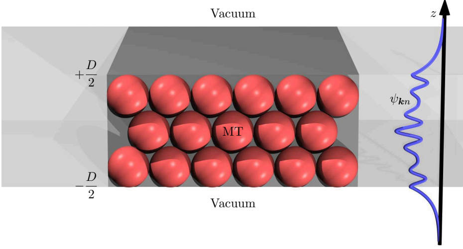
Figure 3.2: In addition to the muffin tins (MT) and the interstitial region, FLAPW calculations of truly two-dimensional geometries introduce vacuum regions for |z| > D/2 , where z denotes the direction perpendicular to the film plane. The wave function \psi_{\mathbf{k}n} of the illustrated three-layer system decays exponentially into the vacuum regions.
