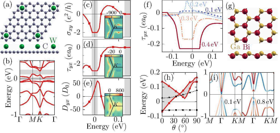
Figure 9.4: Monopole-driven spin-orbit torques in mixed Weyl semimetals. (a) Crystal structure of graphene decorated by W adatoms. (b) First-principles band structure of the perpendicularly magnetized film. The topologically non-trivial gap around the Fermi level and the trivial gap above are highlighted. (c)–(e) Energy dependence of anomalous Hall conductivity \sigma_{xy} , torkance \tau_{yx} , and spin polarization D_{yx} , respectively. In the latter case, the unit D_0 stands for \text{meV}a_0 per unit cell. Insets show the microscopic contributions in momentum space near the K -point. (f) Energy dependence of the torkance \tau_{yx} in a GaBi film upon applying an exchange field \mathbf{B} = B_0(\sin \theta, 0, \cos \theta) perpendicular to the film plane, where the numbers denote B_0 . (g) Crystal structure of the system. (h) Evolution of valence band top (squares) and conduction band bottom (triangles) with varying \theta for B_0 = 0.1 eV (black dashed lines) and B_0 = 0.8 eV (red solid lines). (i) Band structures for \theta = 0^\circ and two different values of B_0 , where colors illustrate the spin polarization normal to the film.
