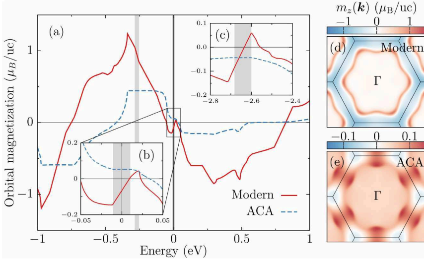
Figure 6.3: (a) Energy dependence of the out-of-plane orbital magnetization m_z in magnetically doped graphene with W adatoms. Red solid lines and blue dashed lines indicate the results based on the modern theory and the atom-centered approximation (ACA), respectively. The gray shaded areas highlight the band gaps with the non-zero Chern numbers \mathcal{C} = \pm 2 . (b) Zoom to the marked region around the Fermi level. (c) The behavior of m_z for Ir adatoms deposited in 2 \times 2 geometry on graphene reveals unique fingerprints of the topologically complex band gap with \mathcal{C} = +2 about 2.65 eV below the Fermi level. (d,e) Distribution of m_z(\mathbf{k}) in momentum space according to the modern theory and the ACA in the case of W adatoms. Note the different color scales.
