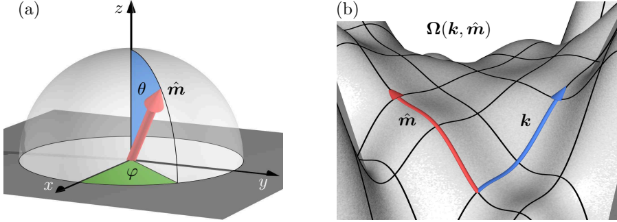
Figure 4.5: (a) The magnetization direction \hat{\mathbf{m}} can be represented in spherical coordinates using the polar angle \theta (blue) and the azimuthal angle \varphi (green). (b) Illustration of the complex phase space that entangles the crystal momentum \mathbf{k} with the dynamical magnetization direction \hat{\mathbf{m}} , resulting eventually in a non-trivial general Berry curvature \Omega(\mathbf{k}, \hat{\mathbf{m}}) .
