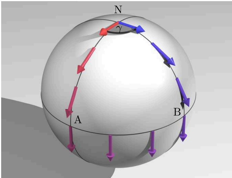
Figure 4.1: The parallel transport of a tangent vector on the sphere along a closed path from the north pole N over A and B and back to N results in a misalignment between original (dark red) and transported (dark blue) vector, owing to the non-trivial curvature on the sphere. The opening angle \gamma can be viewed as a geometric phase that manifests under parallel transport.
