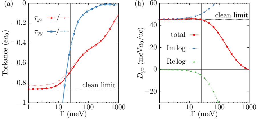
Figure 8.1: Dependence of (a) the torkance and (b) the spiralization on the constant band broadening \Gamma applied to the electronic structure of Mn/W(001). The behavior of \tau_{yx} and \tau_{yy} (dark solid lines) is compared in (a) to the disorder dependence obtained in Ref. [133] (light dotted lines). Additionally, the spiralization in (b) is decomposed into the two contributions entering Eq. (4.61), which are labeled accordingly as “Im log” and “Re log”. Dashed horizontal lines illustrate the Berry phase limit to which \tau_{yx} and D_{yx} converge for \Gamma \rightarrow 0 .
