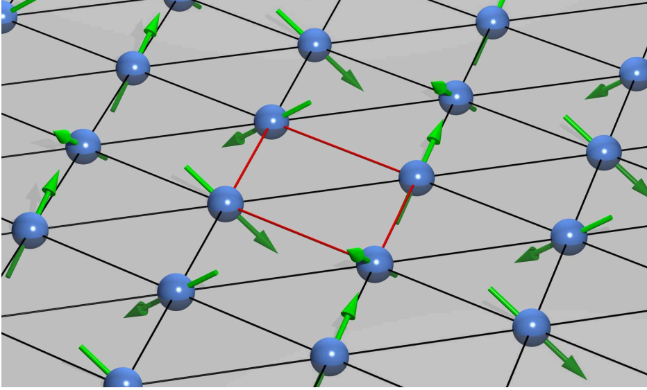
Figure 6.4: Non-coplanar 3Q spin texture on the triangular lattice formed by Mn atoms (blue balls) on a Cu(111) substrate (not shown). The red parallelogram denotes the magnetic unit cell of four atoms, and green arrows indicate the individual spin moments, which compensate over the entire unit cell.
