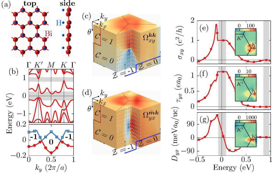
Figure 9.3: Magneto-electric properties of a mixed Weyl semimetal. (a) Top and side view of the semi-hydrogenated Bi(111) bilayer. (b) First-principles band structure for an out-of-plane magnetization, where the region of the topological band gap and the trivial one above are highlighted. Additionally, the evolution of valence band top (red circles) and conduction band bottom (blue squares) with k_y is shown. Bold integers denote the mixed Chern number \mathcal{Z} , and a is the in-plane lattice constant. (c,d) Distribution of momentum and mixed Berry curvatures in the complex phase space close to one of the emergent Weyl points. Gray arrows represent the direction of the curvature field (-\Omega_{yy}^{mk}, \Omega_{yx}^{mk}, \Omega_{xy}^{kk}) , and a logarithmic color scale is used to display two of its components, where dark red (dark blue) denotes large positive (negative) values. (e)–(g) Energy dependence of \sigma_{xy} , \tau_{yx} , and D_{yx} for a perpendicularly magnetized film. Insets show the microscopic contributions in momentum space near the inequivalent valleys K and K' .
