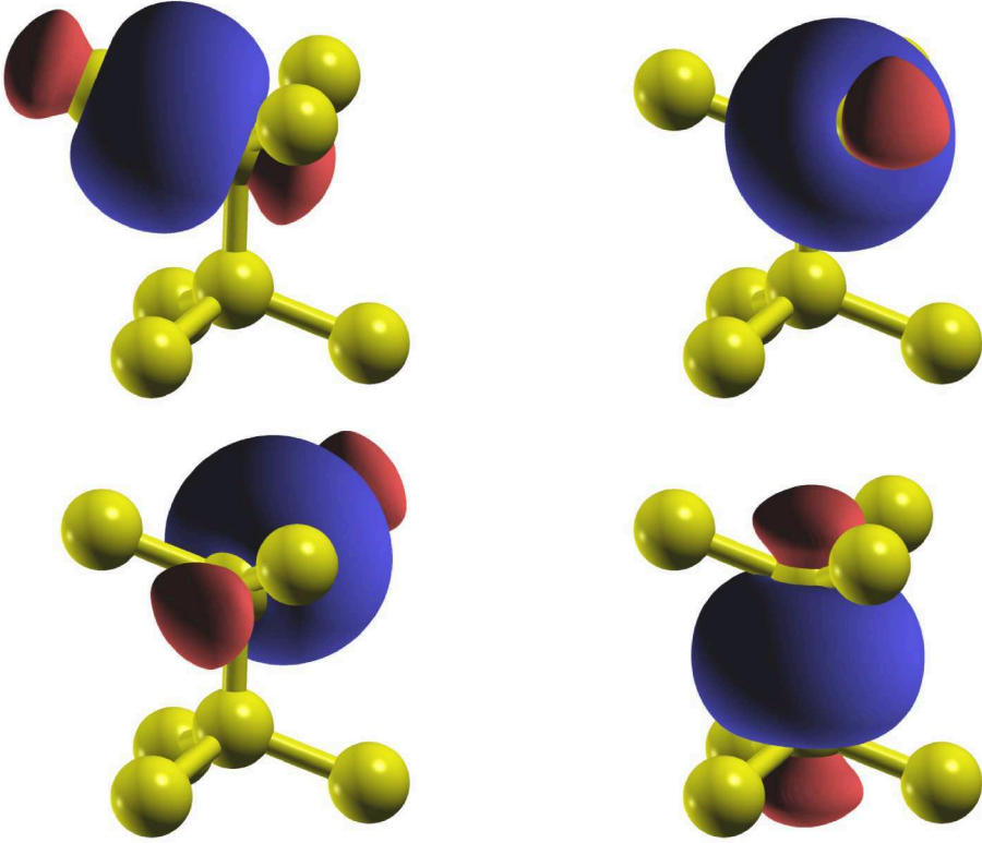
Figure 5.2: The maximally-localized Wannier functions extracted from the four valence bands of diamond reveal the covalent nature of the chemical bonding between the carbon atoms (yellow spheres). Red and blue colors denote positive and negative isosurface values, respectively.
