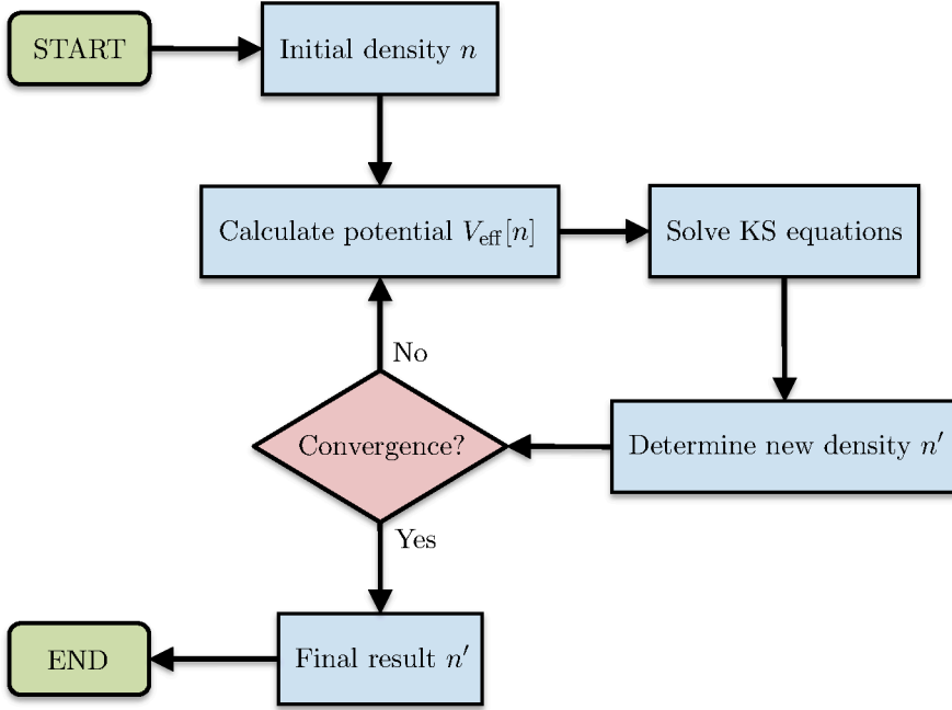
Figure 2.1: Self-consistency circle of density functional theory to determine the charge density n(\mathbf{r}) based on the Kohn-Sham approach (2.11).
