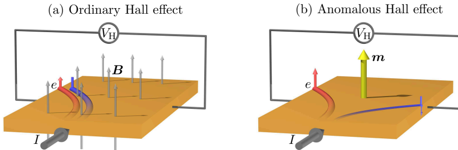
Figure 4.3: (a) Ordinary and (b) anomalous Hall effect due to the charge current I . While the transverse Hall voltage V_H in (a) originates from the applied magnetic field \mathbf{B} , the magnetization \mathbf{m} of a ferromagnet drives the anomalous Hall effect in (b). In the latter case, the resulting asymmetric charge distribution at the sample edges is accompanied by a finite spin polarization due to spin-dependent scattering processes.
