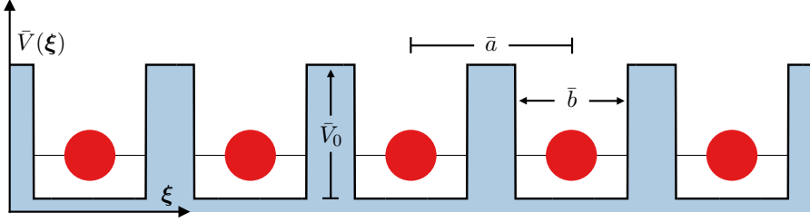
Figure 7.1: Periodic potential \bar{V}(\xi) in the auxiliary real space \xi . As discussed in the main text, the potential landscape of the one-dimensional chain of virtual atoms (red balls) is defined as series of finite potential wells of depth \bar{V}_0 , well width \bar{b} , and lattice constant \bar{a} .
