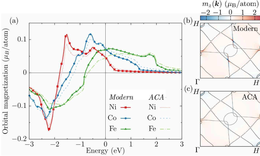
Figure 6.1: (a) Easy-axis orbital magnetization (OM) in the elementary bulk ferromagnets fcc Ni, hcp Co, and bcc Fe, either according to the modern theory (solid lines) or according to the atom-centered approximation (ACA, dashed lines). The OM is given in units of Bohr magneton per atom, and the shift of the Fermi level is measured with respect to the true Fermi energy. (b,c) Distribution of the \mathbf{k} -resolved OM m_z(\mathbf{k}) in bcc Fe based on the modern theory and the ACA, where the plane of k_x = 0 is considered, and \Gamma = (000) , H = (001) , and H'(010) in units of 2\pi over lattice constant.
