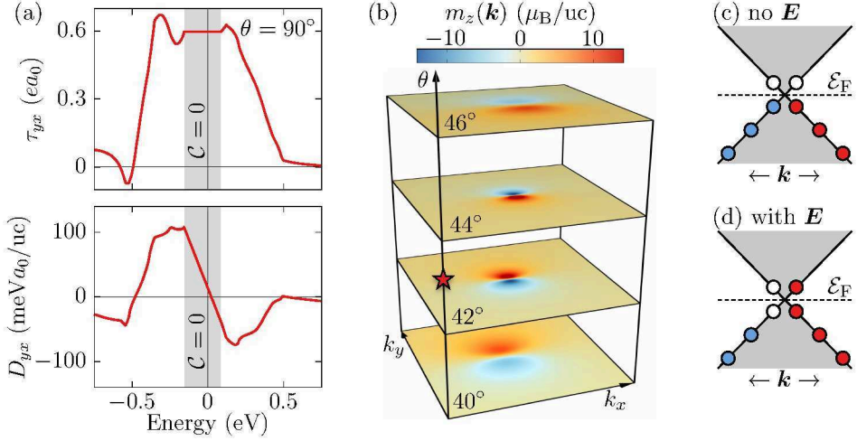
Figure 9.5: (a) Energy dependence of \tau_{yx} and D_{yx} in the functionalized bismuth film for an in-plane magnetization direction, where the shaded region illustrates the topologically trivial energy gap around the Fermi level. (b) Momentum-space distribution of the out-of-plane orbital magnetization (orbital magnetization (OM)) close to the mixed Weyl point that appears for \theta = 43^\circ (star). (c) In equilibrium, the states with positive (red) and negative (blue) local contributions to the OM are occupied equally, and open circles denote unoccupied states. (d) This population can be modified by an applied electric field \mathbf{E} to induce a large net OM.
