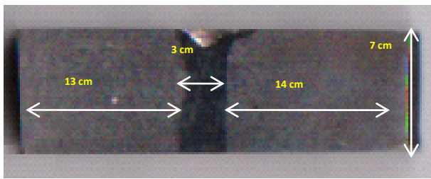
Figure 2. TIG Welding Macrostructure of the Polished Specimen After Cutting and Etching with A solution Containing 25 ml of HCl, 25 mL of H 2 O, and 2.5 ml of HNO 3
