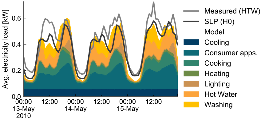
Figure 3.3: Example extraction of three days for the profile generated by 1000 runs of the load model, in comparison to the Standard Load Profile and an average profile of 74 measured residential buildings.
