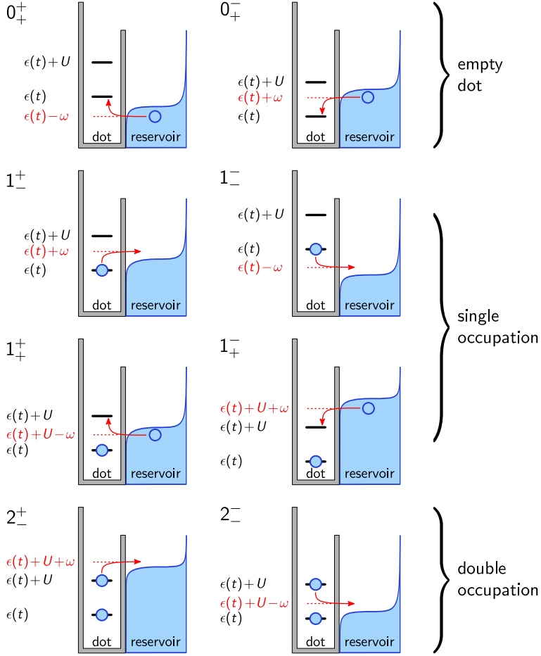
Figure 6.1: Sketch of fluctuation processes which are included in the instantaneous fluctuation vector in Eq. (6.3) for the spin-symmetric case, \epsilon_{\uparrow} = \epsilon_{\downarrow} ('single occupation' refers to mixed states of \uparrow and \downarrow ). The processes are denoted as 0^{\pm}_{\pm} , 1^{\pm}_{\pm} and 2^{\pm}_{\pm} , where the superscript indicates the temporal absorption or emission of the energy \omega during the fluctuation, while the subscript indicates if the occupation momentarily increases or decreases by one electron. Probabilities for individual processes are proportional to the occupation of the reservoir at the relevant energies. An additional Zeeman splitting would split each of the shown processes in two [see Fig. 6.3 (j)].
