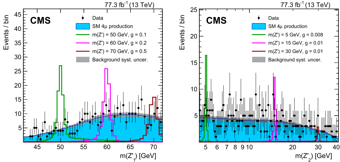
Fig. 4. Distributions of the reconstructed m(Z'_1) and m(Z'_2) observables and a comparison to the predicted q\bar{q}/gg \rightarrow 4\mu background. The variable bin width has been chosen according to the expected mass resolution. The blue histogram represents the expected SM 4\mu background distributions and the gray band shows the systematic uncertainty in its prediction. For illustration, three Z' signal hypotheses with different masses and coupling strengths are also shown by colored lines.
