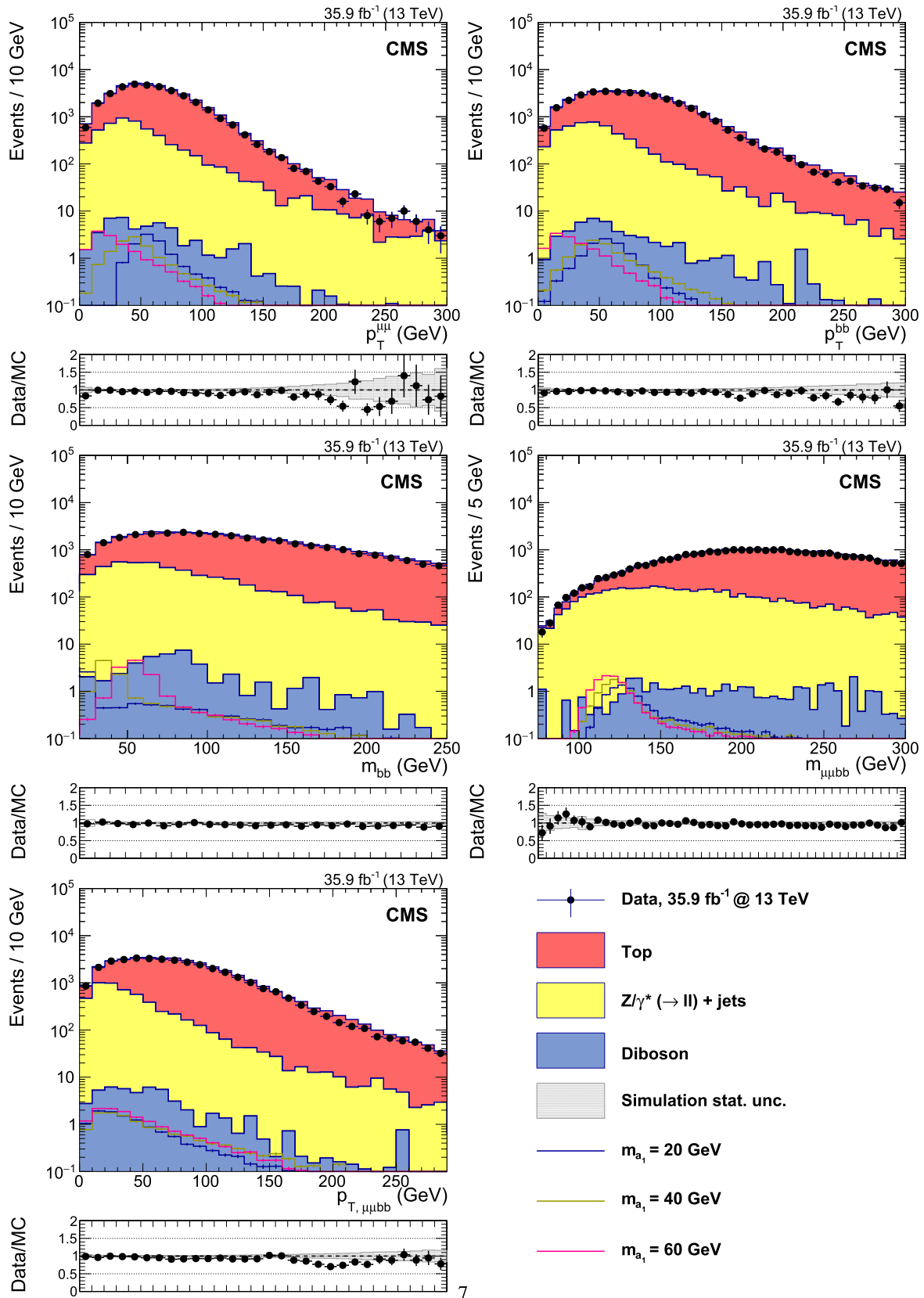
Fig. 3. The distribution of the p_T of the (top left) dimuon and (top right) di-b-jet system, the mass of the (middle left) di-b-jet and (middle right) \mu\mu b\bar{b} system, and (bottom left) the p_T of the \mu\mu b\bar{b} system, all after requiring two muons and two b-tagged jets in the event. Simulated samples are normalised to an integrated luminosity of 35.9 \text{ fb}^{-1} using their theoretical cross sections.
