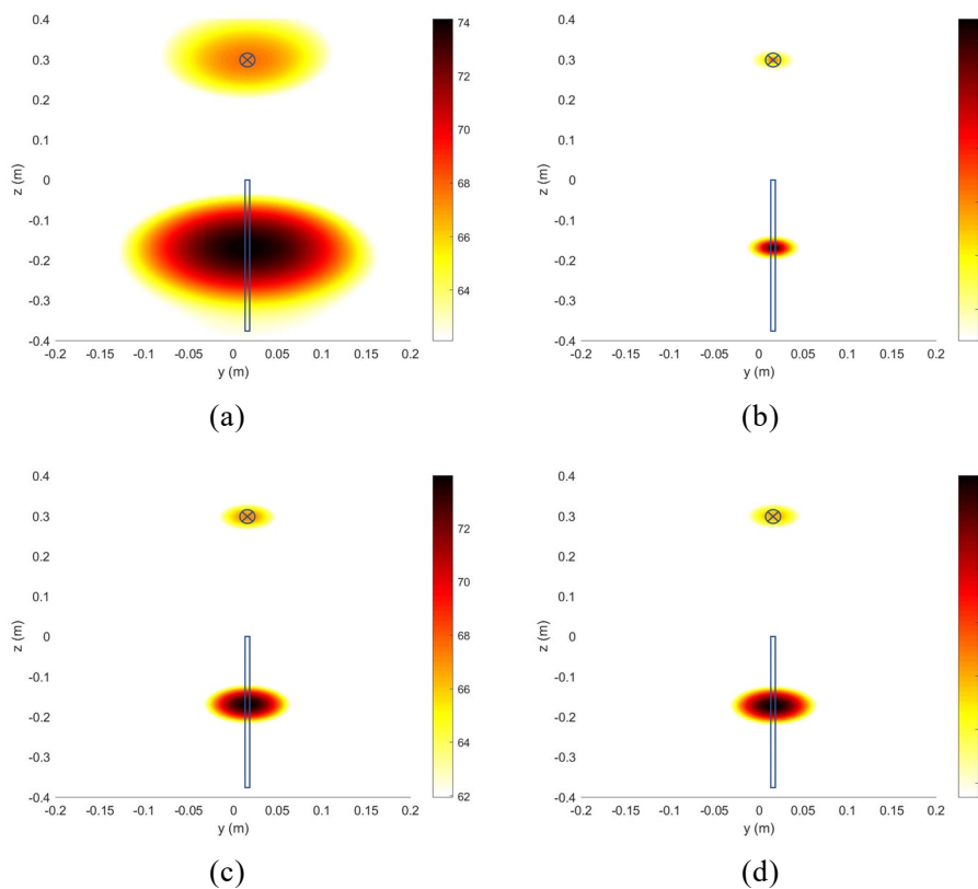
Figure 7 – Source maps of a monopole source and an Aeolian-tone dipole whose axis vertical to the array. Maps are produced by four beamforming algorithms, including (a) CB, (b) CLEAN-SC, (c) OB and (d) the multipole orthogonal beamforming.
