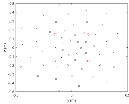
Figure 2 – The schematic representation of the simulation setup: the \times symbols denote the positions of microphones and the red circles denote the positions of sources. The microphone array was set parallelly 1m away from the source plane.
