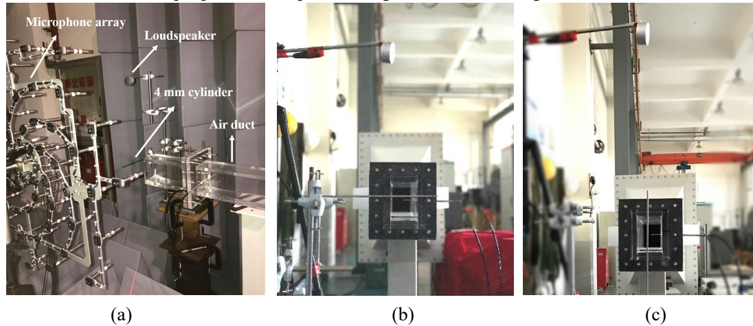
Figure 5 – The experimental setup to produce an Aeolian tone dipole source and a monopole source. (a) shows the trial facilities. (b) shows the setup for Case 1, which produces a dipole whose axis parallel to the array. (c) shows the setup for Case 2, which produces a dipole whose axis vertical to the array.
