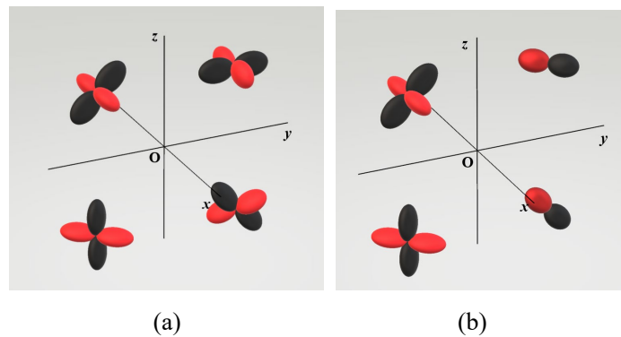
Figure 1 – The directivities of multipole sources in simulations. Case 1 (a) contained four quadrupoles and
