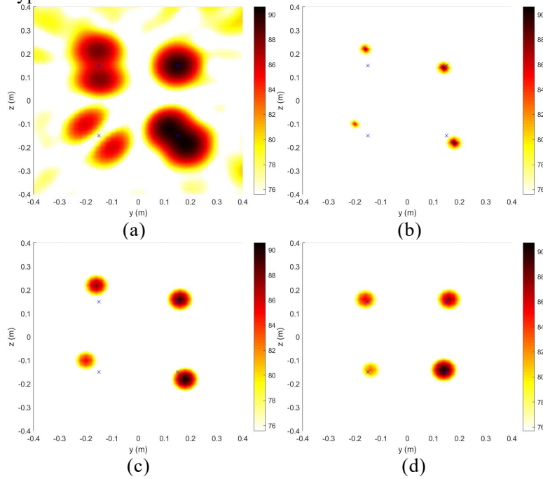
Figure 4 – Source maps of two dipoles and two quadrupoles with different orientations produced by four beamforming algorithms, including (a) CB, (b) CLEAN-SC, (c) OB and (d) the multipole orthogonal beamforming.
