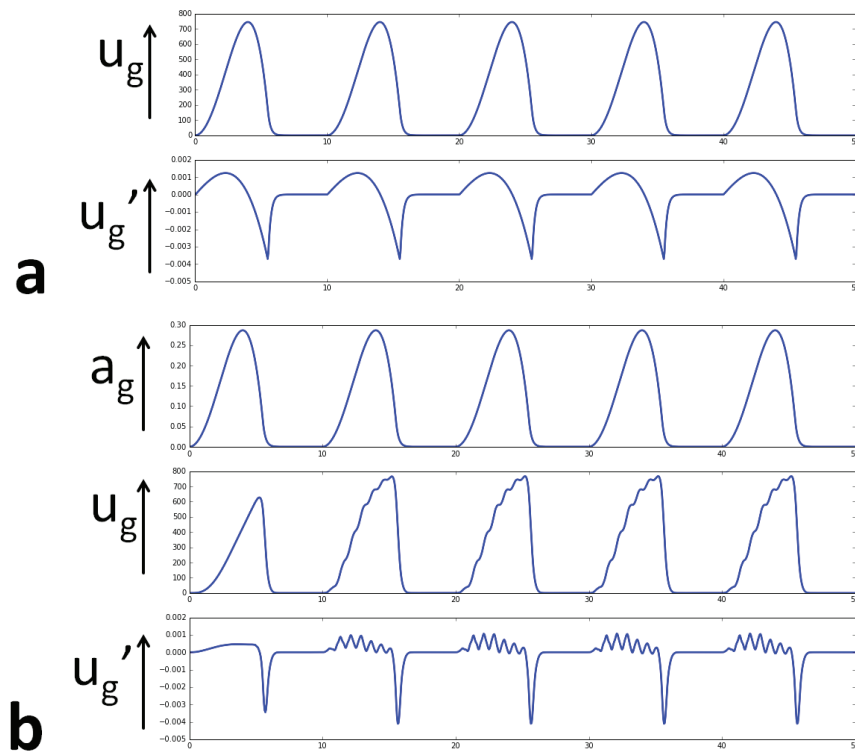
Figure 3 – Time signals for glottal flow u_g and its time derivative u_g' in a model without (model 1, top: a) and with source-filter interaction (model 2, bottom: b) for vowel /a/ and pulmonary pressure PP = 1200 Pa. In case of model 2 the glottal area function is plotted in addition to flow and time derivative of flow. The time axis is 50 msec and thus 5 glottal cycles are given ( F_0 = 100 Hz).
