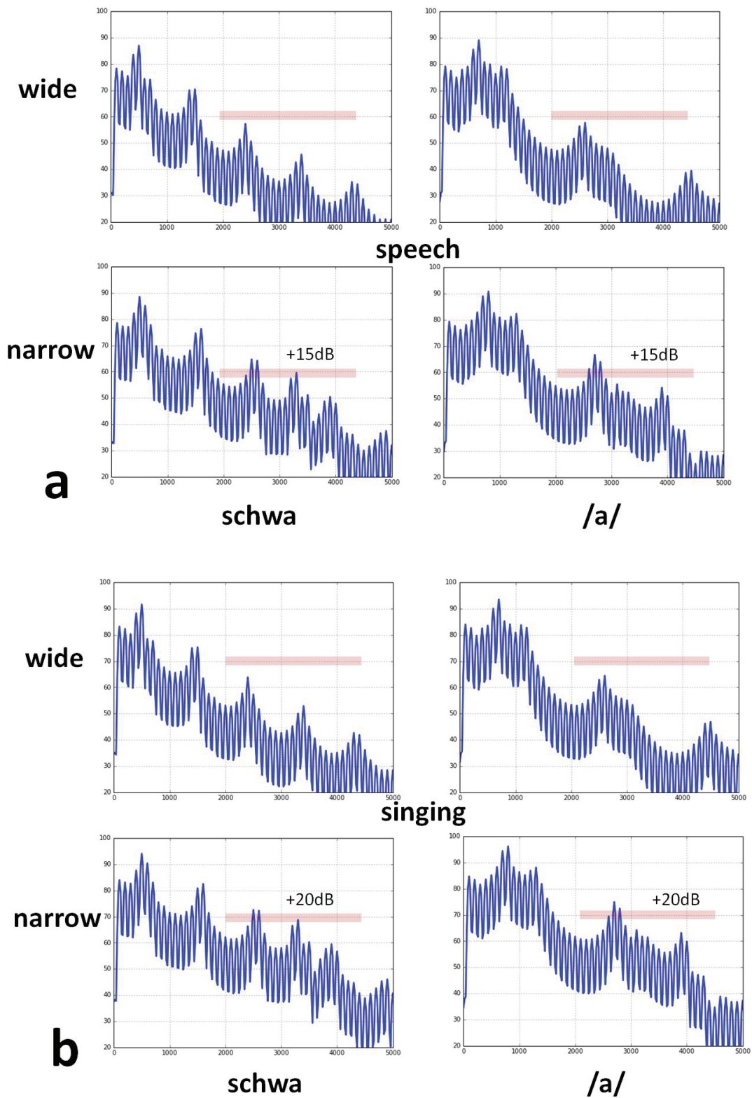
Figure 5: Spectra for schwa- and /a/-vowel and both laryngeal tube sizes using the model with acoustic-aerodynamic interaction (model 2) for speech (a: PP = 600 Pa) and singing (b: p_{\text{sub}} = 1200 Pa) (cases 1 to 8 in table 1). Frequency scale: 0 to 5 kHz; relative amplitude scale covers a range of 80 dB.
