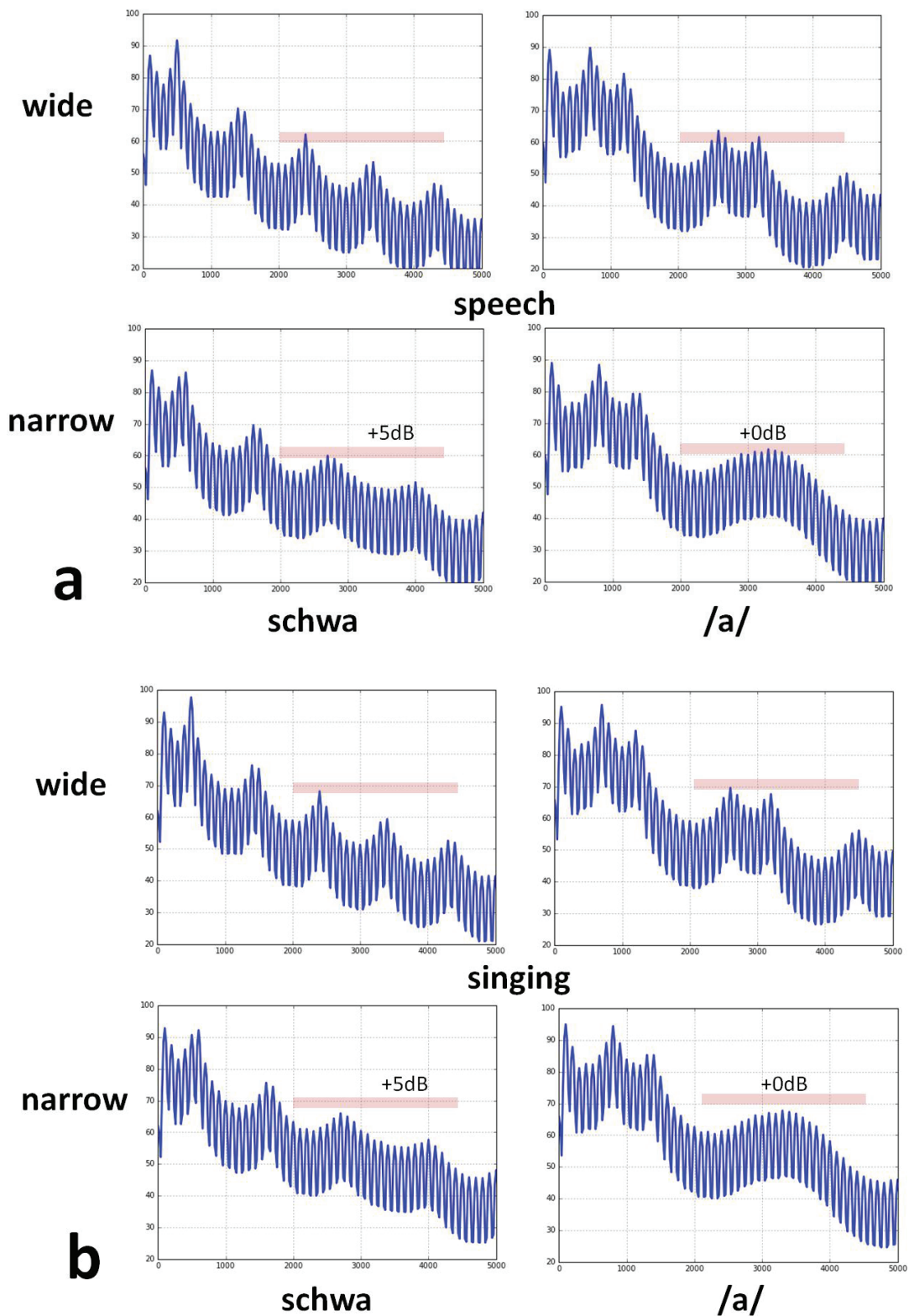
Figure 4: Spectra for schwa- and /a/-vowel and both laryngeal tube sizes using the model without acoustic-aerodynamic interaction (model1) for speech (a: PP = 600 Pa) and singing (b: Pa = 1200 Pa) (cases 1 to 8 in table 1). Frequency scale: 0 to 5 kHz; relative amplitude scale covers a range of 80 dB.
