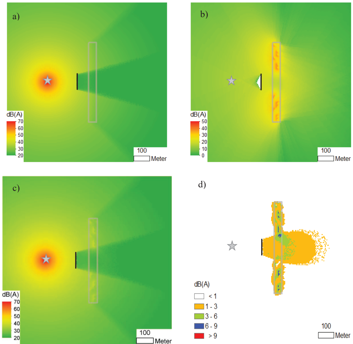
Figure 6 – Sound exposure map with a 50 m deep forest of 500 m length and a barrier of 100 m length in front of the forest. a) Direct sound, b) Reflected sound, c) Direct and reflected sound, d) Level increase because of forest reflections.
