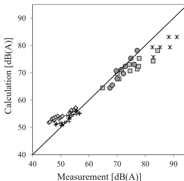
Figure 2 – Comparison of measured vs. calculated A-weighted attenuations.
