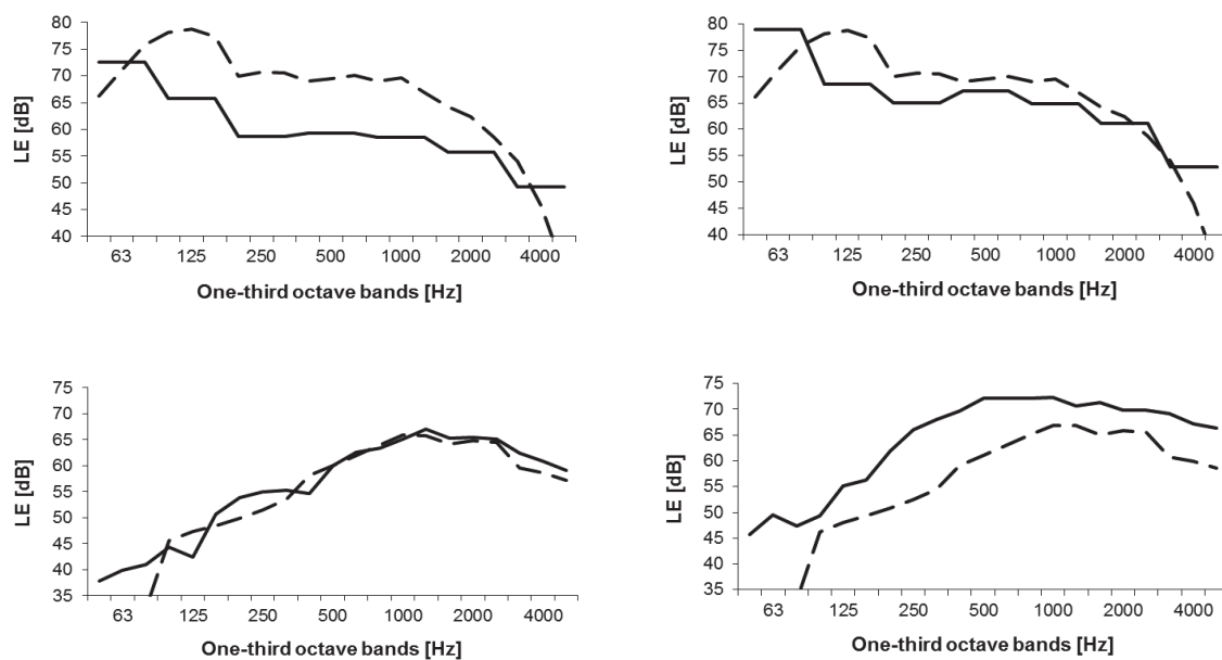
Figure 3 – Examples of measured (bold line) vs. calculated (dashed line) sound exposure level. Upper two examples: explosions of 200 gr TNT, propagation distance 680 m, unfavorable (left) and favorable (right) sound propagation conditions. Lower two examples: signal pistol, propagation distance 50 m, softwood forest (left) and hardwood forest with low-hanging thick branches (right).
