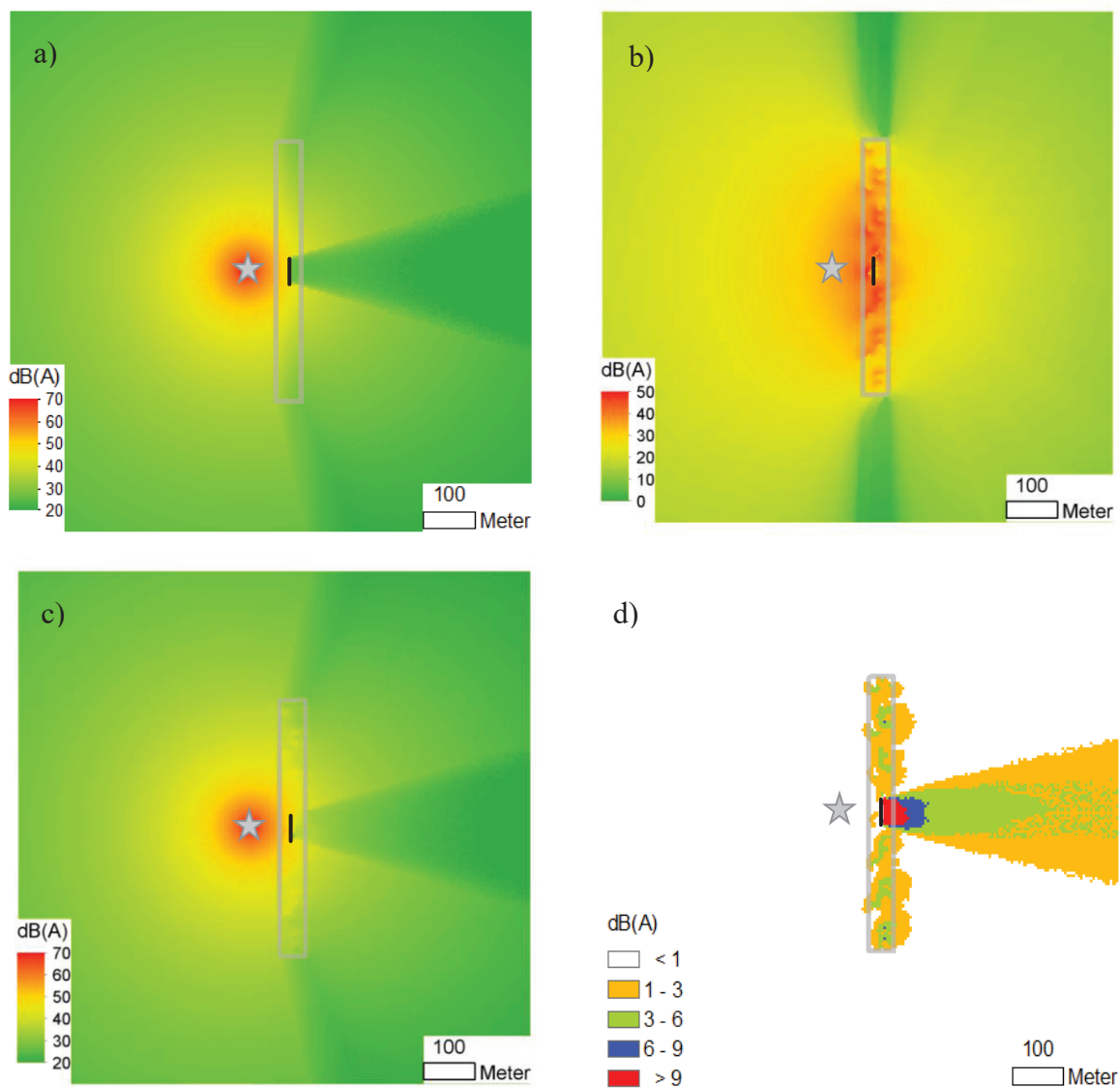
Figure 5 – Sound exposure maps with a 50 m deep forest of 500 m length and a barrier of 50 m length in the forest. a) Direct sound, b) Reflected sound, c) Direct and reflected sound, d) Level increase because of forest reflections.
