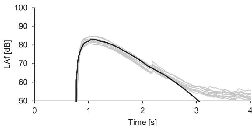
Figure 4 – Examples of measured (grey lines) vs. calculated (black line) level vs. time pattern.
