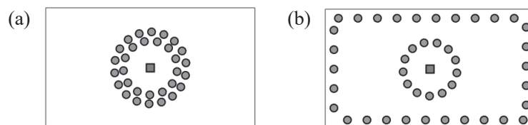
Figure 2 – Actuator array configured in double layer: (a) double circular array, (b) circular array and edge array located at the periphery of the plate.
