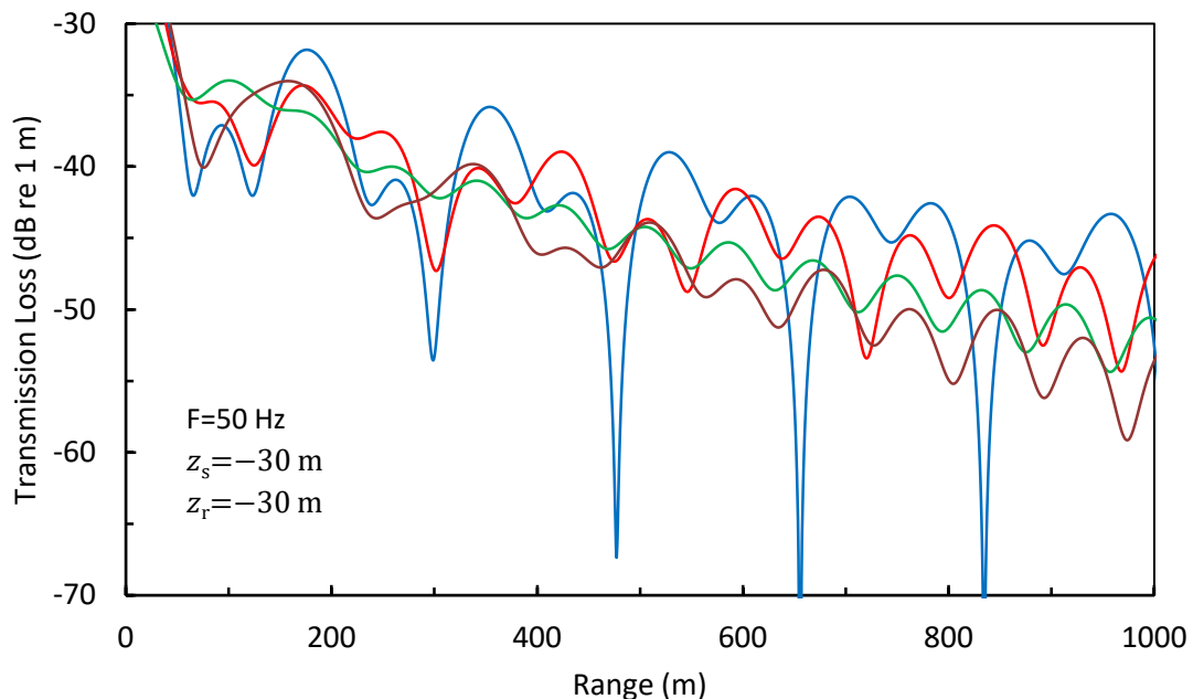
Figure 6 – TL for seabed with 10 m layer of sand with varying properties, above 300 m layer of limestone with fixed properties. — blue — ; c_T = 400 m/s; — red — ; c_T = 600 m/s; — green — c_T = 200 m/s; — brown — ; c_T = 300 m/s.
