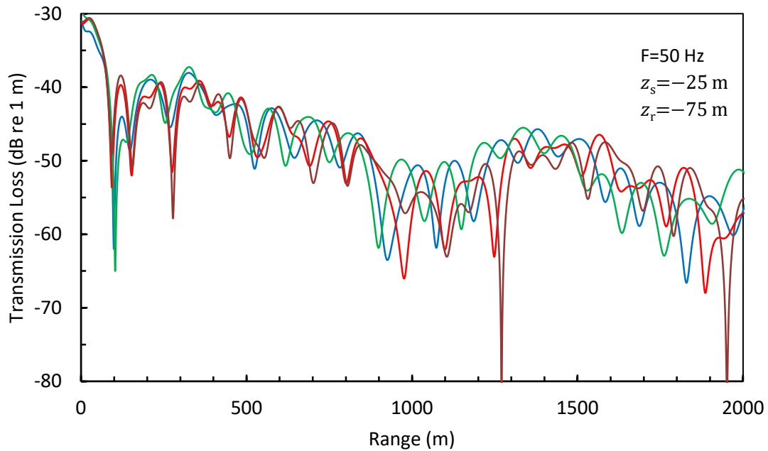
Figure 5 – TL for seabed with 10 m layer of sand with fixed properties, above 300 m layer of limestone with varying properties. — blue — ; c_T = 1315 m/s; — red — ; c_T = 1000 m/s; — green — c_T = 1600 m/s; — brown — ; c_T = 1200 m/s.
