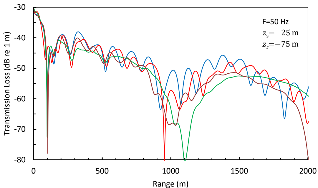
Figure 4 – TL for seabed with 10 m layer of sand with varying properties, above 300 m layer of limestone with fixed properties. — ; c_T = 400 m/s; — ; c_T = 600 m/s; — ; c_T = 200 m/s; — ; c_T = 300 m/s.
